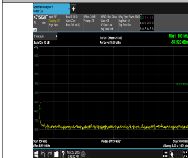
Band2-1.4MHz-16QAM-18900-1RB#0-0.15~30-PASS
