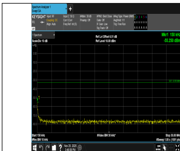
Band2-1.4MHz-QPSK-18900-1RB#5-0.15~30-PASS
