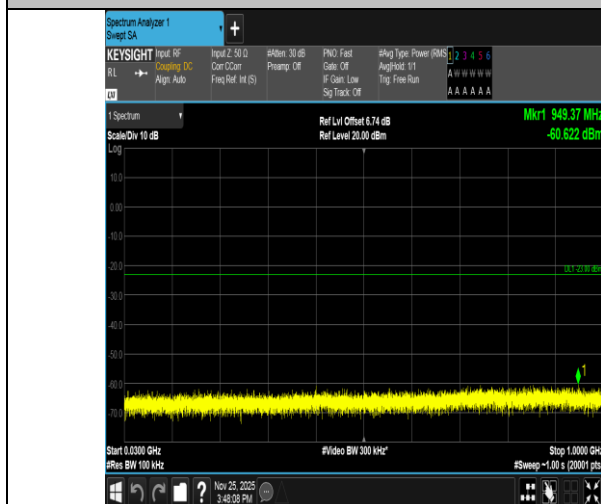
Band2-1.4MHz-16QAM-18900-1RB#5-30~1000-PASS
