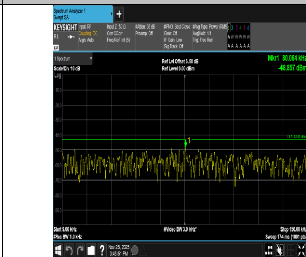
Band2-1.4MHz-16QAM-18900-1RB#0-0.009~0.15-PASS
