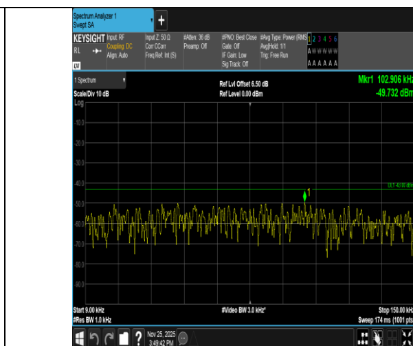
Band2-1.4MHz-16QAM-18900-6RB#0-0.009~0.15-PASS
