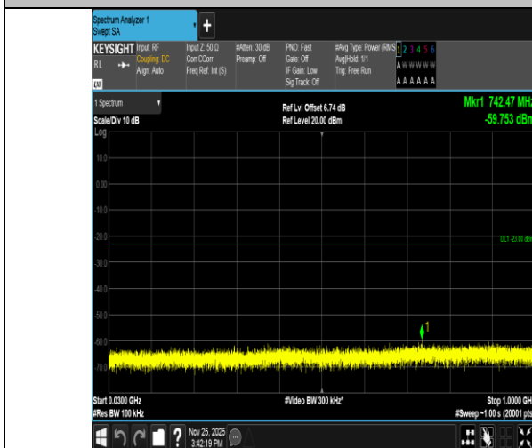
Band2-1.4MHz-16QAM-18607-1RB#5-30~1000-PASS
