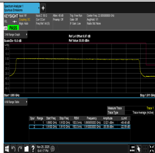
Band2-15MHz-16QAM-19125-75RB#0-PASS
