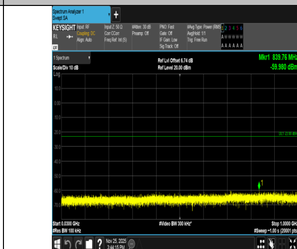
Band2-1.4MHz-16QAM-18607-6RB#0-30~1000-PASS
