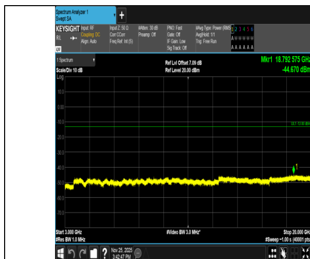
Band2-1.4MHz-16QAM-18607-1RB#5-3000~20000-PASS
