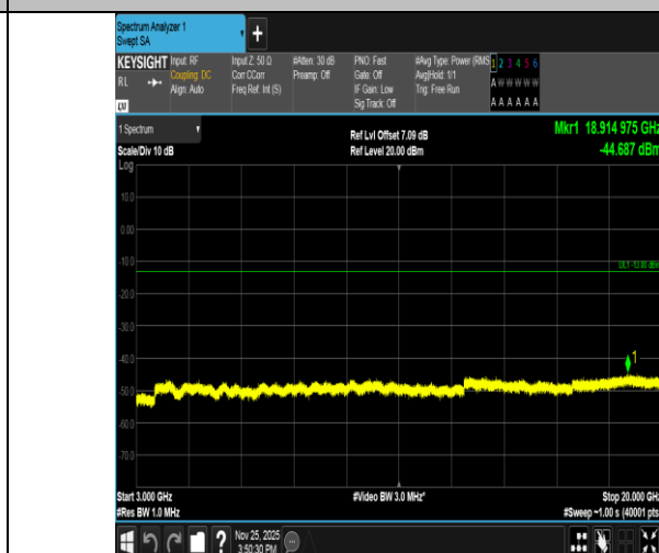
Band2-1.4MHz-16QAM-18900-6RB#0-3000~20000-PASS
