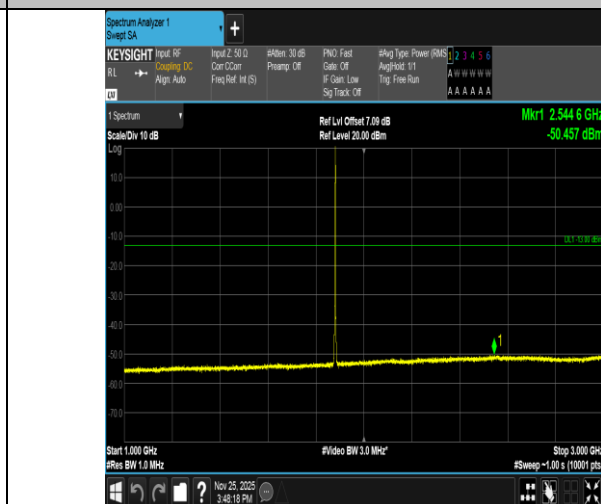
Band2-1.4MHz-16QAM-18900-1RB#5-1000~3000-PASS
