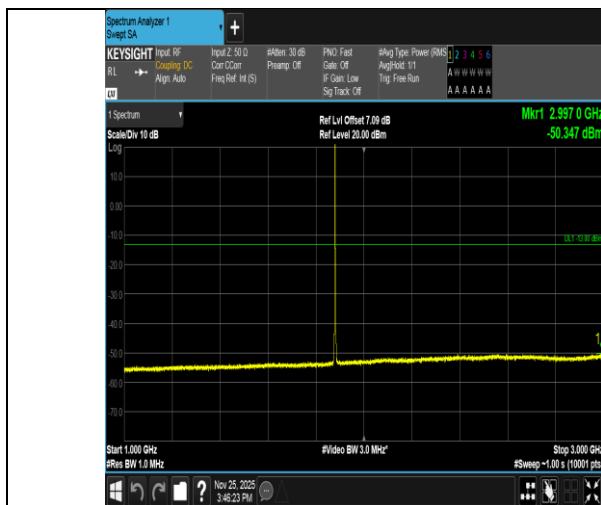
Band2-1.4MHz-16QAM-18900-1RB#0-1000~3000-PASS
