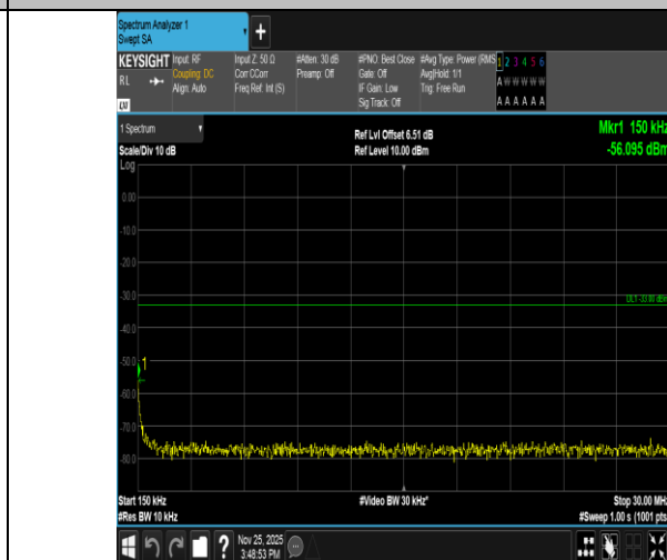
Band2-1.4MHz-QPSK-18900-6RB#0-0.15~30-PASS
