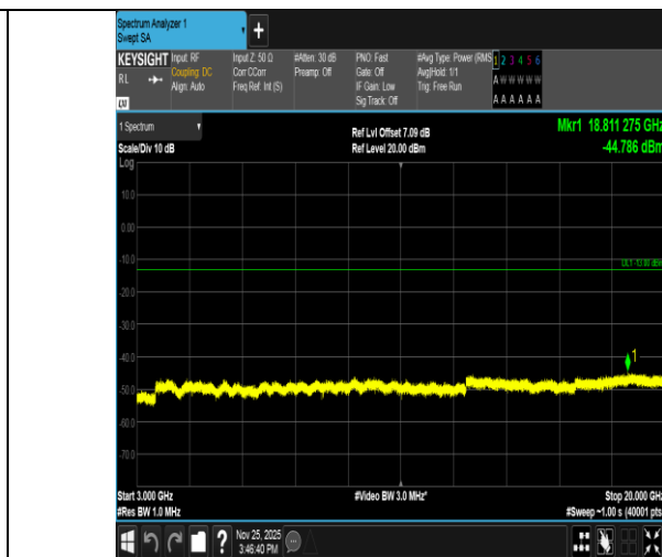
Band2-1.4MHz-16QAM-18900-1RB#0-3000~20000-PASS
