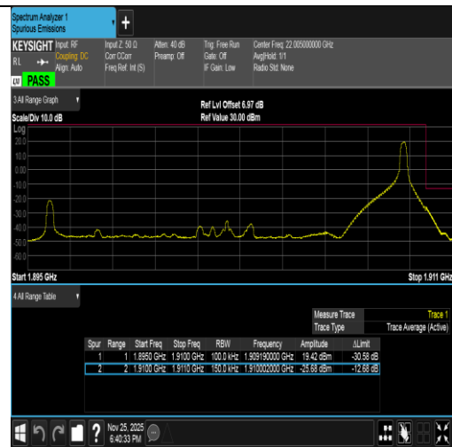
Band2-15MHz-QPSK-19125-1RB#74-PASS
