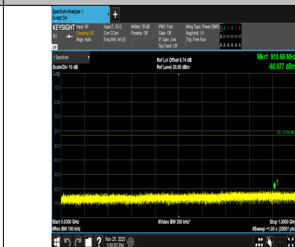
Band2-1.4MHz-16QAM-18900-6RB#0-30~1000-PASS
