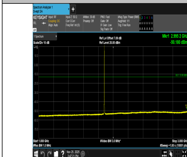
Band2-1.4MHz-QPSK-18900-1RB#5-1000~3000-PASS
