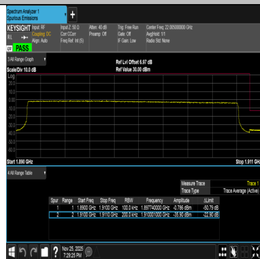
Band2-20MHz-16QAM-19100-100RB#0-PASS
