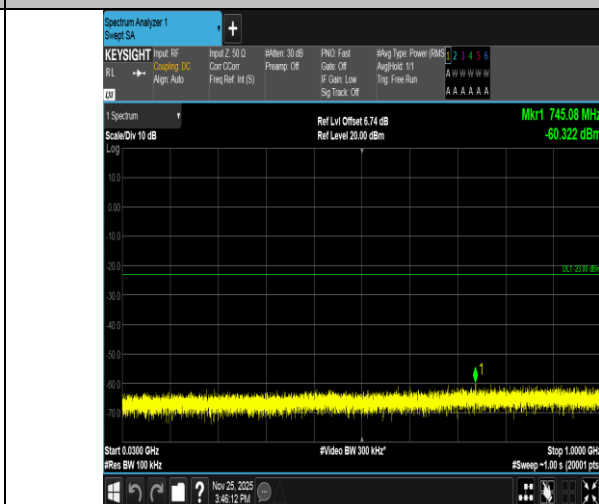
Band2-1.4MHz-16QAM-18900-1RB#0-30~1000-PASS
