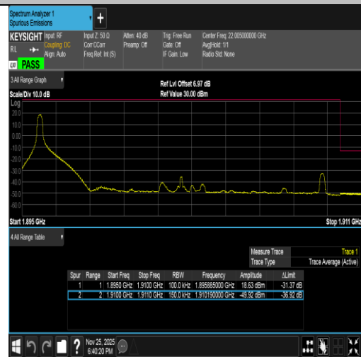
Band2-15MHz-16QAM-19125-1RB#0-PASS
