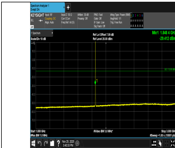
Band2-1.4MHz-16QAM-18607-1RB#0-1000~3000-PASS
