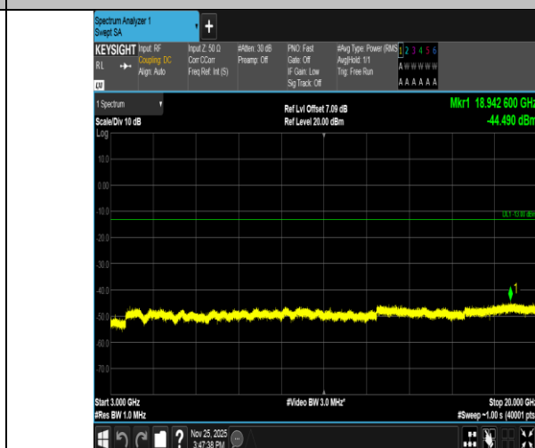
Band2-1.4MHz-QPSK-18900-1RB#5-3000~20000-PASS
