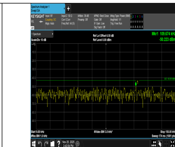
Band2-1.4MHz-16QAM-18607-6RB#0-0.009~0.15-PASS
