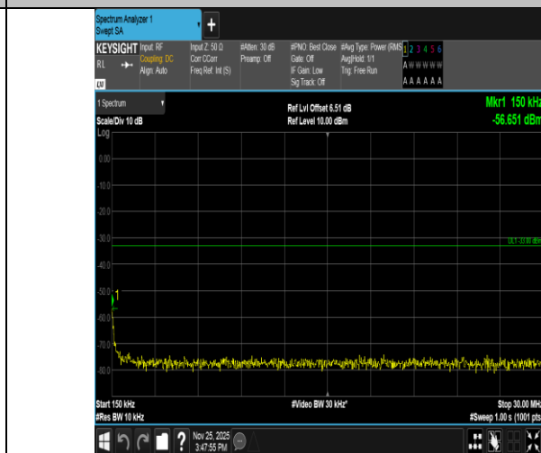
Band2-1.4MHz-16QAM-18900-1RB#5-0.15~30-PASS
