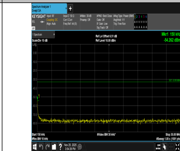
Band2-1.4MHz-QPSK-19193-6RB#0-0.15~30-PASS
