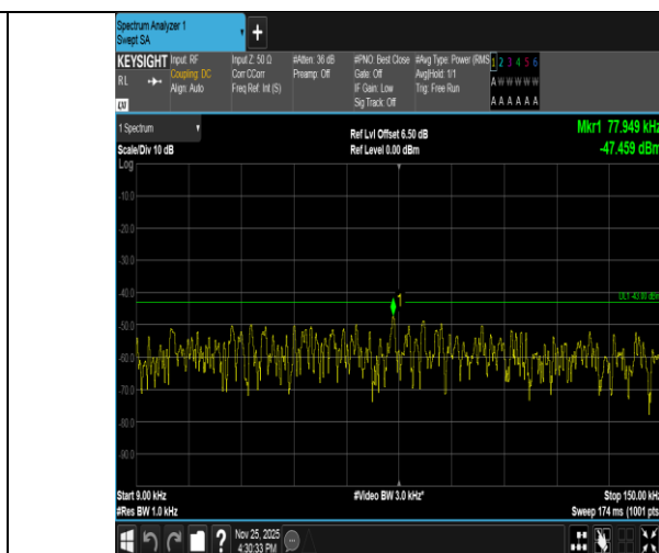
Band2-3MHz-16QAM-18615-15RB#0-0.009~0.15-PASS
