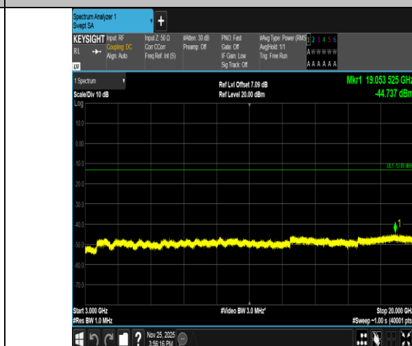
Band2-1.4MHz-16QAM-19193-6RB#0-3000~20000-PASS
