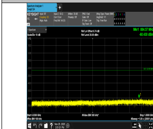
Band2-1.4MHz-QPSK-19193-1RB#0-30~1000-PASS
