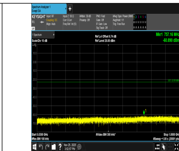
Band2-1.4MHz-QPSK-19193-1RB#5-30~1000-PASS
