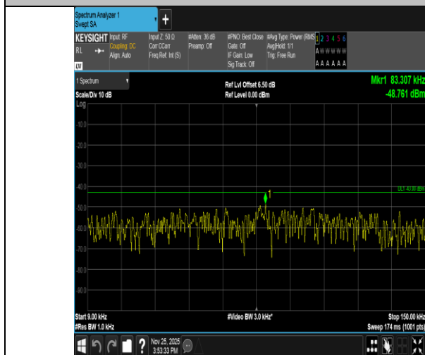
Band2-1.4MHz-16QAM-19193-1RB#5-0.009~0.15-PASS
