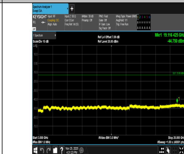
Band2-3MHz-16QAM-18615-15RB#0-3000~20000-PASS
