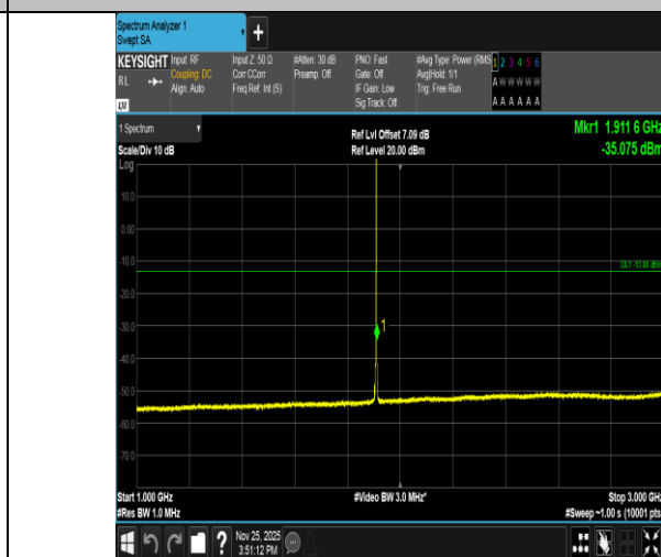
Band2-1.4MHz-QPSK-19193-1RB#0-1000~3000-PASS
