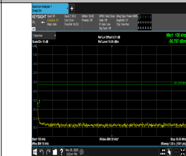
Band2-1.4MHz-16QAM-19193-1RB#5-0.15~30-PASS
