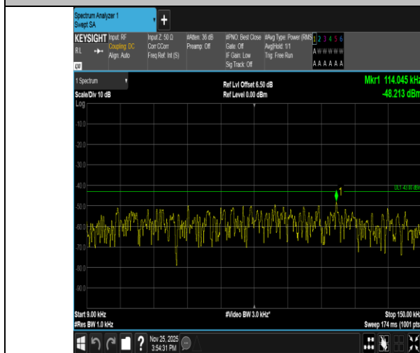
Band2-1.4MHz-QPSK-19193-6RB#0-0.009~0.15-PASS
