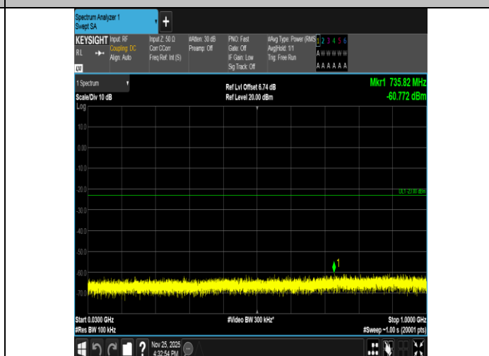
Band2-3MHz-16QAM-18900-1RB#0-30~1000-PASS
