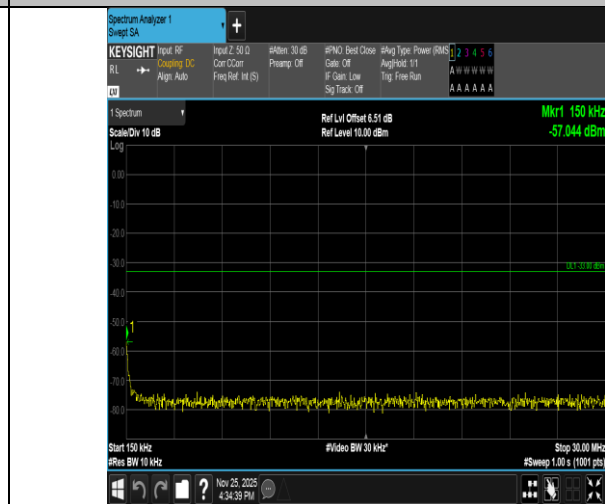
Band2-3MHz-16QAM-18900-1RB#14-0.15~30-PASS
