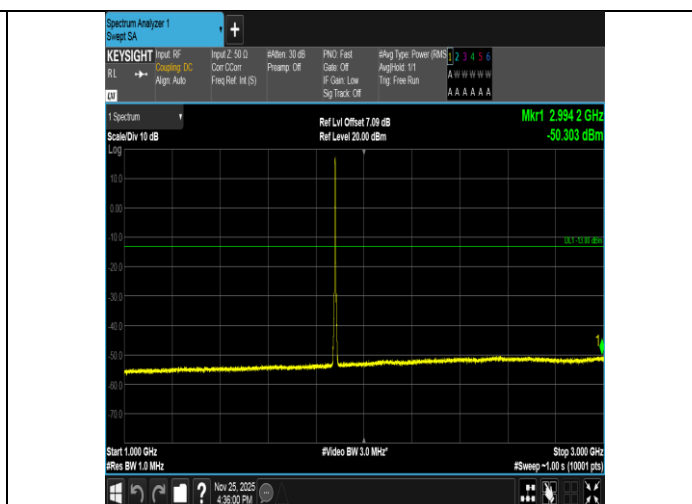
Band2-3MHz-QPSK-18900-15RB#0-1000~3000-PASS
