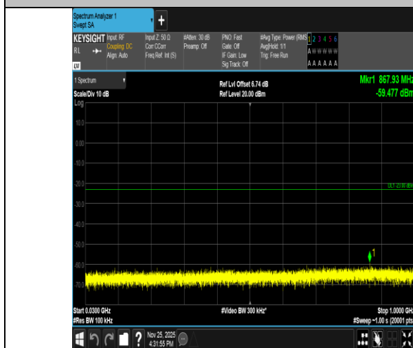
Band2-3MHz-QPSK-18900-1RB#0-30~1000-PASS
