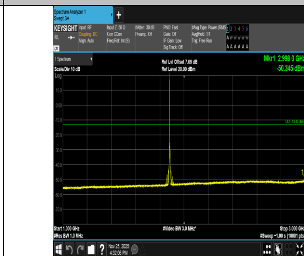
Band2-3MHz-QPSK-18900-1RB#0-1000~3000-PASS
