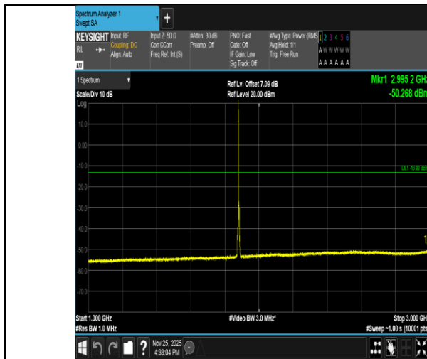
Band2-3MHz-16QAM-18900-1RB#0-1000~3000-PASS
