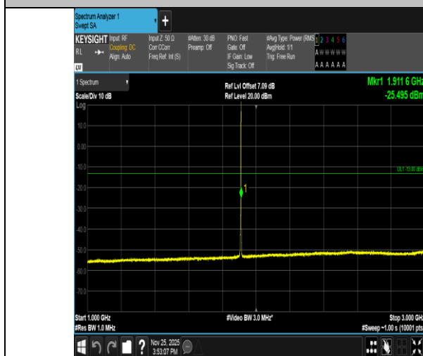
Band2-1.4MHz-QPSK-19193-1RB#5-1000~3000-PASS
