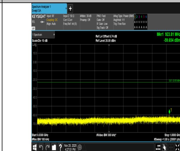
Band2-3MHz-16QAM-18615-1RB#0-30~1000-PASS
