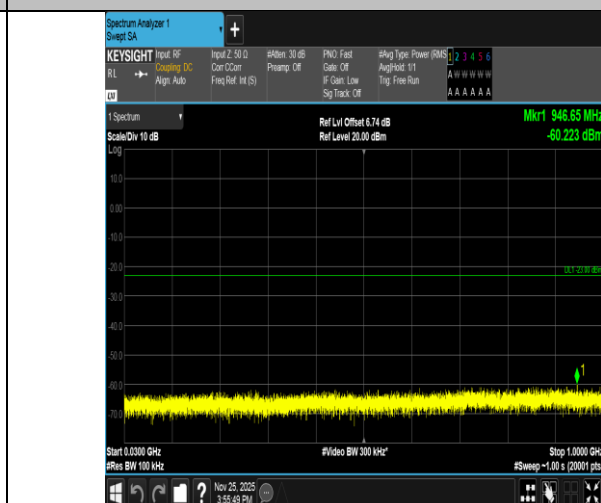
Band2-1.4MHz-16QAM-19193-6RB#0-30~1000-PASS
