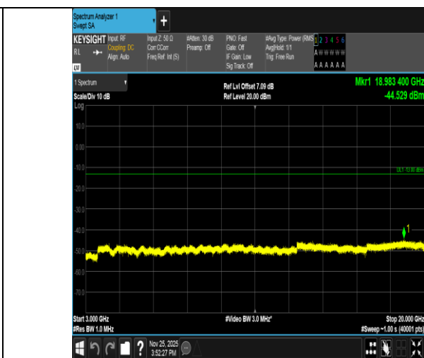
Band2-1.4MHz-16QAM-19193-1RB#0-3000~20000-PASS
