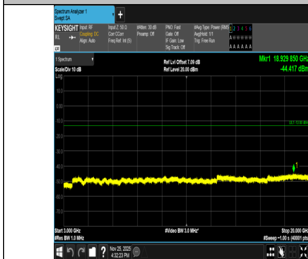
Band2-3MHz-QPSK-18900-1RB#0-3000~20000-PASS
