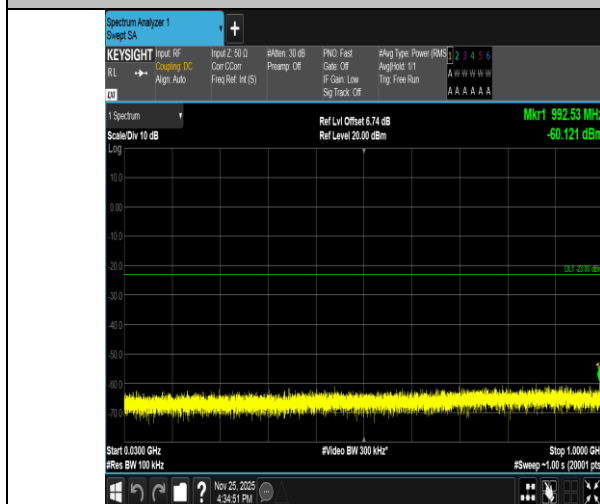
Band2-3MHz-16QAM-18900-1RB#14-30~1000-PASS
