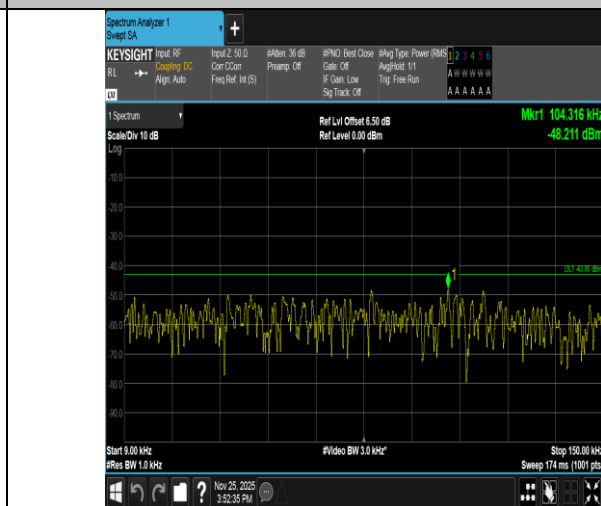
Band2-1.4MHz-QPSK-19193-1RB#5-0.009~0.15-PASS
