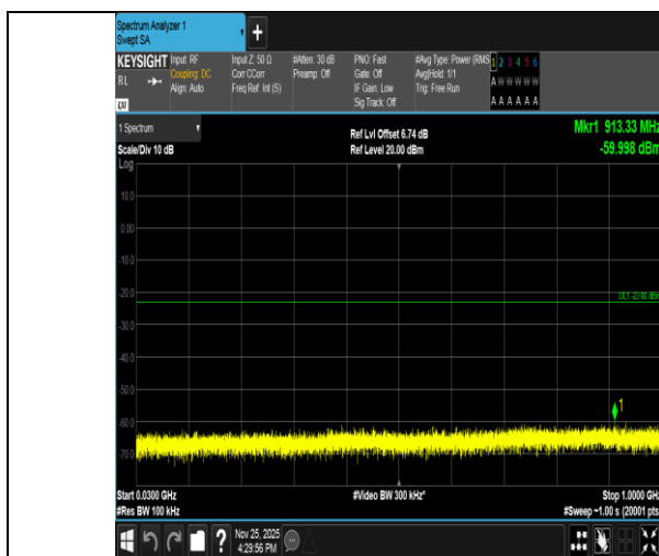
Band2-3MHz-QPSK-18615-15RB#0-30~1000-PASS
