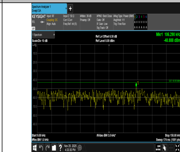
Band2-3MHz-QPSK-18900-1RB#14-0.009~0.15-PASS
