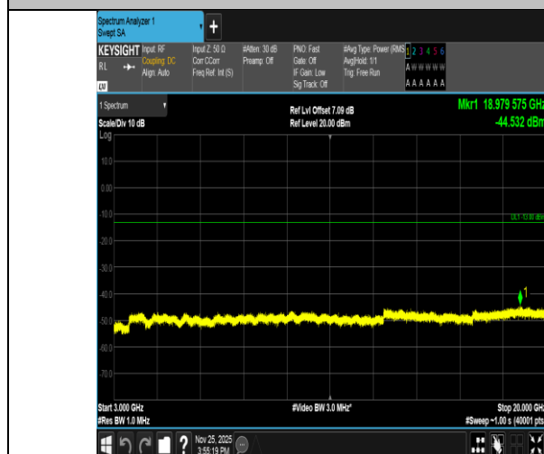
Band2-1.4MHz-QPSK-19193-6RB#0-3000~20000-PASS
