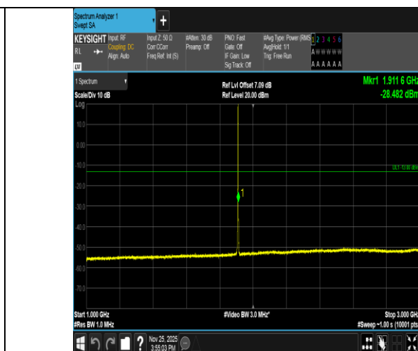
Band2-1.4MHz-QPSK-19193-6RB#0-1000~3000-PASS
