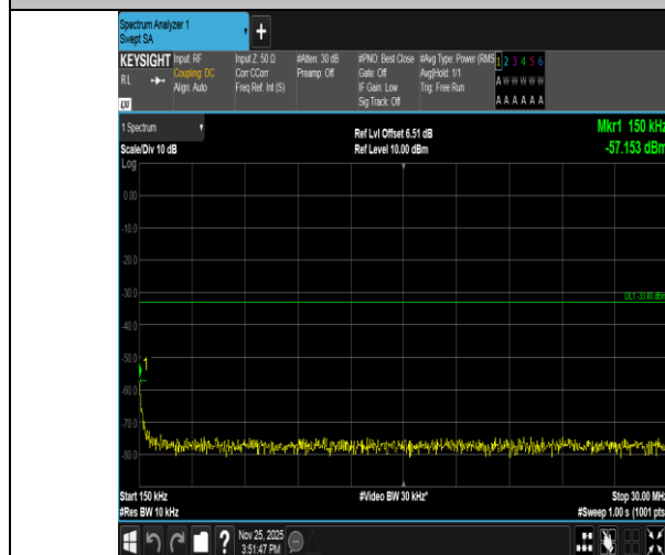
Band2-1.4MHz-16QAM-19193-1RB#0-0.15~30-PASS
