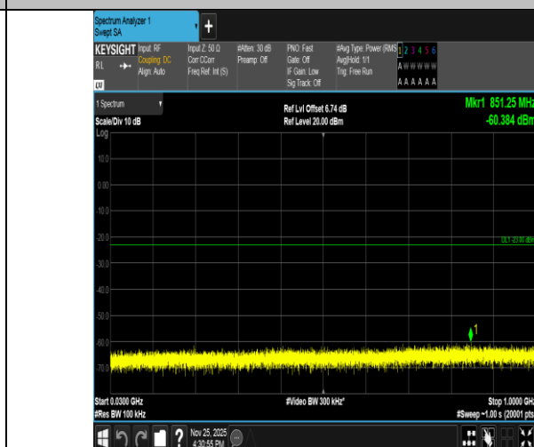
Band2-3MHz-16QAM-18615-15RB#0-30~1000-PASS
