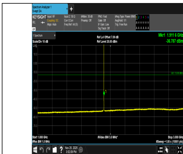
Band2-1.4MHz-16QAM-19193-1RB#0-1000~3000-PASS
