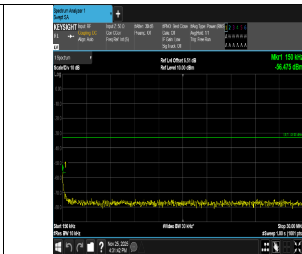
Band2-3MHz-QPSK-18900-1RB#0-0.15~30-PASS
