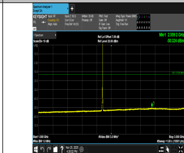
Band2-3MHz-16QAM-18900-1RB#14-1000~3000-PASS
