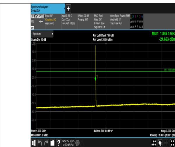
Band2-3MHz-QPSK-18615-15RB#0-1000~3000-PASS
