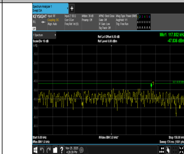
Band2-3MHz-16QAM-18615-1RB#0-0.009~0.15-PASS
