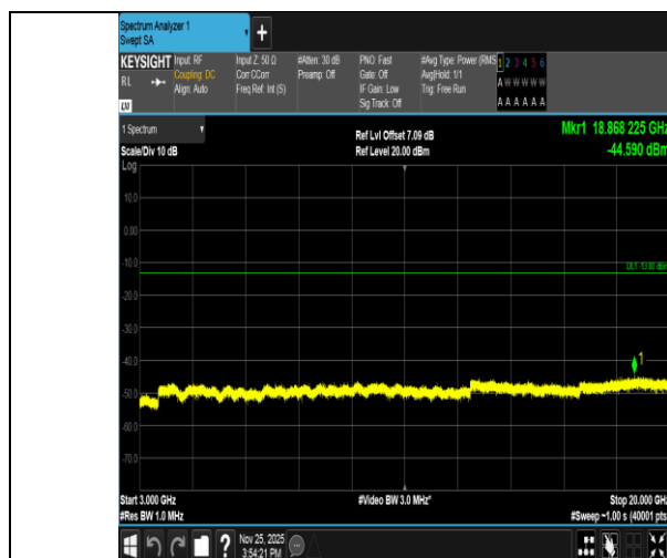
Band2-1.4MHz-16QAM-19193-1RB#5-3000~20000-PASS
