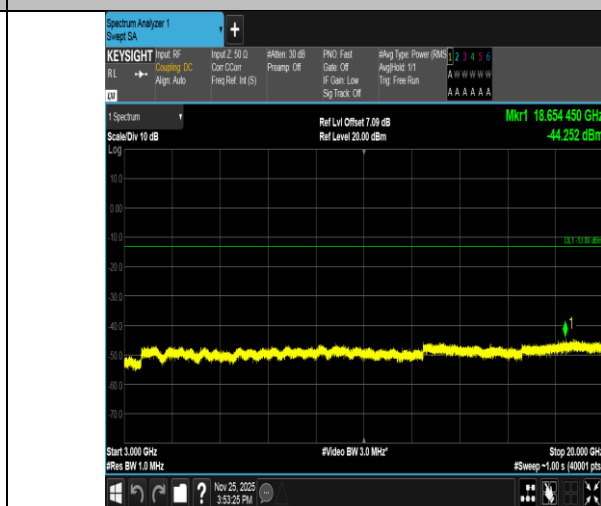
Band2-1.4MHz-QPSK-19193-1RB#5-3000~20000-PASS
