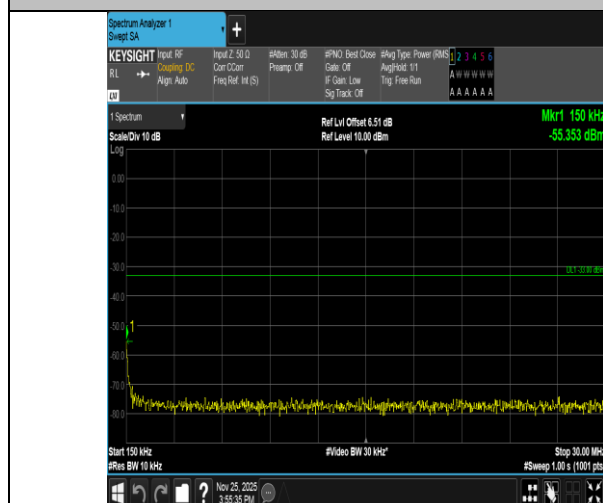
Band2-1.4MHz-16QAM-19193-6RB#0-0.15~30-PASS
