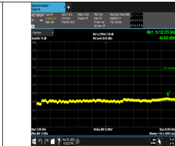
Band2-3MHz-16QAM-18900-1RB#0-3000~20000-PASS
