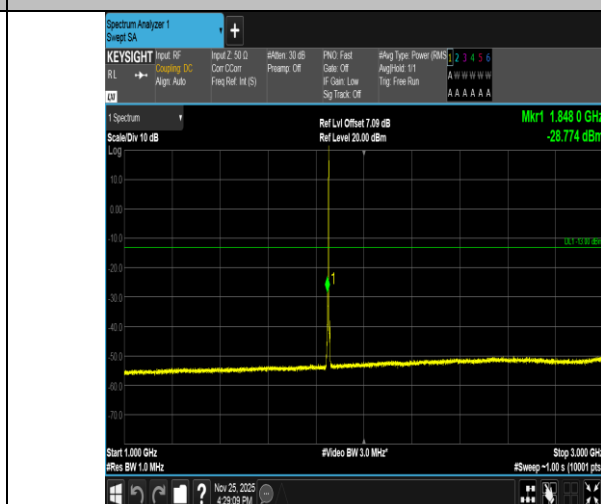
Band2-3MHz-16QAM-18615-1RB#14-1000~3000-PASS
