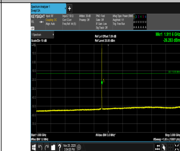
Band2-1.4MHz-16QAM-19193-1RB#5-1000~3000-PASS
