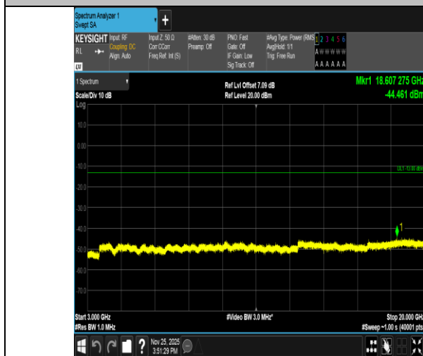
Band2-1.4MHz-QPSK-19193-1RB#0-3000~20000-PASS
