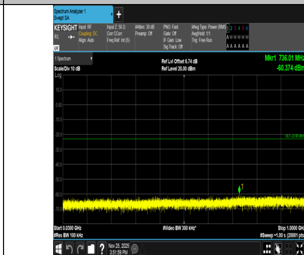
Band2-1.4MHz-16QAM-19193-1RB#0-30~1000-PASS
