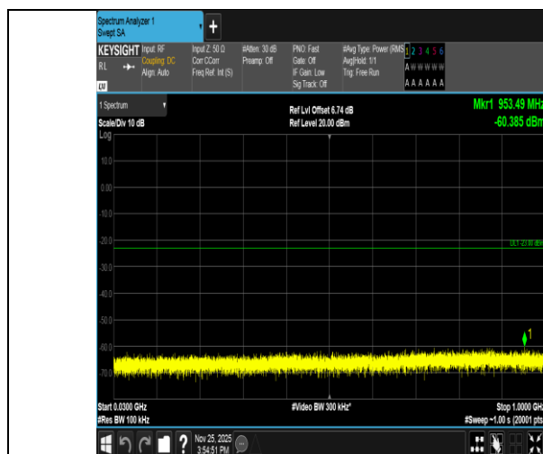
Band2-1.4MHz-QPSK-19193-6RB#0-30~1000-PASS
