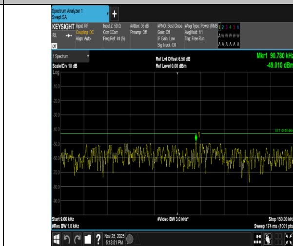
Band2-5MHz-QPSK-18625-1RB#24-0.009~0.15-PASS
