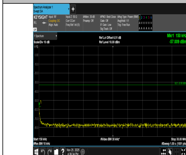
Band2-3MHz-16QAM-18900-15RB#0-0.15~30-PASS
