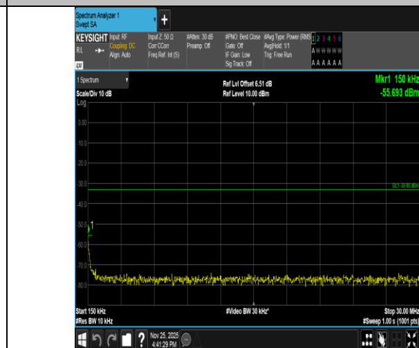
Band2-3MHz-QPSK-19185-15RB#0-0.15~30-PASS
