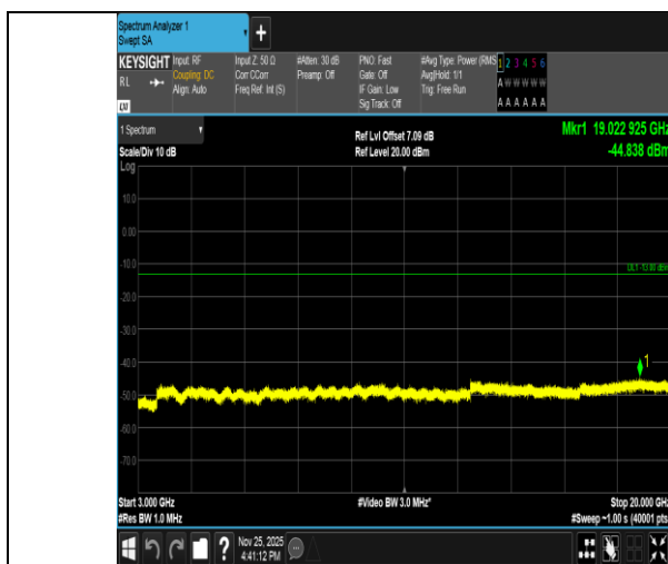
Band2-3MHz-16QAM-19185-1RB#14-3000~20000-PASS
