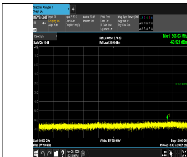
Band2-5MHz-QPSK-18900-25RB#0-30~1000-PASS
