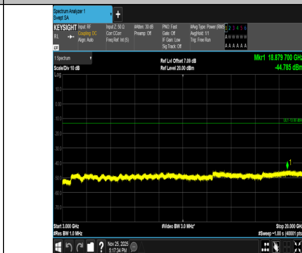
Band2-5MHz-16QAM-18625-25RB#0-3000~20000-PASS
