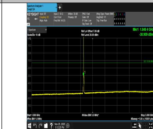
Band2-5MHz-QPSK-18625-1RB#0-1000~3000-PASS
