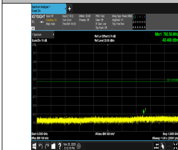
Band2-5MHz-QPSK-18625-1RB#0-30~1000-PASS
