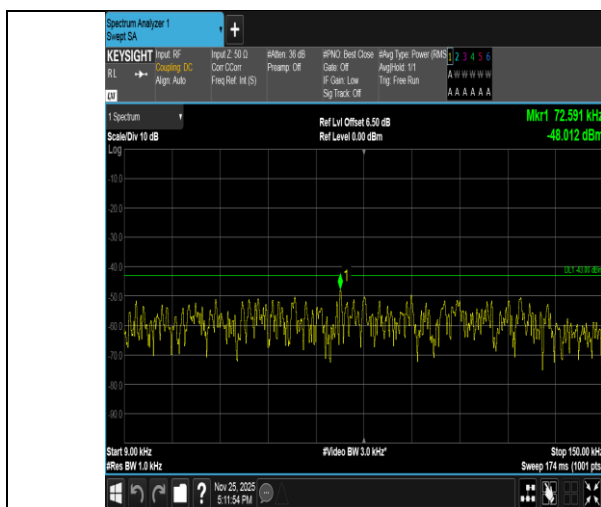
Band2-5MHz-QPSK-18625-1RB#0-0.009~0.15-PASS
