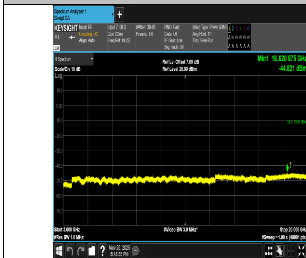
Band2-5MHz-QPSK-18900-1RB#0-3000~20000-PASS
