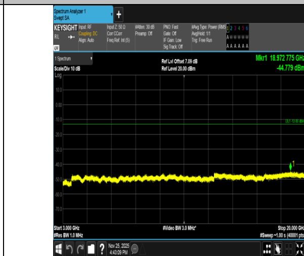
Band2-3MHz-16QAM-19185-15RB#0-3000~20000-PASS
