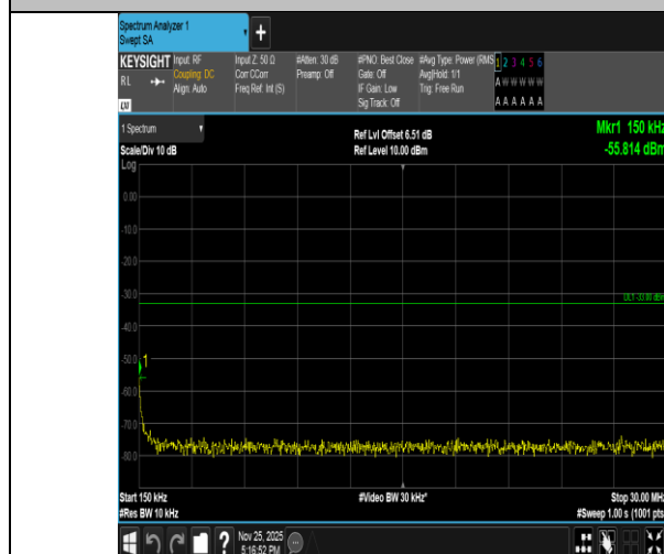
Band2-5MHz-16QAM-18625-25RB#0-0.15~30-PASS
