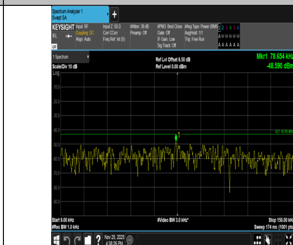
Band2-3MHz-16QAM-19185-1RB#0-0.009~0.15-PASS
