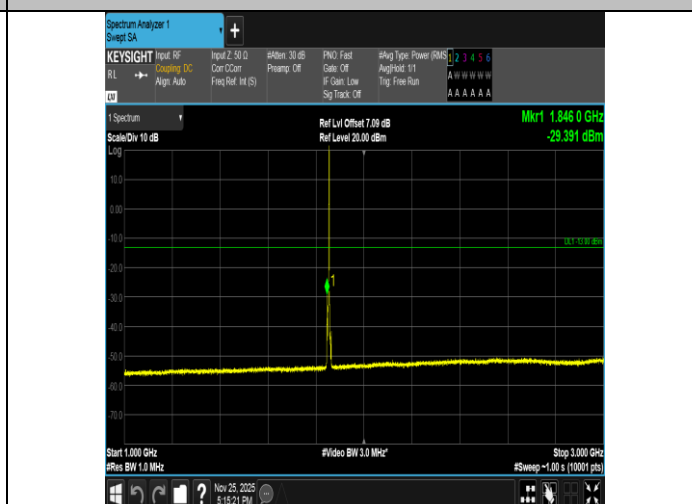
Band2-5MHz-16QAM-18625-1RB#24-1000~3000-PASS
