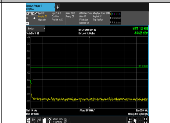
Band2-5MHz-16QAM-18625-1RB#24-0.15~30-PASS
