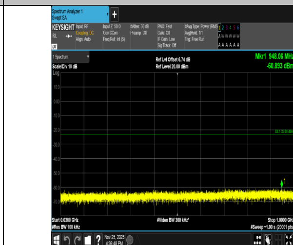
Band2-3MHz-16QAM-18900-15RB#0-30~1000-PASS
