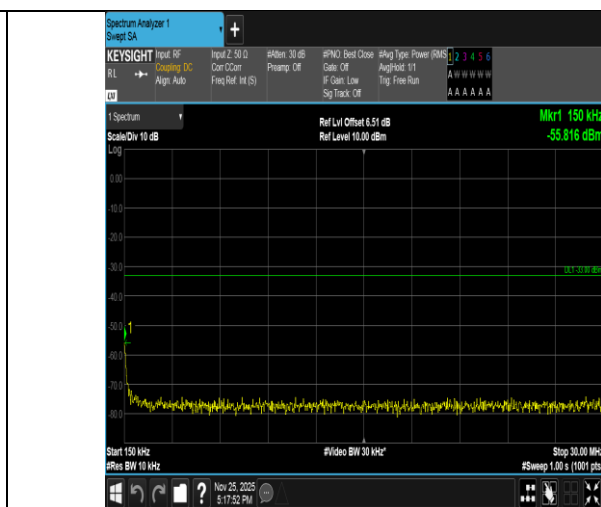
Band2-5MHz-QPSK-18900-1RB#0-0.15~30-PASS
