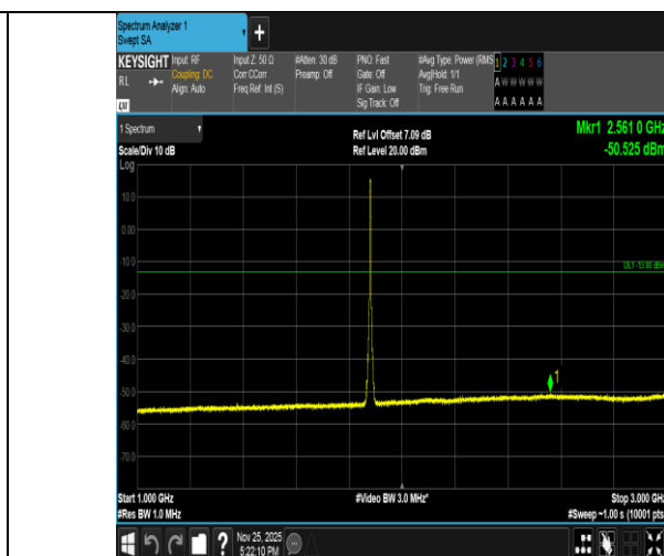
Band2-5MHz-QPSK-18900-25RB#0-1000~3000-PASS
