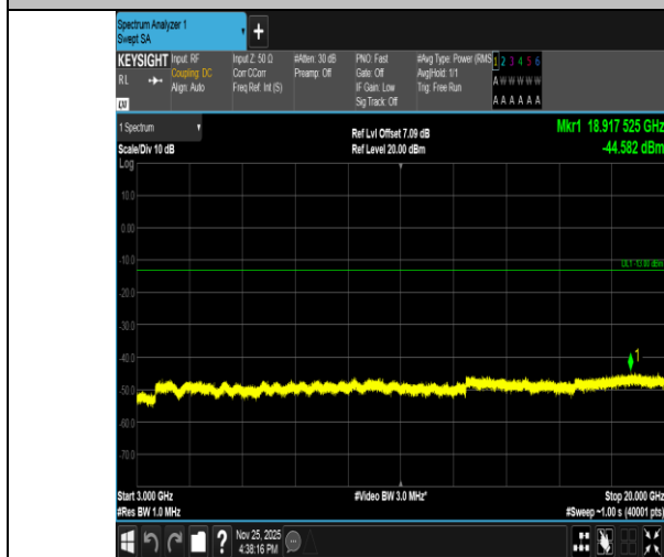
Band2-3MHz-QPSK-19185-1RB#0-3000~20000-PASS
