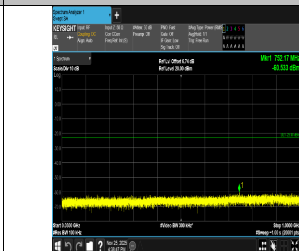
Band2-3MHz-16QAM-19185-1RB#0-30~1000-PASS
