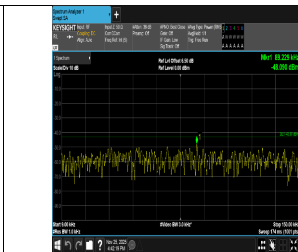
Band2-3MHz-16QAM-19185-15RB#0-0.009~0.15-PASS
