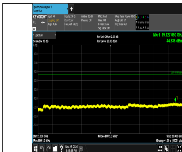
Band2-5MHz-16QAM-18625-1RB#24-3000~20000-PASS
