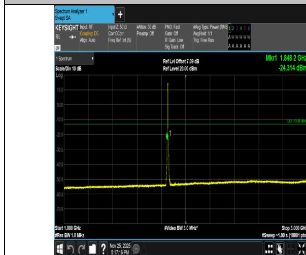
Band2-5MHz-16QAM-18625-25RB#0-1000~3000-PASS
