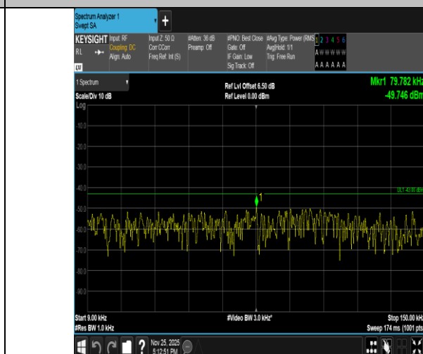
Band2-5MHz-16QAM-18625-1RB#0-0.009~0.15-PASS
