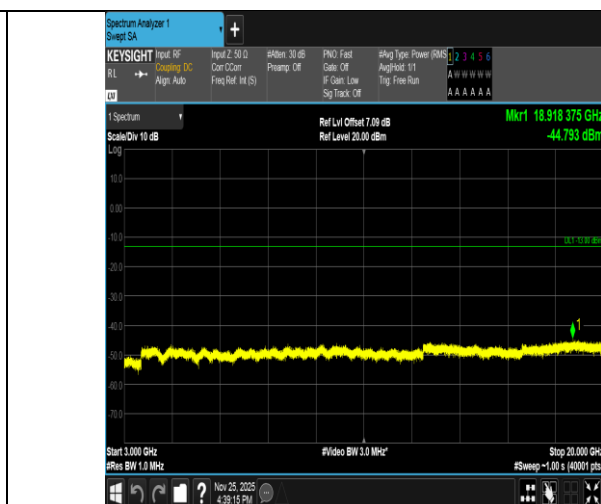
Band2-3MHz-16QAM-19185-1RB#0-3000~20000-PASS
