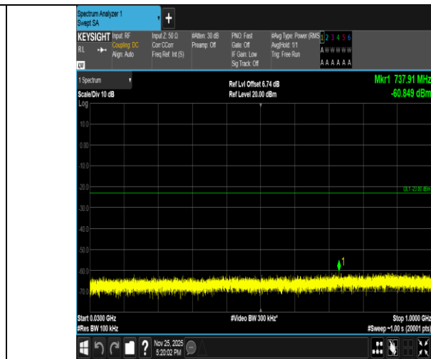
Band2-5MHz-QPSK-18900-1RB#24-30~1000-PASS
