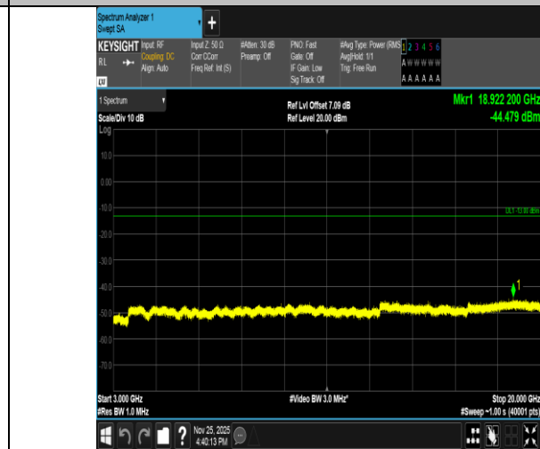
Band2-3MHz-QPSK-19185-1RB#14-3000~20000-PASS
