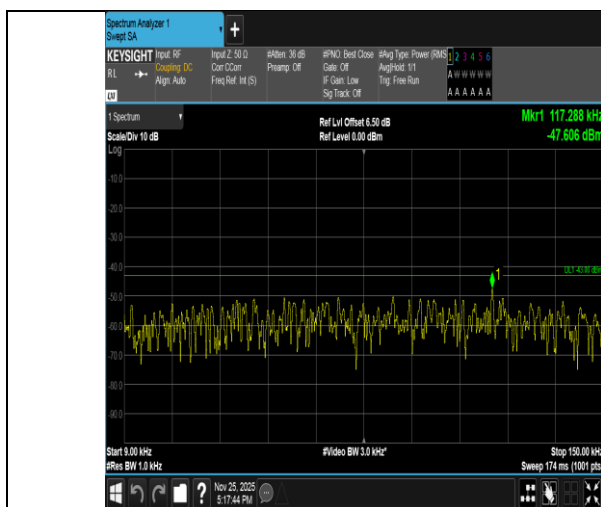
Band2-5MHz-QPSK-18900-1RB#0-0.009~0.15-PASS
