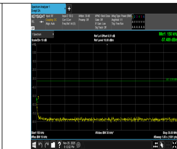
Band2-5MHz-QPSK-18625-1RB#0-0.15~30-PASS
