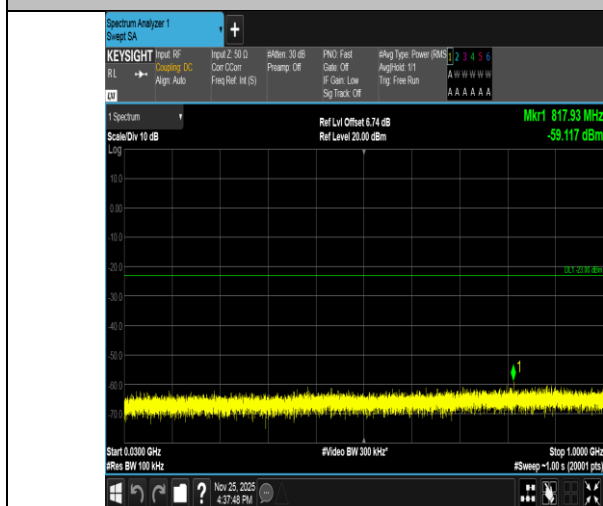
Band2-3MHz-QPSK-19185-1RB#0-30~1000-PASS
