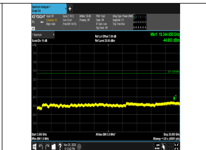
Band2-5MHz-16QAM-18625-1RB#0-3000~20000-PASS
