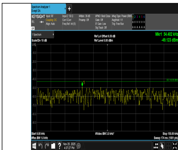
Band2-3MHz-QPSK-19185-1RB#0-0.009~0.15-PASS
