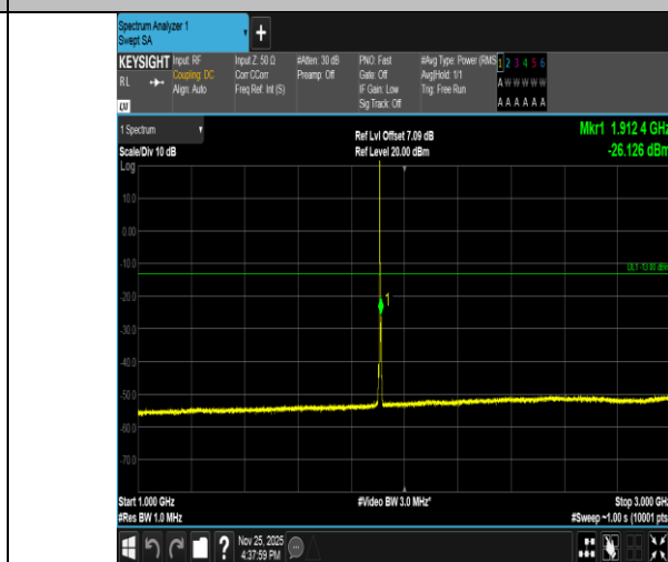
Band2-3MHz-QPSK-19185-1RB#0-1000~3000-PASS
