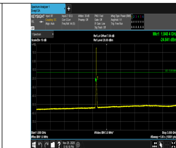
Band2-5MHz-QPSK-18625-25RB#0-1000~3000-PASS
