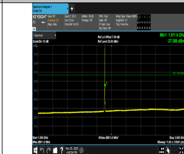
Band2-3MHz-16QAM-19185-1RB#14-1000~3000-PASS
