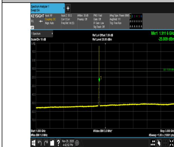
Band2-3MHz-16QAM-19185-15RB#0-1000~3000-PASS
