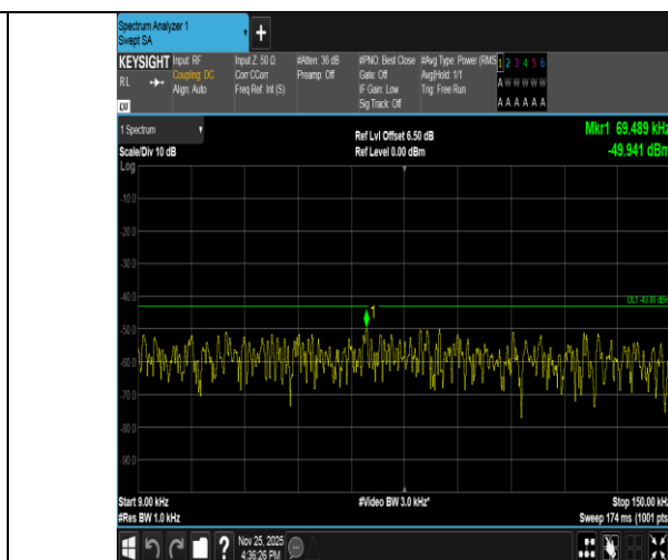
Band2-3MHz-16QAM-18900-15RB#0-0.009~0.15-PASS
