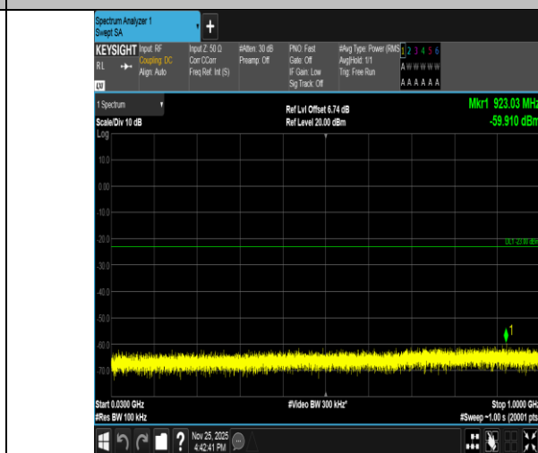
Band2-3MHz-16QAM-19185-15RB#0-30~1000-PASS
