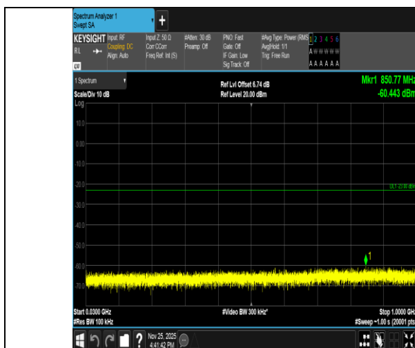
Band2-3MHz-QPSK-19185-15RB#0-30~1000-PASS
