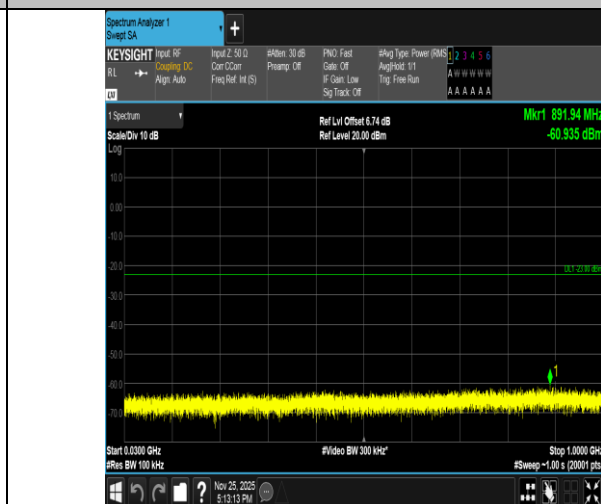
Band2-5MHz-16QAM-18625-1RB#0-30~1000-PASS
