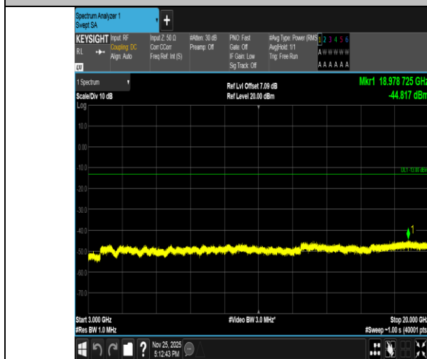
Band2-5MHz-QPSK-18625-1RB#0-3000~20000-PASS
