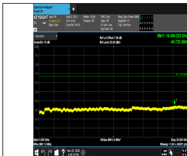
Band2-3MHz-16QAM-18900-1RB#14-3000~20000-PASS
