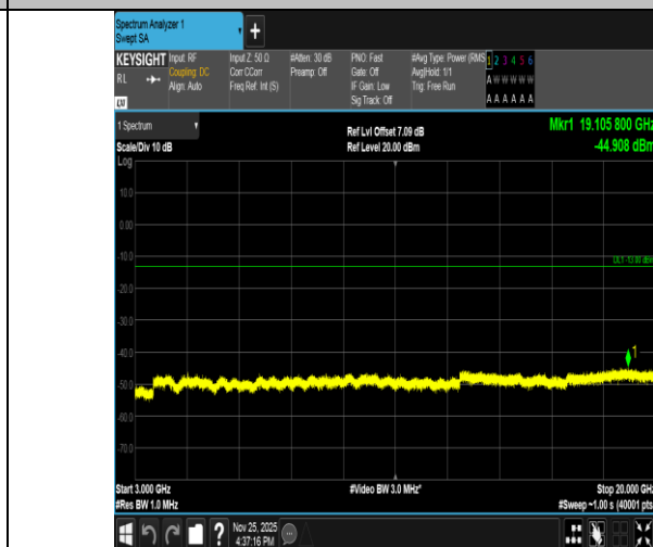
Band2-3MHz-16QAM-18900-15RB#0-3000~20000-PASS
