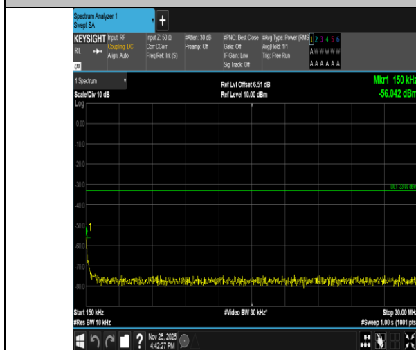
Band2-3MHz-16QAM-19185-15RB#0-0.15~30-PASS
