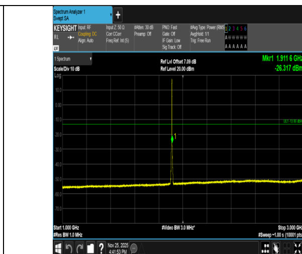
Band2-3MHz-QPSK-19185-15RB#0-1000~3000-PASS
