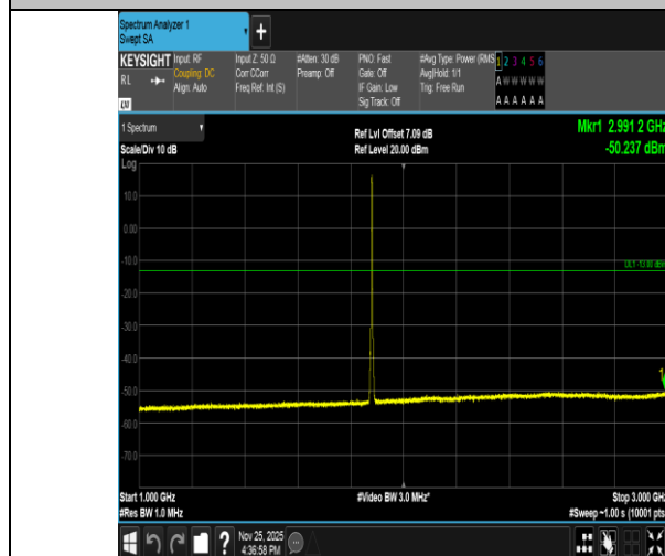
Band2-3MHz-16QAM-18900-15RB#0-1000~3000-PASS
