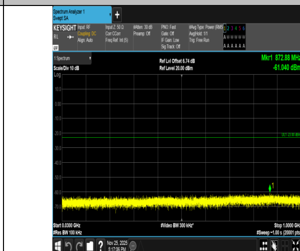
Band2-5MHz-16QAM-18625-25RB#0-30~1000-PASS
