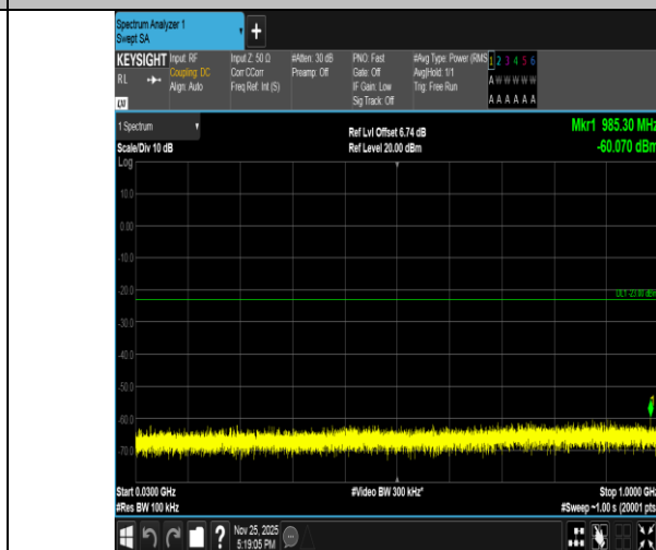
Band2-5MHz-16QAM-18900-1RB#0-30~1000-PASS
