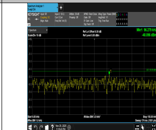
Band2-5MHz-16QAM-18900-1RB#0-0.009~0.15-PASS
