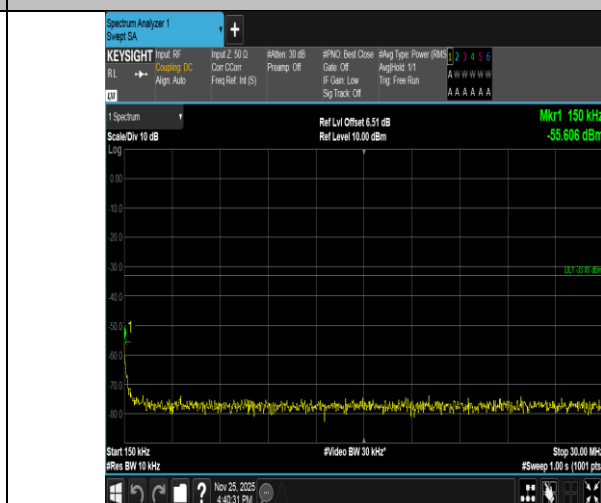
Band2-3MHz-16QAM-19185-1RB#14-0.15~30-PASS
