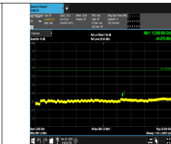
Band2-10MHz-16QAM-18650-1RB#0-3000~20000-PASS
