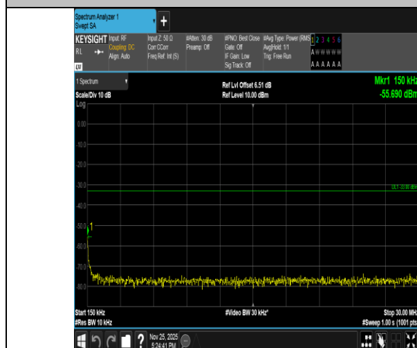
Band2-5MHz-16QAM-19175-1RB#0-0.15~30-PASS
