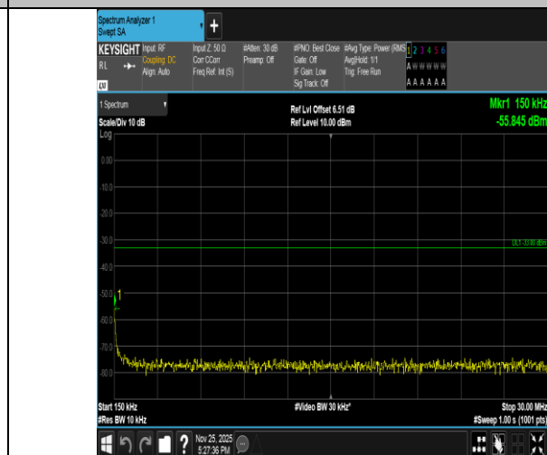
Band2-5MHz-QPSK-19175-25RB#0-0.15~30-PASS
