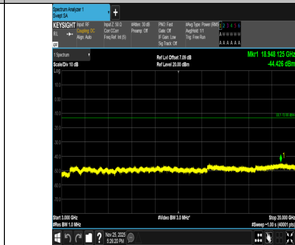
Band2-5MHz-QPSK-19175-1RB#24-3000~20000-PASS
