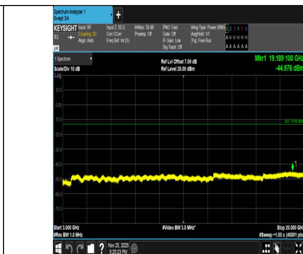
Band2-5MHz-16QAM-19175-1RB#0-3000~20000-PASS
