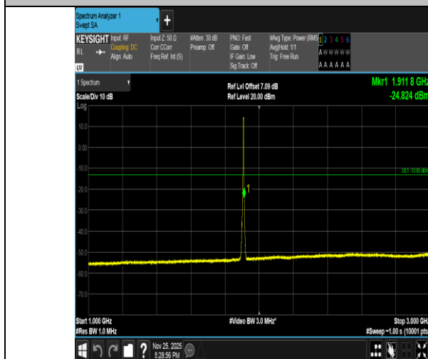
Band2-5MHz-16QAM-19175-25RB#0-1000~3000-PASS
