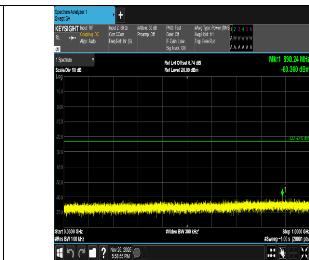
Band2-10MHz-QPSK-18650-1RB#49-30~1000-PASS
