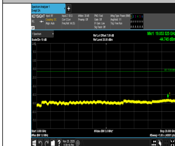
Band2-5MHz-QPSK-19175-25RB#0-3000~20000-PASS
