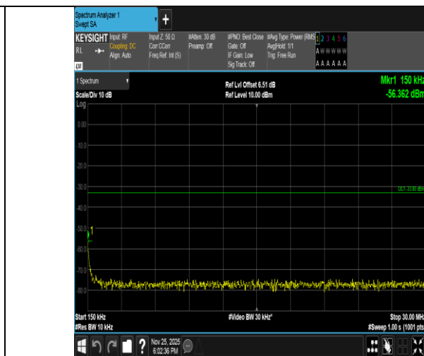
Band2-10MHz-QPSK-18900-1RB#0-0.15~30-PASS
