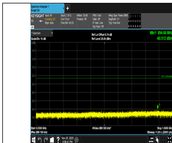
Band2-10MHz-QPSK-18900-50RB#0-30~1000-PASS
