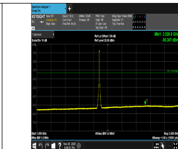
Band2-10MHz-QPSK-18900-50RB#0-1000~3000-PASS
