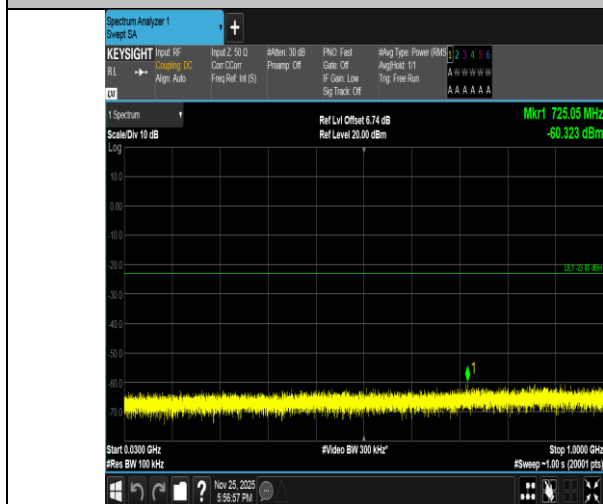
Band2-10MHz-QPSK-18650-1RB#0-30~1000-PASS
