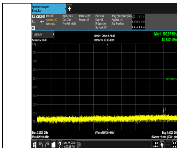
Band2-5MHz-QPSK-19175-25RB#0-30~1000-PASS
