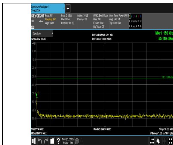
Band2-10MHz-QPSK-18650-1RB#49-0.15~30-PASS
