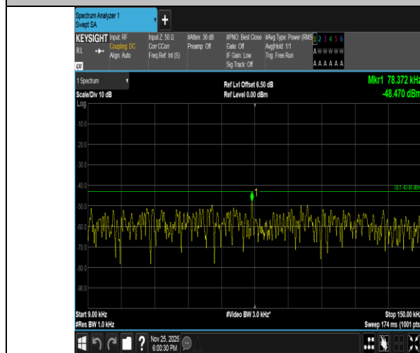
Band2-10MHz-QPSK-18650-50RB#0-0.009~0.15-PASS
