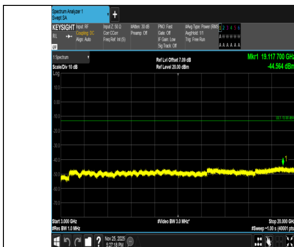
Band2-5MHz-16QAM-19175-1RB#24-3000~20000-PASS
