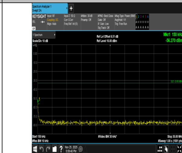
Band2-10MHz-16QAM-18650-1RB#49-0.15~30-PASS
