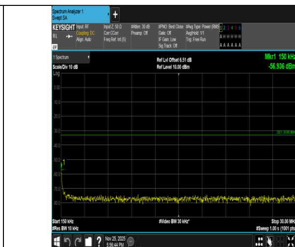
Band2-10MHz-QPSK-18650-1RB#0-0.15~30-PASS
