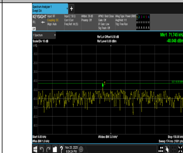
Band2-10MHz-QPSK-18900-1RB#49-0.009~0.15-PASS
