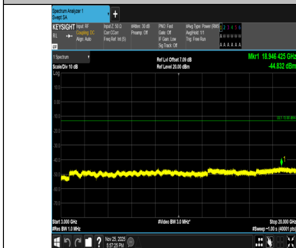
Band2-10MHz-QPSK-18650-1RB#0-3000~20000-PASS
