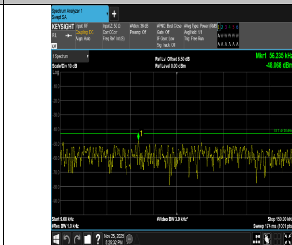
Band2-5MHz-QPSK-19175-1RB#24-0.009~0.15-PASS
