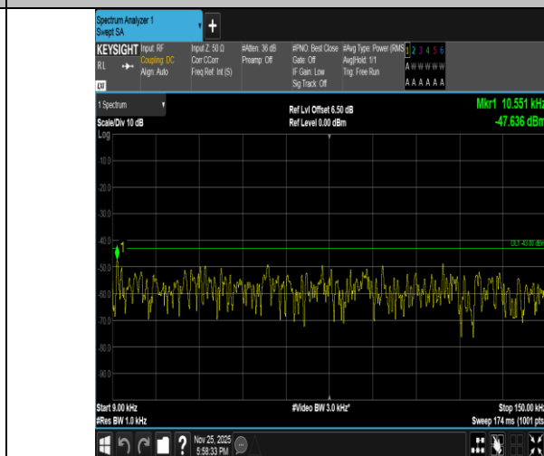
Band2-10MHz-QPSK-18650-1RB#49-0.009~0.15-PASS
