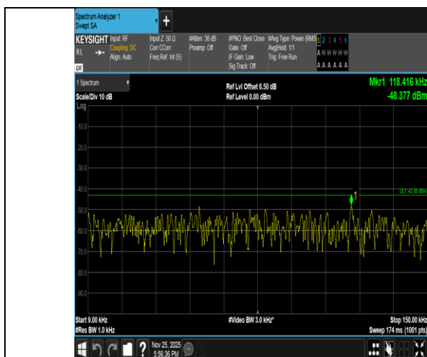
Band2-10MHz-QPSK-18650-1RB#0-0.009~0.15-PASS
