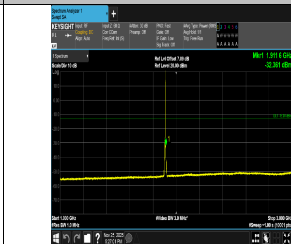
Band2-5MHz-16QAM-19175-1RB#24-1000~3000-PASS
