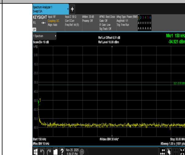
Band2-5MHz-16QAM-19175-1RB#24-0.15~30-PASS
