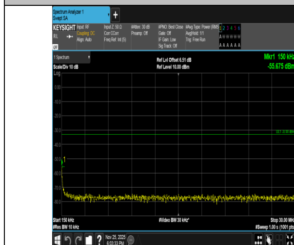
Band2-10MHz-16QAM-18900-1RB#0-0.15~30-PASS
