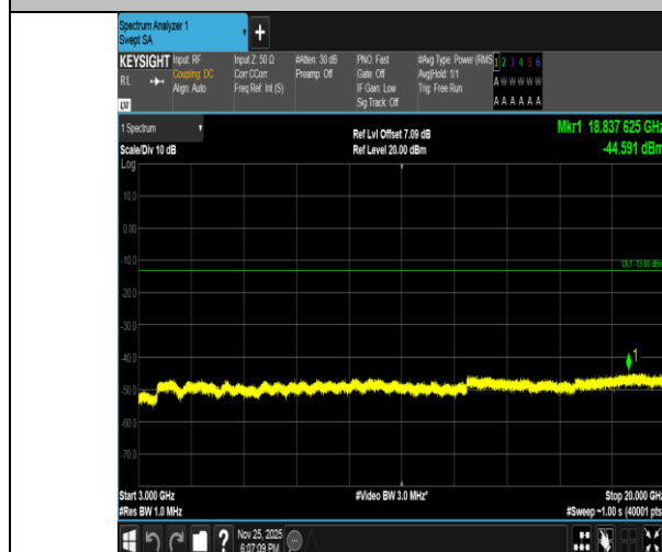
Band2-10MHz-QPSK-18900-50RB#0-3000~20000-PASS
