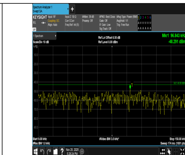
Band2-5MHz-16QAM-19175-25RB#0-0.009~0.15-PASS
