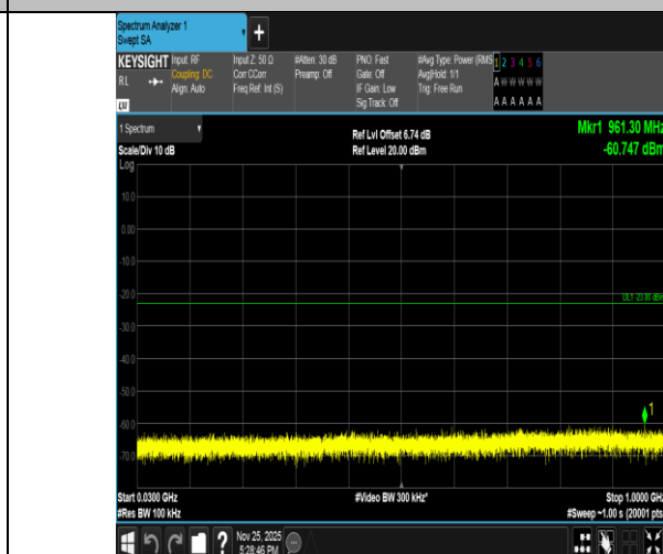
Band2-5MHz-16QAM-19175-25RB#0-30~1000-PASS
