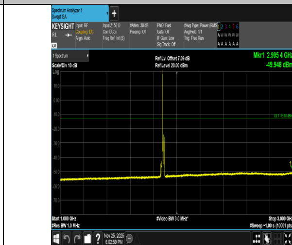
Band2-10MHz-QPSK-18900-1RB#0-1000~3000-PASS
