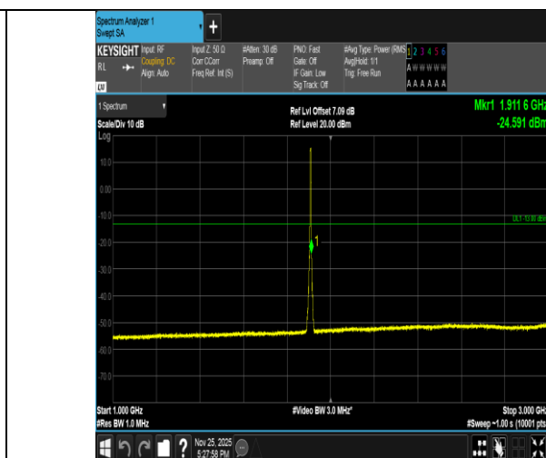
Band2-5MHz-QPSK-19175-25RB#0-1000~3000-PASS
