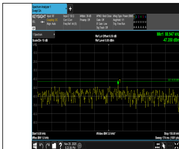
Band2-5MHz-QPSK-19175-1RB#0-0.009~0.15-PASS
