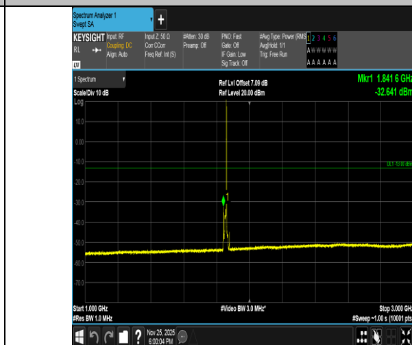
Band2-10MHz-16QAM-18650-1RB#49-1000~3000-PASS
