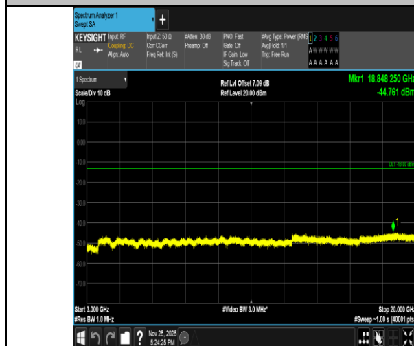
Band2-5MHz-QPSK-19175-1RB#0-3000~20000-PASS
