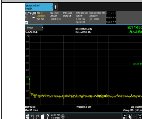
Band2-5MHz-16QAM-19175-25RB#0-0.15~30-PASS
