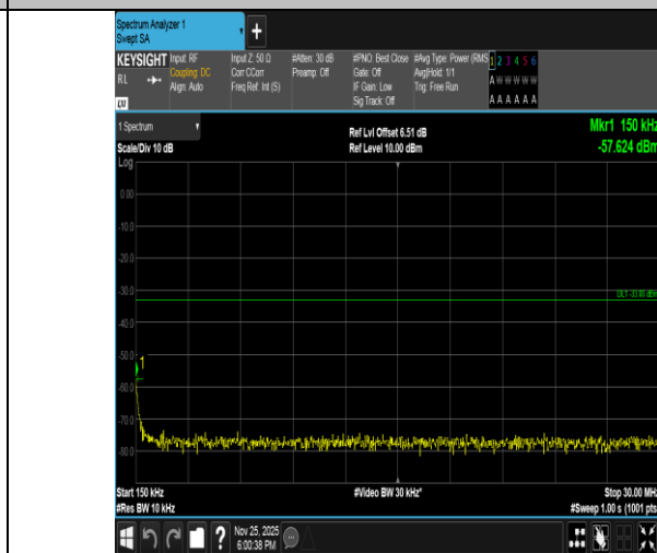
Band2-10MHz-QPSK-18650-50RB#0-0.15~30-PASS
