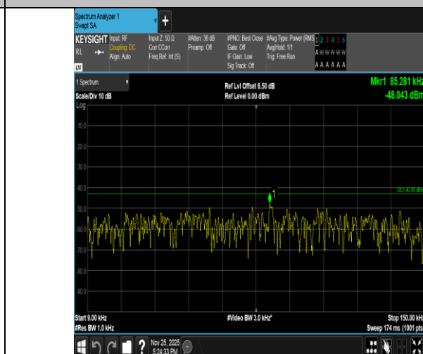
Band2-5MHz-16QAM-19175-1RB#0-0.009~0.15-PASS
