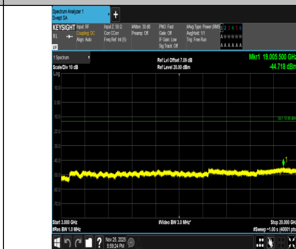
Band2-10MHz-QPSK-18650-1RB#49-3000~20000-PASS
