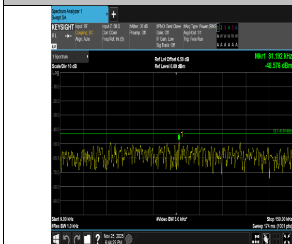
Band2-15MHz-16QAM-18675-1RB#74-0.009~0.15-PASS
