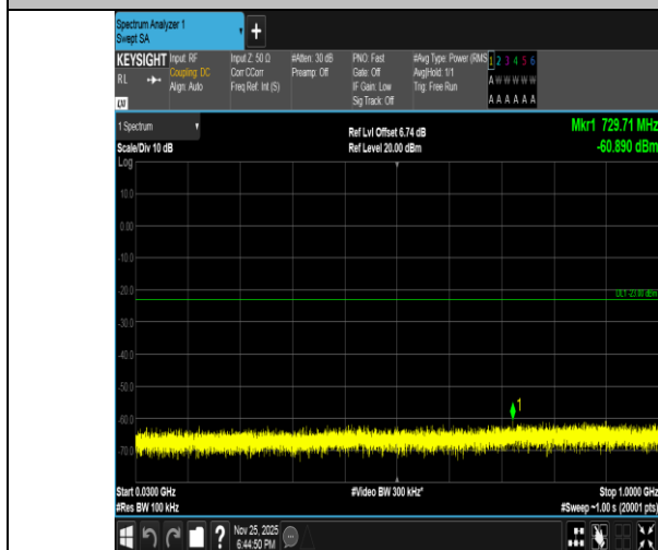
Band2-15MHz-16QAM-18675-1RB#74-30~1000-PASS
