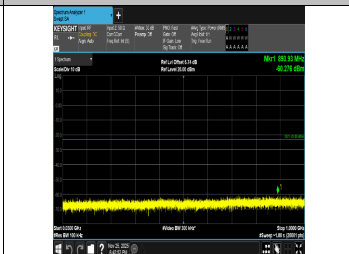
Band2-15MHz-16QAM-18675-1RB#0-30~1000-PASS
