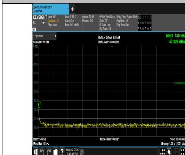
Band2-15MHz-16QAM-18675-75RB#0-0.15~30-PASS
