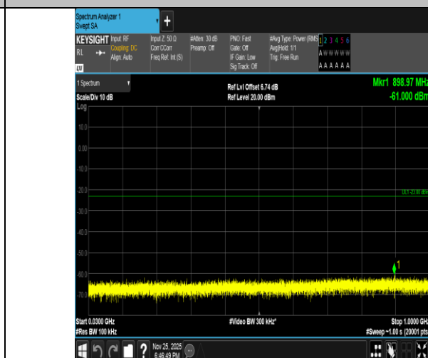
Band2-15MHz-16QAM-18675-75RB#0-30~1000-PASS
