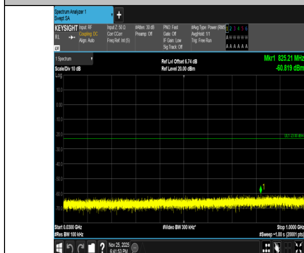
Band2-15MHz-QPSK-18675-1RB#0-30~1000-PASS
