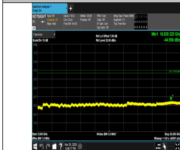
Band2-15MHz-QPSK-18900-1RB#0-3000~20000-PASS
