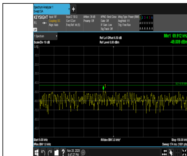
Band2-15MHz-QPSK-18900-1RB#0-0.009~0.15-PASS
