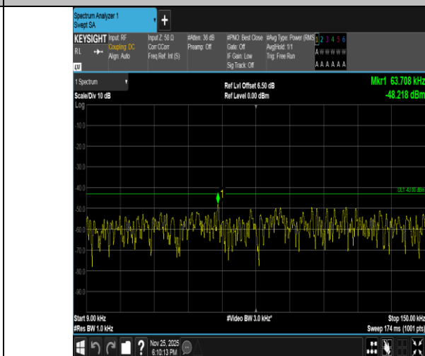
Band2-10MHz-QPSK-19150-1RB#49-0.009~0.15-PASS
