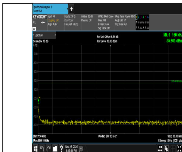
Band2-15MHz-QPSK-18900-1RB#74-0.15~30-PASS
