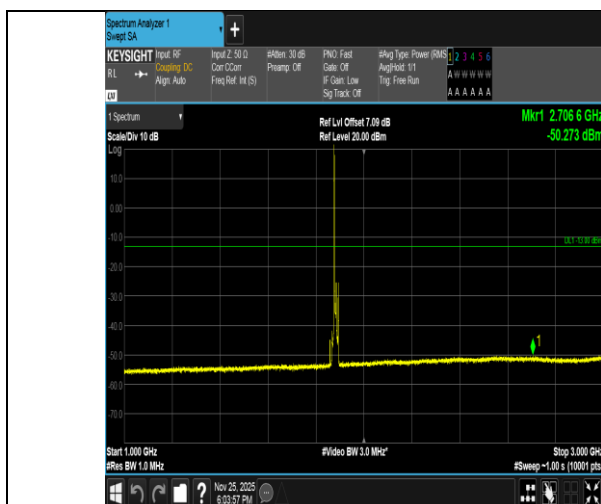
Band2-10MHz-16QAM-18900-1RB#0-1000~3000-PASS
