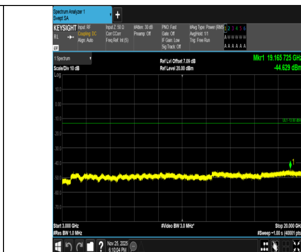
Band2-10MHz-16QAM-19150-1RB#0-3000~20000-PASS
