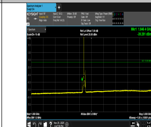
Band2-15MHz-QPSK-18900-1RB#0-1000~3000-PASS
