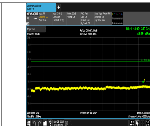
Band2-10MHz-16QAM-18900-1RB#0-3000~20000-PASS
