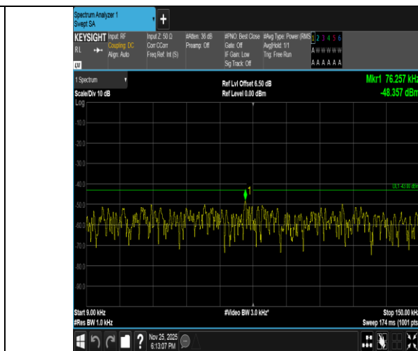
Band2-10MHz-16QAM-19150-50RB#0-0.009~0.15-PASS
