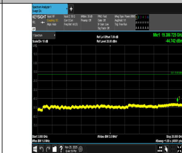
Band2-15MHz-QPSK-18675-1RB#74-3000~20000-PASS
