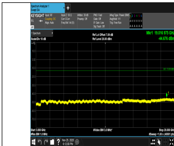
Band2-10MHz-16QAM-19150-1RB#49-3000~20000-PASS
