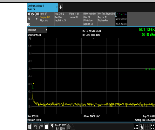
Band2-15MHz-QPSK-18900-75RB#0-0.15~30-PASS
