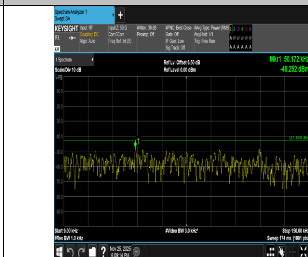
Band2-10MHz-16QAM-19150-1RB#0-0.009~0.15-PASS
