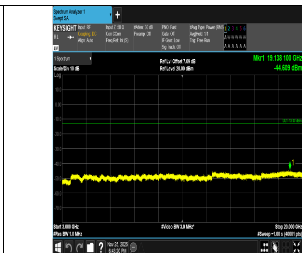
Band2-15MHz-16QAM-18675-1RB#0-3000~20000-PASS
