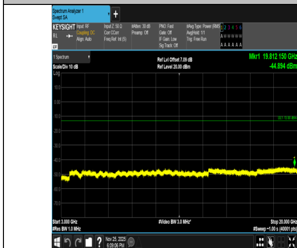
Band2-10MHz-QPSK-19150-1RB#0-3000~20000-PASS
