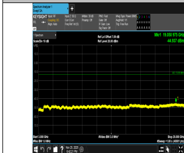
Band2-15MHz-QPSK-18675-1RB#0-3000~20000-PASS
