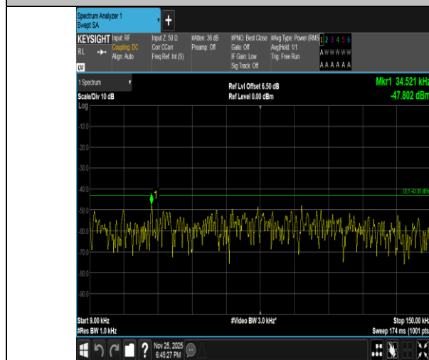
Band2-15MHz-QPSK-18675-75RB#0-0.009~0.15-PASS
