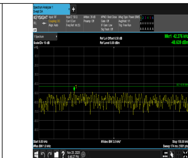
Band2-15MHz-16QAM-18675-75RB#0-0.009~0.15-PASS
