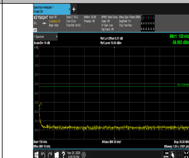
Band2-10MHz-16QAM-18900-1RB#49-0.15~30-PASS
