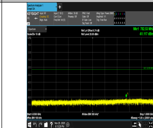
Band2-10MHz-16QAM-19150-50RB#0-30~1000-PASS
