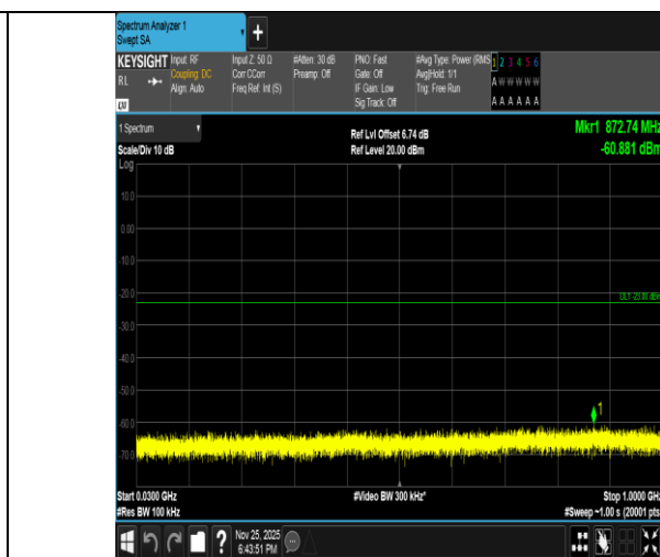
Band2-15MHz-QPSK-18675-1RB#74-30~1000-PASS
