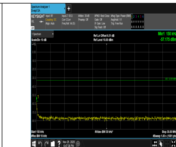
Band2-15MHz-QPSK-18900-1RB#0-0.15~30-PASS
