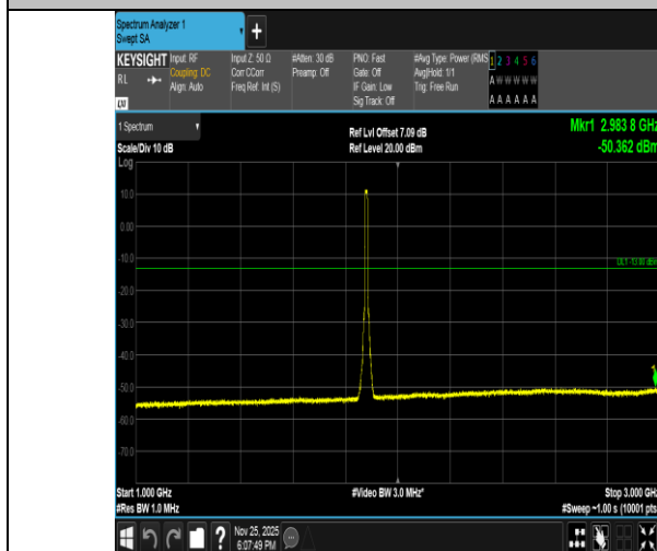
Band2-10MHz-16QAM-18900-50RB#0-1000~3000-PASS
