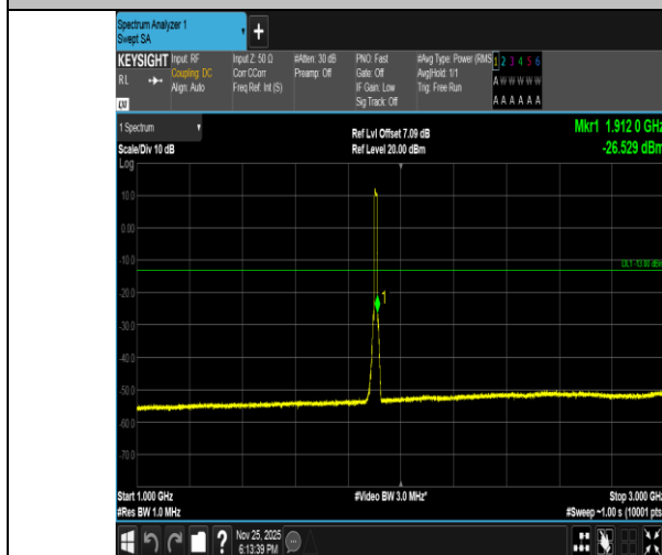
Band2-10MHz-16QAM-19150-50RB#0-1000~3000-PASS
