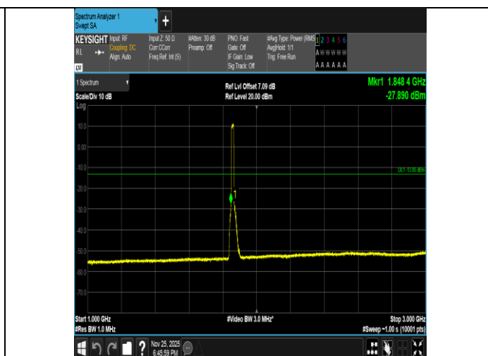
Band2-15MHz-QPSK-18675-75RB#0-1000~3000-PASS
