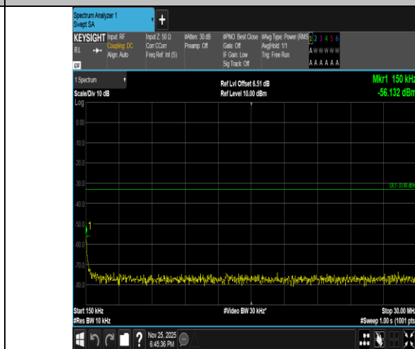
Band2-15MHz-QPSK-18675-75RB#0-0.15~30-PASS
