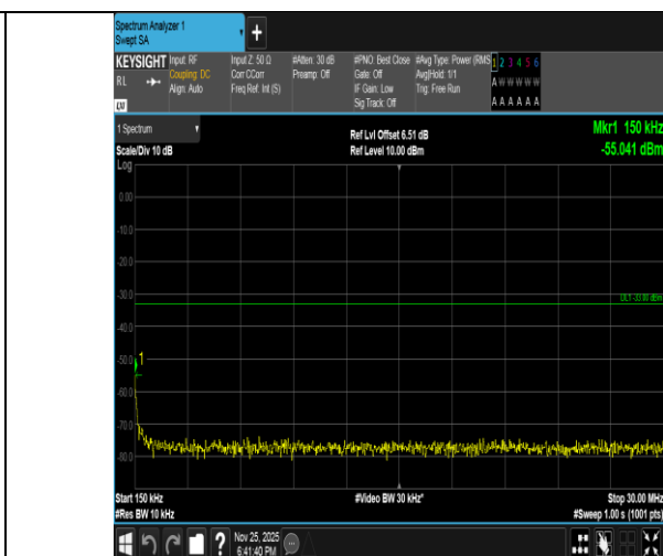
Band2-15MHz-QPSK-18675-1RB#0-0.15~30-PASS
