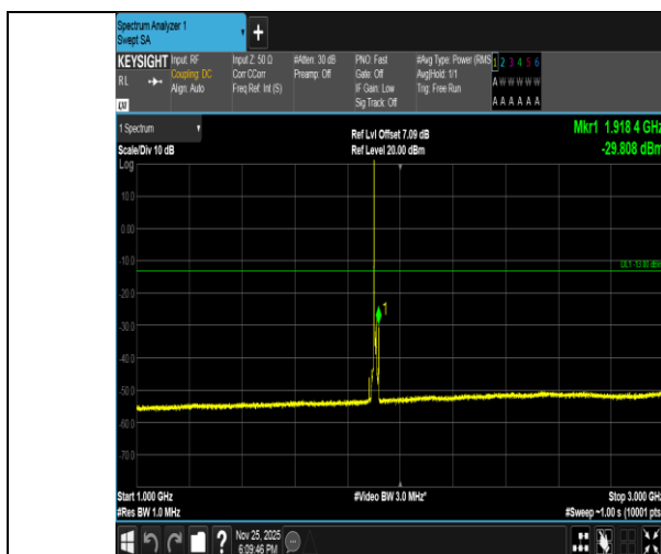
Band2-10MHz-16QAM-19150-1RB#0-1000~3000-PASS
