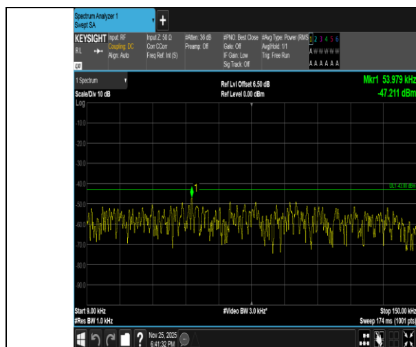
Band2-15MHz-QPSK-18675-1RB#0-0.009~0.15-PASS
