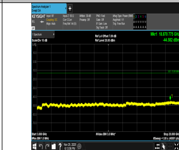
Band2-10MHz-16QAM-19150-50RB#0-3000~20000-PASS
