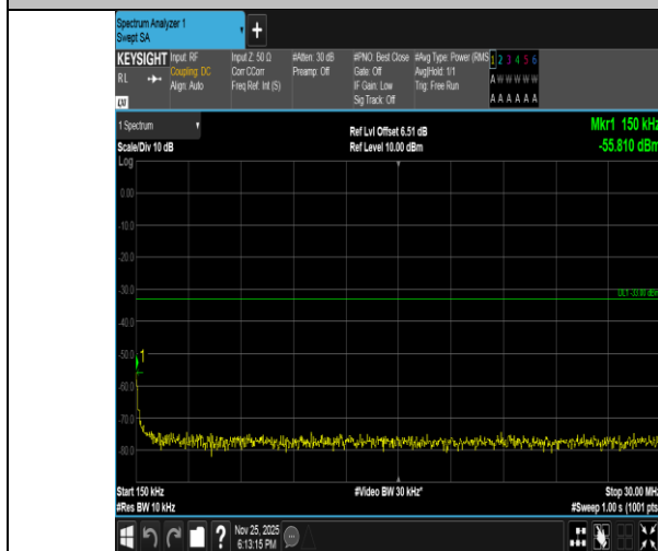
Band2-10MHz-16QAM-19150-50RB#0-0.15~30-PASS
