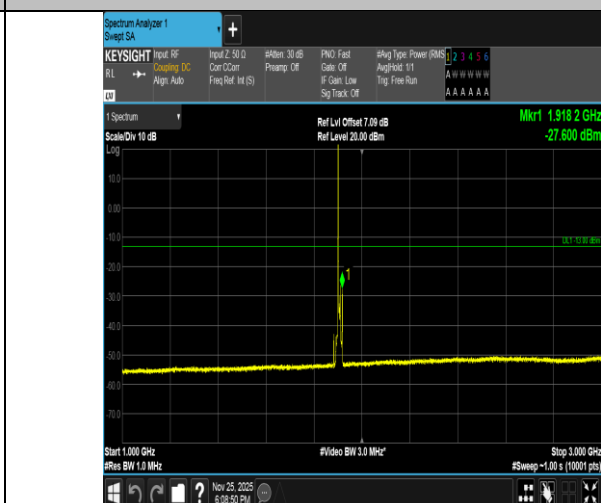
Band2-10MHz-QPSK-19150-1RB#0-1000~3000-PASS
