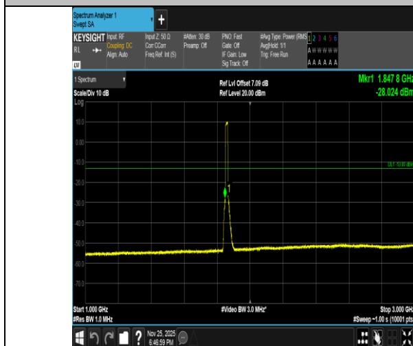
Band2-15MHz-16QAM-18675-75RB#0-1000~3000-PASS
