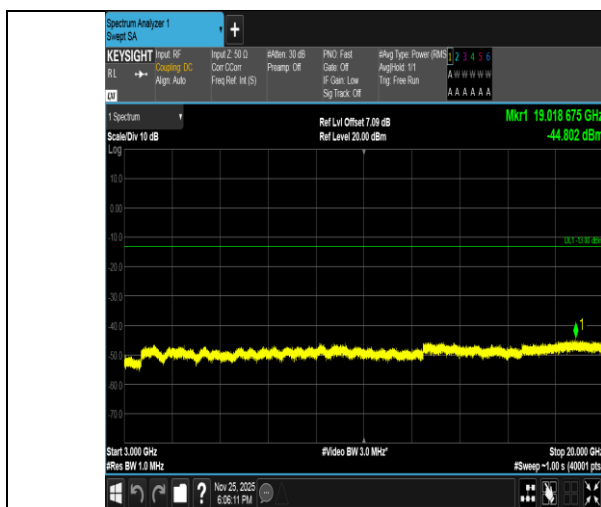
Band2-10MHz-16QAM-18900-1RB#49-3000~20000-PASS
