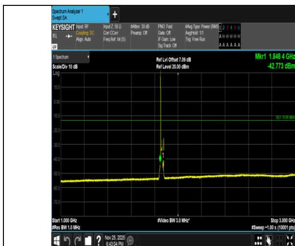
Band2-15MHz-16QAM-18675-1RB#0-1000~3000-PASS
