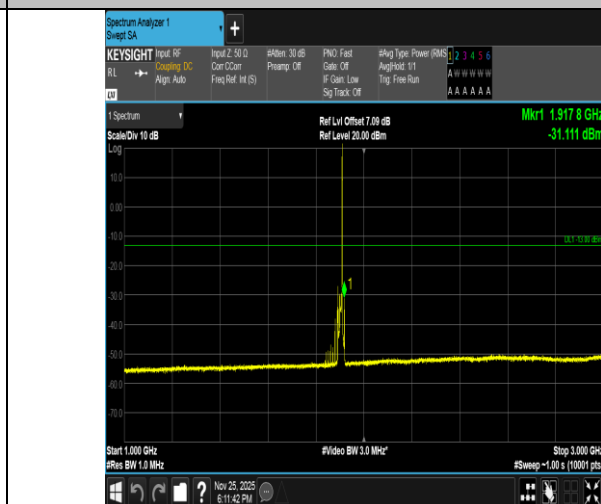
Band2-10MHz-16QAM-19150-1RB#49-1000~3000-PASS
