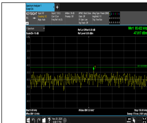
Band2-10MHz-QPSK-19150-1RB#0-0.009~0.15-PASS
