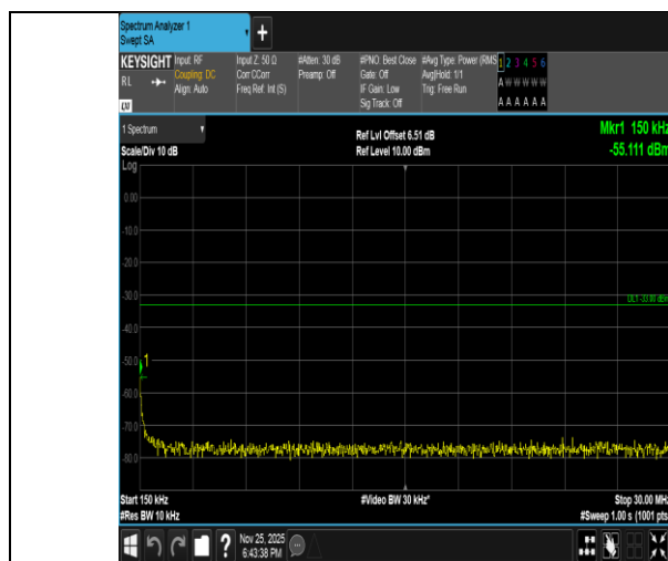
Band2-15MHz-QPSK-18675-1RB#74-0.15~30-PASS
