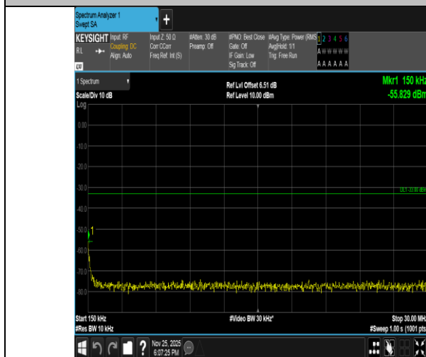
Band2-10MHz-16QAM-18900-50RB#0-0.15~30-PASS
