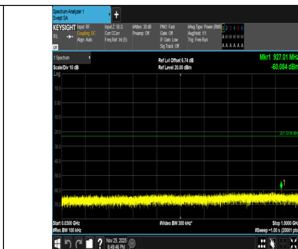
Band2-15MHz-QPSK-18900-1RB#74-30~1000-PASS
