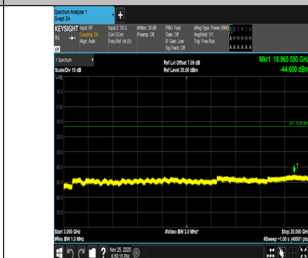
Band2-15MHz-QPSK-18900-1RB#74-3000~20000-PASS
