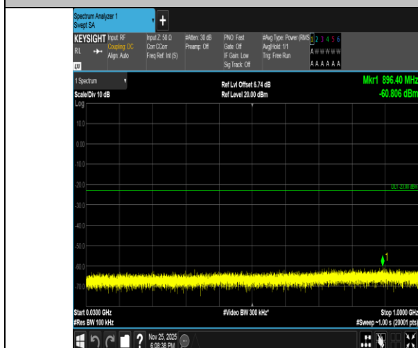
Band2-10MHz-QPSK-19150-1RB#0-30~1000-PASS
