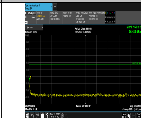
Band2-10MHz-16QAM-19150-1RB#49-0.15~30-PASS
