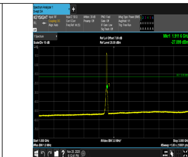
Band2-10MHz-QPSK-19150-50RB#0-1000~3000-PASS
