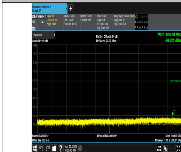
Band2-10MHz-16QAM-18900-1RB#49-30~1000-PASS
