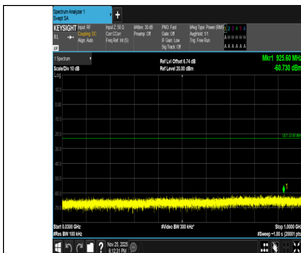
Band2-10MHz-QPSK-19150-50RB#0-30~1000-PASS
