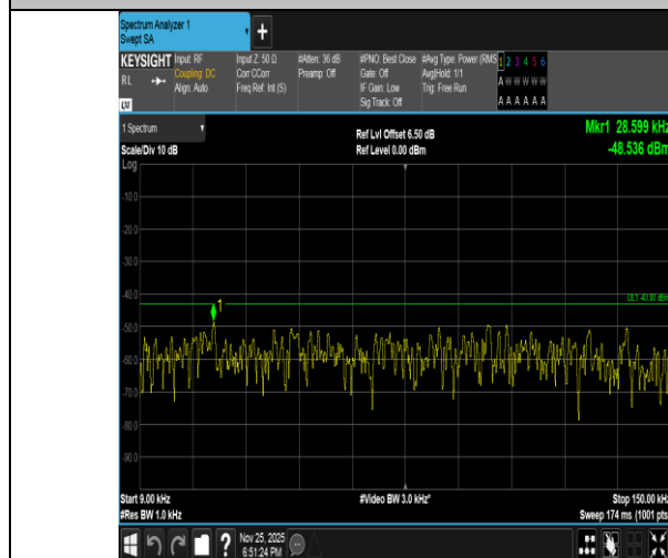
Band2-15MHz-QPSK-18900-75RB#0-0.009~0.15-PASS
