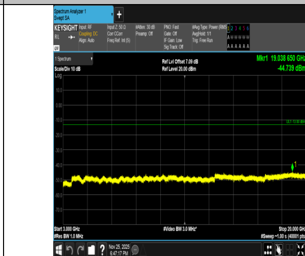
Band2-15MHz-16QAM-18675-75RB#0-3000~20000-PASS
