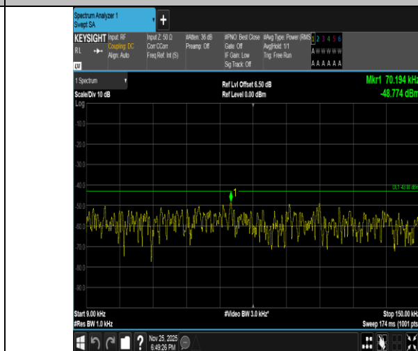
Band2-15MHz-QPSK-18900-1RB#74-0.009~0.15-PASS
