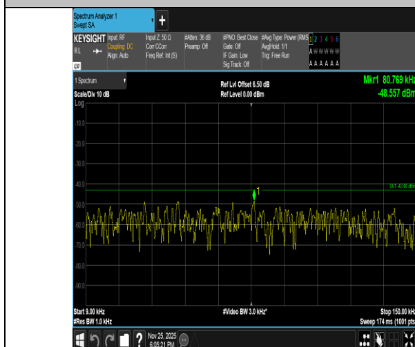
Band2-10MHz-16QAM-18900-1RB#49-0.009~0.15-PASS
