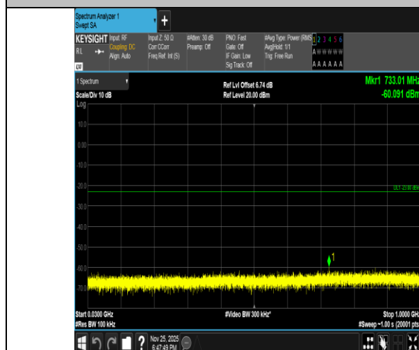
Band2-15MHz-QPSK-18900-1RB#0-30~1000-PASS
