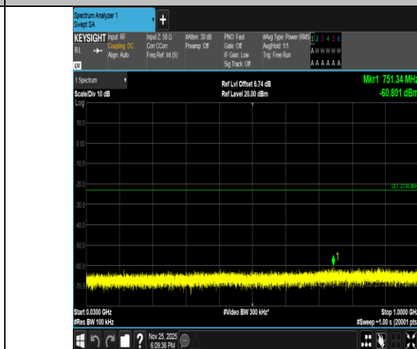
Band2-10MHz-16QAM-19150-1RB#0-30~1000-PASS
