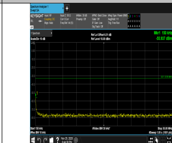
Band2-15MHz-16QAM-18675-1RB#74-0.15~30-PASS
