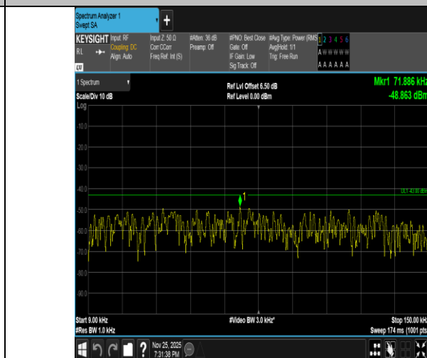
Band2-20MHz-QPSK-18700-1RB#99-0.009~0.15-PASS
