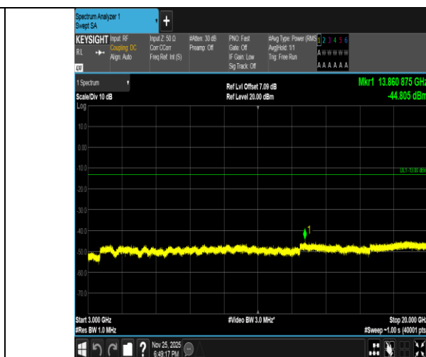
Band2-15MHz-16QAM-18900-1RB#0-3000~20000-PASS
