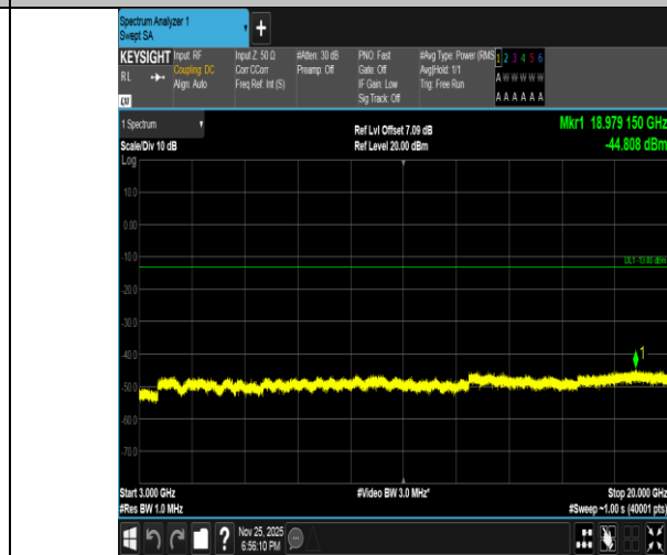
Band2-15MHz-QPSK-19125-1RB#74-3000~20000-PASS
