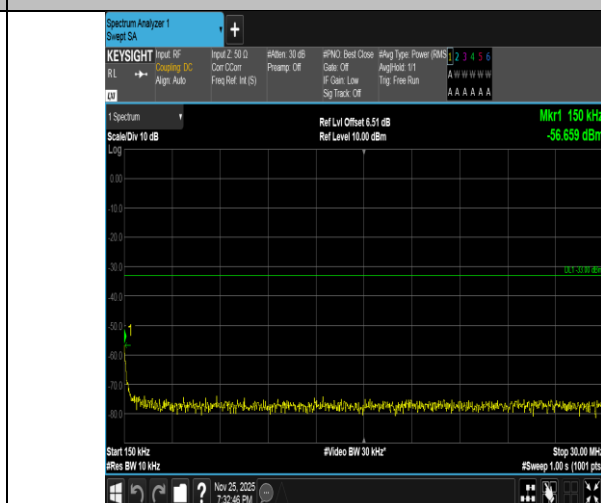
Band2-20MHz-16QAM-18700-1RB#99-0.15~30-PASS
