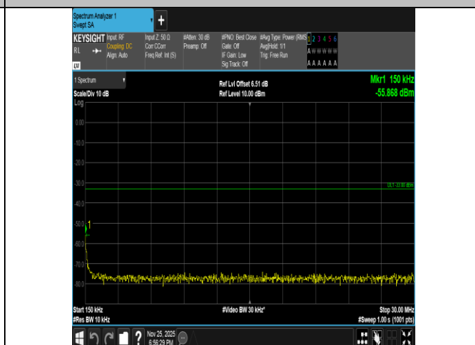
Band2-15MHz-16QAM-19125-1RB#74-0.15~30-PASS
