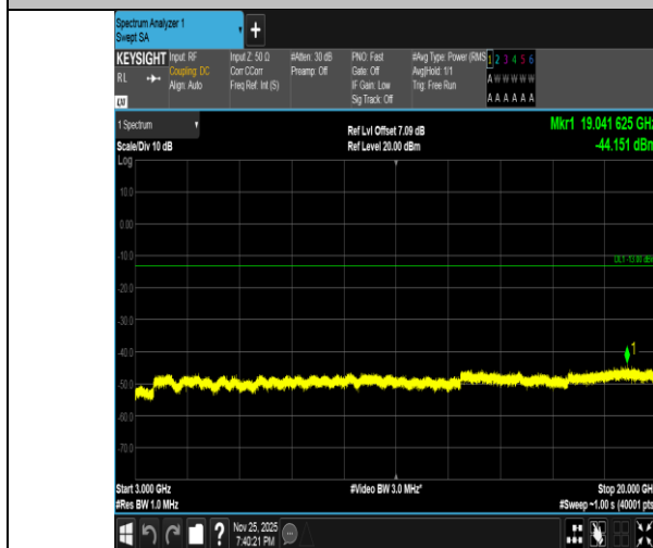
Band2-20MHz-QPSK-18900-100RB#0-3000~20000-PASS
