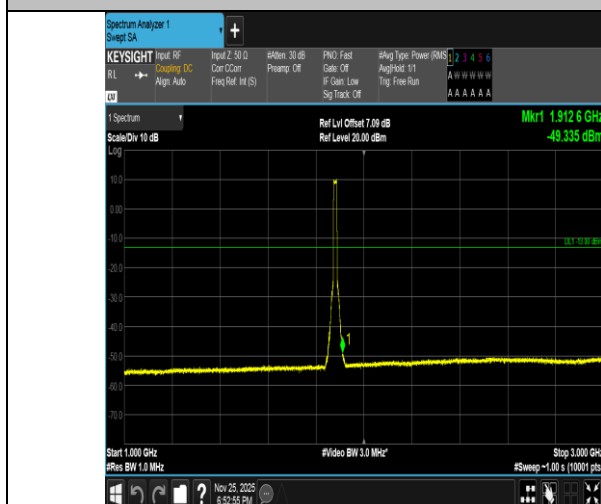
Band2-15MHz-16QAM-18900-75RB#0-1000~3000-PASS
