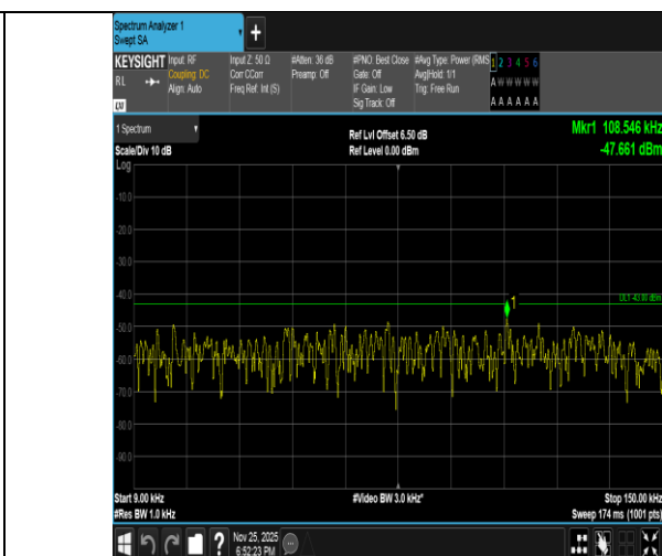
Band2-15MHz-16QAM-18900-75RB#0-0.009~0.15-PASS
