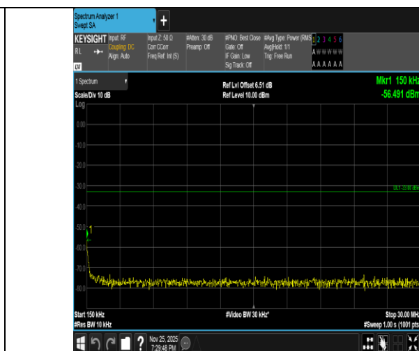
Band2-20MHz-QPSK-18700-1RB#0-0.15~30-PASS
