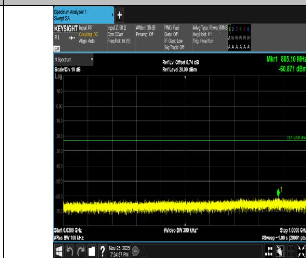
Band2-20MHz-16QAM-18700-100RB#0-30~1000-PASS
