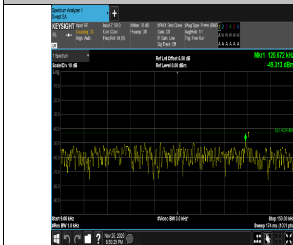
Band2-15MHz-16QAM-18900-1RB#74-0.009~0.15-PASS
