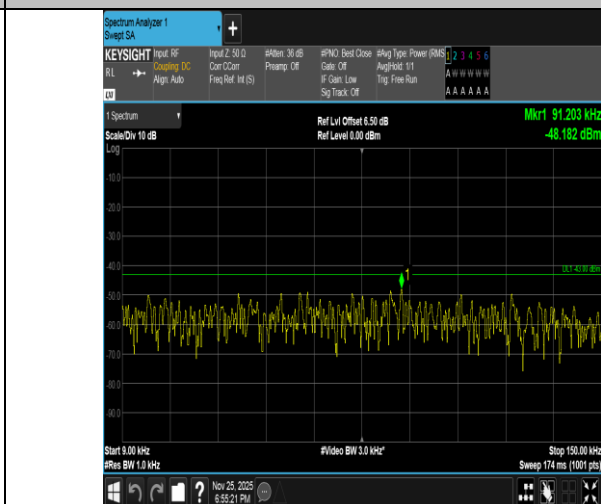
Band2-15MHz-QPSK-19125-1RB#74-0.009~0.15-PASS
