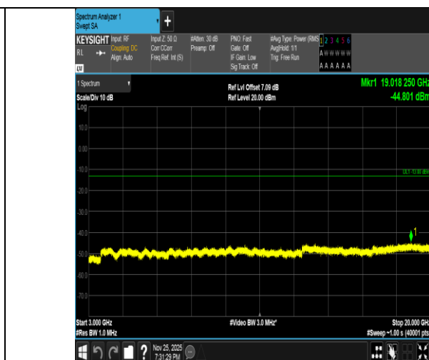
Band2-20MHz-16QAM-18700-1RB#0-3000~20000-PASS
