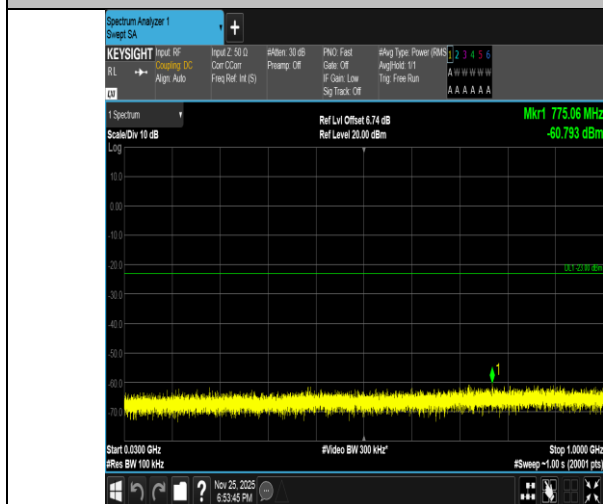
Band2-15MHz-QPSK-19125-1RB#0-30~1000-PASS
