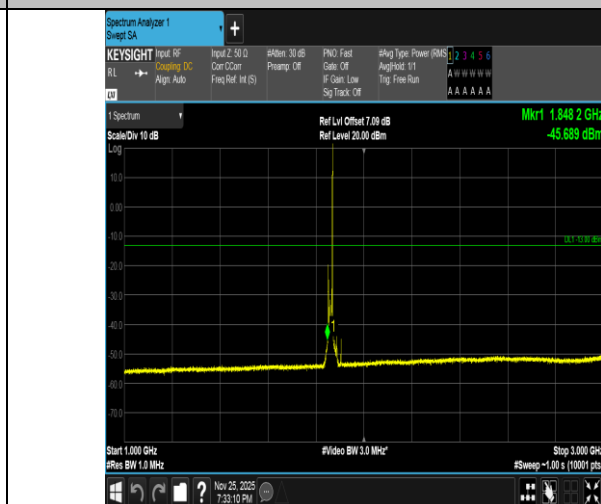
Band2-20MHz-16QAM-18700-1RB#99-1000~3000-PASS
