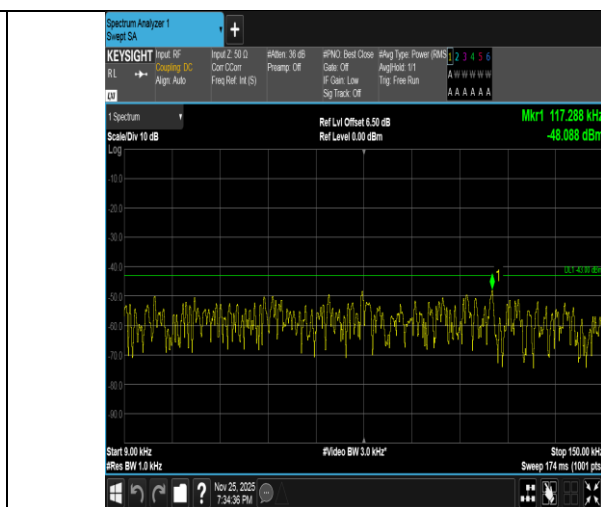
Band2-20MHz-16QAM-18700-100RB#0-0.009~0.15-PASS
