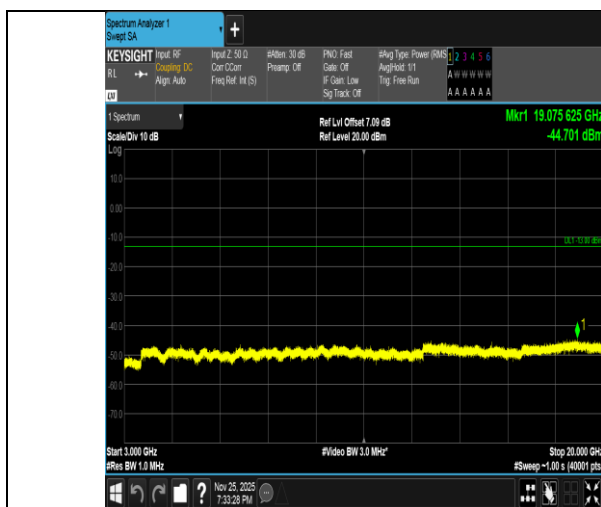
Band2-20MHz-16QAM-18700-1RB#99-3000~20000-PASS
