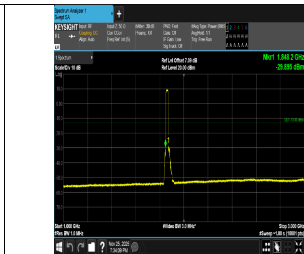
Band2-20MHz-QPSK-18700-100RB#0-1000~3000-PASS
