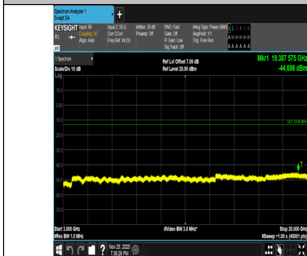
Band2-20MHz-QPSK-18900-1RB#0-3000~20000-PASS
