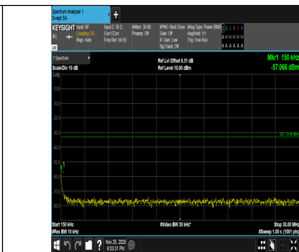
Band2-15MHz-QPSK-19125-1RB#0-0.15~30-PASS
