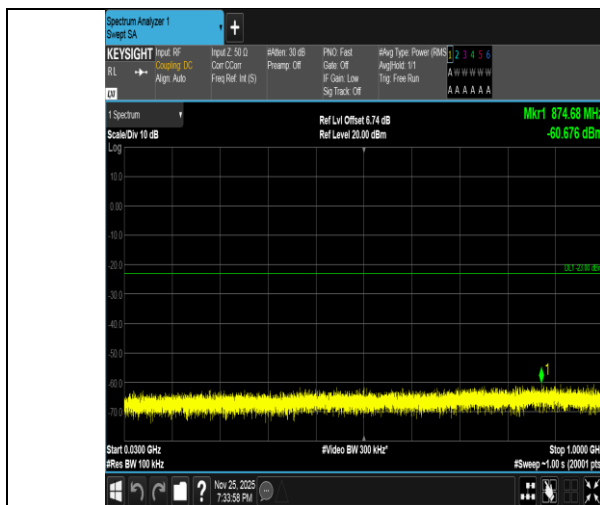
Band2-20MHz-QPSK-18700-100RB#0-30~1000-PASS
