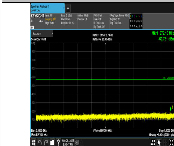
Band2-15MHz-16QAM-18900-1RB#74-30~1000-PASS
