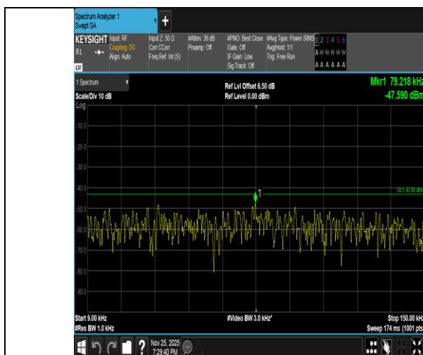
Band2-20MHz-QPSK-18700-1RB#0-0.009~0.15-PASS
