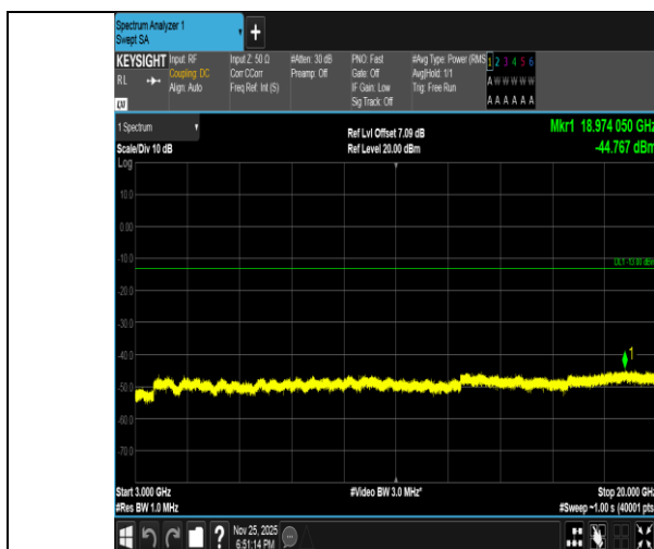
Band2-15MHz-16QAM-18900-1RB#74-3000~20000-PASS
