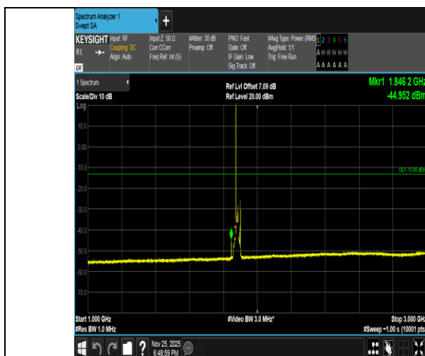
Band2-15MHz-16QAM-18900-1RB#0-1000~3000-PASS
