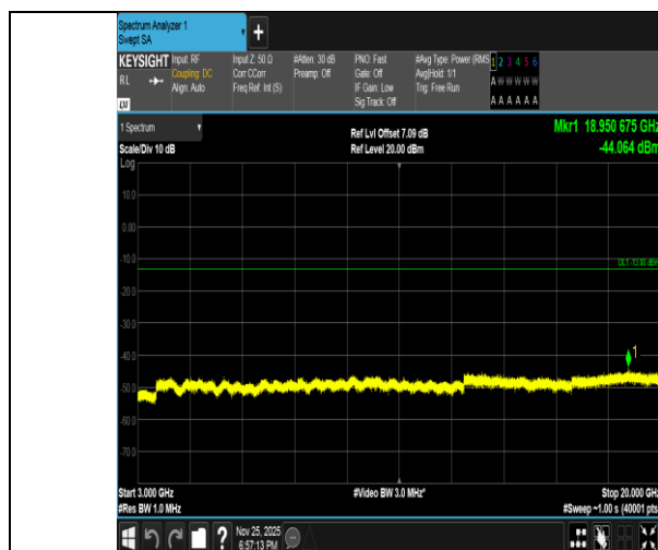
Band2-15MHz-16QAM-19125-1RB#74-3000~20000-PASS
