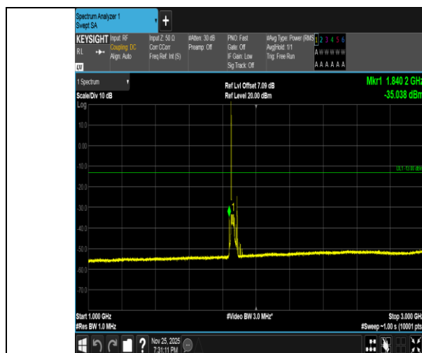
Band2-20MHz-16QAM-18700-1RB#0-1000~3000-PASS
