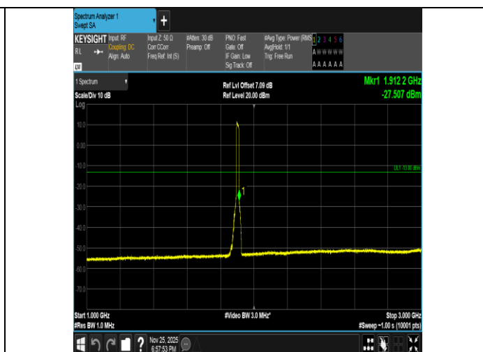
Band2-15MHz-QPSK-19125-75RB#0-1000~3000-PASS
