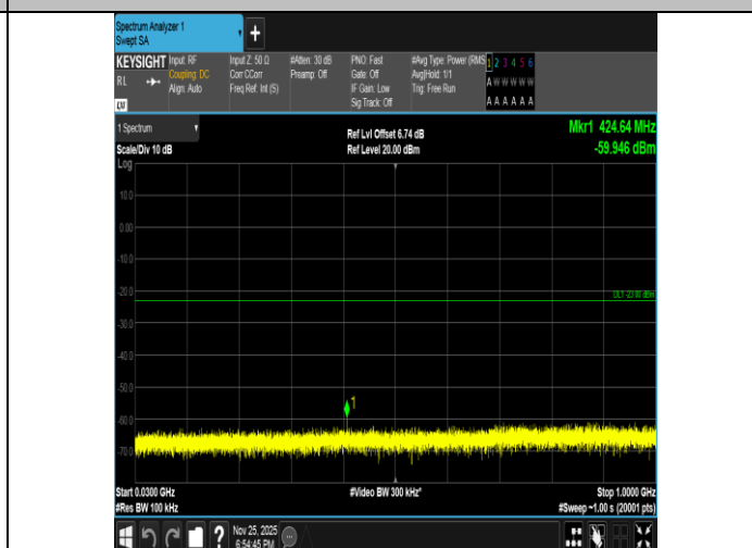
Band2-15MHz-16QAM-19125-1RB#0-30~1000-PASS
