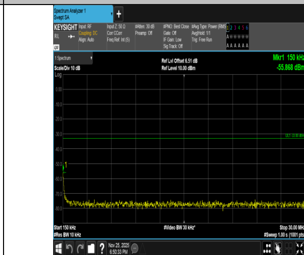
Band2-15MHz-16QAM-18900-1RB#74-0.15~30-PASS
