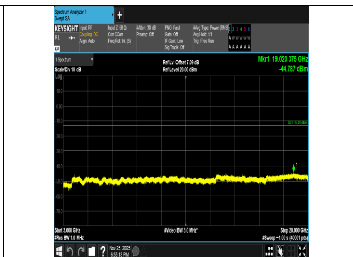
Band2-15MHz-16QAM-19125-1RB#0-3000~20000-PASS
