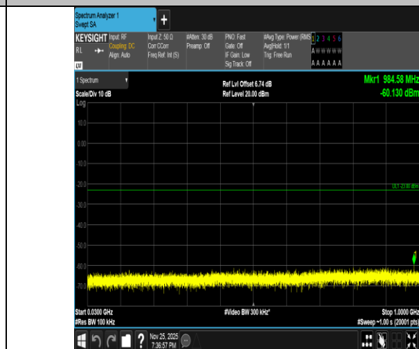
Band2-20MHz-16QAM-18900-1RB#0-30~1000-PASS
