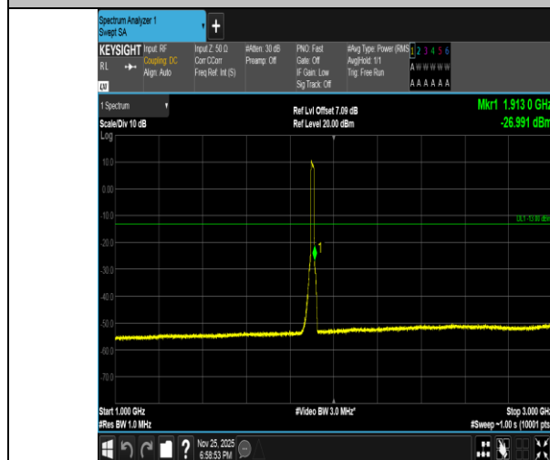
Band2-15MHz-16QAM-19125-75RB#0-1000~3000-PASS
