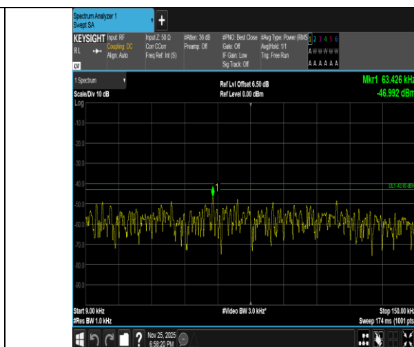
Band2-15MHz-16QAM-19125-75RB#0-0.009~0.15-PASS
