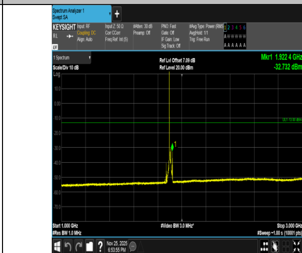
Band2-15MHz-QPSK-19125-1RB#0-1000~3000-PASS
