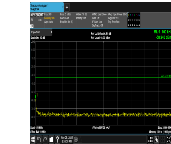
Band2-15MHz-QPSK-19125-1RB#74-0.15~30-PASS
