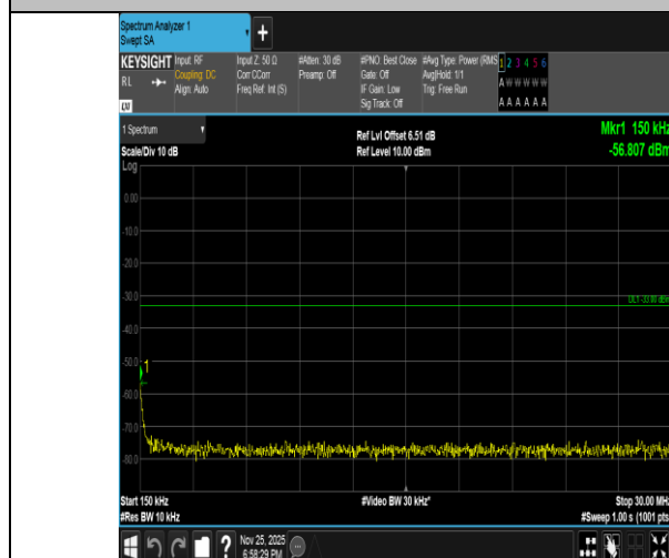
Band2-15MHz-16QAM-19125-75RB#0-0.15~30-PASS
