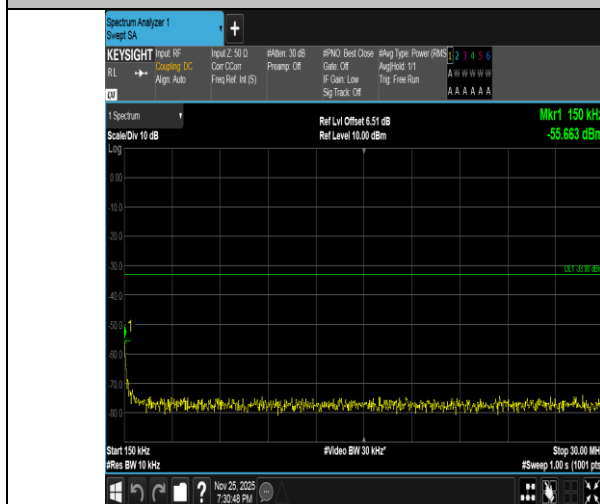
Band2-20MHz-16QAM-18700-1RB#0-0.15~30-PASS
