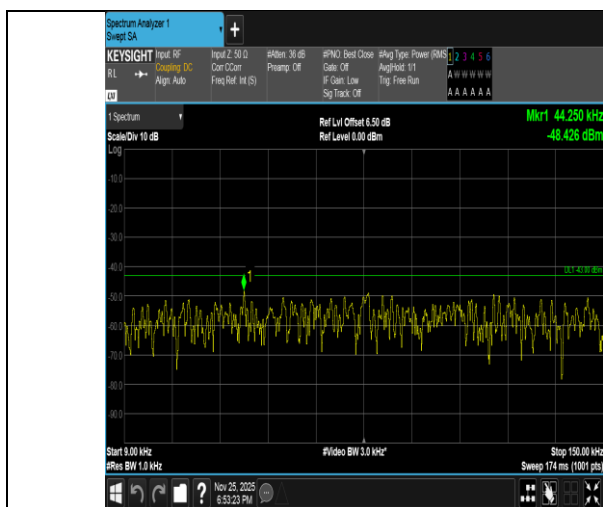
Band2-15MHz-QPSK-19125-1RB#0-0.009~0.15-PASS
