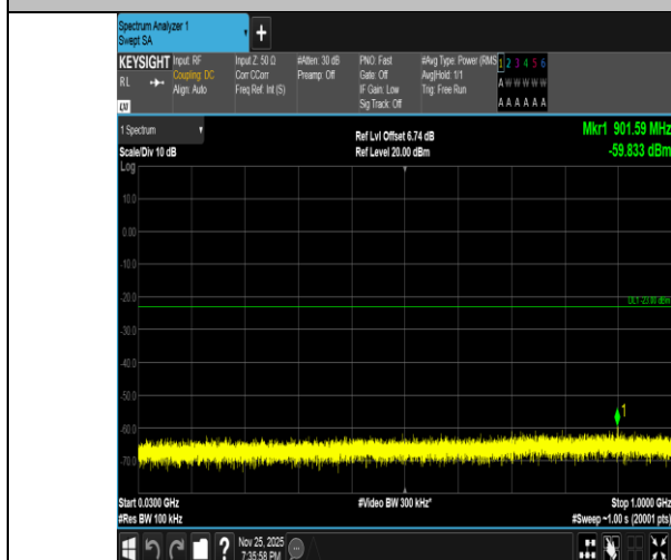
Band2-20MHz-QPSK-18900-1RB#0-30~1000-PASS
