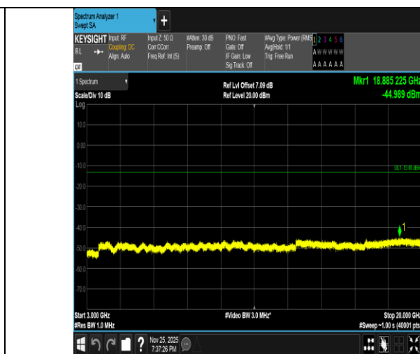
Band2-20MHz-16QAM-18900-1RB#0-3000~20000-PASS
