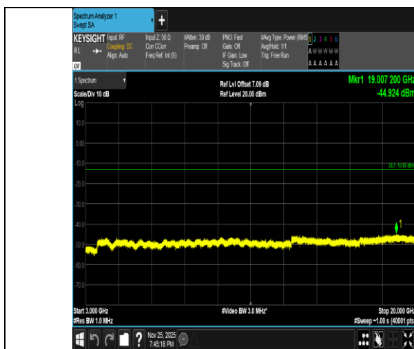
Band2-20MHz-16QAM-19100-1RB#99-3000~20000-PASS
