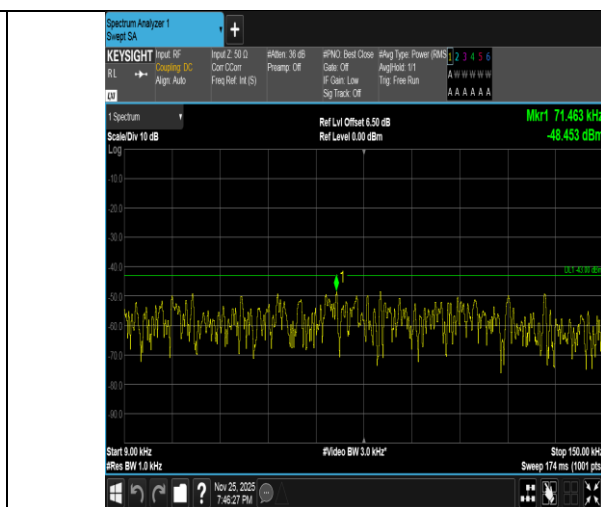
Band2-20MHz-16QAM-19100-100RB#0-0.009~0.15-PASS
