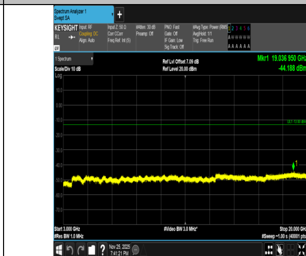
Band2-20MHz-16QAM-18900-100RB#0-3000~20000-PASS
