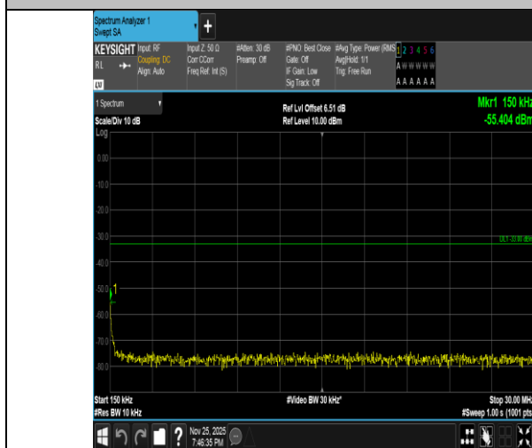
Band2-20MHz-16QAM-19100-100RB#0-0.15~30-PASS
