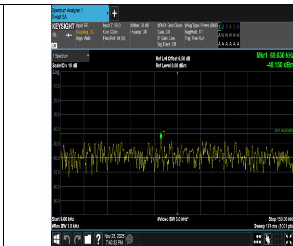
Band2-20MHz-16QAM-18900-100RB#0-0.009~0.15-PASS
