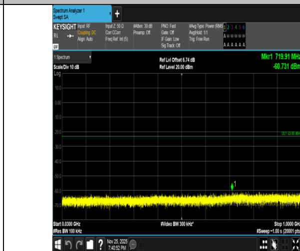
Band2-20MHz-16QAM-18900-100RB#0-30~1000-PASS
