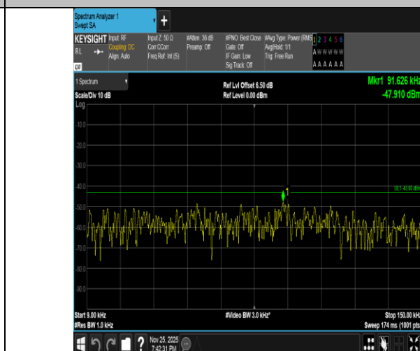
Band2-20MHz-16QAM-19100-1RB#0-0.009~0.15-PASS
