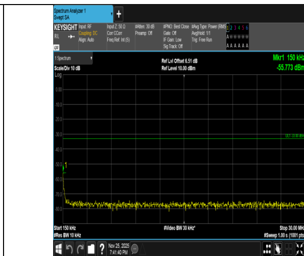
Band2-20MHz-QPSK-19100-1RB#0-0.15~30-PASS
