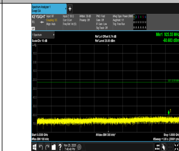
Band2-20MHz-16QAM-19100-100RB#0-30~1000-PASS
