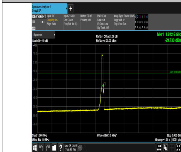
Band2-20MHz-16QAM-19100-100RB#0-1000~3000-PASS
