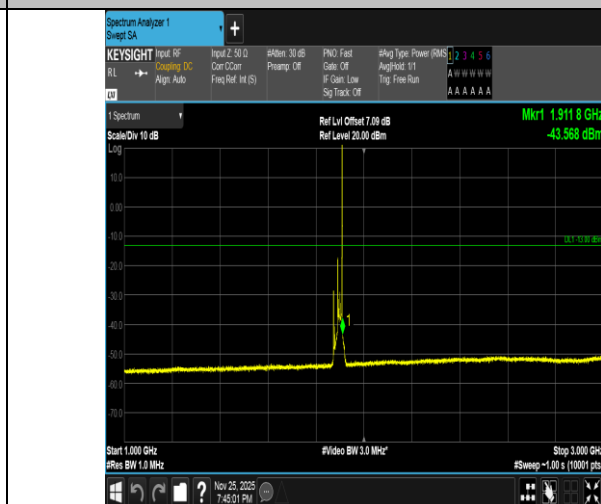
Band2-20MHz-16QAM-19100-1RB#99-1000~3000-PASS
