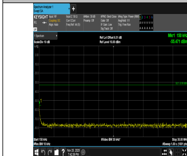
Band2-20MHz-16QAM-19100-1RB#0-0.15~30-PASS
