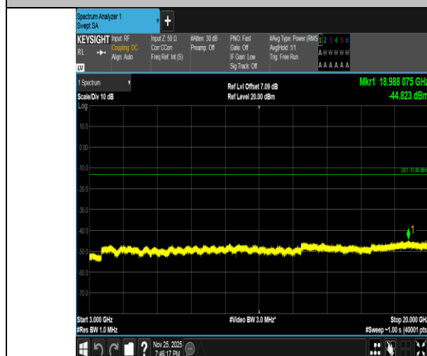
Band2-20MHz-QPSK-19100-100RB#0-3000~20000-PASS
