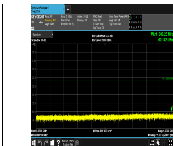
Band2-20MHz-QPSK-19100-100RB#0-30~1000-PASS
