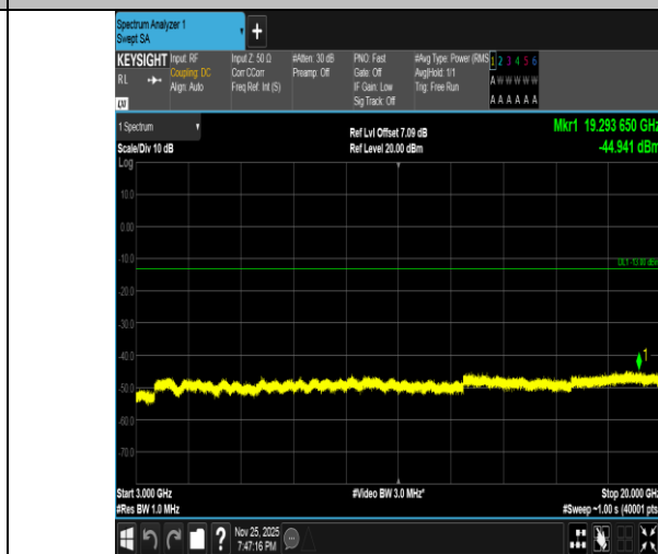
Band2-20MHz-16QAM-19100-100RB#0-3000~20000-PASS
