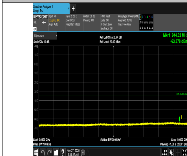
Band38-10MHz-QPSK-37800-1RB#0-30~1000-PASS
