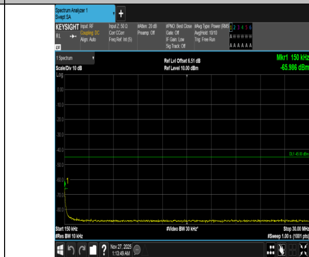
Band38-5MHz-QPSK-38000-1RB#0-0.15~30-PASS
