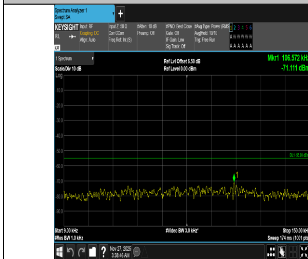
Band38-10MHz-QPSK-37800-1RB#0-0.009~0.15-PASS
