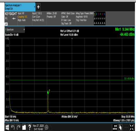
Band38-10MHz-16QAM-37800-1RB#0-0.15~30-PASS
