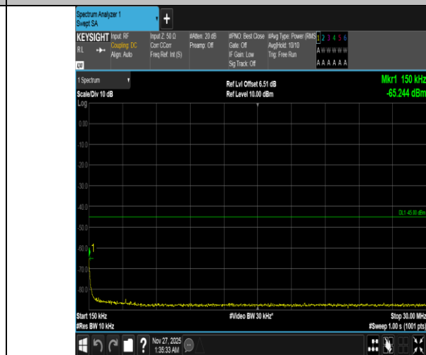
Band38-5MHz-QPSK-38000-25RB#0-0.15~30-PASS
