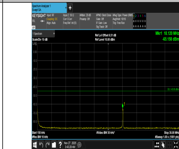
Band38-10MHz-QPSK-37800-1RB#49-0.15~30-PASS
