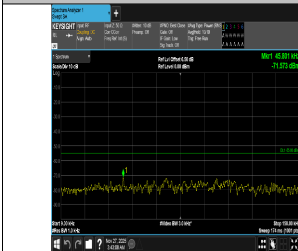
Band38-10MHz-QPSK-37800-1RB#49-0.009~0.15-PASS
