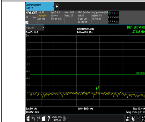
Band38-5MHz-16QAM-38000-25RB#0-0.009~0.15-PASS
