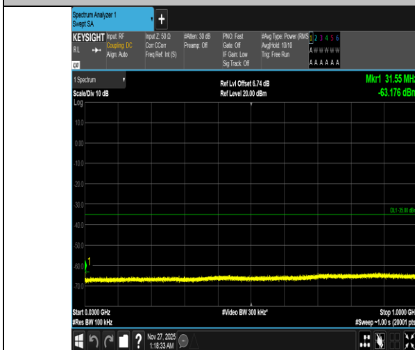
Band38-5MHz-16QAM-38000-1RB#0-30~1000-PASS
