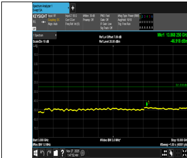
Band38-5MHz-16QAM-38000-25RB#0-3000~18000-PASS
