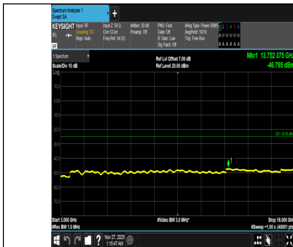
Band38-5MHz-QPSK-38000-1RB#0-3000~18000-PASS
