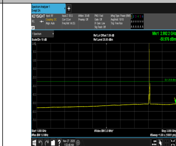
Band38-5MHz-QPSK-38225-1RB#0-1000~3000-PASS
