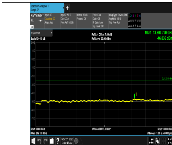
Band38-10MHz-QPSK-37800-1RB#49-3000~18000-PASS
