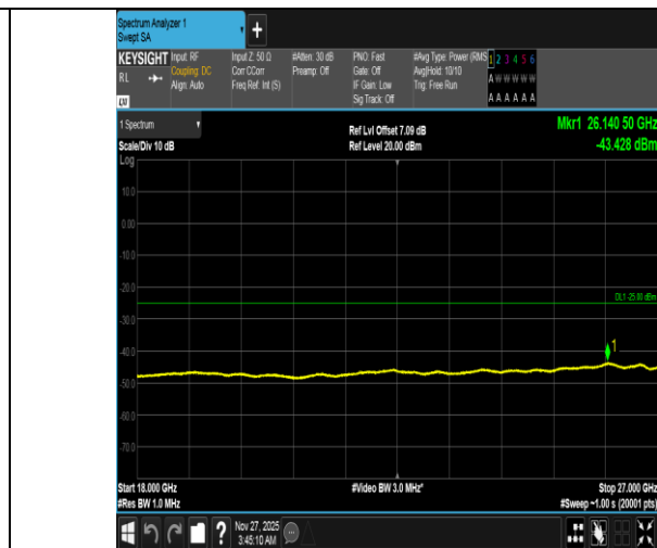
Band38-10MHz-QPSK-37800-1RB#49-18000~27000-PASS
