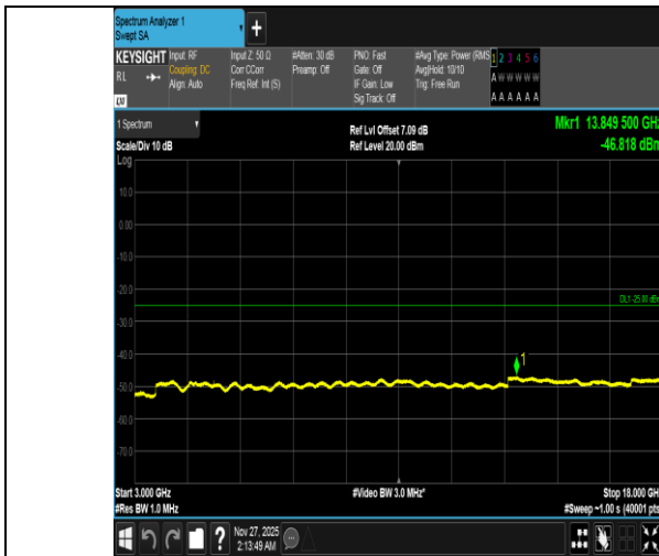
Band38-5MHz-QPSK-38225-1RB#24-3000~18000-PASS
