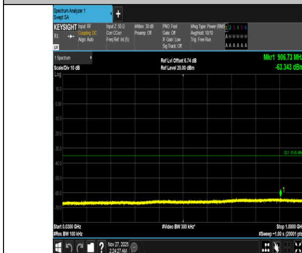
Band38-5MHz-16QAM-38225-25RB#0-30~1000-PASS
