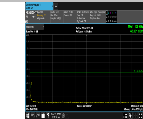
Band38-5MHz-16QAM-38000-1RB#0-0.15~30-PASS
