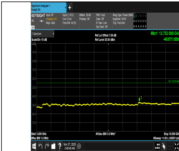
Band38-10MHz-QPSK-37800-50RB#0-3000~18000-PASS
