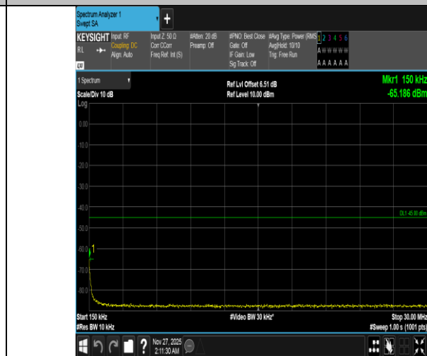
Band38-5MHz-QPSK-38225-1RB#24-0.15~30-PASS
