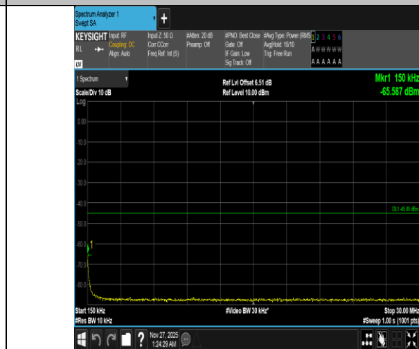
Band38-5MHz-QPSK-38000-1RB#24-0.15~30-PASS
