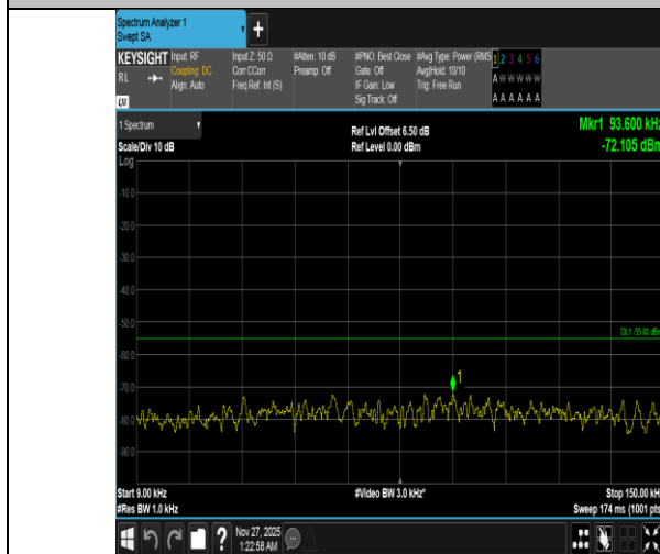
Band38-5MHz-QPSK-38000-1RB#24-0.009~0.15-PASS
