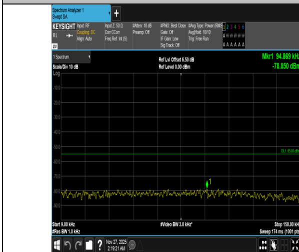
Band38-5MHz-QPSK-38225-25RB#0-0.009~0.15-PASS
