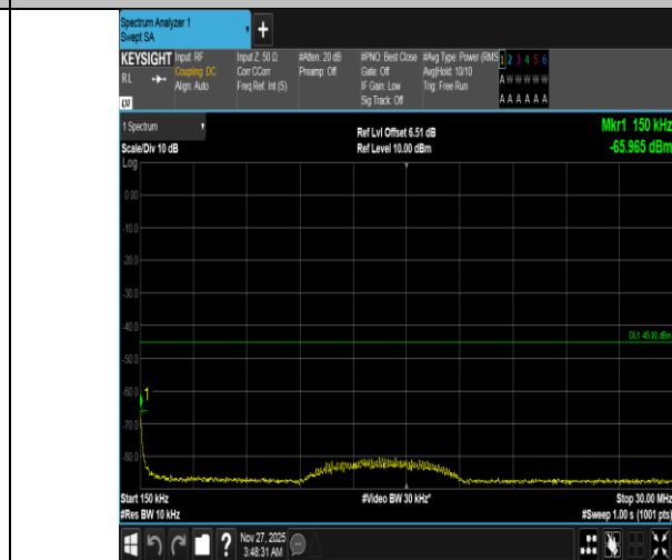
Band38-10MHz-QPSK-37800-50RB#0-0.15~30-PASS
