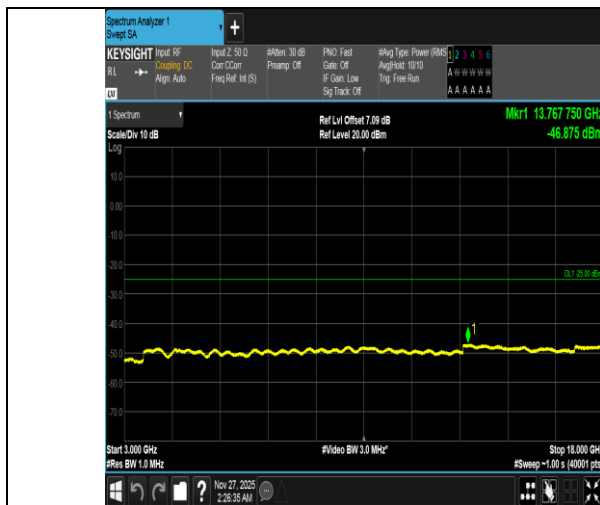
Band38-5MHz-16QAM-38225-25RB#0-3000~18000-PASS
