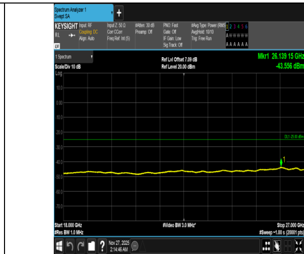
Band38-5MHz-QPSK-38225-1RB#24-18000~27000-PASS
