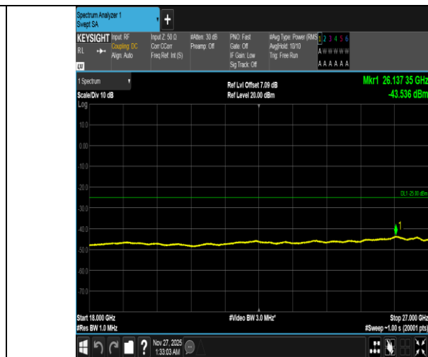
Band38-5MHz-16QAM-38000-1RB#24-18000~27000-PASS
