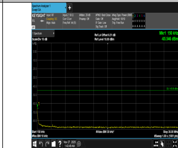
Band38-5MHz-16QAM-38000-25RB#0-0.15~30-PASS
