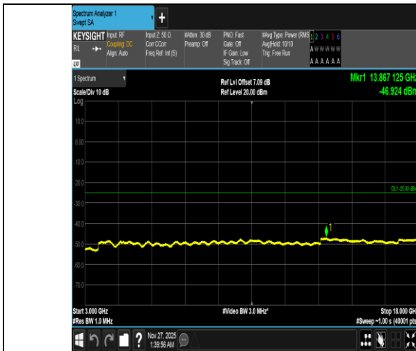
Band38-5MHz-QPSK-38000-25RB#0-3000~18000-PASS
