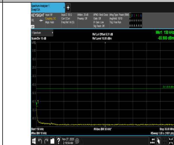
Band38-5MHz-QPSK-38225-25RB#0-0.15~30-PASS
