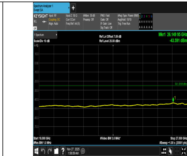
Band38-5MHz-QPSK-38225-1RB#0-18000~27000-PASS
