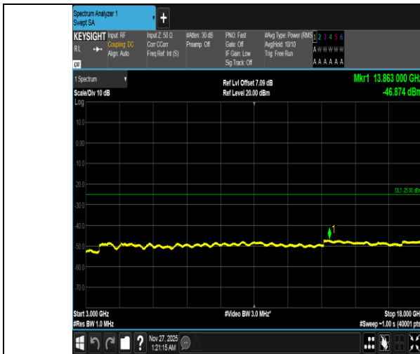
Band38-5MHz-16QAM-38000-1RB#0-3000~18000-PASS
