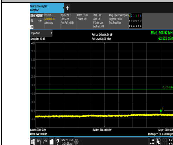
Band38-5MHz-QPSK-38225-25RB#0-30~1000-PASS
