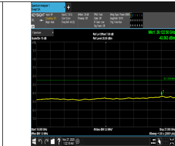
Band38-5MHz-16QAM-38000-1RB#0-18000~27000-PASS
