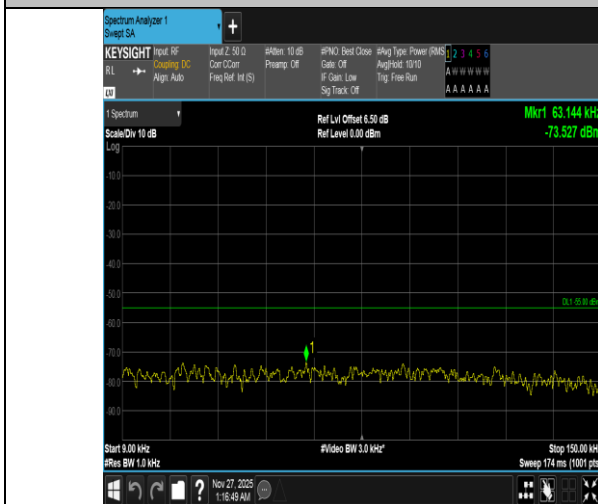
Band38-5MHz-16QAM-38000-1RB#0-0.009~0.15-PASS
