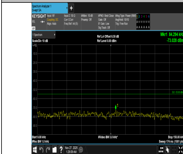
Band38-5MHz-16QAM-38000-1RB#24-0.009~0.15-PASS
