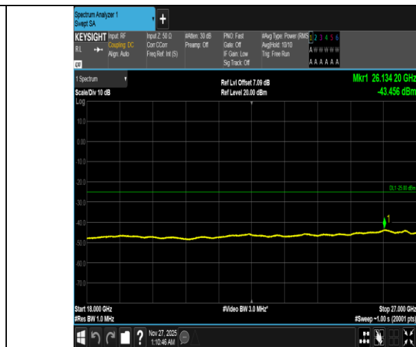
Band38-5MHz-16QAM-37775-25RB#0-18000~27000-PASS
