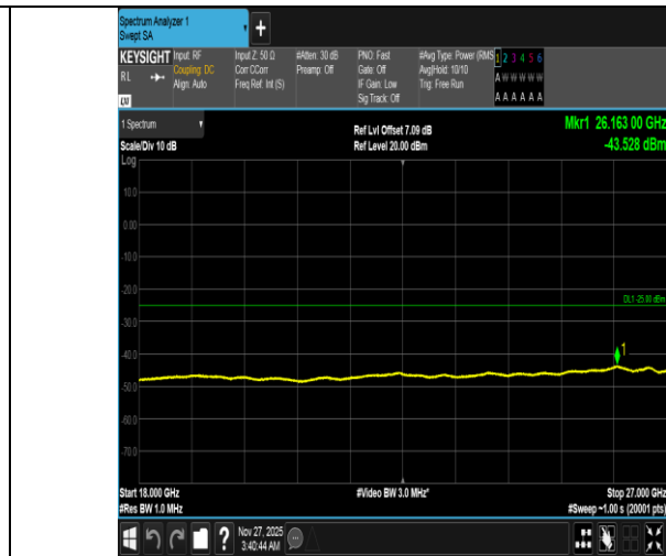
Band38-10MHz-QPSK-37800-1RB#0-18000~27000-PASS
