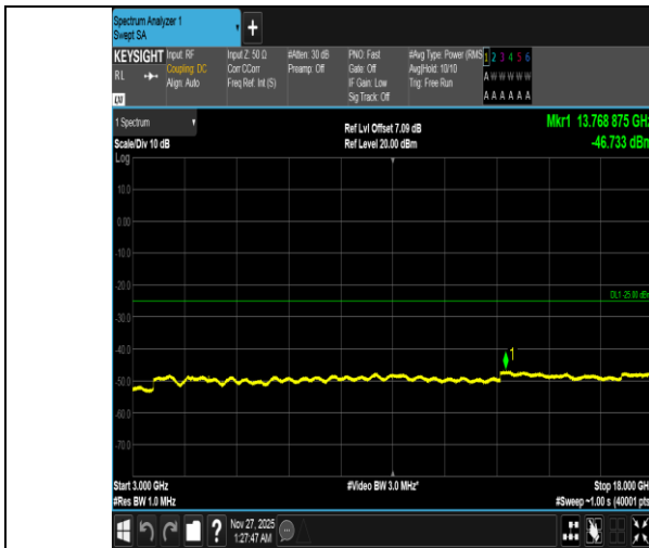
Band38-5MHz-QPSK-38000-1RB#24-3000~18000-PASS
