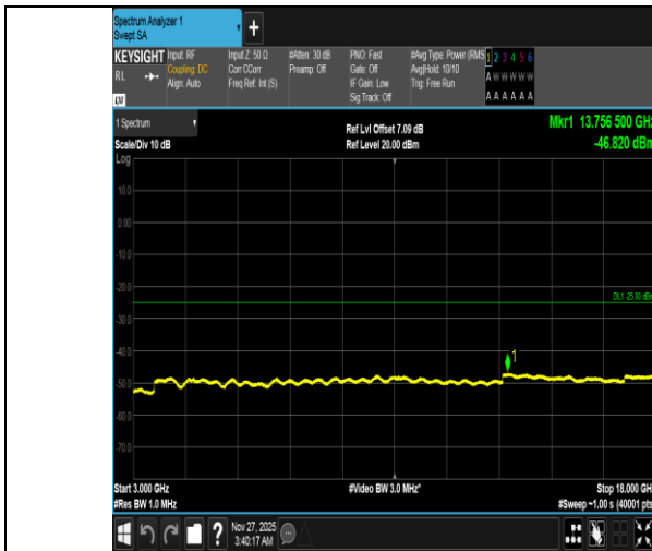
Band38-10MHz-QPSK-37800-1RB#0-3000~18000-PASS
