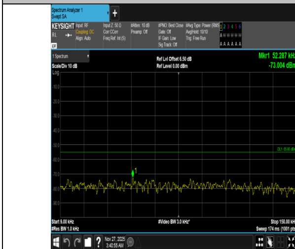
Band38-10MHz-16QAM-37800-1RB#0-0.009~0.15-PASS
