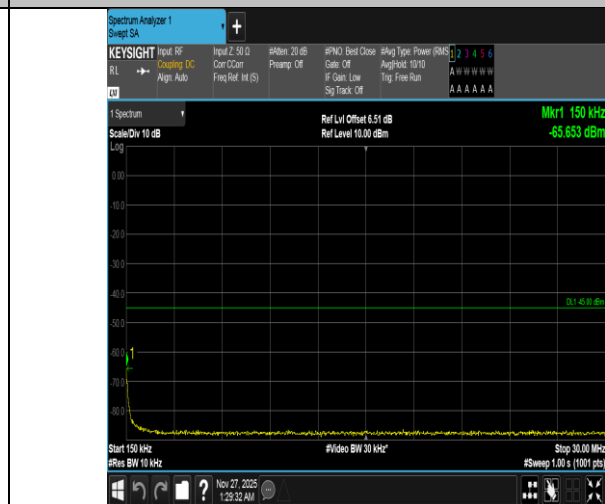
Band38-5MHz-16QAM-38000-1RB#24-0.15~30-PASS
