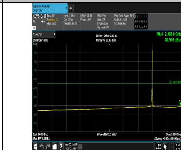
Band38-5MHz-QPSK-38000-25RB#0-1000~3000-PASS
