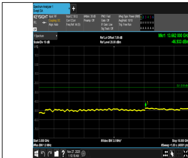
Band38-5MHz-16QAM-37775-25RB#0-3000~18000-PASS
