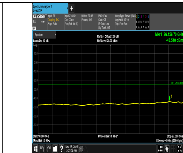
Band38-5MHz-16QAM-38225-25RB#0-18000~27000-PASS
