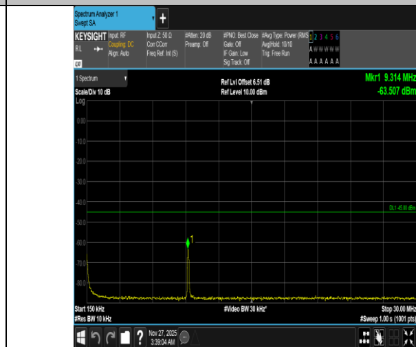
Band38-10MHz-QPSK-37800-1RB#0-0.15~30-PASS
