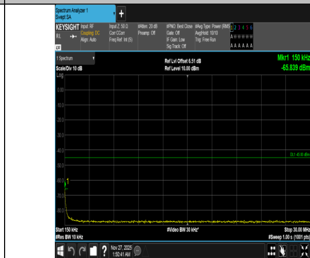
Band38-5MHz-QPSK-38225-1RB#0-0.15~30-PASS
