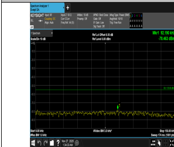
Band38-5MHz-QPSK-38000-25RB#0-0.009~0.15-PASS
