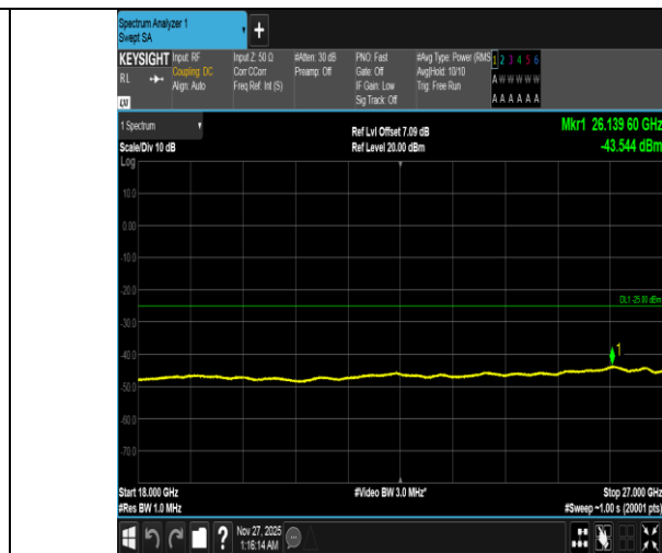
Band38-5MHz-QPSK-38000-1RB#0-18000~27000-PASS
