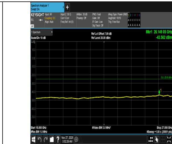
Band38-10MHz-16QAM-37800-50RB#0-18000~27000-PASS
