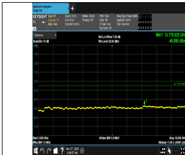
Band38-15MHz-QPSK-37825-1RB#0-3000~18000-PASS
