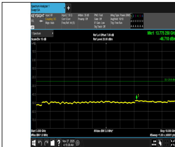
Band38-10MHz-16QAM-38200-1RB#0-3000~18000-PASS
