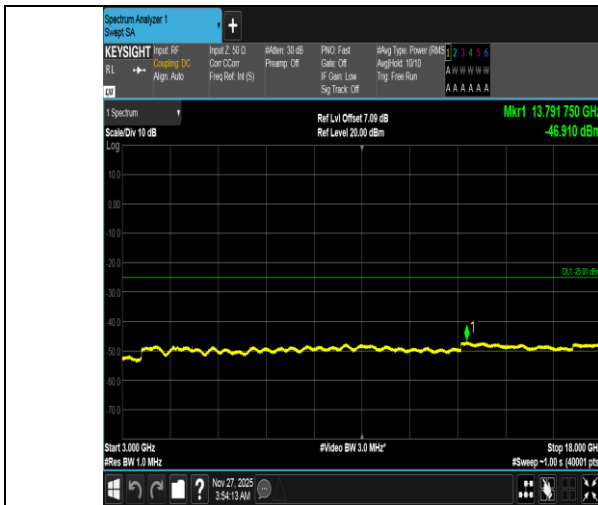
Band38-10MHz-QPSK-38000-1RB#0-3000~18000-PASS
