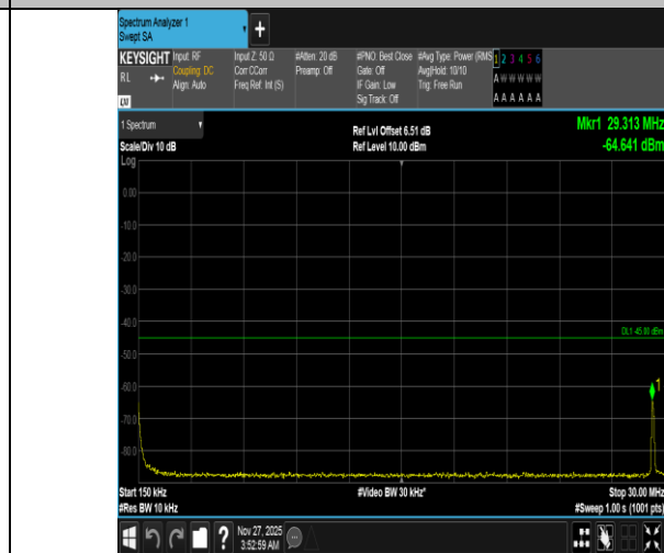
Band38-10MHz-QPSK-38000-1RB#0-0.15~30-PASS
