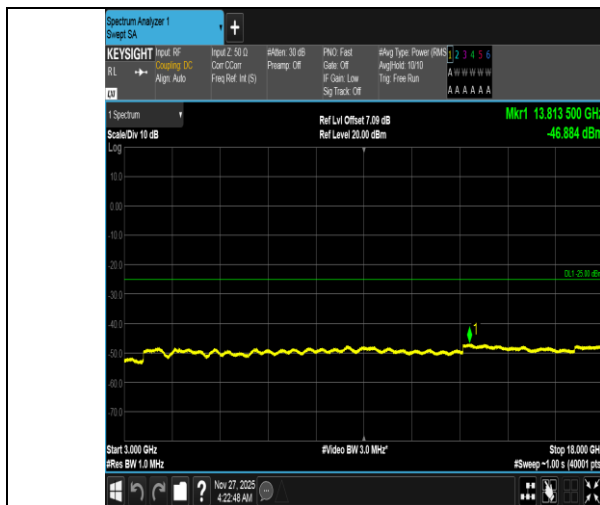
Band38-10MHz-16QAM-38200-1RB#49-3000~18000-PASS
