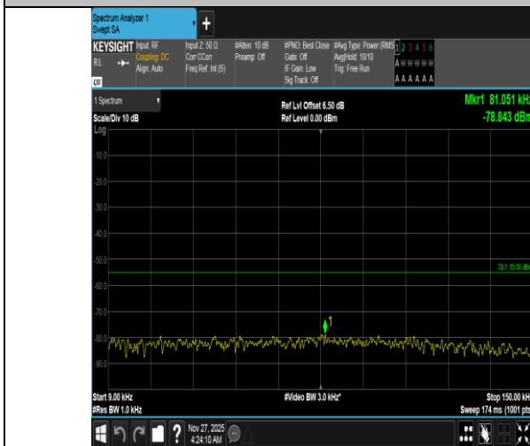
Band38-10MHz-QPSK-38200-50RB#0-0.009~0.15-PASS
