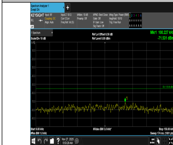
Band38-15MHz-QPSK-37825-1RB#74-0.009~0.15-PASS
