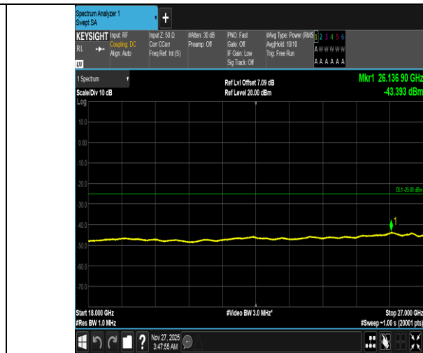
Band38-10MHz-16QAM-37800-1RB#49-18000~27000-PASS
