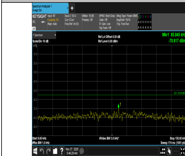
Band38-15MHz-QPSK-37825-1RB#0-0.009~0.15-PASS
