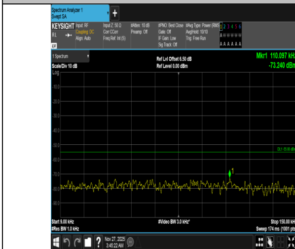
Band38-10MHz-16QAM-37800-1RB#49-0.009~0.15-PASS
