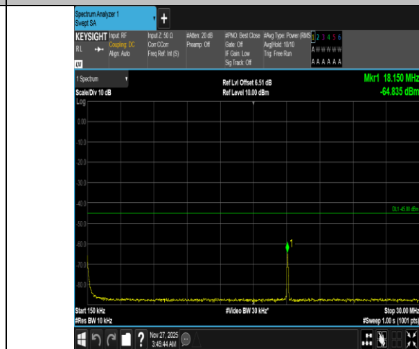
Band38-10MHz-16QAM-37800-1RB#49-0.15~30-PASS
