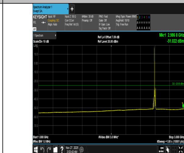
Band38-10MHz-QPSK-38000-1RB#0-1000~3000-PASS
