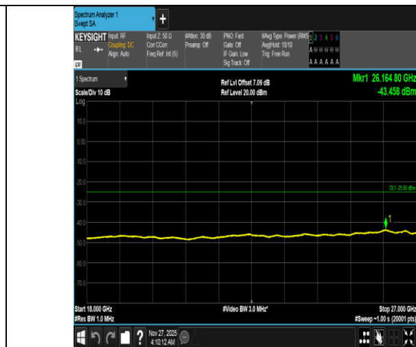
Band38-10MHz-QPSK-38200-1RB#0-18000~27000-PASS
