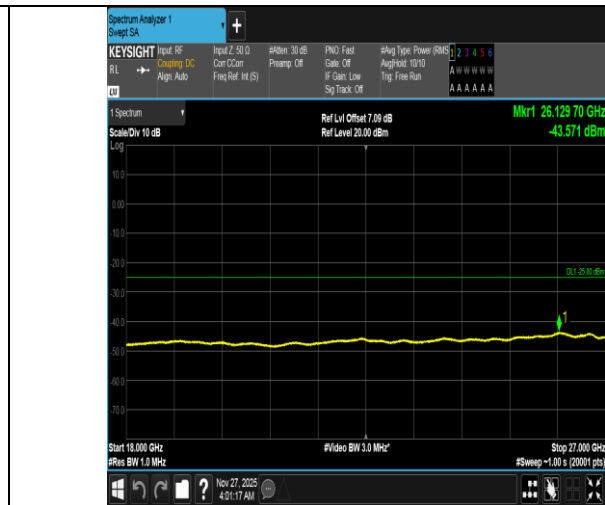
Band38-10MHz-16QAM-38000-1RB#49-18000~27000-PASS
