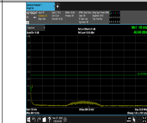
Band38-10MHz-16QAM-37800-50RB#0-0.15~30-PASS
