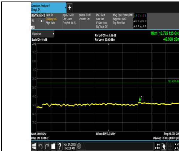
Band38-10MHz-16QAM-37800-1RB#0-3000~18000-PASS
