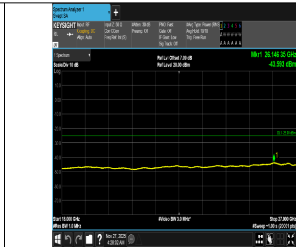
Band38-10MHz-QPSK-38200-50RB#0-18000~27000-PASS
