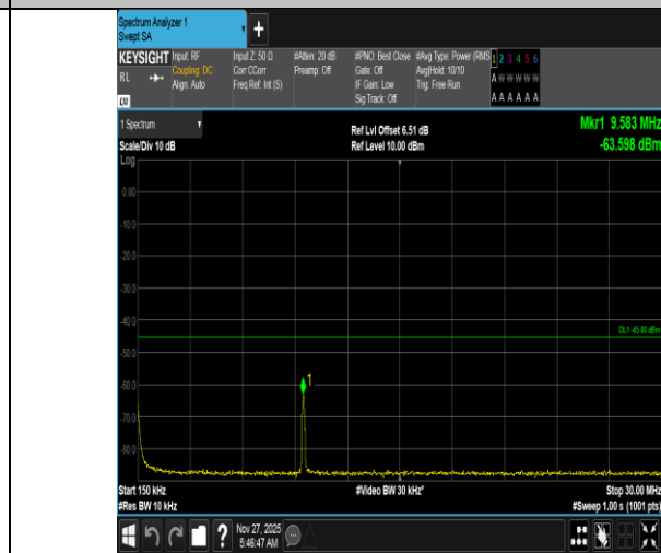
Band38-15MHz-QPSK-37825-1RB#0-0.15~30-PASS
