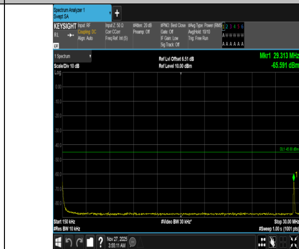
Band38-10MHz-16QAM-38000-1RB#0-0.15~30-PASS
