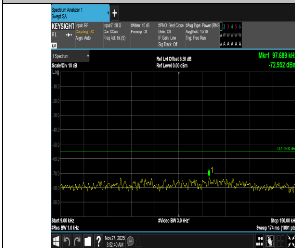
Band38-10MHz-QPSK-38000-1RB#0-0.009~0.15-PASS
