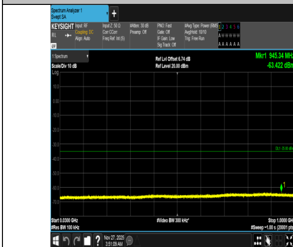
Band38-10MHz-16QAM-37800-50RB#0-30~1000-PASS
