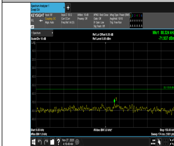
Band38-10MHz-QPSK-38200-1RB#49-0.009~0.15-PASS
