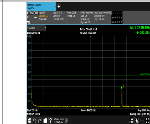
Band38-15MHz-QPSK-37825-1RB#74-0.15~30-PASS
