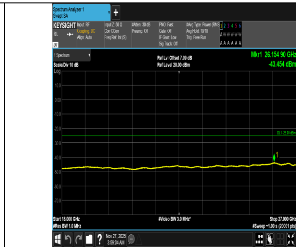
Band38-10MHz-QPSK-38000-1RB#49-18000~27000-PASS
