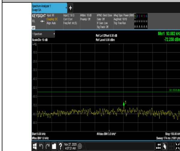
Band38-10MHz-QPSK-38200-1RB#0-0.009~0.15-PASS
