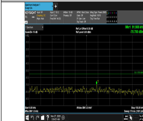
Band38-10MHz-16QAM-38000-1RB#0-0.009~0.15-PASS
