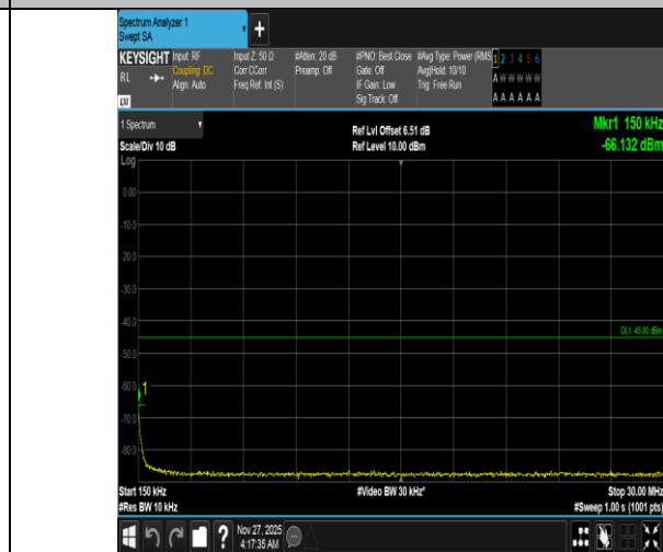
Band38-10MHz-QPSK-38200-1RB#49-0.15~30-PASS
