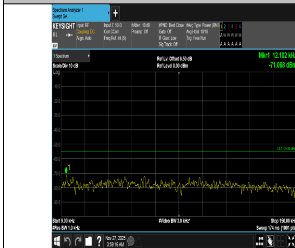
Band38-10MHz-16QAM-38000-1RB#49-0.009~0.15-PASS
