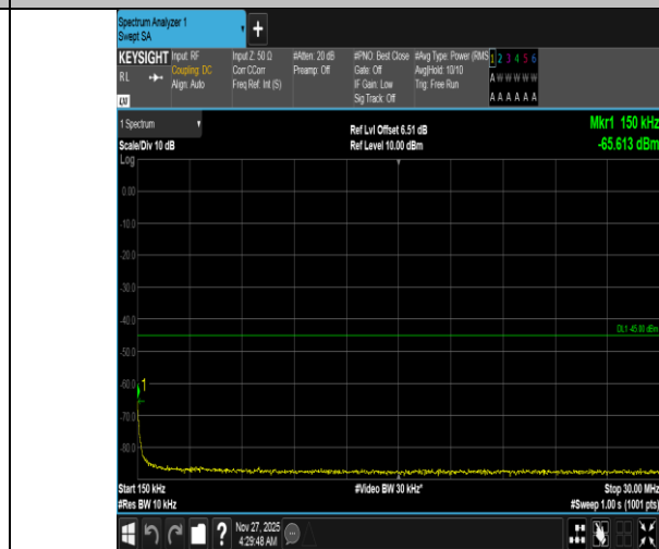
Band38-10MHz-16QAM-38200-50RB#0-0.15~30-PASS
