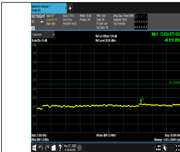
Band38-10MHz-QPSK-38200-1RB#49-3000~18000-PASS
