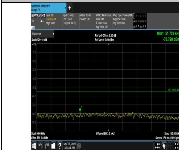
Band38-10MHz-16QAM-38000-50RB#0-0.009~0.15-PASS
