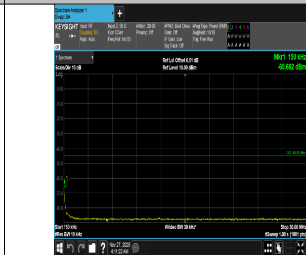
Band38-10MHz-16QAM-38200-1RB#0-0.15~30-PASS
