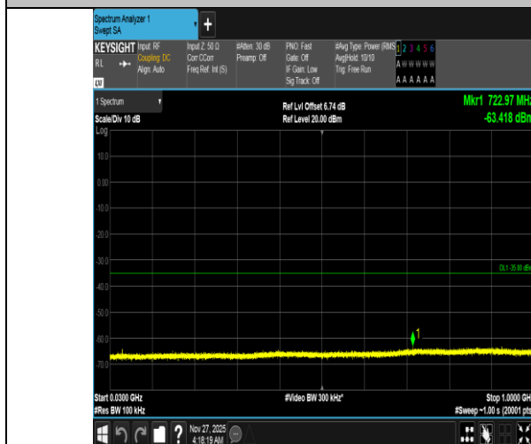
Band38-10MHz-QPSK-38200-1RB#49-30~1000-PASS
