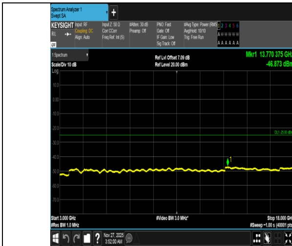
Band38-10MHz-16QAM-37800-50RB#0-3000~18000-PASS
