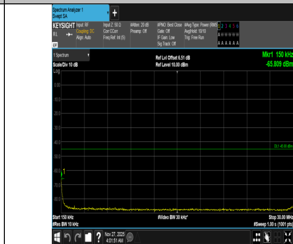
Band38-10MHz-QPSK-38000-50RB#0-0.15~30-PASS
