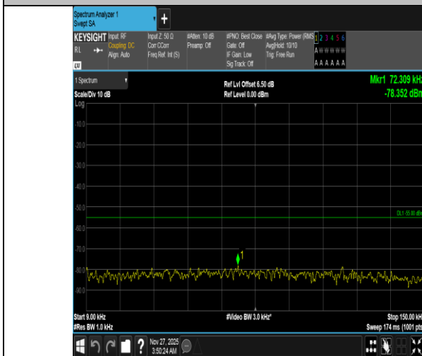
Band38-10MHz-16QAM-37800-50RB#0-0.009~0.15-PASS
