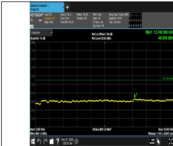
Band38-10MHz-QPSK-38000-1RB#49-3000~18000-PASS
