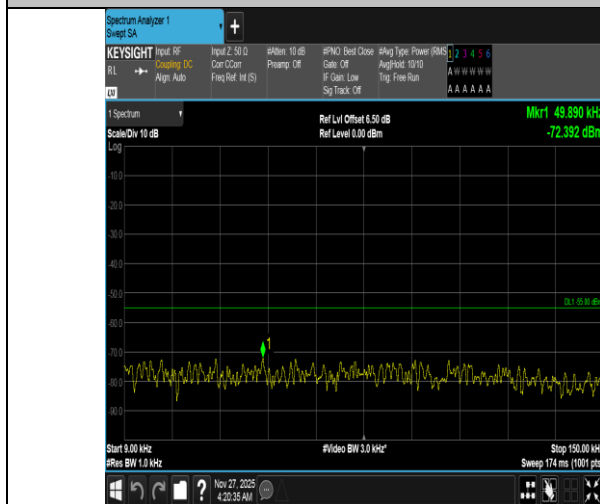
Band38-10MHz-16QAM-38200-1RB#49-0.009~0.15-PASS
