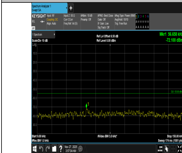
Band38-10MHz-QPSK-38000-1RB#49-0.009~0.15-PASS
