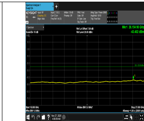
Band38-10MHz-16QAM-38000-50RB#0-18000~27000-PASS
