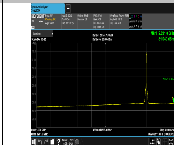
Band38-10MHz-16QAM-38000-50RB#0-1000~3000-PASS
