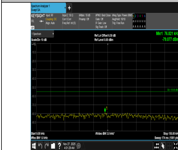
Band38-10MHz-QPSK-38000-50RB#0-0.009~0.15-PASS
