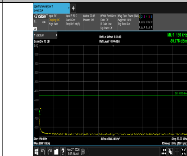
Band38-10MHz-QPSK-38000-1RB#49-0.15~30-PASS
