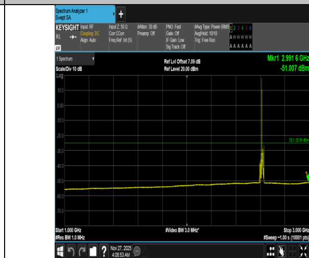
Band38-10MHz-QPSK-38200-1RB#0-1000~3000-PASS
