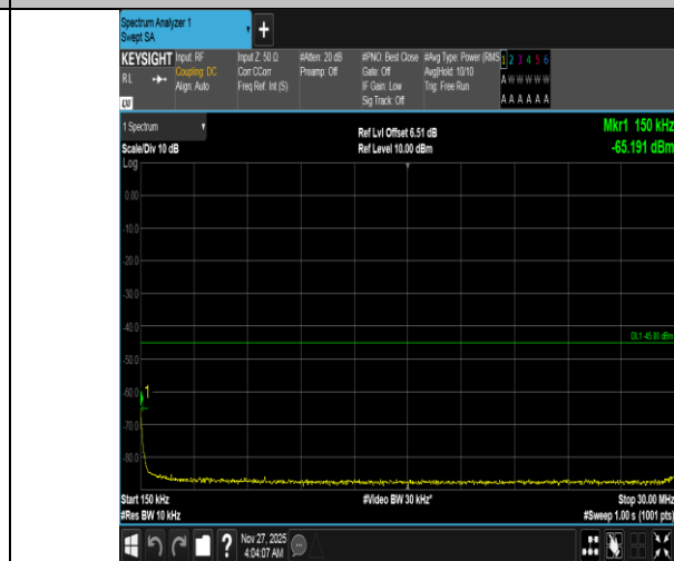
Band38-10MHz-16QAM-38000-50RB#0-0.15~30-PASS
