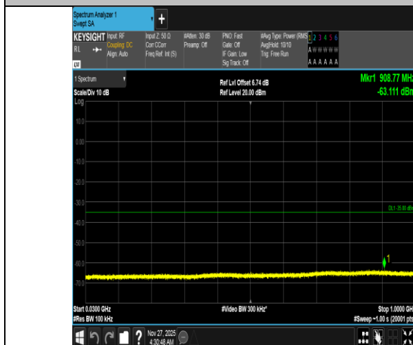
Band38-10MHz-16QAM-38200-50RB#0-30~1000-PASS
