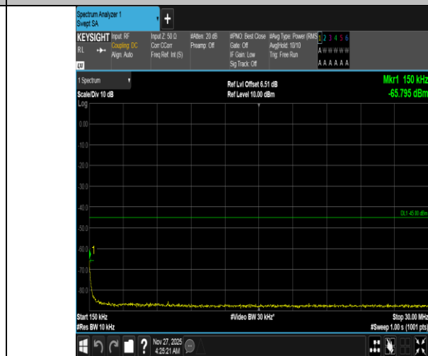
Band38-10MHz-QPSK-38200-50RB#0-0.15~30-PASS
