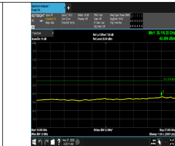
Band38-10MHz-QPSK-38200-1RB#49-18000~27000-PASS
