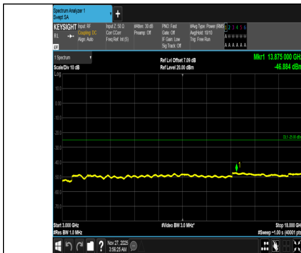
Band38-10MHz-16QAM-38000-1RB#0-3000~18000-PASS
