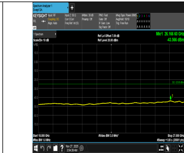
Band38-10MHz-QPSK-38000-1RB#0-18000~27000-PASS
