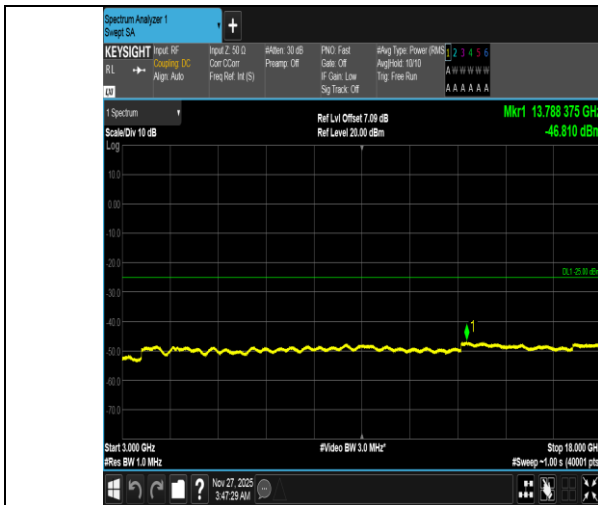
Band38-10MHz-16QAM-37800-1RB#49-3000~18000-PASS
