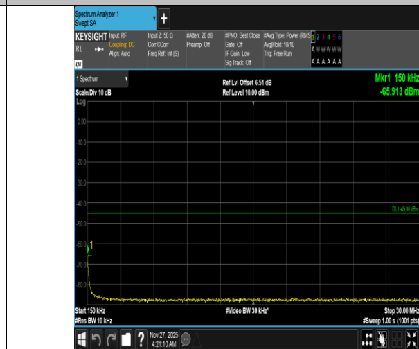
Band38-10MHz-16QAM-38200-1RB#49-0.15~30-PASS
