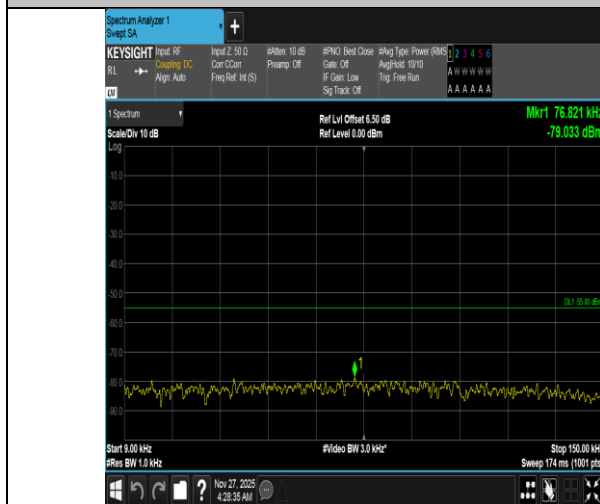
Band38-10MHz-16QAM-38200-50RB#0-0.009~0.15-PASS
