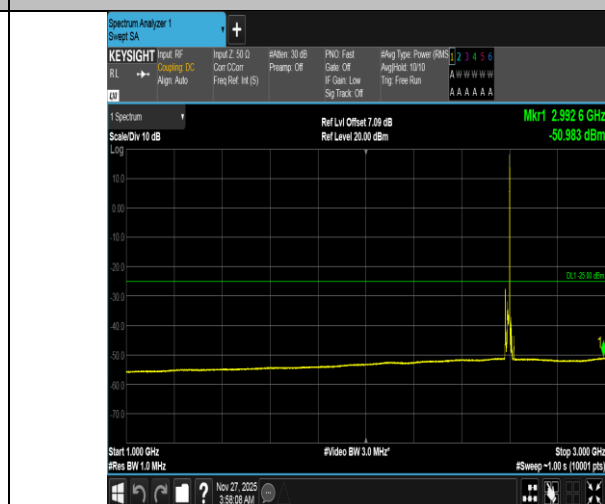
Band38-10MHz-QPSK-38000-1RB#49-1000~3000-PASS
