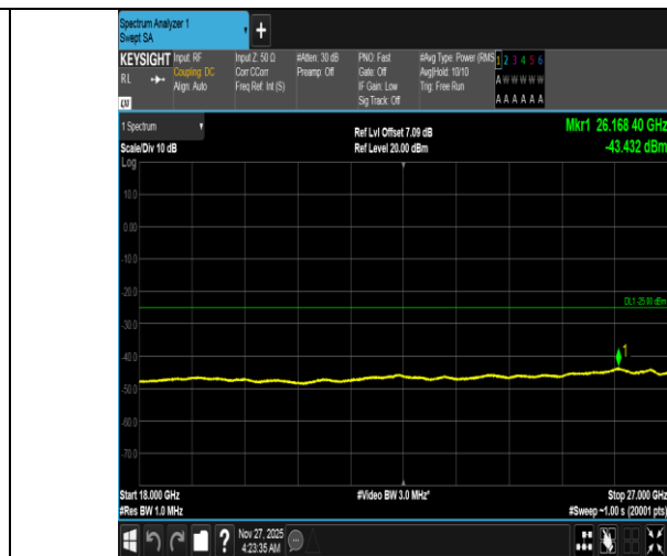
Band38-10MHz-16QAM-38200-1RB#49-18000~27000-PASS
