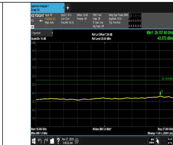
Band38-10MHz-16QAM-38000-1RB#0-18000~27000-PASS
