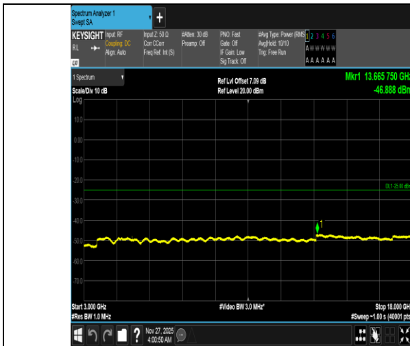
Band38-10MHz-16QAM-38000-1RB#49-3000~18000-PASS
