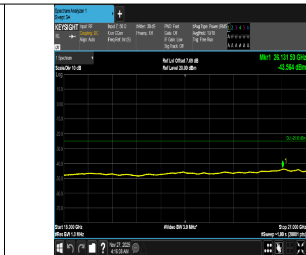
Band38-10MHz-16QAM-38200-1RB#0-18000~27000-PASS
