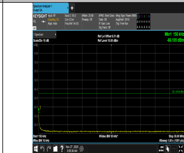
Band38-10MHz-16QAM-38000-1RB#49-0.15~30-PASS
