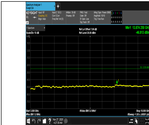
Band38-10MHz-QPSK-38200-50RB#0-3000~18000-PASS
