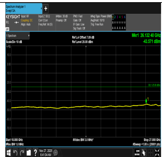
Band38-15MHz-QPSK-38175-75RB#0-18000~27000-PASS
