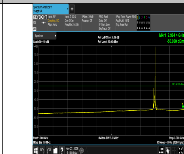
Band38-15MHz-QPSK-38000-1RB#74-1000~3000-PASS
