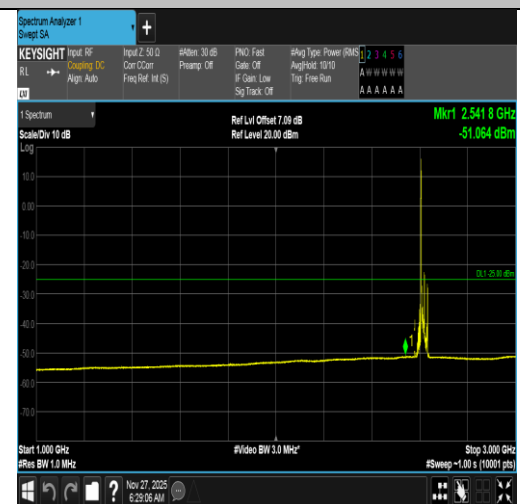
Band38-15MHz-16QAM-38175-1RB#0-1000~3000-PASS
