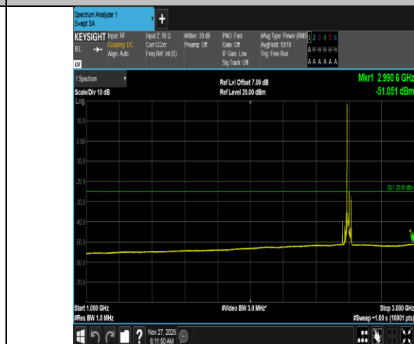
Band38-15MHz-16QAM-38000-1RB#0-1000~3000-PASS
