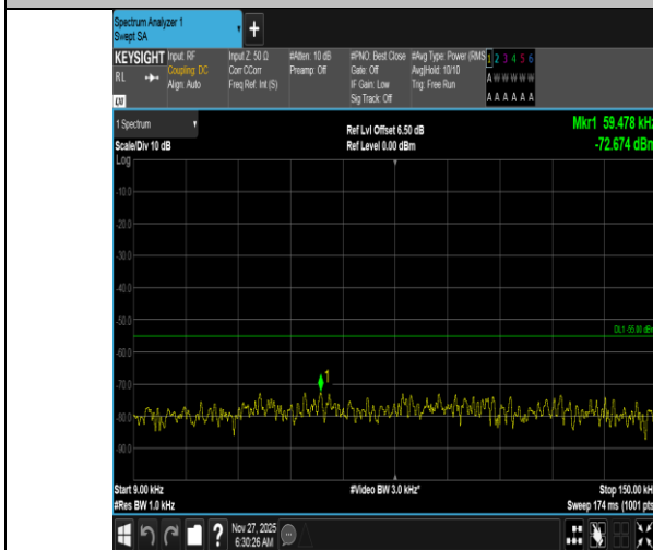
Band38-15MHz-QPSK-38175-1RB#74-0.009~0.15-PASS
