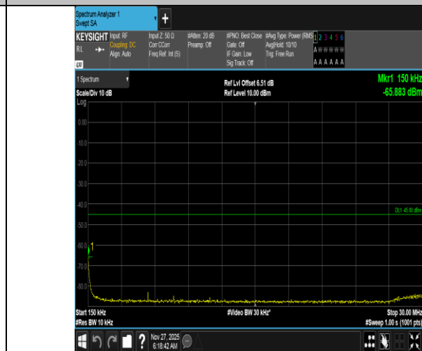
Band38-15MHz-QPSK-38000-75RB#0-0.15~30-PASS
