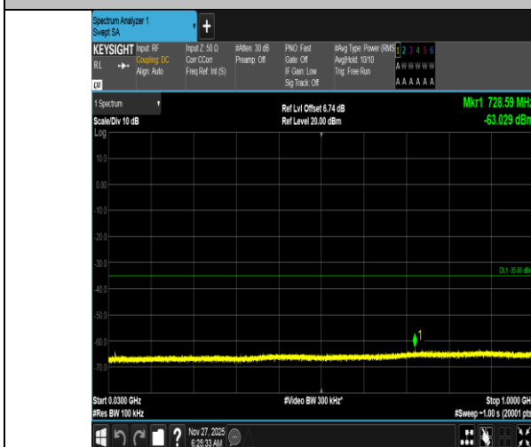
Band38-15MHz-QPSK-38175-1RB#0-30~1000-PASS
