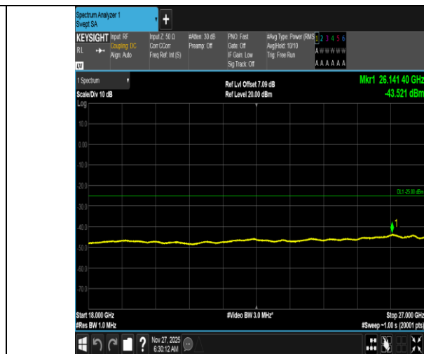
Band38-15MHz-16QAM-38175-1RB#0-18000~27000-PASS
