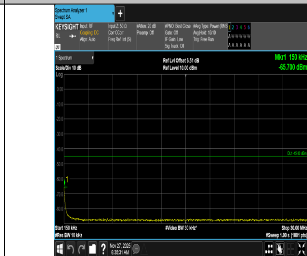
Band38-15MHz-16QAM-38175-1RB#74-0.15~30-PASS
