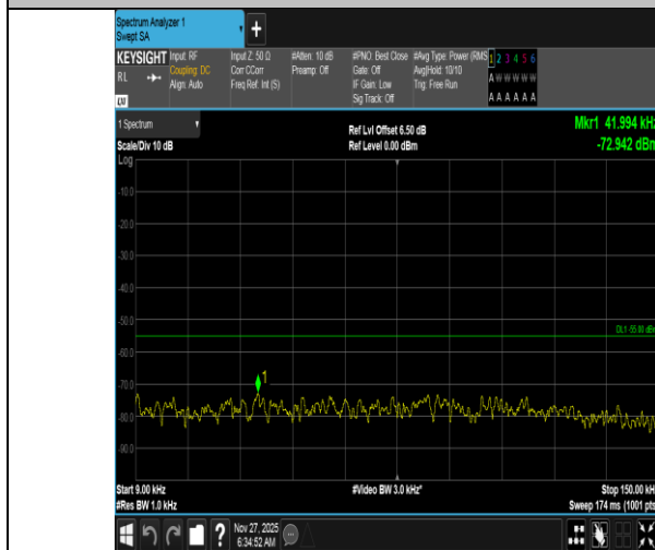
Band38-15MHz-16QAM-38175-1RB#74-0.009~0.15-PASS
