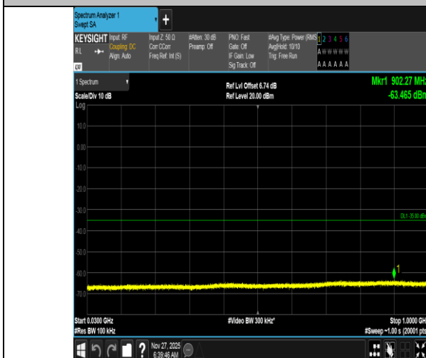
Band38-15MHz-QPSK-38175-75RB#0-30~1000-PASS
