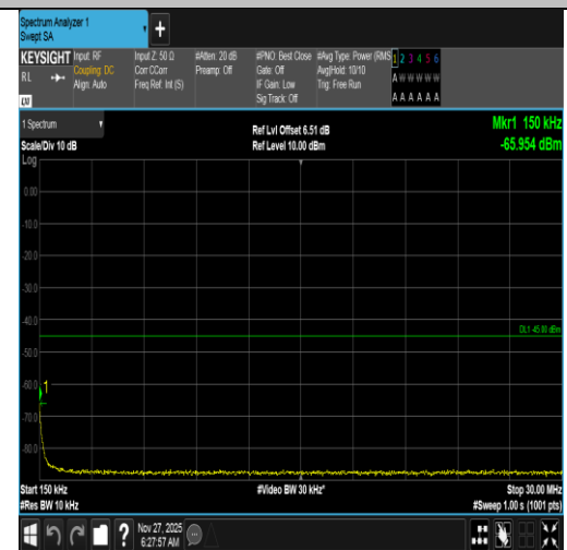
Band38-15MHz-16QAM-38175-1RB#0-0.15~30-PASS
