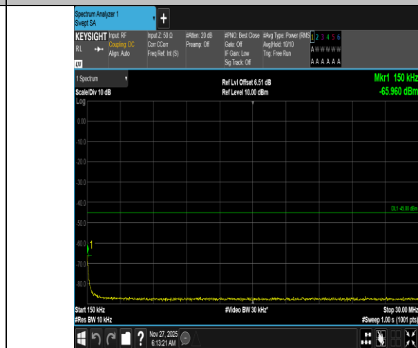
Band38-15MHz-QPSK-38000-1RB#74-0.15~30-PASS
