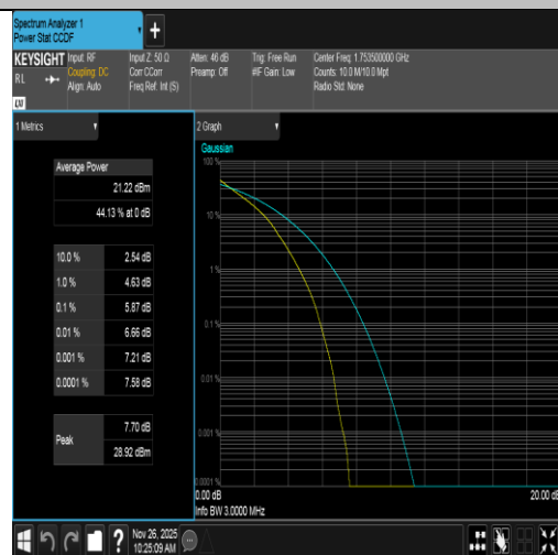
Band4-3MHz-QPSK-20385-15RB#0-PASS
