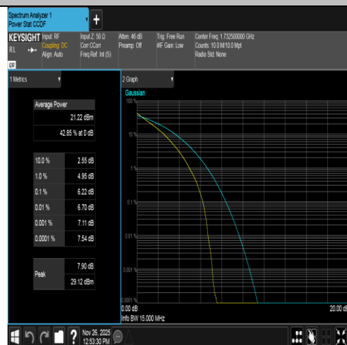
Band4-15MHz-QPSK-20175-75RB#0-PASS
