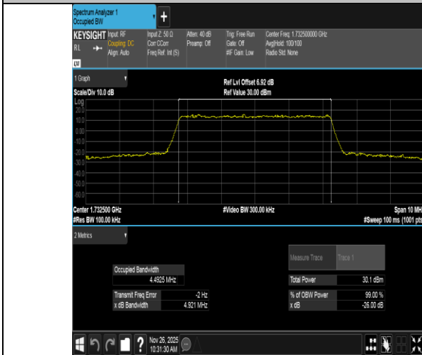
Band4-5MHz-QPSK-20175-25RB#0-PASS
