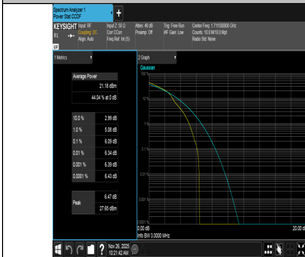
Band4-3MHz-16QAM-19965-1RB#0-PASS
