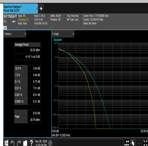
Band4-15MHz-16QAM-20025-75RB#0-PASS
