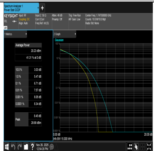
Band4-15MHz-16QAM-20325-75RB#0-PASS
