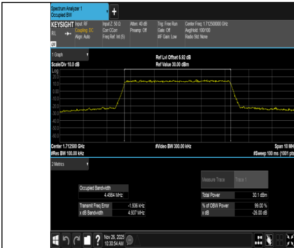
Band4-5MHz-QPSK-19975-25RB#0-PASS
