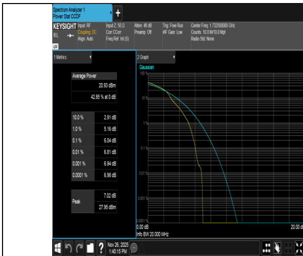
Band4-20MHz-16QAM-20175-1RB#0-PASS
