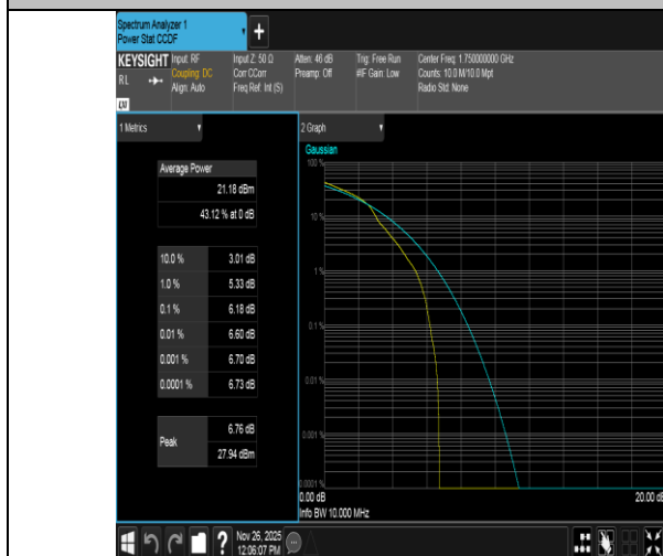
Band4-10MHz-16QAM-20350-1RB#0-PASS
