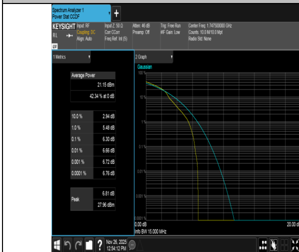
Band4-15MHz-16QAM-20325-1RB#0-PASS
