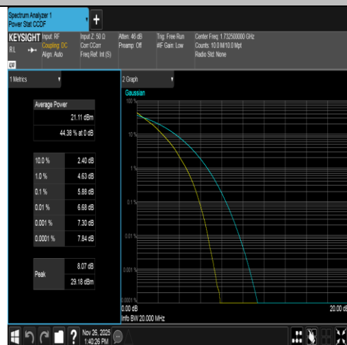
Band4-20MHz-QPSK-20175-100RB#0-PASS
