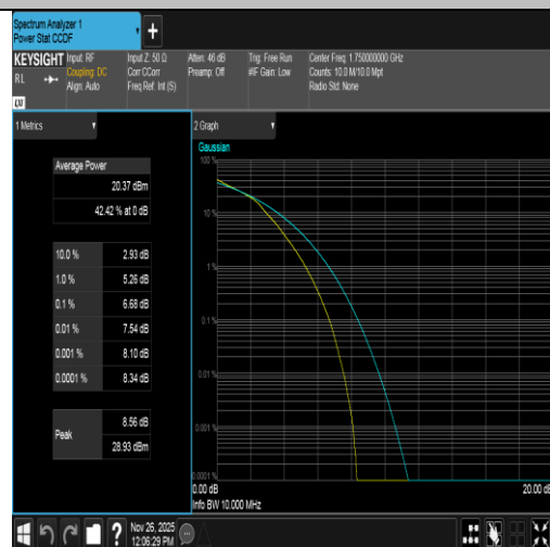
Band4-10MHz-16QAM-20350-50RB#0-PASS
