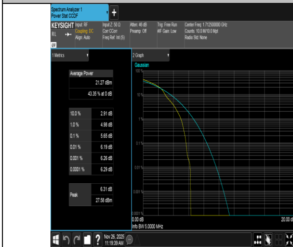
Band4-5MHz-16QAM-19975-1RB#0-PASS
