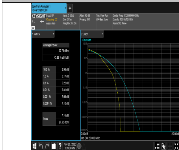
Band4-20MHz-16QAM-20050-1RB#0-PASS
