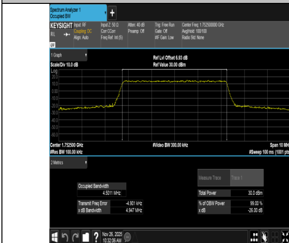
Band4-5MHz-QPSK-20375-25RB#0-PASS
