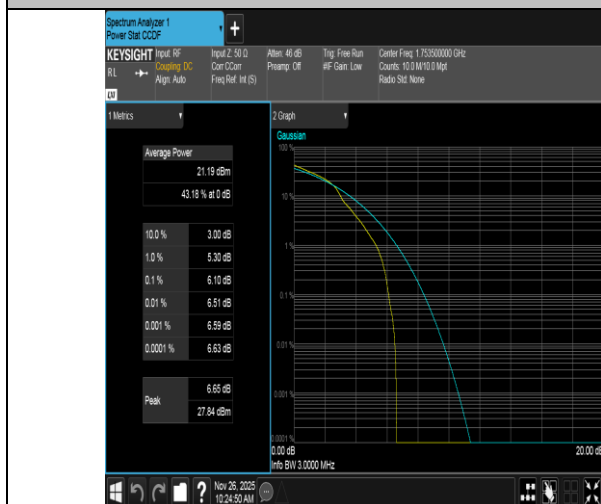
Band4-3MHz-16QAM-20385-1RB#0-PASS
