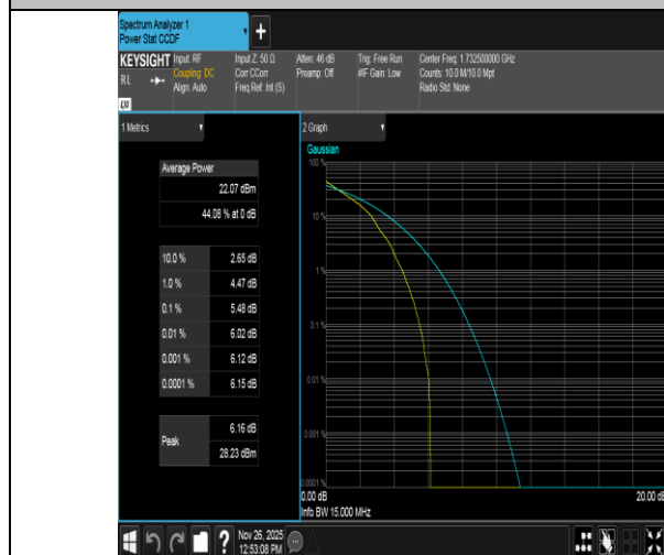
Band4-15MHz-QPSK-20175-1RB#0-PASS
