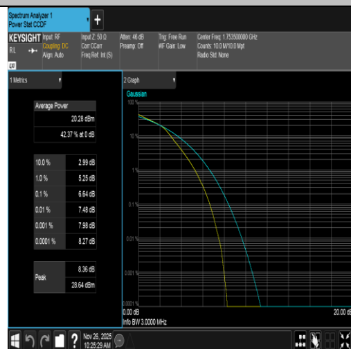
Band4-3MHz-16QAM-20385-15RB#0-PASS
