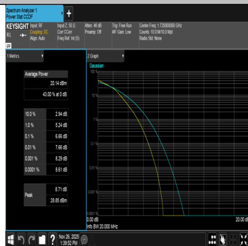
Band4-20MHz-16QAM-20050-100RB#0-PASS
