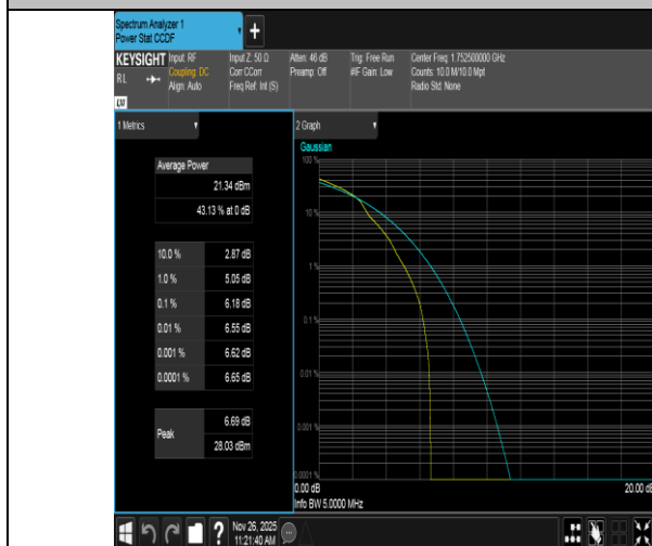
Band4-5MHz-16QAM-20375-1RB#0-PASS
