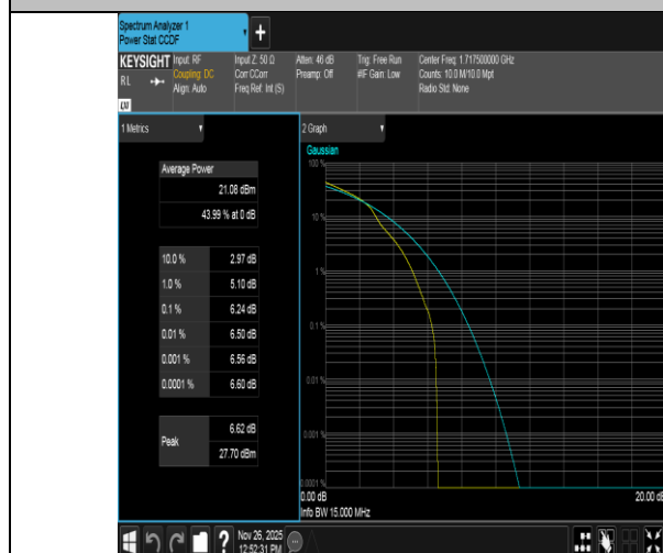
Band4-15MHz-16QAM-20025-1RB#0-PASS
