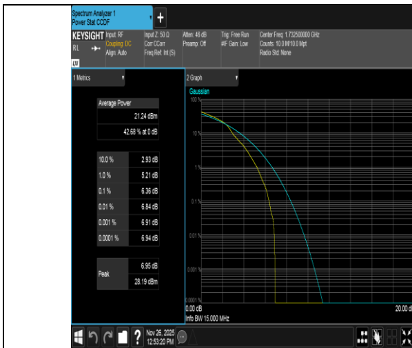
Band4-15MHz-16QAM-20175-1RB#0-PASS
