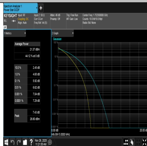
Band4-5MHz-QPSK-20375-25RB#0-PASS
