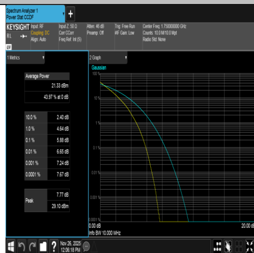
Band4-10MHz-QPSK-20350-50RB#0-PASS
