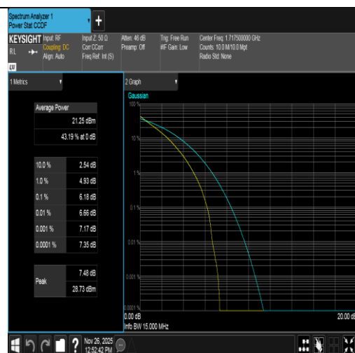
Band4-15MHz-QPSK-20025-75RB#0-PASS
