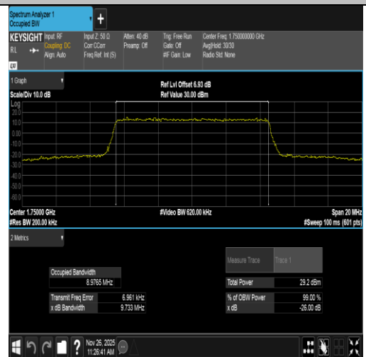
Band4-10MHz-16QAM-20350-50RB#0-PASS
