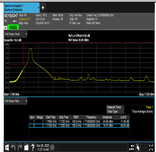
Band4-10MHz-16QAM-20000-1RB#0-PASS
