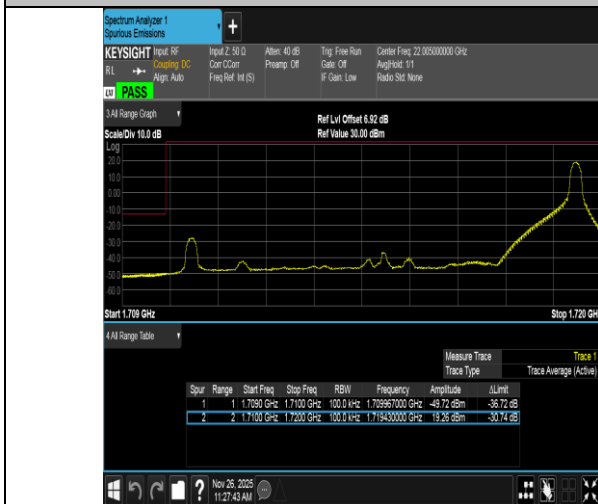
Band4-10MHz-16QAM-20000-1RB#49-PASS
