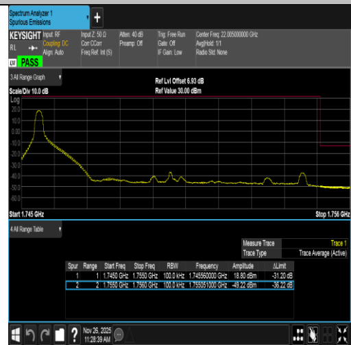
Band4-10MHz-16QAM-20350-1RB#0-PASS
