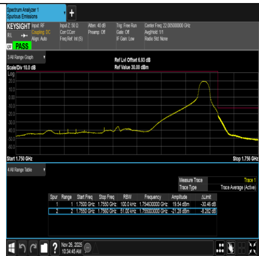
Band4-5MHz-QPSK-20375-1RB#24-PASS
