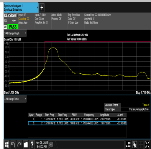
Band4-3MHz-16QAM-19965-1RB#0-PASS
