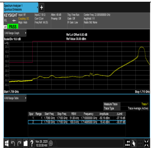
Band4-5MHz-QPSK-19975-1RB#24-PASS
