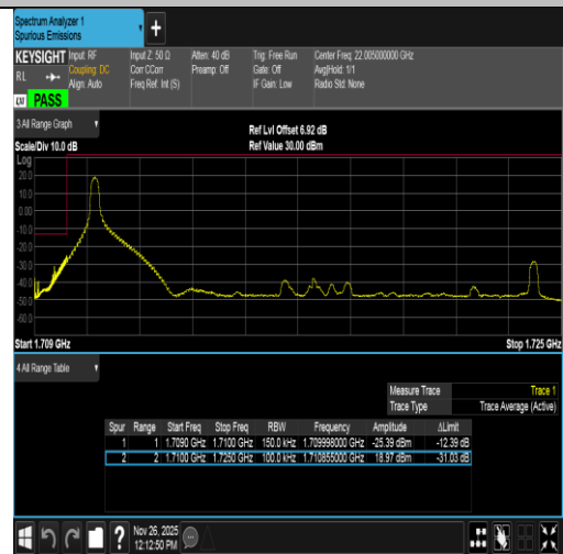
Band4-15MHz-16QAM-20025-1RB#0-PASS
