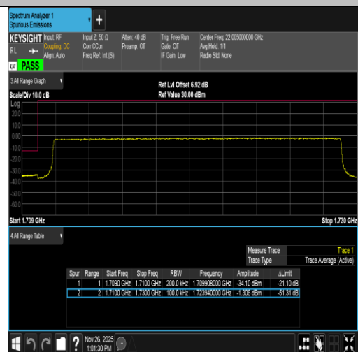
Band4-20MHz-16QAM-20050-100RB#0-PASS
