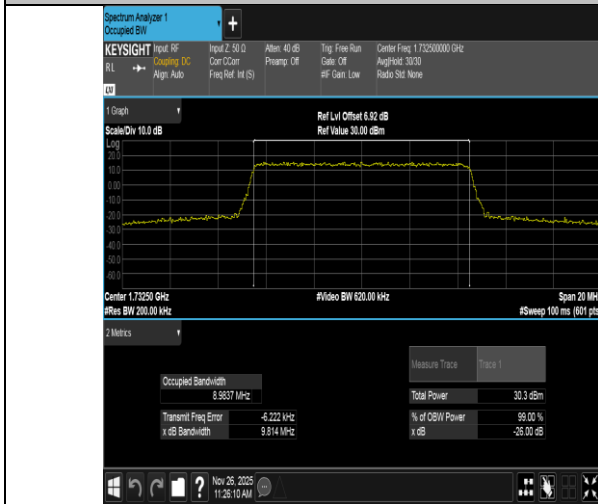
Band4-10MHz-QPSK-17175-50RB#0-PASS
