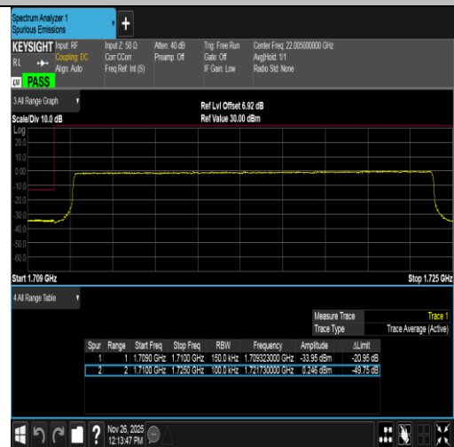
Band4-15MHz-16QAM-20025-75RB#0-PASS
