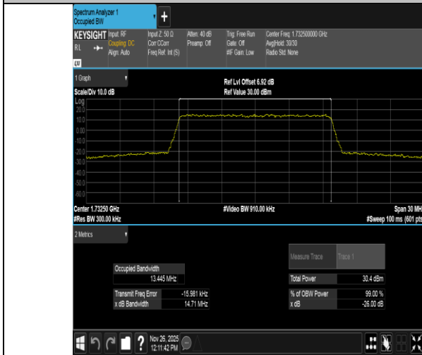
Band4-15MHz-QPSK-20175-75RB#0-PASS
