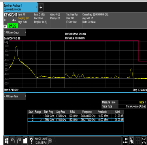
Band4-15MHz-16QAM-20325-1RB#0-PASS
