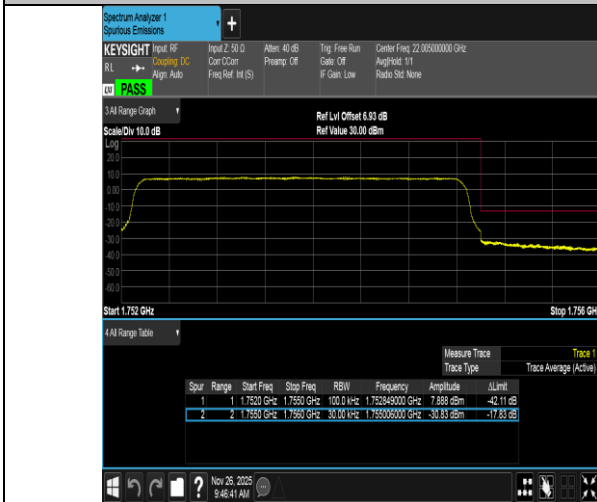
Band4-3MHz-QPSK-20385-15RB#0-PASS
