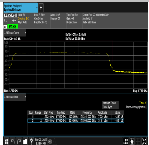
Band4-3MHz-16QAM-20385-15RB#0-PASS
