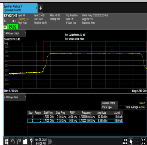
Band4-3MHz-16QAM-19965-15RB#0-PASS
