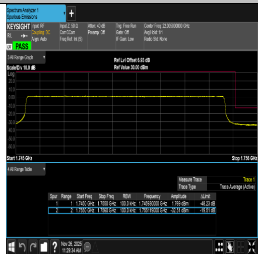
Band4-10MHz-16QAM-20350-50RB#0-PASS
