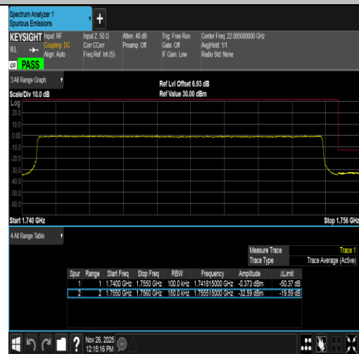
Band4-15MHz-16QAM-20325-75RB#0-PASS
