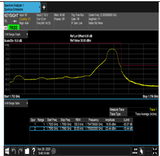
Band4-3MHz-QPSK-20385-1RB#14-PASS
