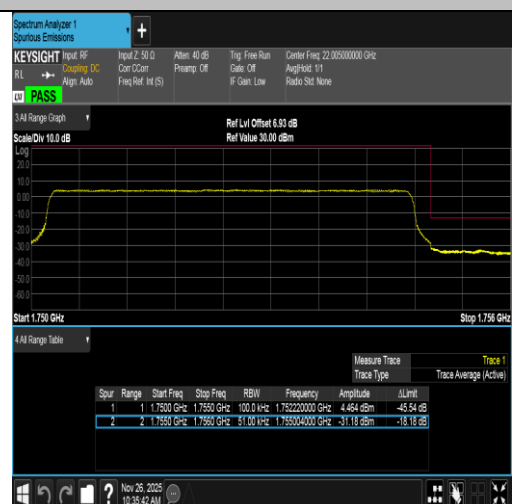
Band4-5MHz-16QAM-20375-25RB#0-PASS
