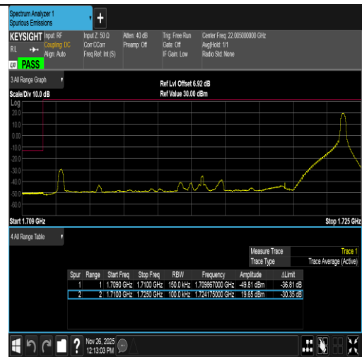
Band4-15MHz-QPSK-20025-1RB#74-PASS
