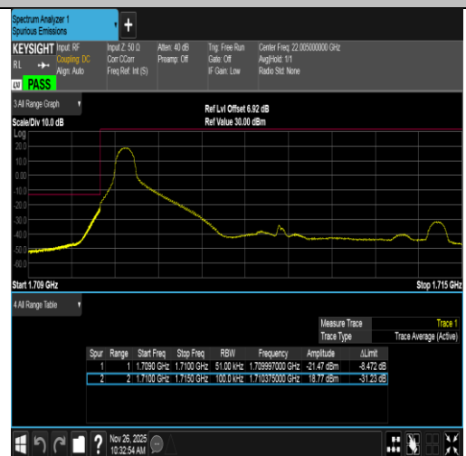
Band4-5MHz-16QAM-19975-1RB#0-PASS
