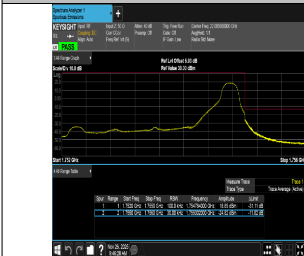
Band4-3MHz-16QAM-20385-1RB#14-PASS
