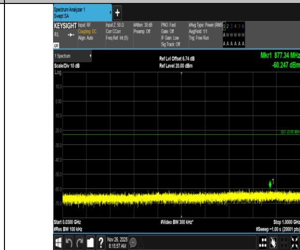
Band4-1.4MHz-16QAM-20175-6RB#0-30~1000-PASS
