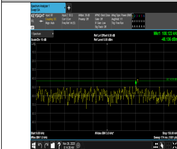
Band4-1.4MHz-QPSK-20175-6RB#0-0.009~0.15-PASS
