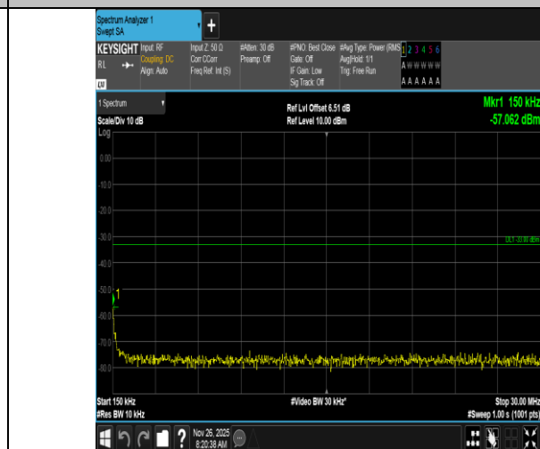
Band4-1.4MHz-QPSK-20393-6RB#0-0.15~30-PASS
