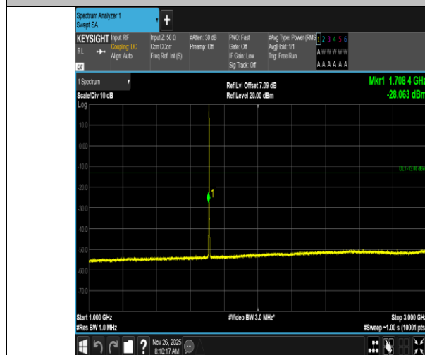
Band4-1.4MHz-16QAM-19957-6RB#0-1000~3000-PASS
