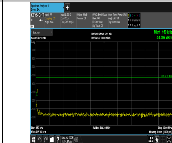
Band4-1.4MHz-QPSK-20175-6RB#0-0.15~30-PASS
