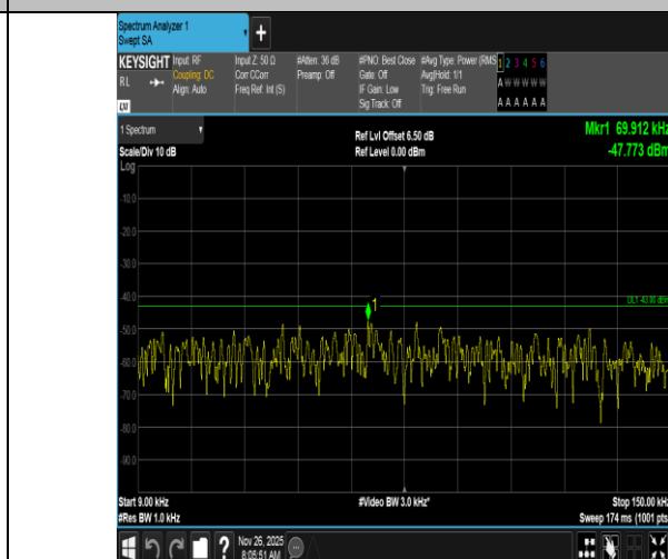
Band4-1.4MHz-16QAM-19957-1RB#0-0.009~0.15-PASS
