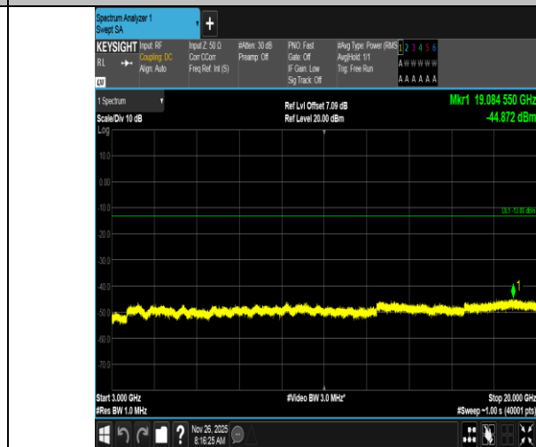
Band4-1.4MHz-16QAM-20175-6RB#0-3000~20000-PASS
