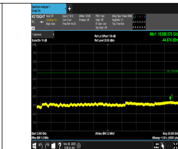
Band4-1.4MHz-16QAM-19957-1RB#0-3000~20000-PASS
