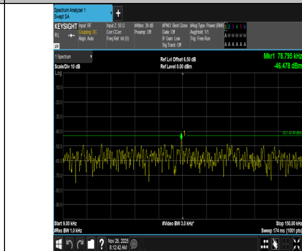
Band4-1.4MHz-QPSK-20175-1RB#5-0.009~0.15-PASS
