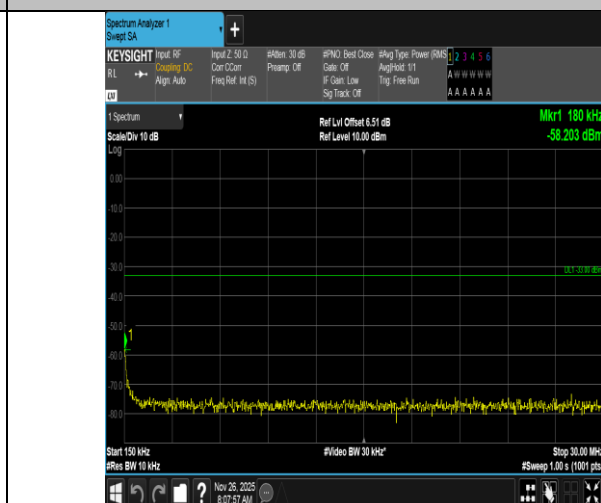
Band4-1.4MHz-16QAM-19957-1RB#5-0.15~30-PASS
