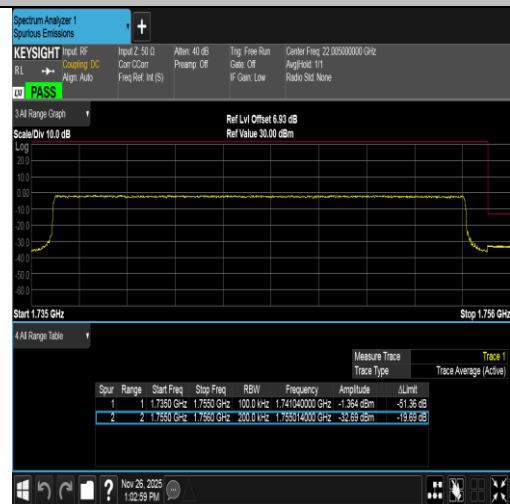
Band4-20MHz-16QAM-20300-100RB#0-PASS
