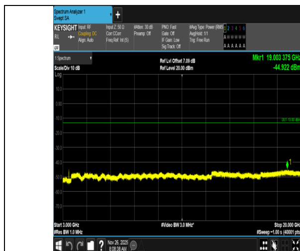
Band4-1.4MHz-16QAM-19957-1RB#5-3000~20000-PASS
