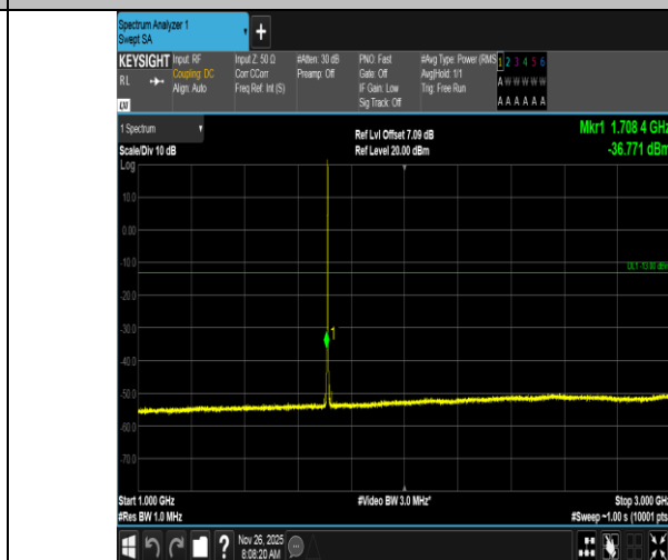
Band4-1.4MHz-16QAM-19957-1RB#5-1000~3000-PASS
