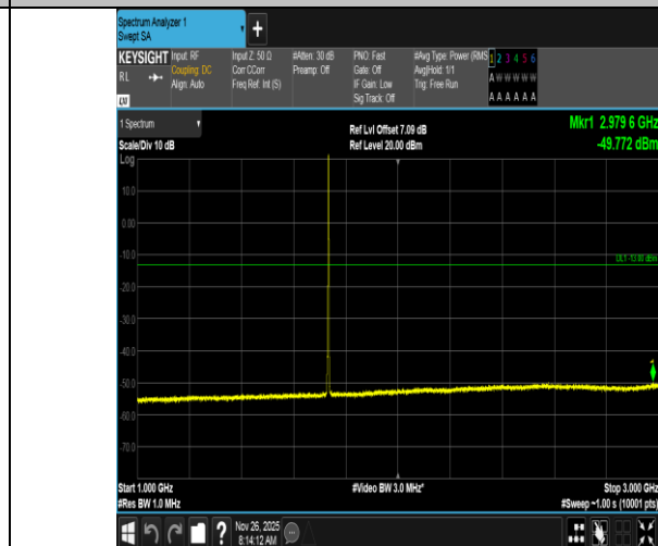
Band4-1.4MHz-16QAM-20175-1RB#5-1000~3000-PASS
