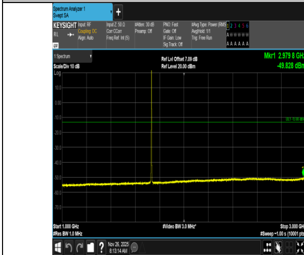
Band4-1.4MHz-QPSK-20175-1RB#5-1000~3000-PASS
