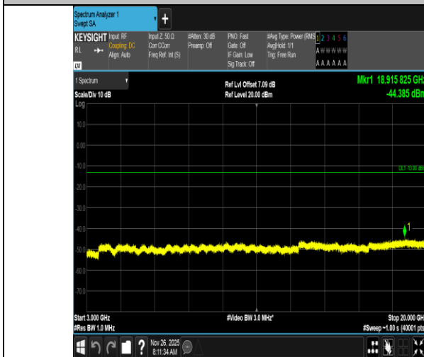
Band4-1.4MHz-QPSK-20175-1RB#0-3000~20000-PASS
