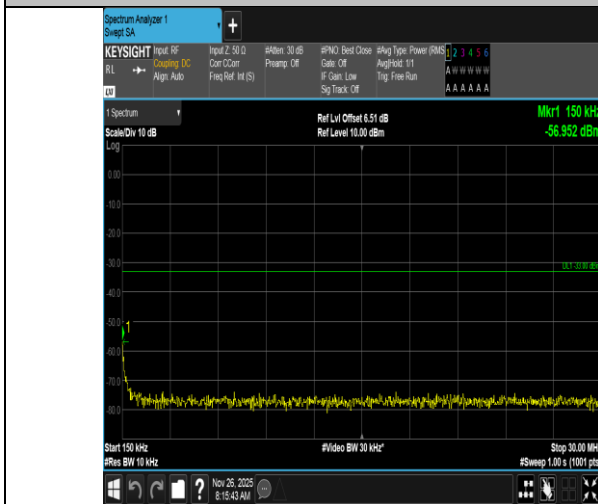
Band4-1.4MHz-16QAM-20175-6RB#0-0.15~30-PASS
