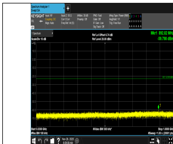
Band4-1.4MHz-QPSK-19957-6RB#0-30~1000-PASS
