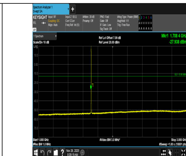
Band4-1.4MHz-QPSK-19957-6RB#0-1000~3000-PASS
