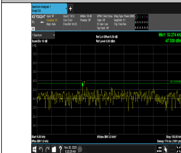
Band4-1.4MHz-QPSK-20393-6RB#0-0.009~0.15-PASS
