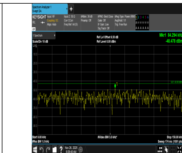
Band4-1.4MHz-16QAM-19957-6RB#0-0.009~0.15-PASS
