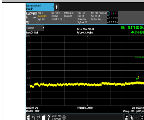
Band4-1.4MHz-QPSK-19957-6RB#0-3000~20000-PASS
