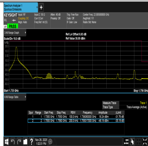
Band4-20MHz-16QAM-20300-1RB#0-PASS
