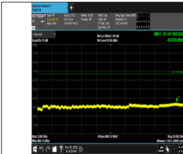
Band4-1.4MHz-16QAM-20175-1RB#5-3000~20000-PASS
