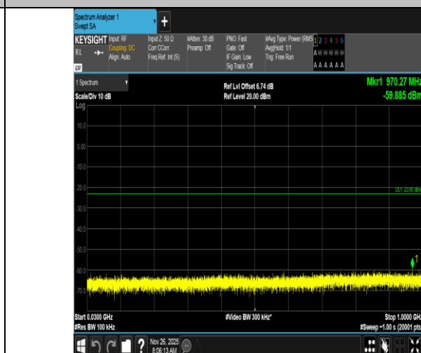
Band4-1.4MHz-16QAM-19957-1RB#0-30~1000-PASS
