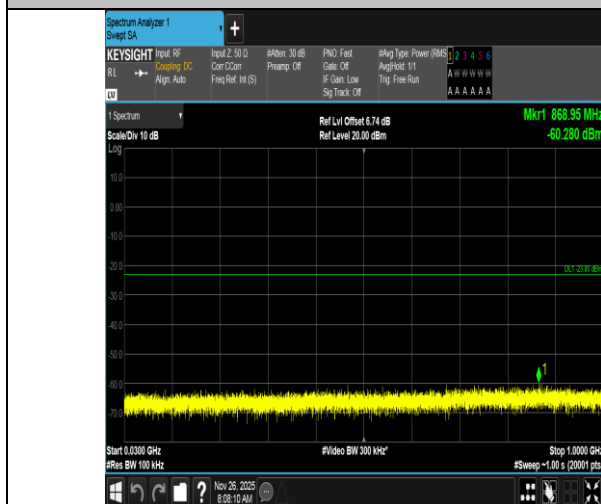
Band4-1.4MHz-16QAM-19957-1RB#5-30~1000-PASS
