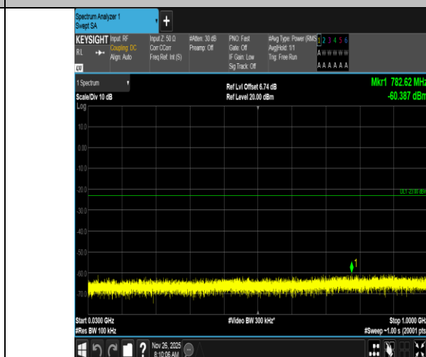
Band4-1.4MHz-16QAM-19957-6RB#0-30~1000-PASS
