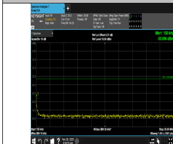
Band4-1.4MHz-16QAM-19957-6RB#0-0.15~30-PASS
