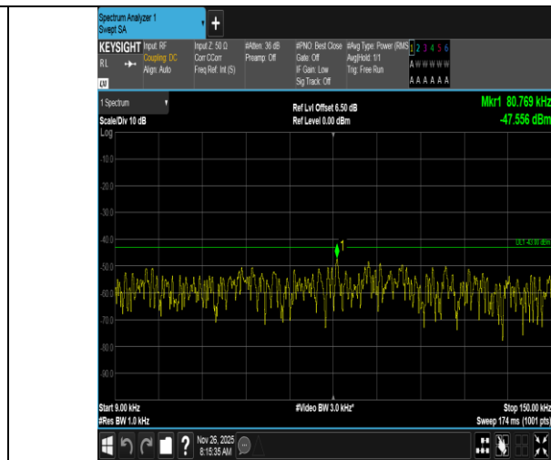
Band4-1.4MHz-16QAM-20175-6RB#0-0.009~0.15-PASS
