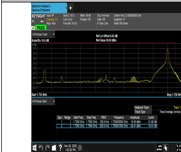
Band4-20MHz-16QAM-20300-1RB#99-PASS
