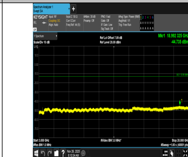
Band4-1.4MHz-16QAM-19957-6RB#0-3000~20000-PASS
