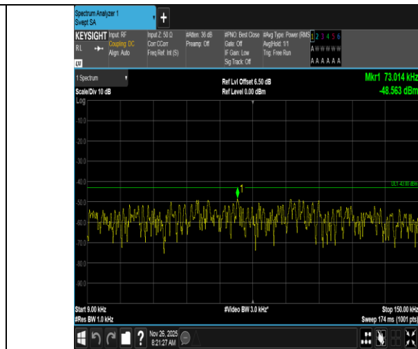
Band4-1.4MHz-16QAM-20393-6RB#0-0.009~0.15-PASS
