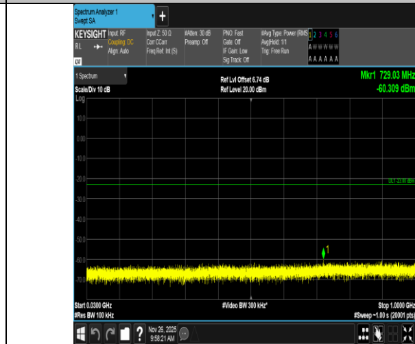
Band4-3MHz-16QAM-20175-15RB#0-30~1000-PASS
