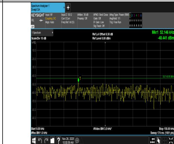
Band4-3MHz-QPSK-20385-1RB#14-0.009~0.15-PASS
