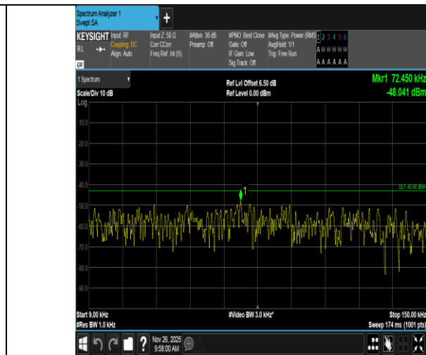
Band4-3MHz-16QAM-20175-15RB#0-0.009~0.15-PASS
