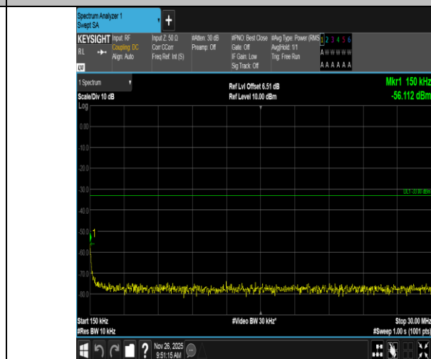
Band4-3MHz-QPSK-19965-15RB#0-0.15~30-PASS
