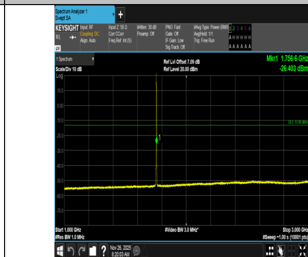
Band4-1.4MHz-16QAM-20393-1RB#5-1000~3000-PASS
