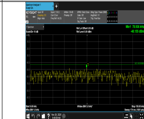
Band4-3MHz-QPSK-19965-1RB#14-0.009~0.15-PASS
