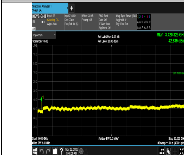
Band4-3MHz-QPSK-19965-1RB#0-3000~20000-PASS
