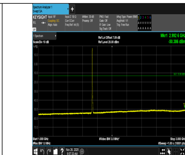
Band4-3MHz-QPSK-20175-15RB#0-1000~3000-PASS
