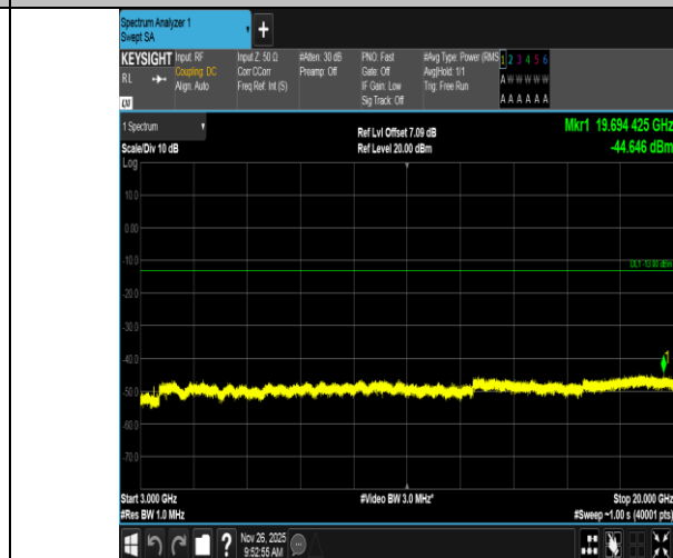
Band4-3MHz-16QAM-19965-15RB#0-3000~20000-PASS
