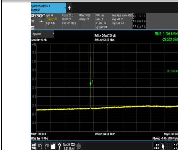
Band4-1.4MHz-16QAM-20393-6RB#0-1000~3000-PASS
