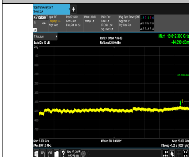
Band4-3MHz-QPSK-20175-15RB#0-3000~20000-PASS
