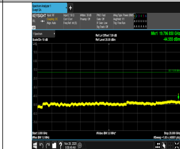
Band4-3MHz-16QAM-20175-15RB#0-3000~20000-PASS
