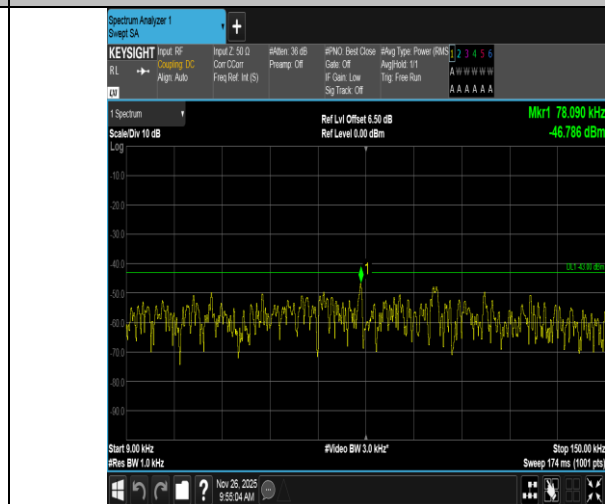
Band4-3MHz-QPSK-20175-1RB#14-0.009~0.15-PASS
