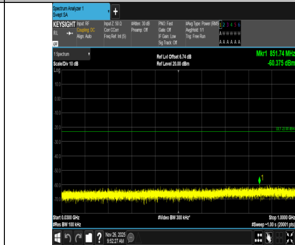
Band4-3MHz-16QAM-19965-15RB#0-30~1000-PASS
