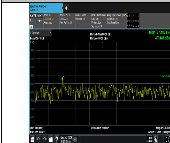
Band4-3MHz-QPSK-20175-15RB#0-0.009~0.15-PASS
