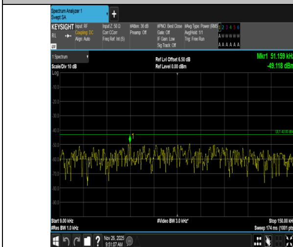
Band4-3MHz-QPSK-19965-15RB#0-0.009~0.15-PASS
