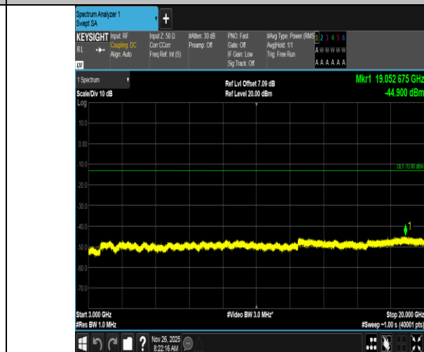
Band4-1.4MHz-16QAM-20393-6RB#0-3000~20000-PASS
