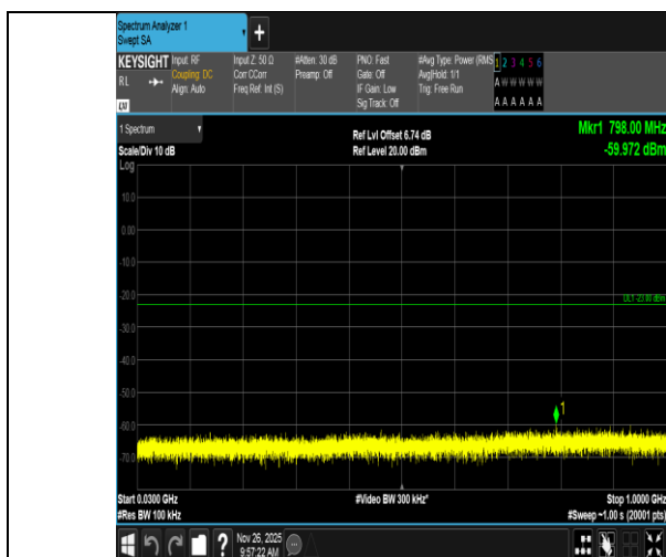
Band4-3MHz-QPSK-20175-15RB#0-30~1000-PASS
