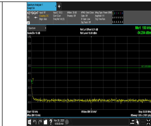
Band4-3MHz-QPSK-20385-1RB#0-0.15~30-PASS
