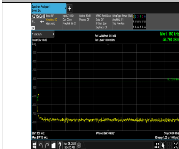
Band4-3MHz-16QAM-20175-1RB#0-0.15~30-PASS
