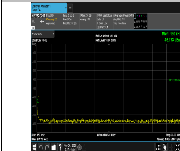
Band4-1.4MHz-16QAM-20393-1RB#0-0.15~30-PASS
