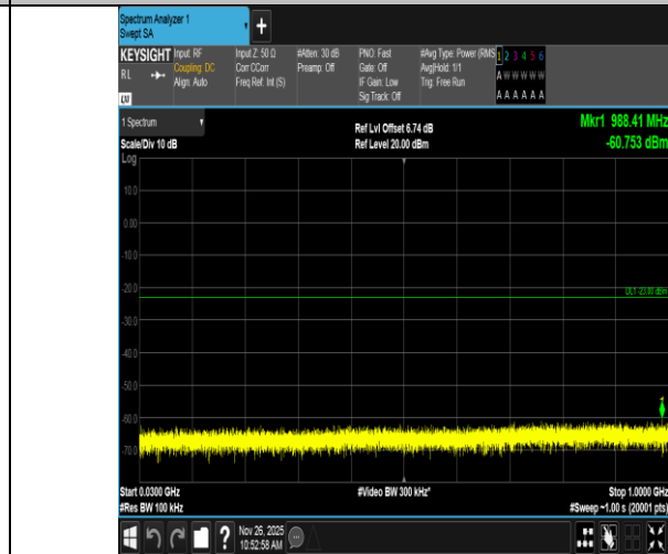
Band4-5MHz-16QAM-20175-25RB#0-30~1000-PASS
