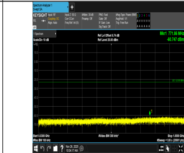
Band4-3MHz-16QAM-20385-15RB#0-30~1000-PASS
