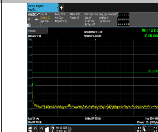
Band4-3MHz-16QAM-20385-1RB#14-0.15~30-PASS
