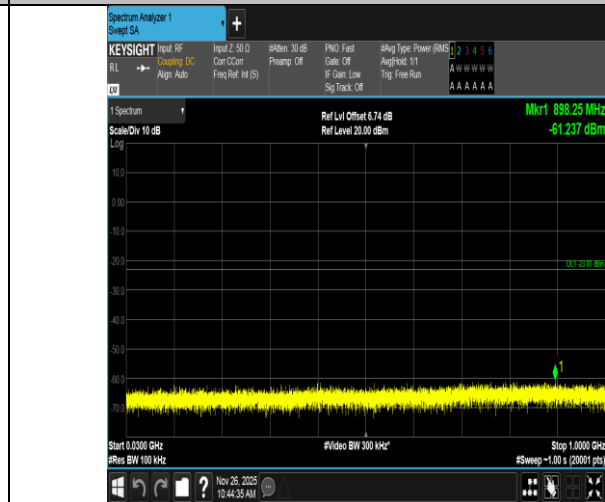
Band4-5MHz-16QAM-19975-25RB#0-30~1000-PASS
