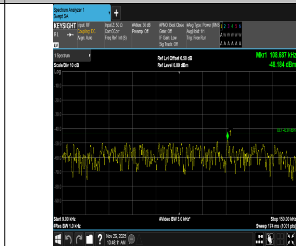
Band4-5MHz-QPSK-20175-1RB#24-0.009~0.15-PASS
