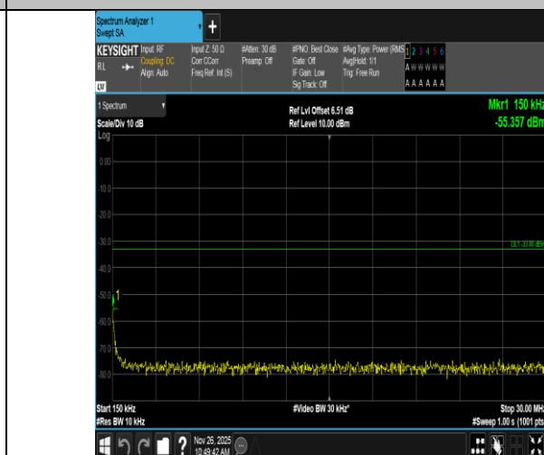
Band4-5MHz-16QAM-20175-1RB#24-0.15~30-PASS
