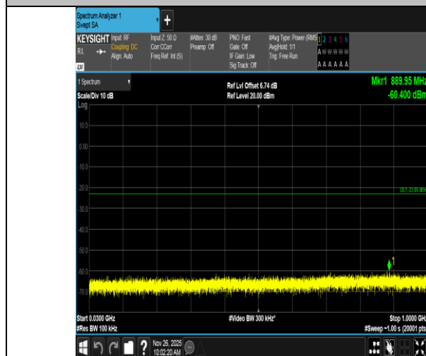
Band4-3MHz-16QAM-20385-1RB#14-30~1000-PASS
