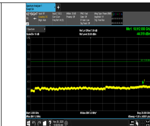
Band4-3MHz-16QAM-20385-1RB#0-3000~20000-PASS
