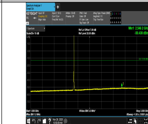
Band4-5MHz-16QAM-20175-1RB#24-1000~3000-PASS
