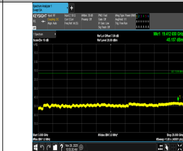
Band4-5MHz-16QAM-20175-25RB#0-3000~20000-PASS
