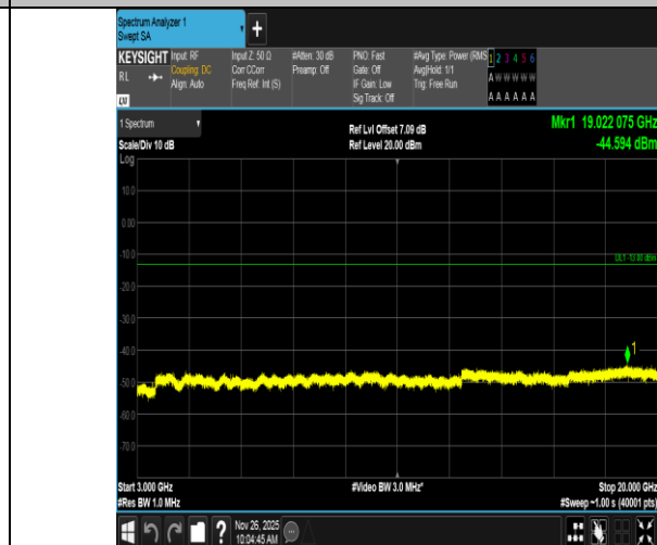
Band4-3MHz-16QAM-20385-15RB#0-3000~20000-PASS
