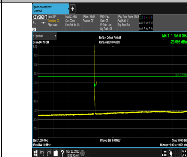
Band4-3MHz-16QAM-20385-1RB#14-1000~3000-PASS
