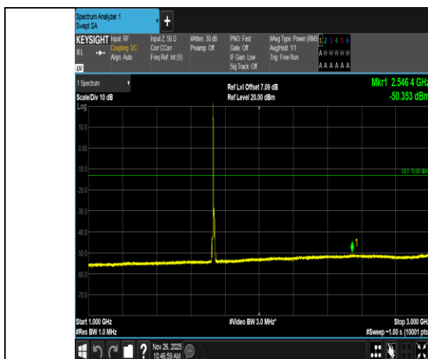
Band4-5MHz-16QAM-20175-1RB#0-1000~3000-PASS
