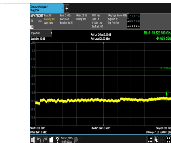
Band4-5MHz-16QAM-20175-1RB#0-3000~20000-PASS
