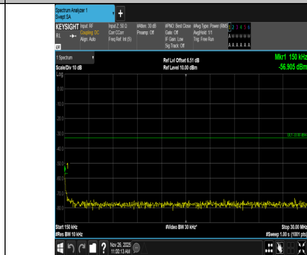
Band4-5MHz-QPSK-20375-25RB#0-0.15~30-PASS
