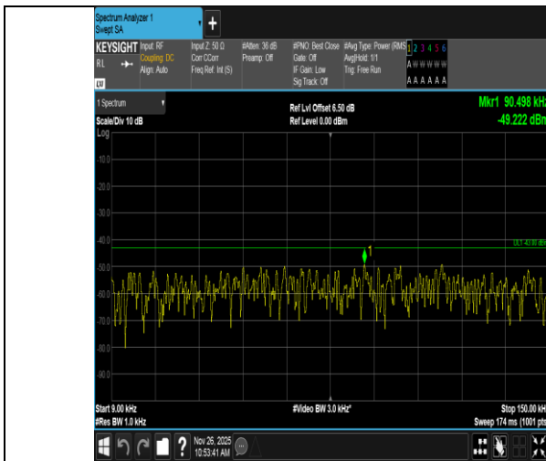
Band4-5MHz-QPSK-20375-1RB#0-0.009~0.15-PASS
