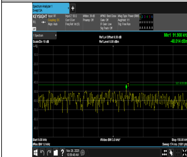
Band4-5MHz-QPSK-20375-25RB#0-0.009~0.15-PASS
