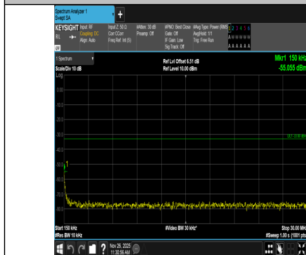
Band4-10MHz-16QAM-20000-1RB#0-0.15~30-PASS
