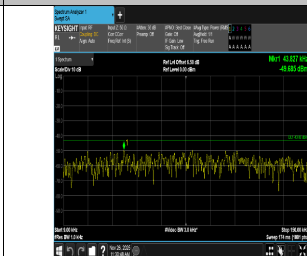
Band4-10MHz-16QAM-20000-1RB#0-0.009~0.15-PASS
