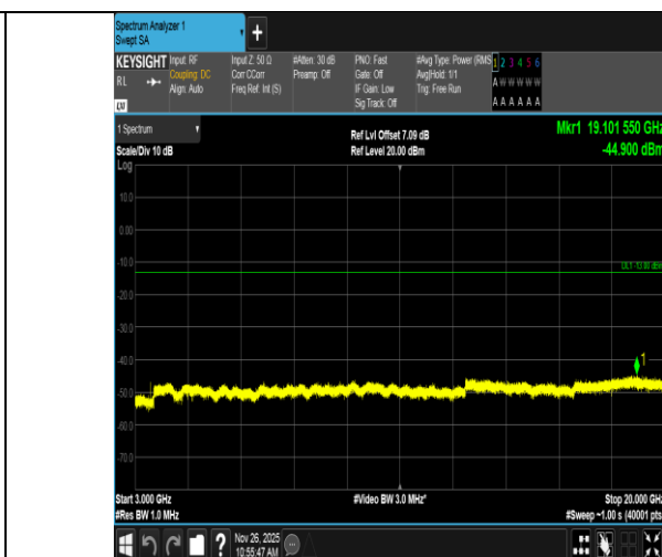
Band4-5MHz-16QAM-20375-1RB#0-3000~20000-PASS
