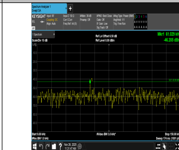
Band4-10MHz-QPSK-20000-1RB#49-0.009~0.15-PASS
