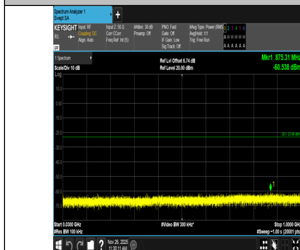
Band4-10MHz-QPSK-20000-1RB#0-30~1000-PASS
