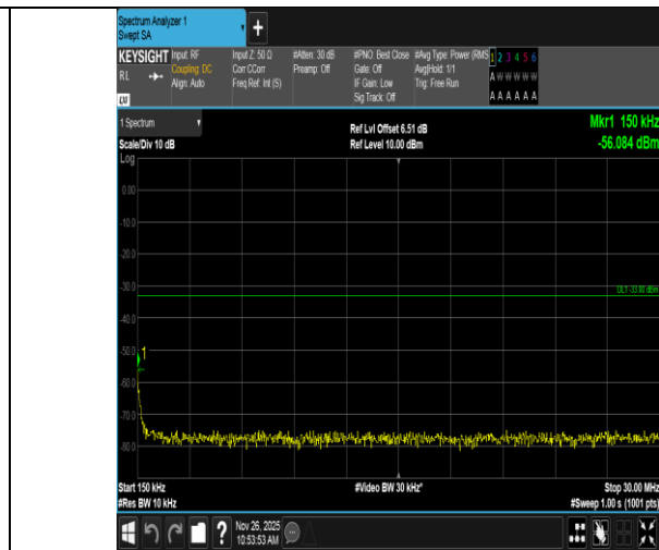
Band4-5MHz-QPSK-20375-1RB#0-0.15~30-PASS
