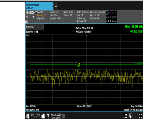
Band4-5MHz-QPSK-20375-1RB#24-0.009~0.15-PASS
