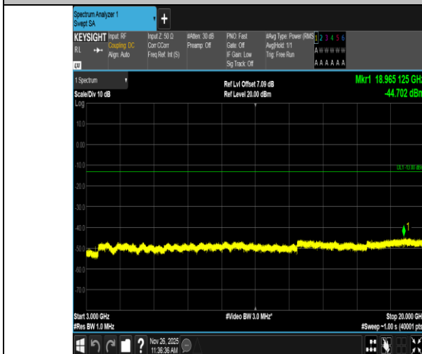
Band4-10MHz-QPSK-20175-1RB#0-3000~20000-PASS
