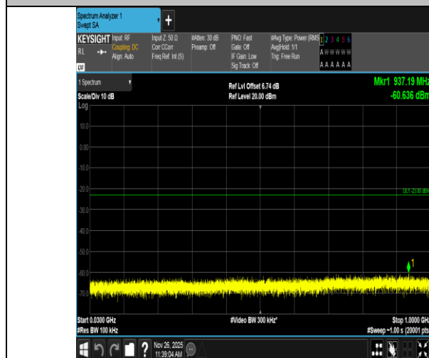
Band4-10MHz-16QAM-20175-1RB#49-30~1000-PASS
