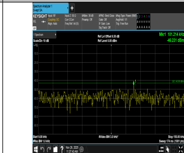
Band4-10MHz-QPSK-20175-1RB#49-0.009~0.15-PASS
