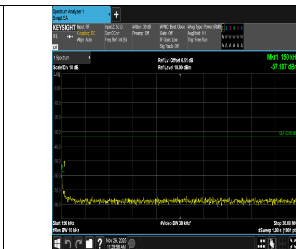
Band4-10MHz-QPSK-20000-1RB#0-0.15~30-PASS
