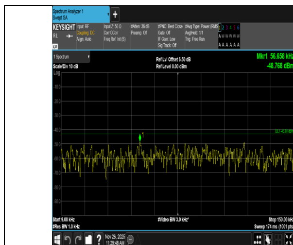
Band4-10MHz-QPSK-20000-1RB#0-0.009~0.15-PASS
