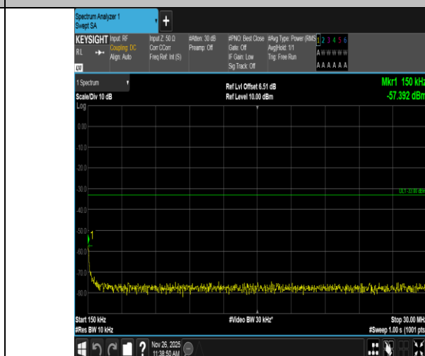
Band4-10MHz-16QAM-20175-1RB#49-0.15~30-PASS
