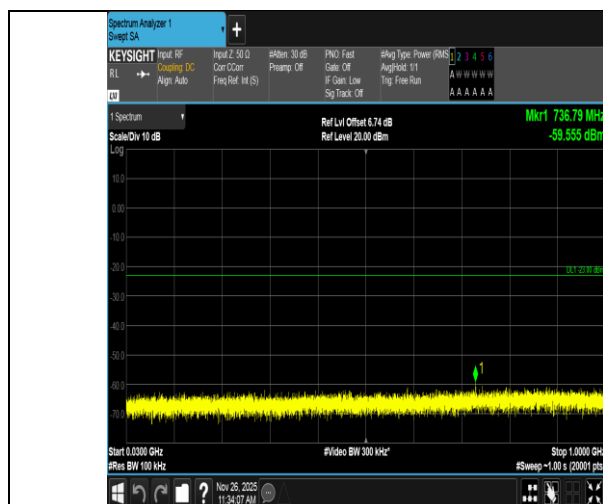
Band4-10MHz-QPSK-20000-50RB#0-30~1000-PASS
