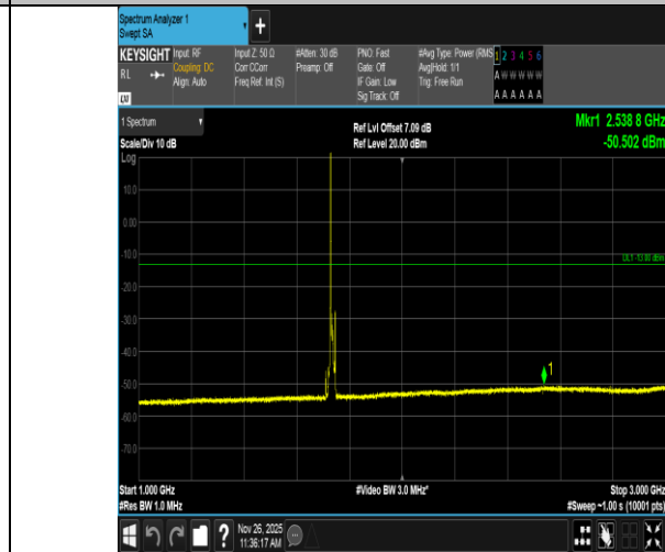
Band4-10MHz-QPSK-20175-1RB#0-1000~3000-PASS
