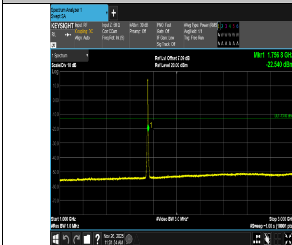
Band4-5MHz-16QAM-20375-25RB#0-1000~3000-PASS
