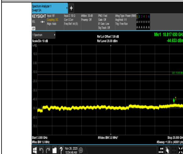
Band4-5MHz-QPSK-20375-1RB#0-3000~20000-PASS
