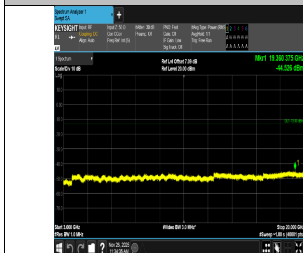
Band4-10MHz-QPSK-20000-50RB#0-3000~20000-PASS
