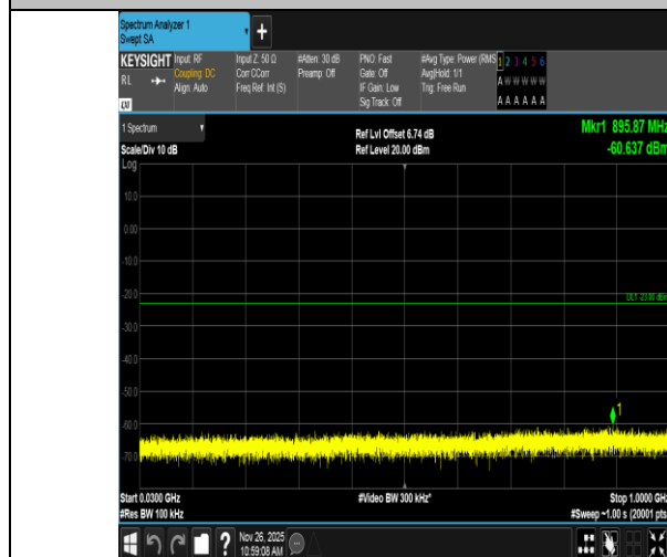
Band4-5MHz-16QAM-20375-1RB#24-30~1000-PASS
