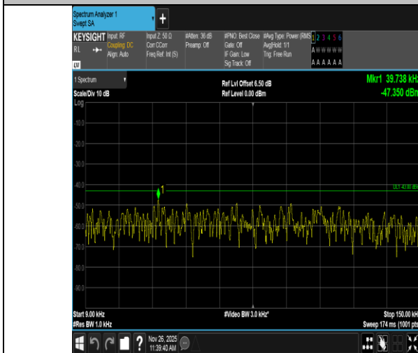
Band4-10MHz-QPSK-20175-50RB#0-0.009~0.15-PASS
