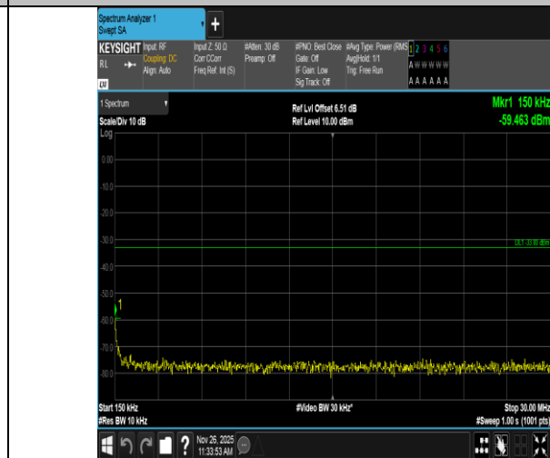
Band4-10MHz-QPSK-20000-50RB#0-0.15~30-PASS
