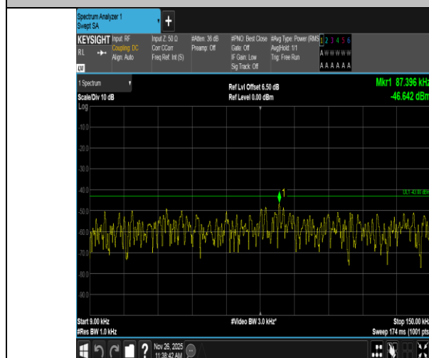
Band4-10MHz-16QAM-20175-1RB#49-0.009~0.15-PASS
