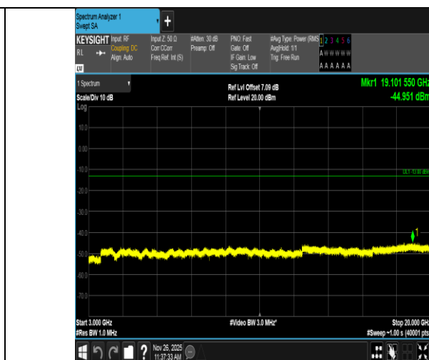
Band4-10MHz-16QAM-20175-1RB#0-3000~20000-PASS
