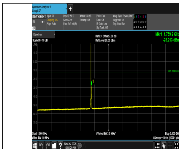
Band4-5MHz-16QAM-20375-1RB#0-1000~3000-PASS
