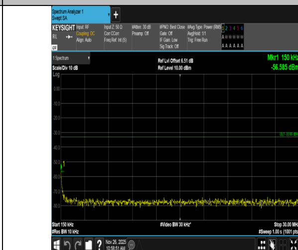
Band4-5MHz-16QAM-20375-1RB#24-0.15~30-PASS
