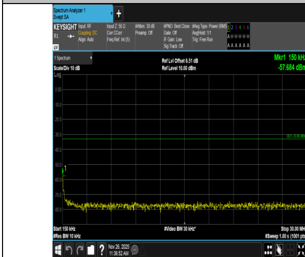
Band4-10MHz-16QAM-20175-1RB#0-0.15~30-PASS
