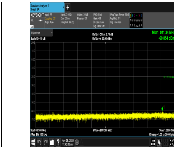
Band4-10MHz-QPSK-20175-50RB#0-30~1000-PASS
