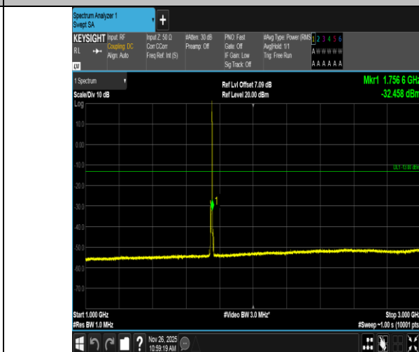
Band4-5MHz-16QAM-20375-1RB#24-1000~3000-PASS
