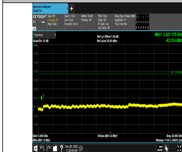
Band4-10MHz-QPSK-20000-1RB#0-3000~20000-PASS
