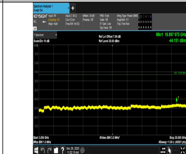
Band4-5MHz-16QAM-20375-25RB#0-3000~20000-PASS
