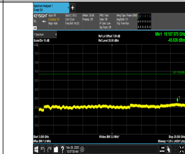
Band4-5MHz-QPSK-20375-1RB#24-3000~20000-PASS
