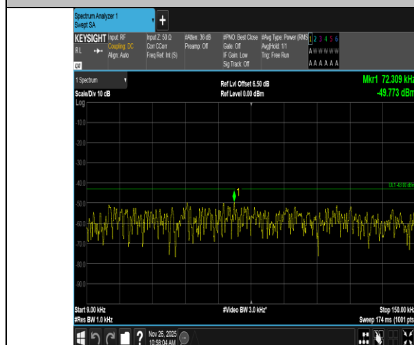
Band4-5MHz-16QAM-20375-1RB#24-0.009~0.15-PASS
