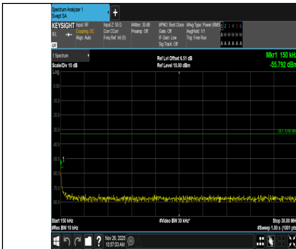
Band4-5MHz-QPSK-20375-1RB#24-0.15~30-PASS
