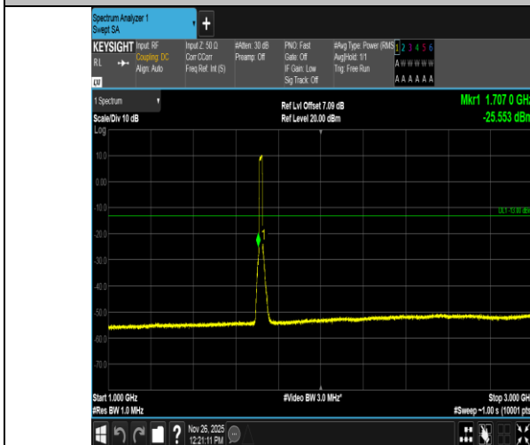
Band4-15MHz-16QAM-20025-75RB#0-1000~3000-PASS
