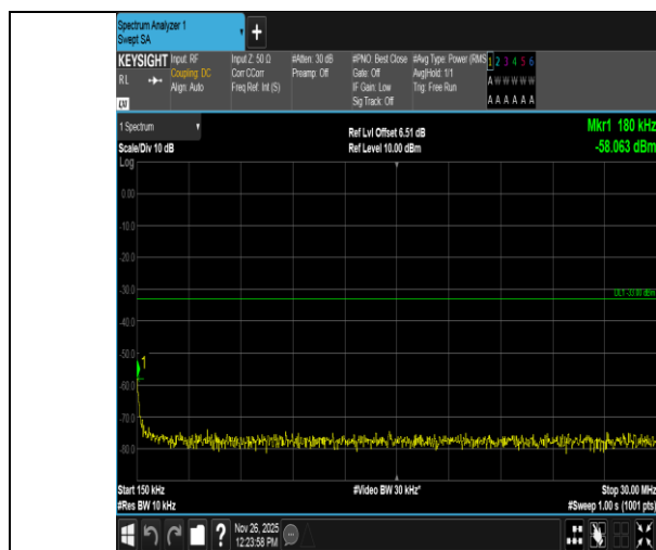
Band4-15MHz-QPSK-20175-1RB#74-0.15~30-PASS
