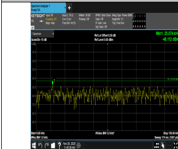
Band4-10MHz-QPSK-20350-50RB#0-0.009~0.15-PASS
