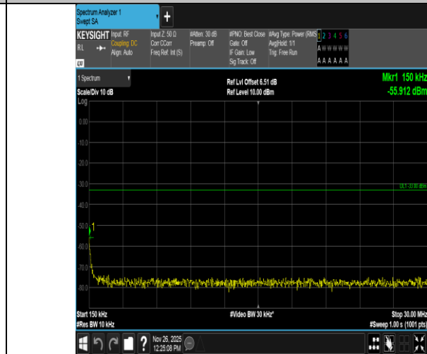
Band4-15MHz-16QAM-20175-1RB#74-0.15~30-PASS
