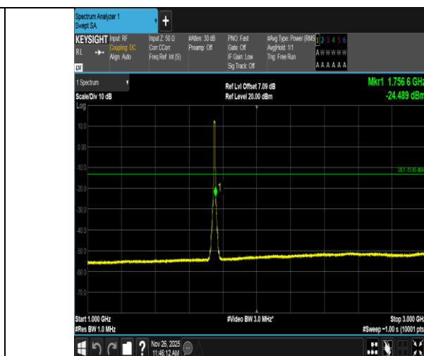
Band4-10MHz-QPSK-20350-50RB#0-1000~3000-PASS
