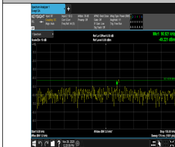
Band4-15MHz-QPSK-20175-75RB#0-0.009~0.15-PASS
