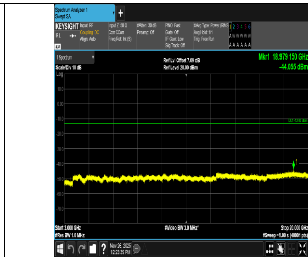
Band4-15MHz-16QAM-20175-1RB#0-3000~20000-PASS
