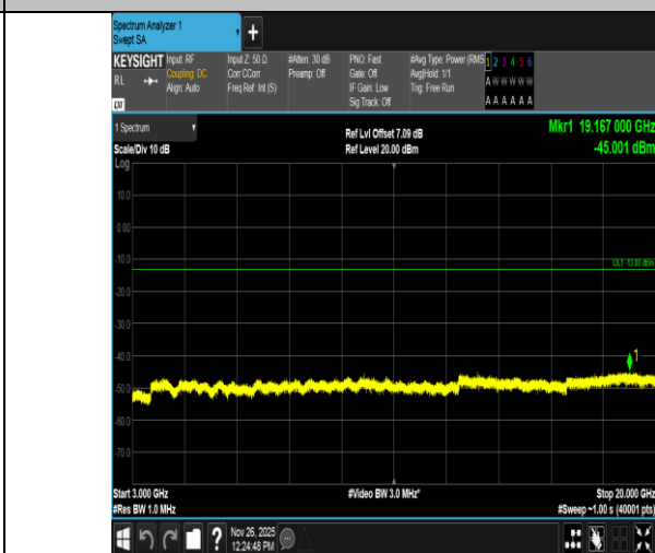
Band4-15MHz-QPSK-20175-1RB#74-3000~20000-PASS
