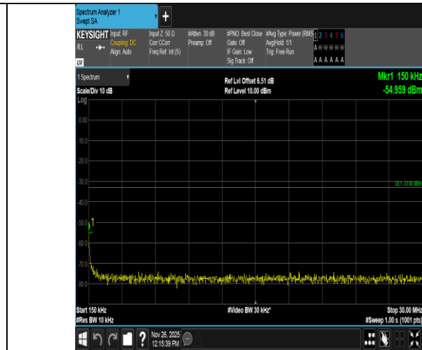
Band4-15MHz-QPSK-20025-1RB#0-0.15~30-PASS
