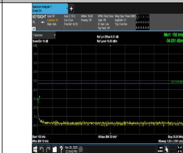
Band4-15MHz-QPSK-20025-75RB#0-0.15~30-PASS
