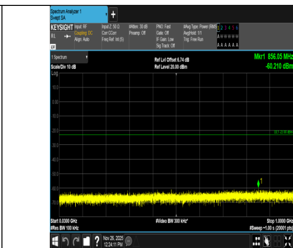
Band4-15MHz-QPSK-20175-1RB#74-30~1000-PASS
