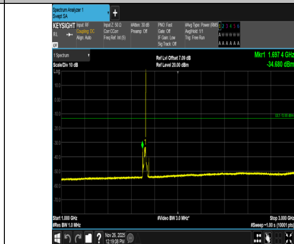
Band4-15MHz-16QAM-20025-1RB#74-1000~3000-PASS
