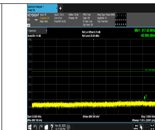
Band4-15MHz-QPSK-20025-1RB#74-30~1000-PASS
