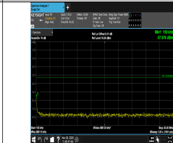
Band4-10MHz-QPSK-20350-50RB#0-0.15~30-PASS
