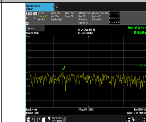
Band4-15MHz-16QAM-20175-1RB#0-0.009~0.15-PASS
