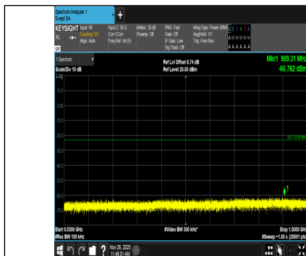
Band4-10MHz-QPSK-20350-50RB#0-30~1000-PASS
