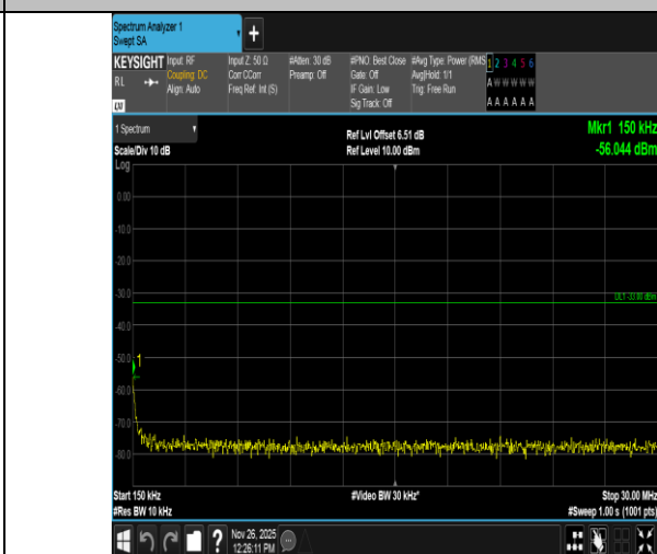
Band4-15MHz-QPSK-20175-75RB#0-0.15~30-PASS
