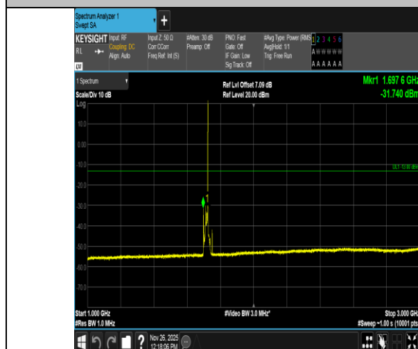
Band4-15MHz-QPSK-20025-1RB#74-1000~3000-PASS
