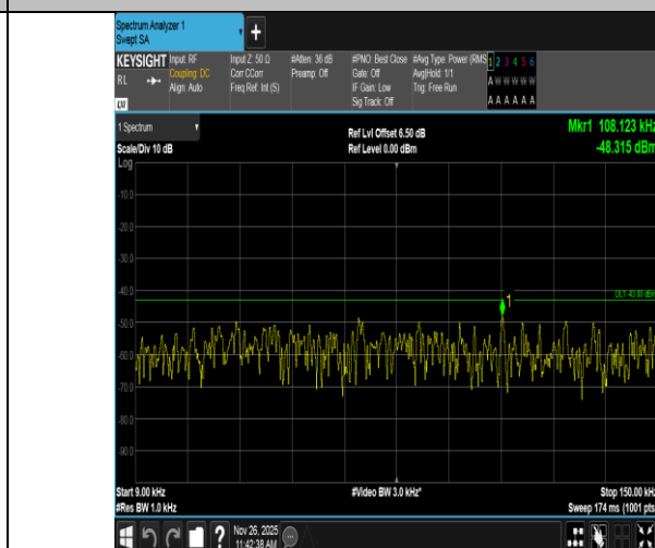
Band4-10MHz-16QAM-20350-1RB#0-0.009~0.15-PASS
