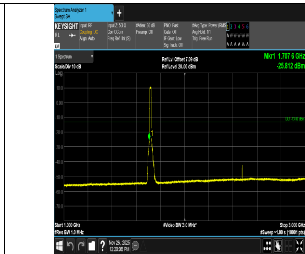
Band4-15MHz-QPSK-20025-75RB#0-1000~3000-PASS
