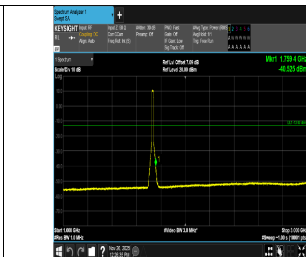
Band4-15MHz-QPSK-20175-75RB#0-1000~3000-PASS
