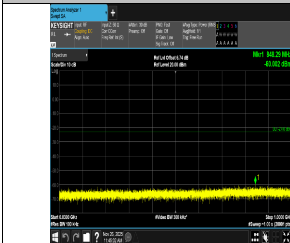
Band4-10MHz-16QAM-20350-1RB#49-30~1000-PASS
