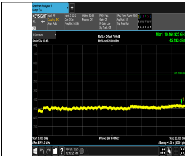
Band4-15MHz-16QAM-20025-1RB#74-3000~20000-PASS
