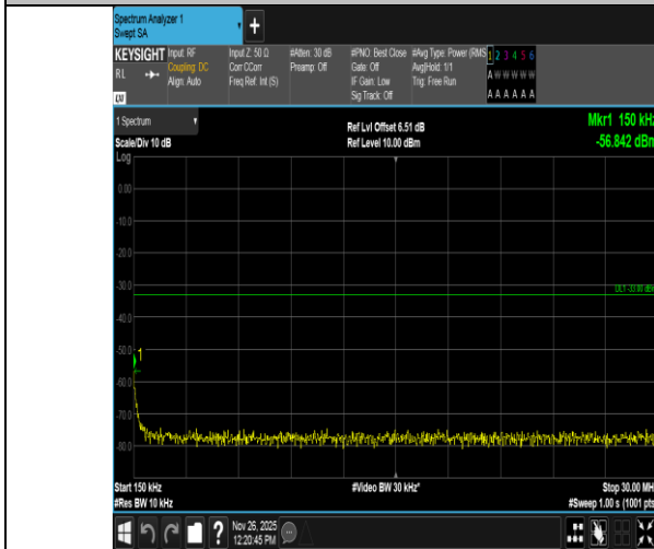
Band4-15MHz-16QAM-20025-75RB#0-0.15~30-PASS
