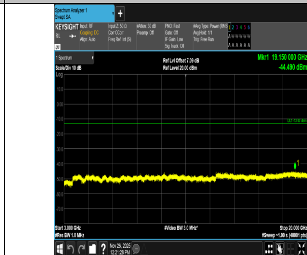
Band4-15MHz-16QAM-20025-75RB#0-3000~20000-PASS
