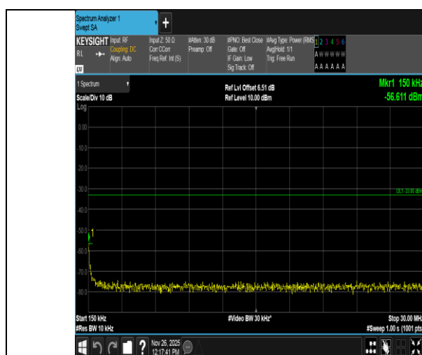
Band4-15MHz-QPSK-20025-1RB#74-0.15~30-PASS
