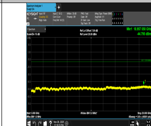
Band4-15MHz-QPSK-20025-1RB#74-3000~20000-PASS
