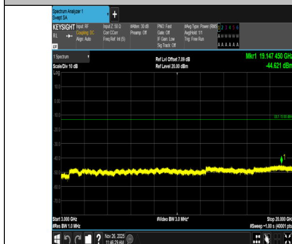
Band4-10MHz-QPSK-20350-50RB#0-3000~20000-PASS
