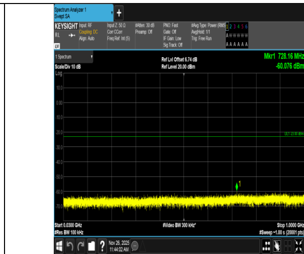
Band4-10MHz-QPSK-20350-1RB#49-30~1000-PASS
