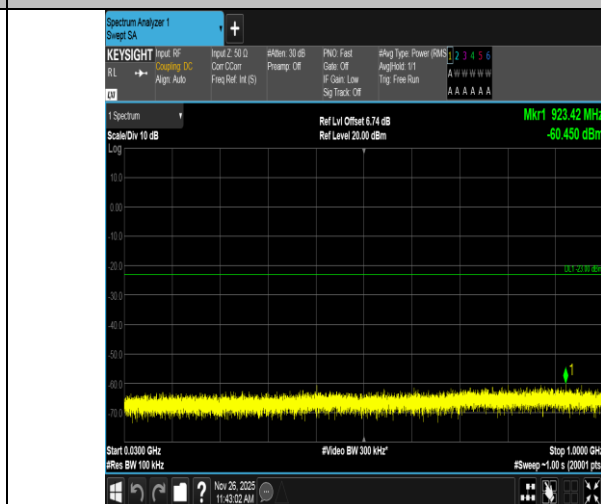
Band4-10MHz-16QAM-20350-1RB#0-30~1000-PASS
