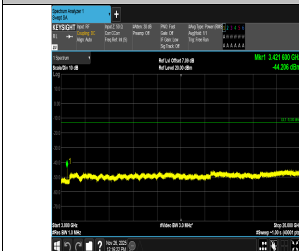
Band4-15MHz-QPSK-20025-1RB#0-3000~20000-PASS
