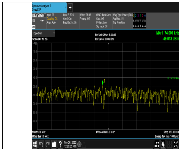
Band4-15MHz-16QAM-20025-75RB#0-0.009~0.15-PASS
