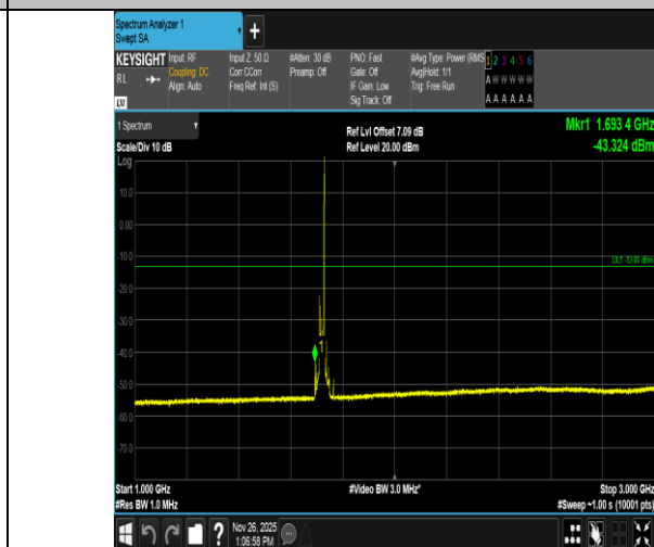
Band4-20MHz-16QAM-20050-1RB#99-1000~3000-PASS
