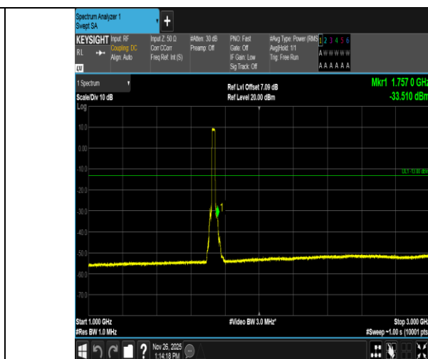
Band4-20MHz-QPSK-20175-100RB#0-1000~3000-PASS
