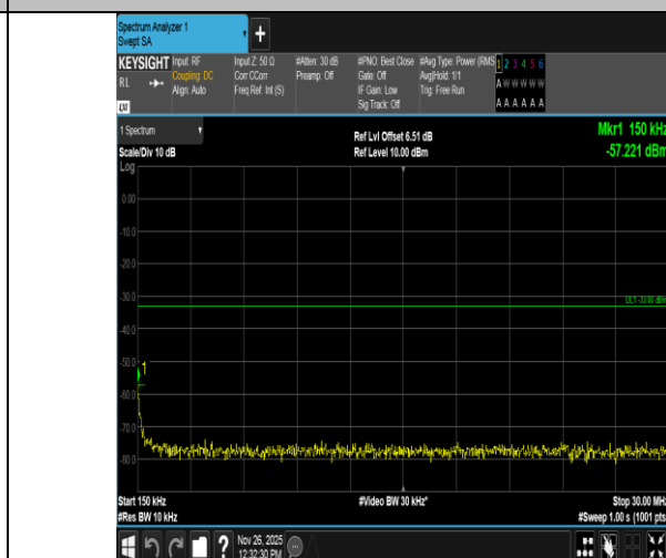
Band4-15MHz-QPSK-20325-75RB#0-0.15~30-PASS
