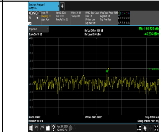
Band4-15MHz-16QAM-20325-1RB#0-0.009~0.15-PASS
