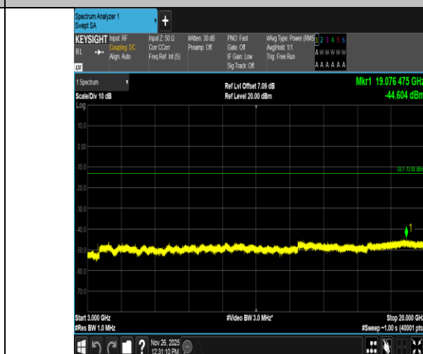
Band4-15MHz-QPSK-20325-1RB#74-3000~20000-PASS
