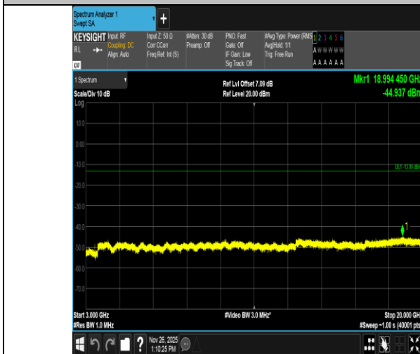
Band4-20MHz-QPSK-20175-1RB#0-3000~20000-PASS
