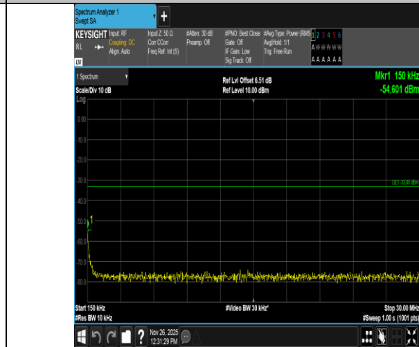
Band4-15MHz-16QAM-20325-1RB#74-0.15~30-PASS
