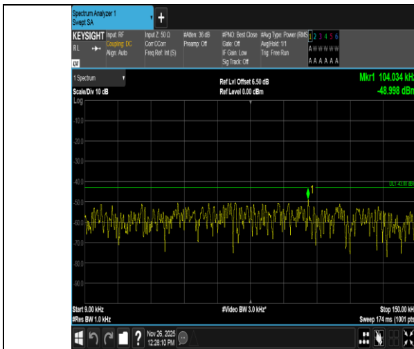
Band4-15MHz-QPSK-20325-1RB#0-0.009~0.15-PASS
