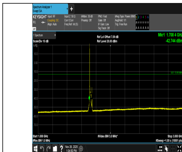
Band4-20MHz-16QAM-20050-1RB#0-1000~3000-PASS
