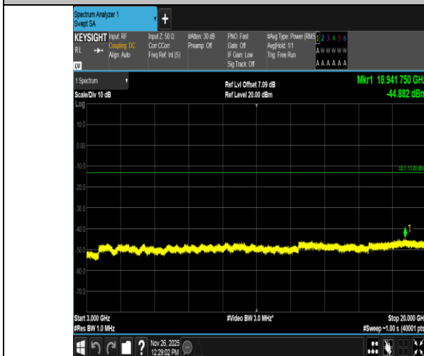
Band4-15MHz-QPSK-20325-1RB#0-3000~20000-PASS
