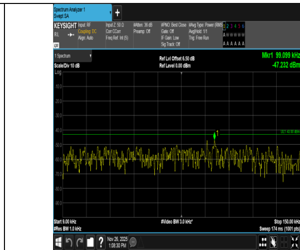
Band4-20MHz-16QAM-20050-100RB#0-0.009~0.15-PASS
