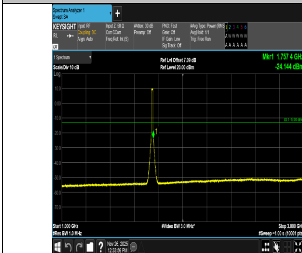
Band4-15MHz-16QAM-20325-75RB#0-1000~3000-PASS
