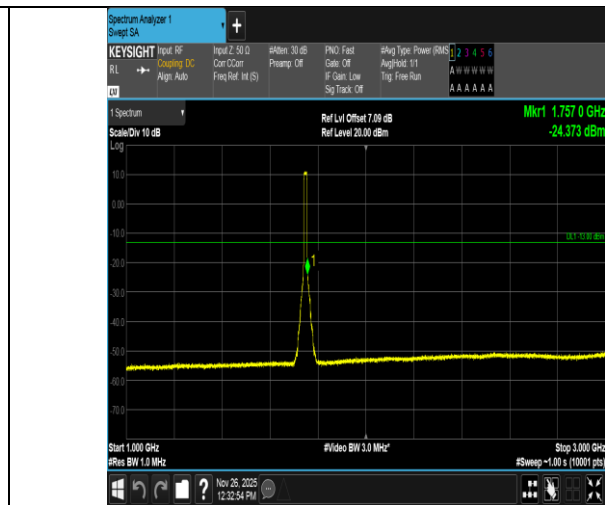
Band4-15MHz-QPSK-20325-75RB#0-1000~3000-PASS
