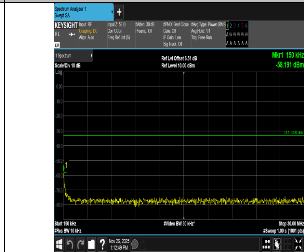
Band4-20MHz-16QAM-20175-1RB#99-0.15~30-PASS
