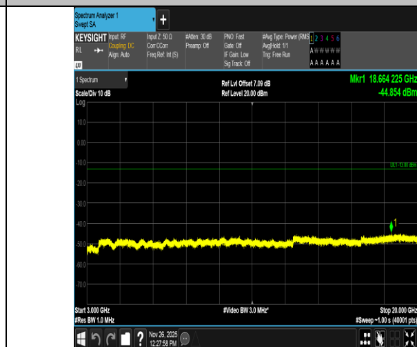
Band4-15MHz-16QAM-20175-75RB#0-3000~20000-PASS
