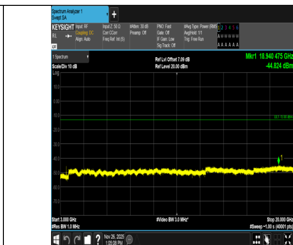
Band4-20MHz-16QAM-20050-1RB#0-3000~20000-PASS
