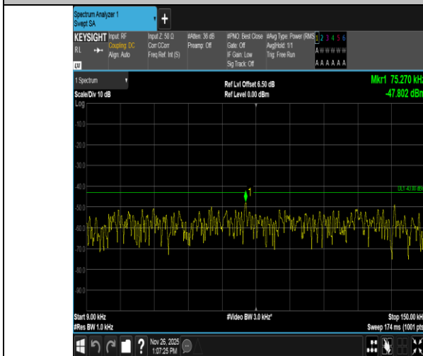
Band4-20MHz-QPSK-20050-100RB#0-0.009~0.15-PASS
