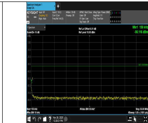
Band4-15MHz-QPSK-20325-1RB#0-0.15~30-PASS
