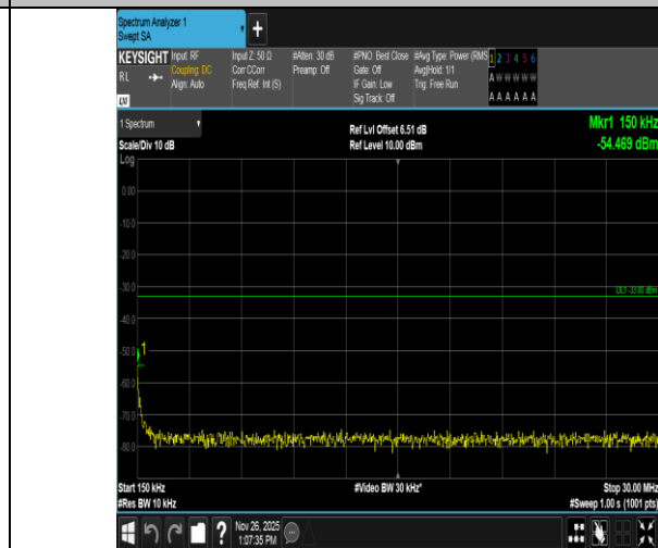
Band4-20MHz-QPSK-20050-100RB#0-0.15~30-PASS
