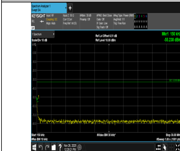
Band4-15MHz-16QAM-20325-1RB#0-0.15~30-PASS
