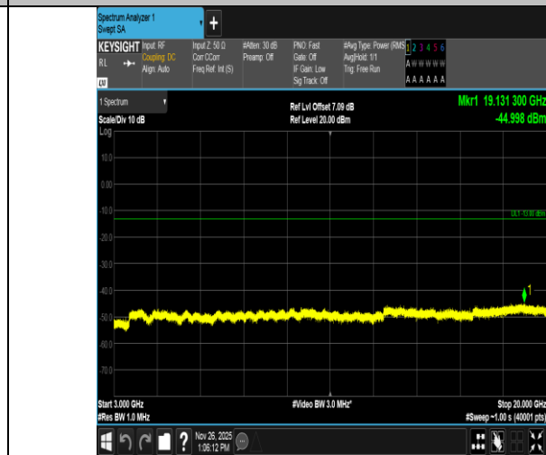
Band4-20MHz-QPSK-20050-1RB#99-3000~20000-PASS
