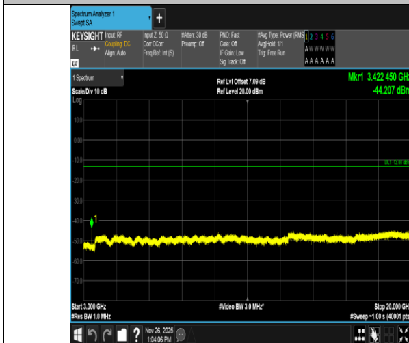
Band4-20MHz-QPSK-20050-1RB#0-3000~20000-PASS
