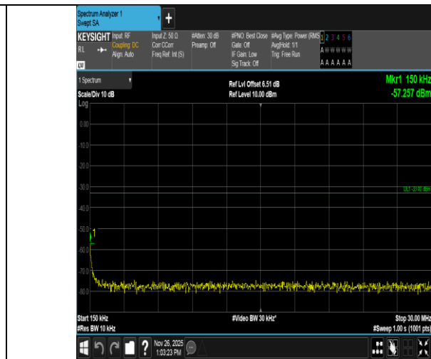
Band4-20MHz-QPSK-20050-1RB#0-0.15~30-PASS
