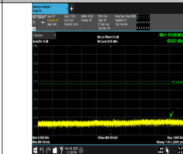
Band4-20MHz-16QAM-20175-1RB#0-30~1000-PASS
