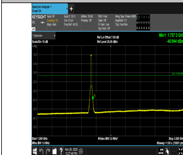
Band4-15MHz-16QAM-20175-75RB#0-1000~3000-PASS
