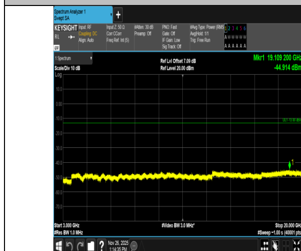
Band4-20MHz-QPSK-20175-100RB#0-3000~20000-PASS
