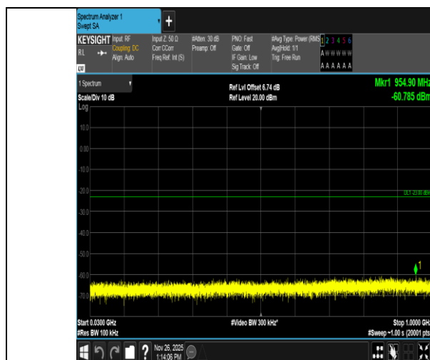
Band4-20MHz-QPSK-20175-100RB#0-30~1000-PASS
