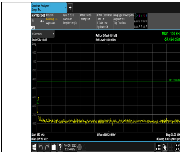
Band4-20MHz-QPSK-20175-1RB#99-0.15~30-PASS
