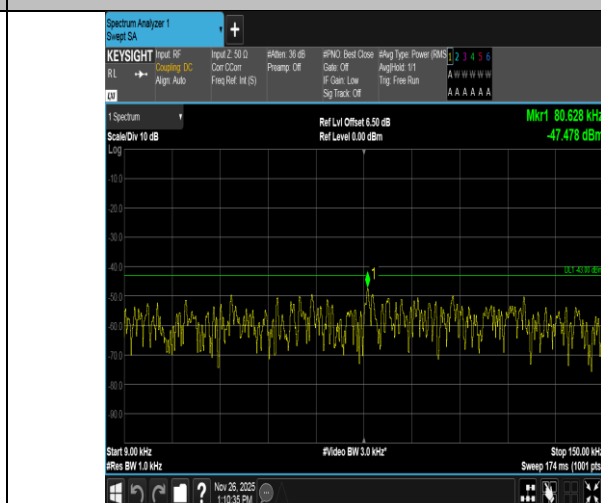
Band4-20MHz-16QAM-20175-1RB#0-0.009~0.15-PASS
