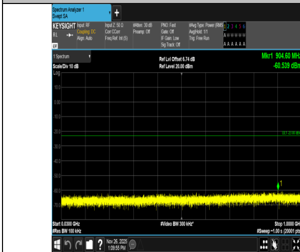
Band4-20MHz-QPSK-20175-1RB#0-30~1000-PASS
