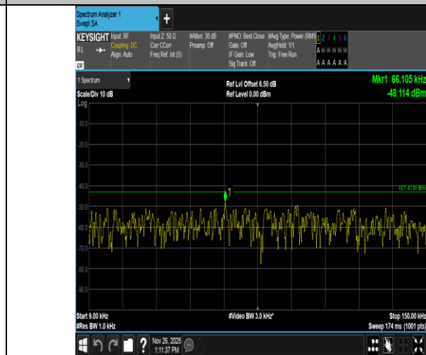
Band4-20MHz-QPSK-20175-1RB#99-0.009~0.15-PASS
