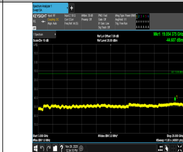
Band4-15MHz-16QAM-20325-75RB#0-3000~20000-PASS
