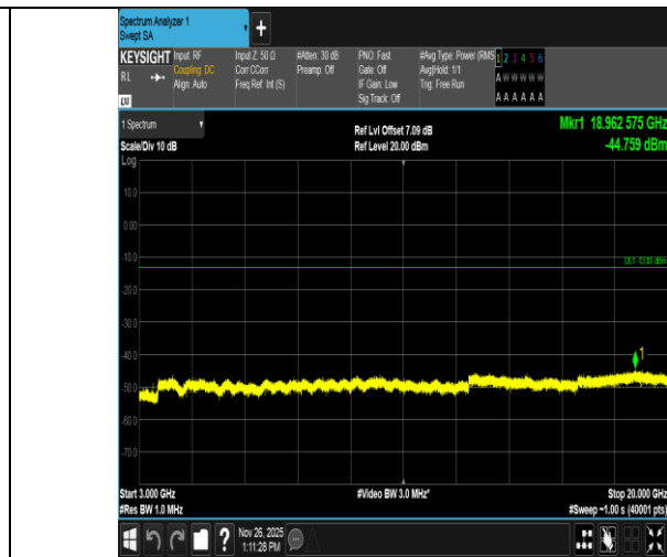
Band4-20MHz-16QAM-20175-1RB#0-3000~20000-PASS
