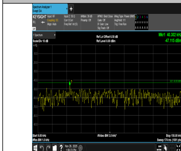
Band4-20MHz-16QAM-20050-1RB#99-0.009~0.15-PASS
