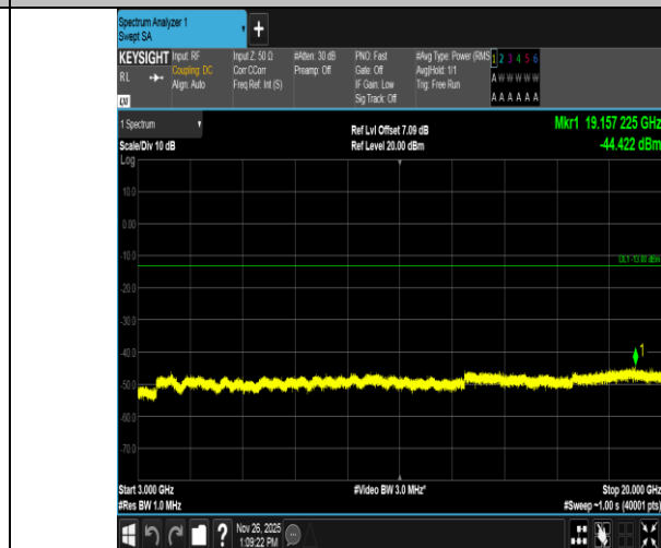
Band4-20MHz-16QAM-20050-100RB#0-3000~20000-PASS
