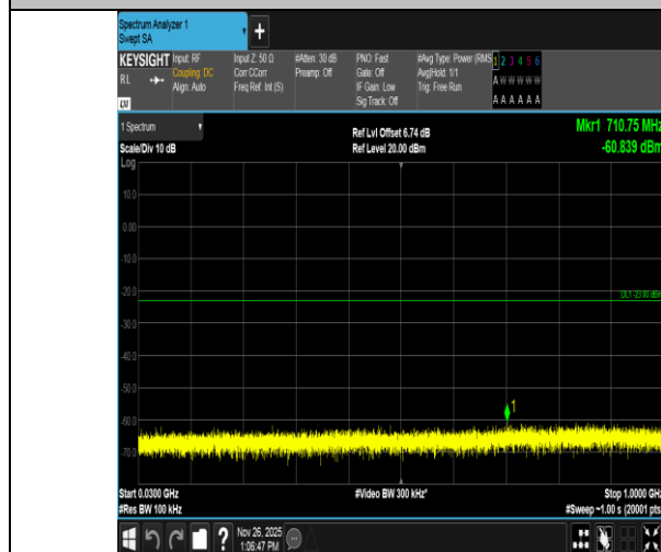
Band4-20MHz-16QAM-20050-1RB#99-30~1000-PASS
