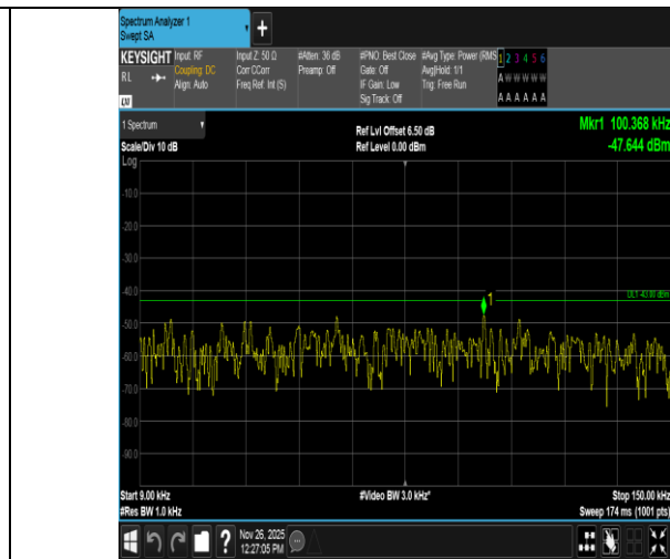
Band4-15MHz-16QAM-20175-75RB#0-0.009~0.15-PASS
