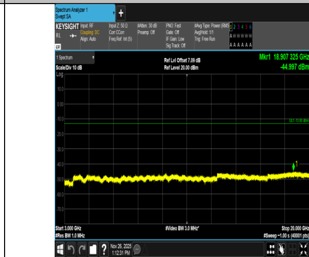
Band4-20MHz-QPSK-20175-1RB#99-3000~20000-PASS
