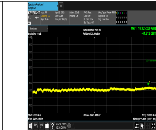
Band4-15MHz-16QAM-20325-1RB#0-3000~20000-PASS
