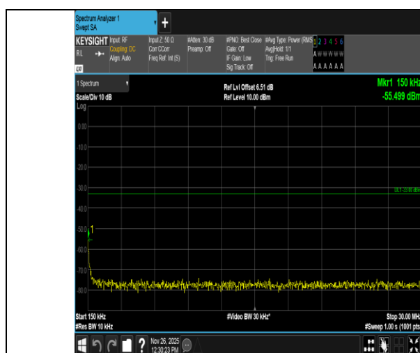
Band4-15MHz-QPSK-20325-1RB#74-0.15~30-PASS
