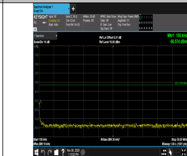
Band4-20MHz-QPSK-20175-100RB#0-0.15~30-PASS
