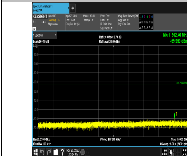
Band4-20MHz-16QAM-20175-1RB#99-30~1000-PASS
