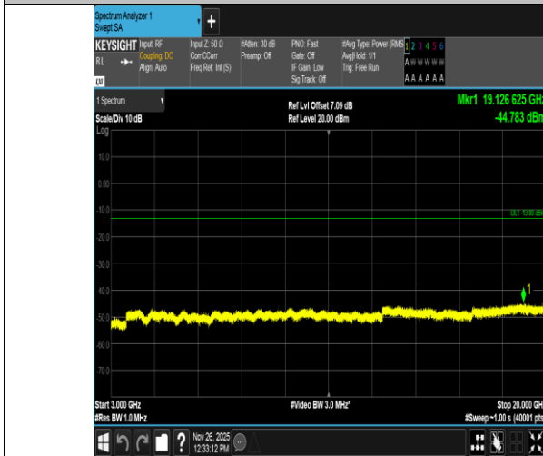
Band4-15MHz-QPSK-20325-75RB#0-3000~20000-PASS
