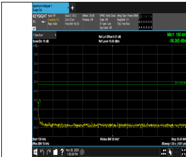
Band4-20MHz-QPSK-20050-1RB#99-0.15~30-PASS
