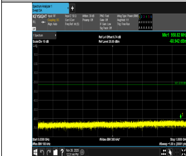
Band4-15MHz-16QAM-20325-1RB#74-30~1000-PASS
