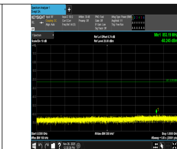
Band4-15MHz-QPSK-20325-1RB#74-30~1000-PASS
