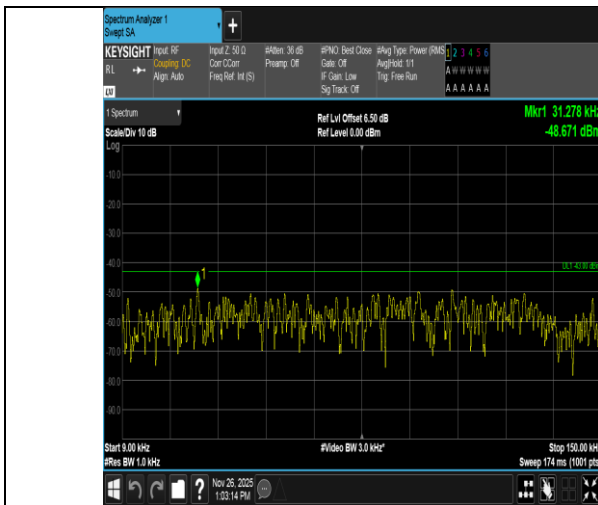
Band4-20MHz-QPSK-20050-1RB#0-0.009~0.15-PASS
