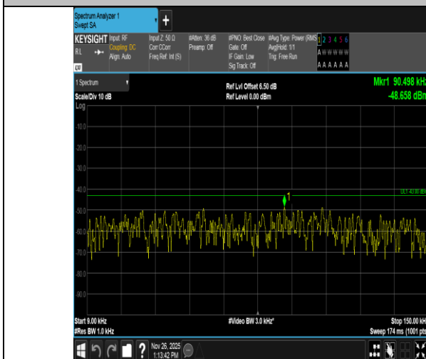
Band4-20MHz-QPSK-20175-100RB#0-0.009~0.15-PASS
