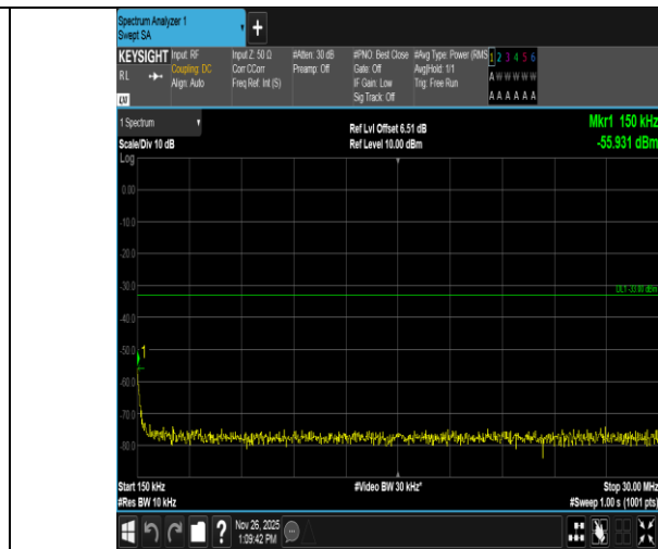
Band4-20MHz-QPSK-20175-1RB#0-0.15~30-PASS
