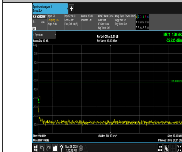
Band4-20MHz-16QAM-20175-1RB#0-0.15~30-PASS
