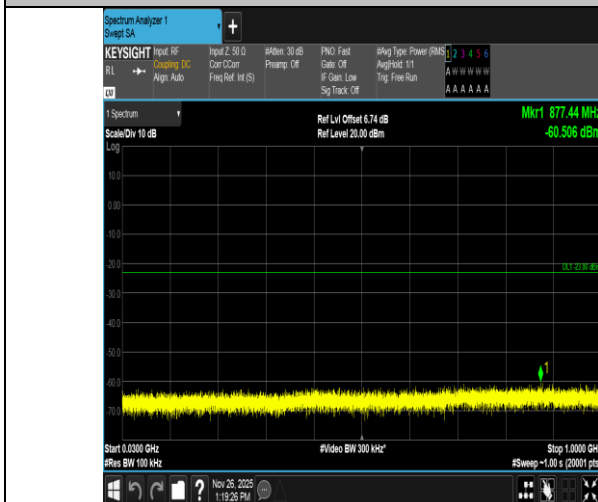
Band4-20MHz-16QAM-20300-1RB#99-30~1000-PASS
