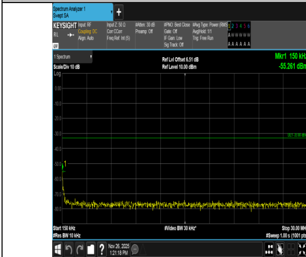
Band4-20MHz-16QAM-20300-100RB#0-0.15~30-PASS
