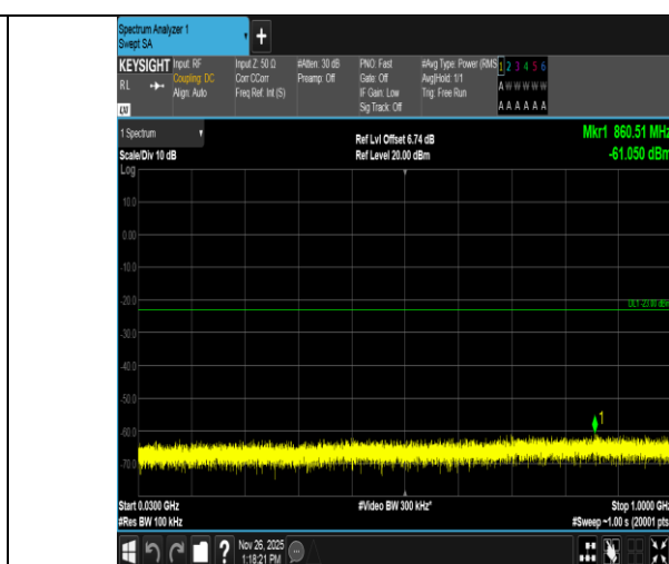
Band4-20MHz-QPSK-20300-1RB#99-30~1000-PASS
