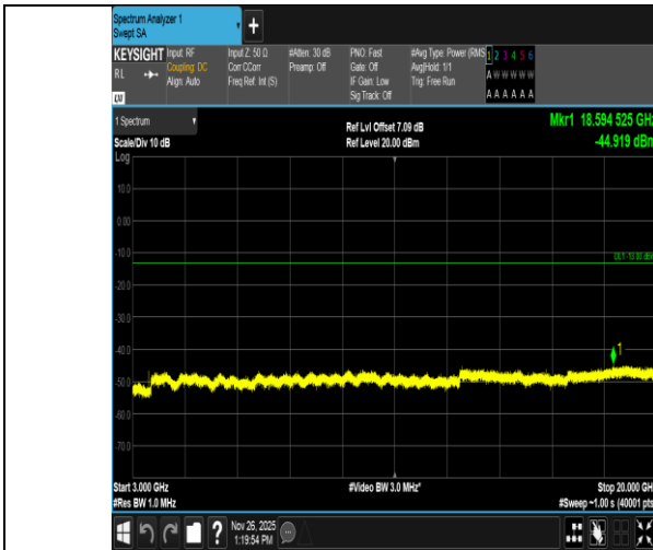
Band4-20MHz-16QAM-20300-1RB#99-3000~20000-PASS
