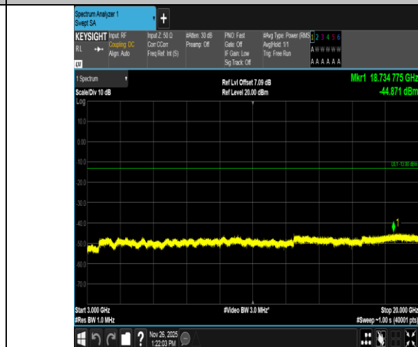
Band4-20MHz-16QAM-20300-100RB#0-3000~20000-PASS
