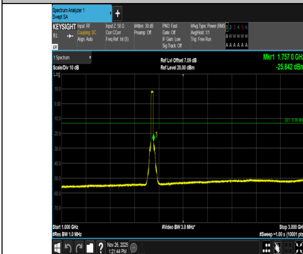
Band4-20MHz-16QAM-20300-100RB#0-1000~3000-PASS
