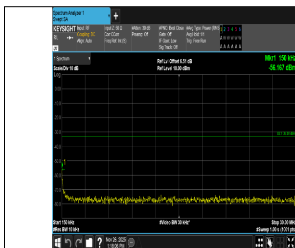
Band4-20MHz-QPSK-20300-1RB#99-0.15~30-PASS
