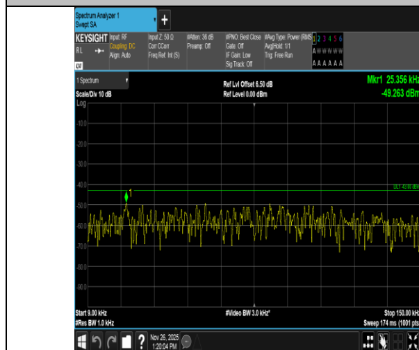
Band4-20MHz-QPSK-20300-100RB#0-0.009~0.15-PASS
