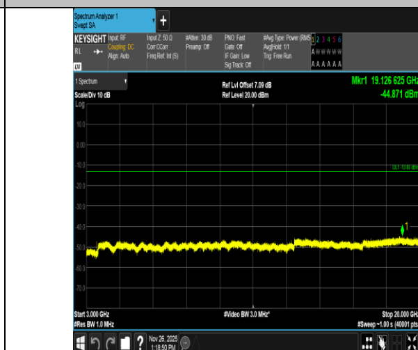
Band4-20MHz-QPSK-20300-1RB#99-3000~20000-PASS
