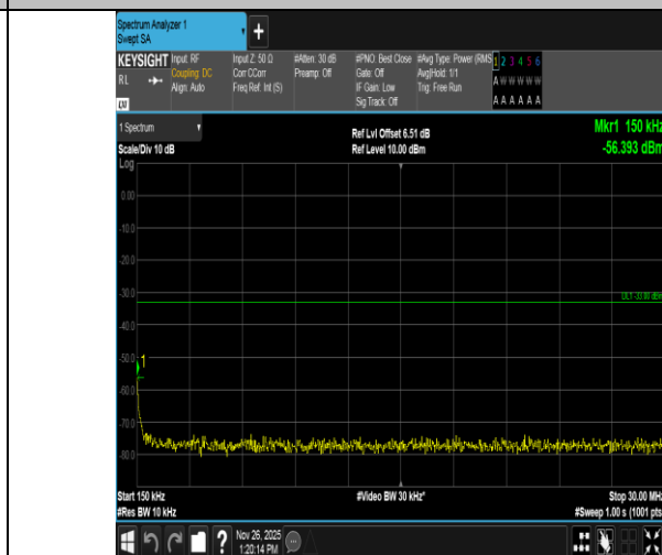
Band4-20MHz-QPSK-20300-100RB#0-0.15~30-PASS
