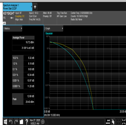
Band41-15MHz-16QAM-39725-75RB#0-PASS
