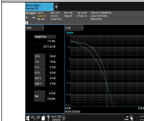
Band41-20MHz-16QAM-41490-1RB#0-PASS
