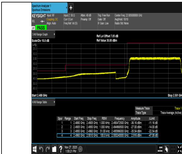
Band41-5MHz-QPSK-39675-25RB#0-PASS
