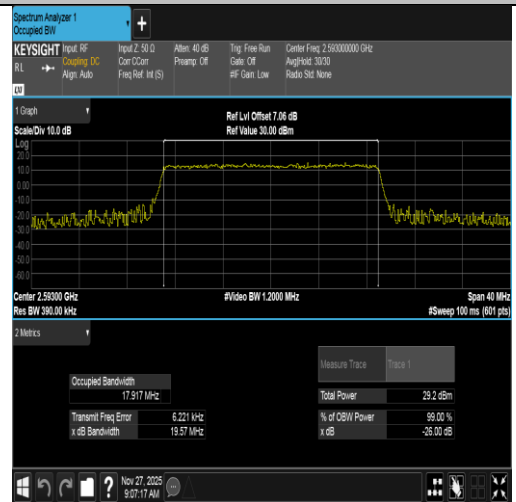
Band41-20MHz-16QAM-40620-100RB#0-PASS
