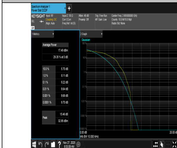
Band41-10MHz-16QAM-41540-1RB#0-PASS
