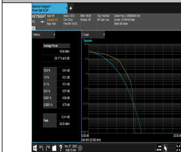
Band41-20MHz-16QAM-39750-1RB#0-PASS
