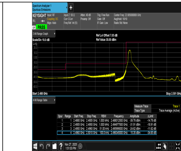
Band41-5MHz-16QAM-39675-1RB#0-PASS
