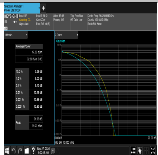
Band41-15MHz-16QAM-41515-75RB#0-PASS
