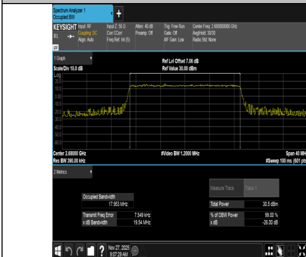
Band41-20MHz-QPSK-41490-100RB#0-PASS
