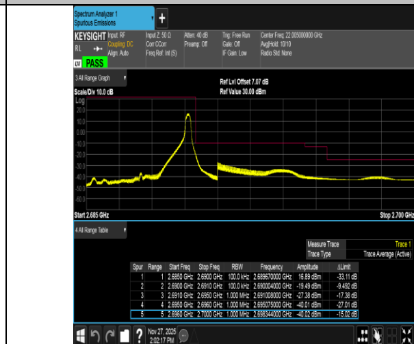
Band41-5MHz-QPSK-41565-1RB#24-PASS
