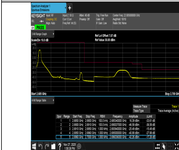
Band41-5MHz-QPSK-41565-1RB#0-PASS
