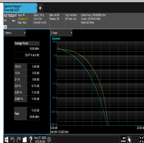
Band41-10MHz-16QAM-41540-50RB#0-PASS
