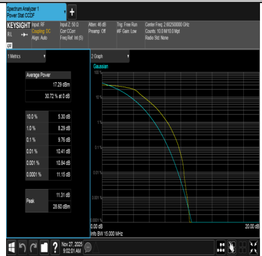
Band41-15MHz-QPSK-41515-75RB#0-PASS
