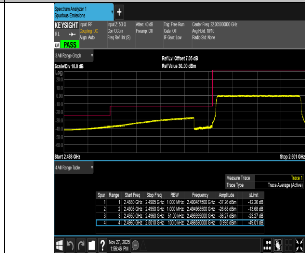
Band41-5MHz-16QAM-39675-25RB#0-PASS
