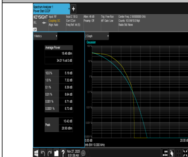
Band41-10MHz-QPSK-40620-1RB#0-PASS
