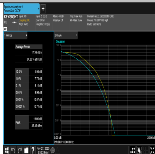
Band41-10MHz-QPSK-40620-50RB#0-PASS
