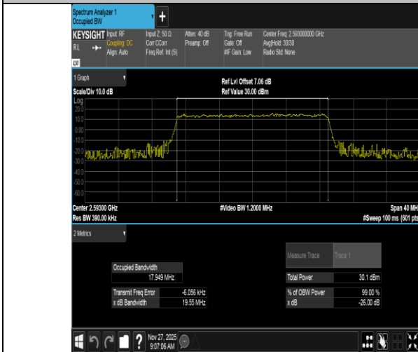
Band41-20MHz-QPSK-40620-100RB#0-PASS
