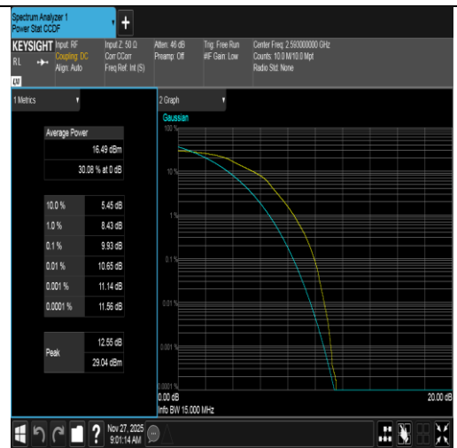
Band41-15MHz-16QAM-40620-75RB#0-PASS
