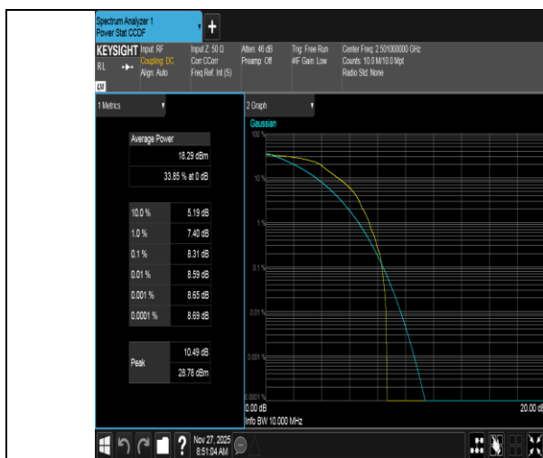
Band41-10MHz-QPSK-39700-1RB#0-PASS
