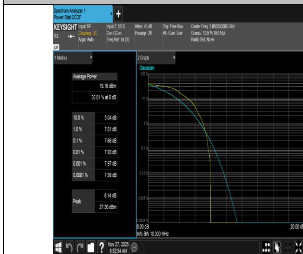
Band41-10MHz-QPSK-41540-1RB#0-PASS
