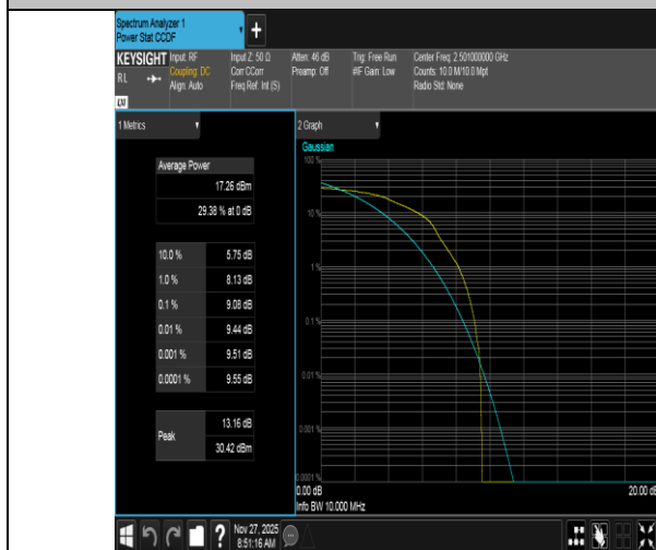
Band41-10MHz-16QAM-39700-1RB#0-PASS
