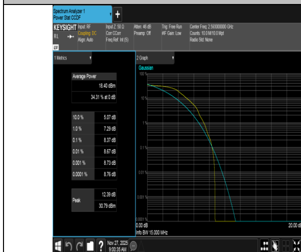
Band41-15MHz-QPSK-40620-1RB#0-PASS
