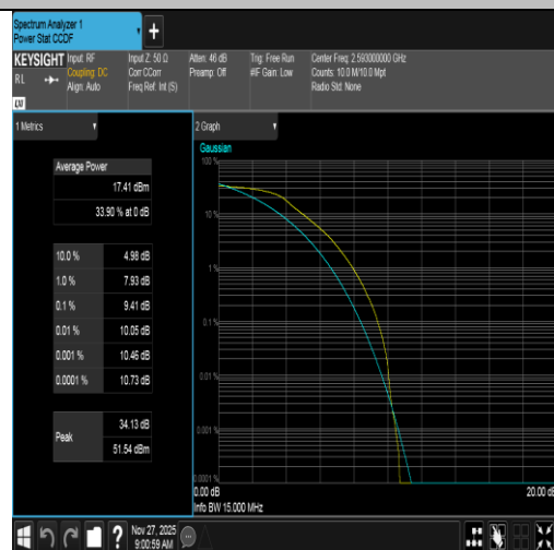
Band41-15MHz-QPSK-40620-75RB#0-PASS
