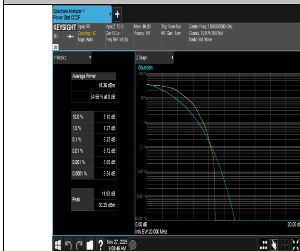
Band41-20MHz-QPSK-40620-1RB#0-PASS
