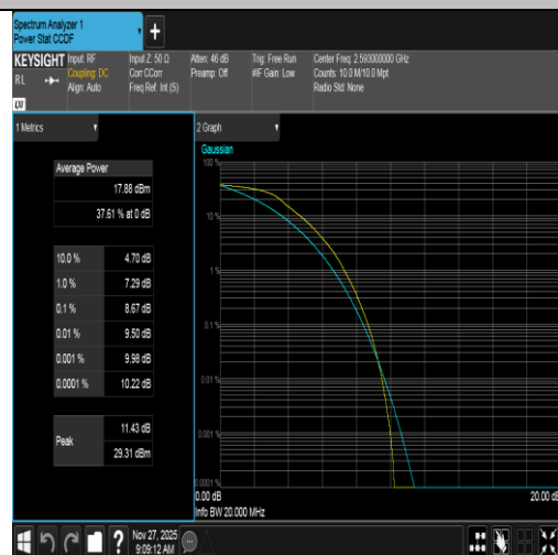
Band41-20MHz-QPSK-40620-100RB#0-PASS
