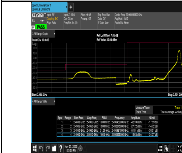
Band41-5MHz-16QAM-39675-1RB#24-PASS
