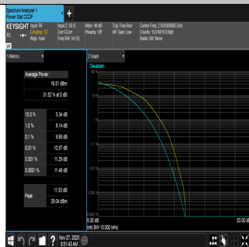
Band41-10MHz-16QAM-39700-50RB#0-PASS
