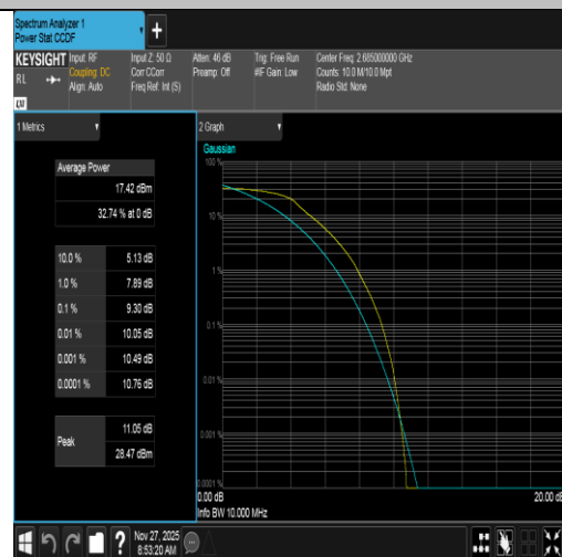
Band41-10MHz-QPSK-41540-50RB#0-PASS
