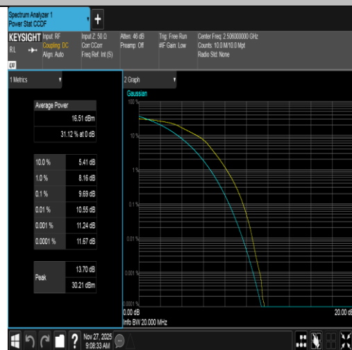
Band41-20MHz-16QAM-39750-100RB#0-PASS
