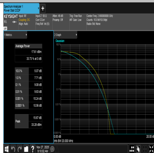
Band41-20MHz-QPSK-41490-100RB#0-PASS
