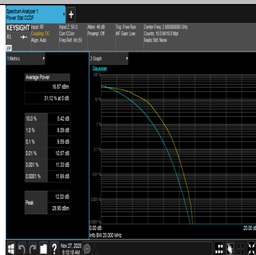
Band41-20MHz-16QAM-41490-100RB#0-PASS
