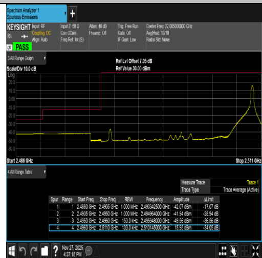
Band41-15MHz-QPSK-39725-1RB#74-PASS
