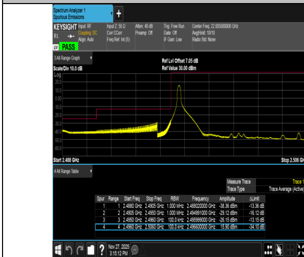
Band41-10MHz-QPSK-39700-1RB#0-PASS
