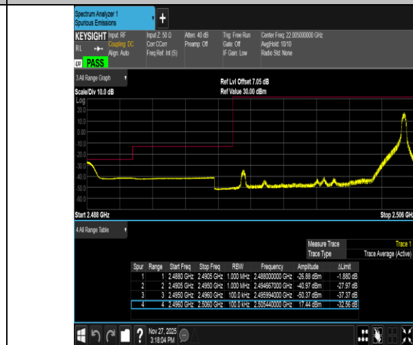
Band41-10MHz-QPSK-39700-1RB#49-PASS
