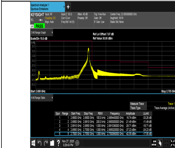
Band41-10MHz-16QAM-41540-1RB#49-PASS
