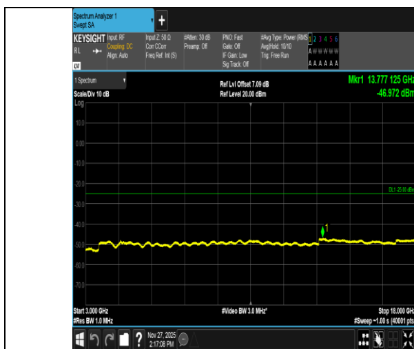
Band41-5MHz-16QAM-39675-1RB#24-3000~18000-PASS
