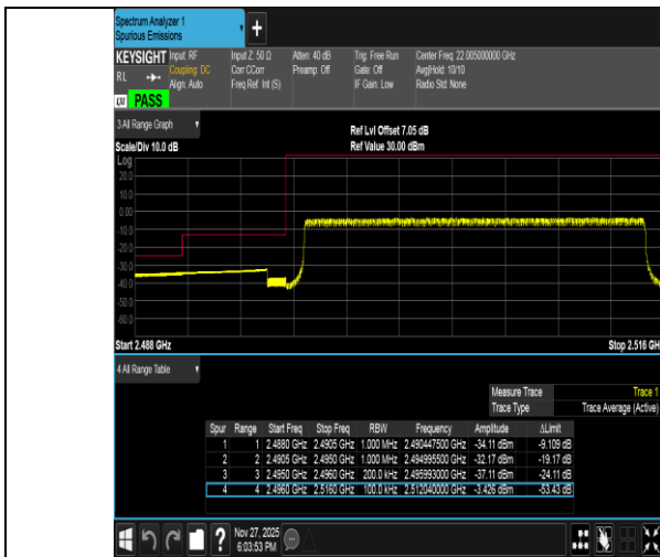
Band41-20MHz-QPSK-39750-100RB#0-PASS
