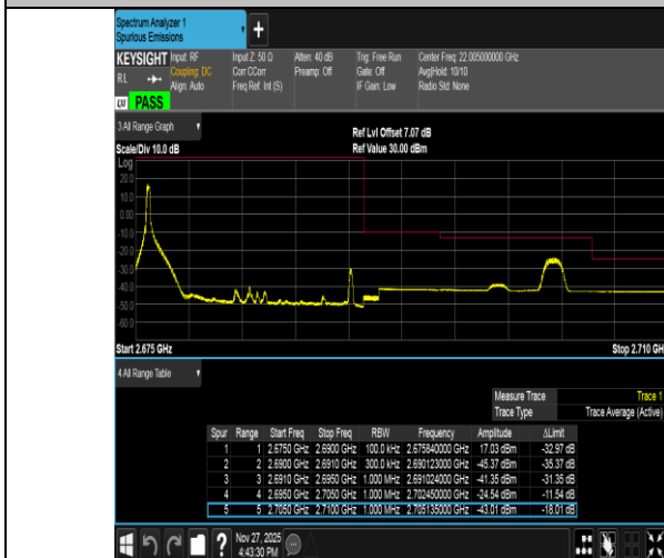
Band41-15MHz-QPSK-41515-1RB#0-PASS
