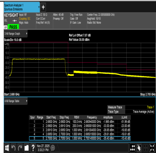
Band41-10MHz-16QAM-41540-50RB#0-PASS
