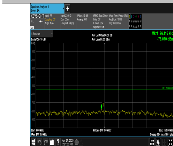
Band41-5MHz-16QAM-39675-25RB#0-0.009~0.15-PASS
