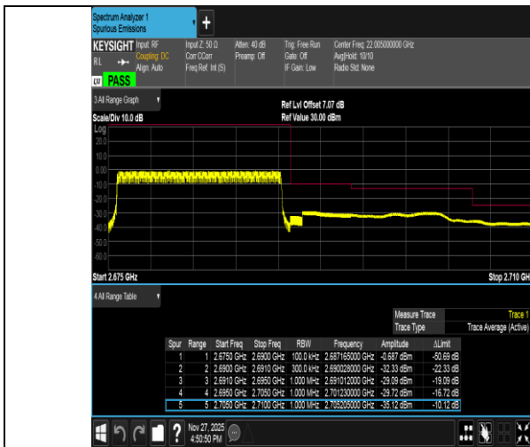
Band41-15MHz-QPSK-41515-75RB#0-PASS
