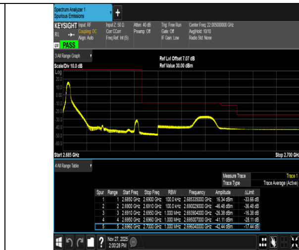
Band41-5MHz-16QAM-41565-1RB#0-PASS
