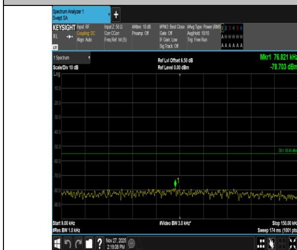
Band41-5MHz-QPSK-39675-25RB#0-0.009~0.15-PASS
