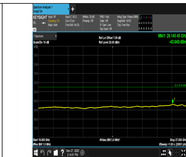
Band41-5MHz-QPSK-39675-1RB#24-18000~27000-PASS
