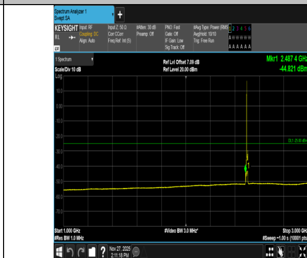
Band41-5MHz-16QAM-39675-1RB#0-1000~3000-PASS
