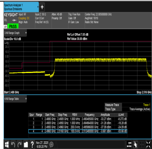
Band41-20MHz-16QAM-39750-100RB#0-PASS
