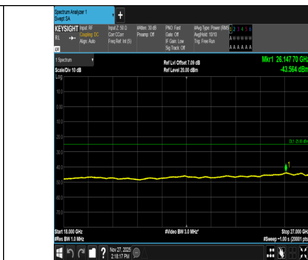
Band41-5MHz-16QAM-39675-1RB#24-18000~27000-PASS
