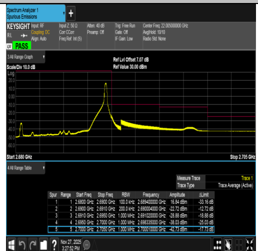
Band41-10MHz-QPSK-41540-1RB#49-PASS
