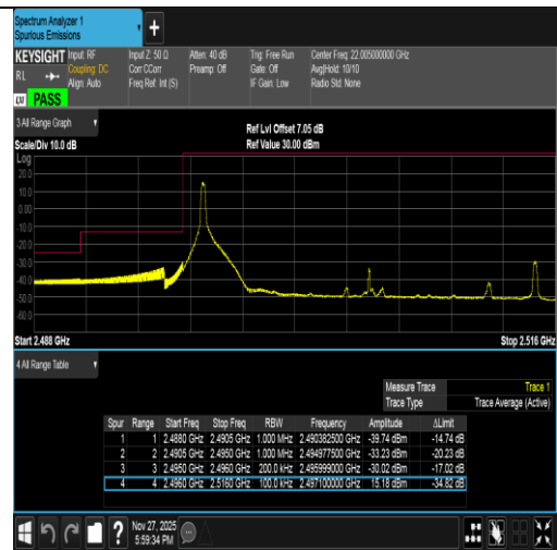
Band41-20MHz-16QAM-39750-1RB#0-PASS
