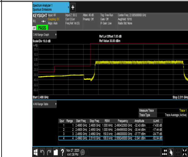
Band41-15MHz-16QAM-39725-75RB#0-PASS
