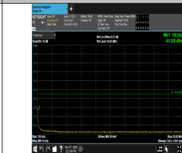
Band41-5MHz-16QAM-39675-25RB#0-0.15~30-PASS
