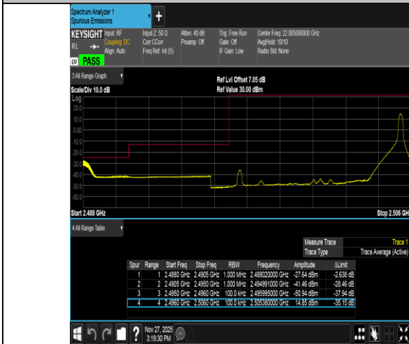
Band41-10MHz-16QAM-39700-1RB#49-PASS
