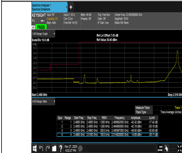
Band41-20MHz-16QAM-39750-1RB#99-PASS
