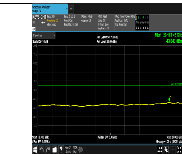
Band41-5MHz-QPSK-39675-25RB#0-18000~27000-PASS
