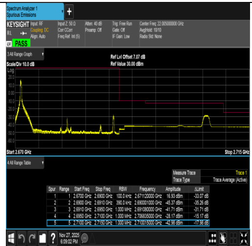
Band41-20MHz-16QAM-41490-1RB#0-PASS
