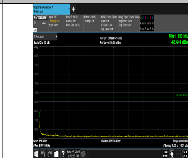
Band41-5MHz-QPSK-39675-25RB#0-0.15~30-PASS
