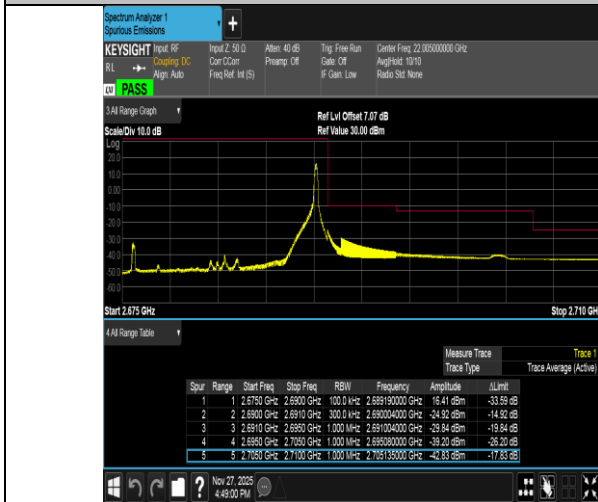
Band41-15MHz-16QAM-41515-1RB#74-PASS
