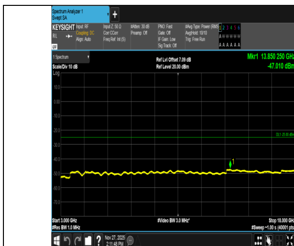
Band41-5MHz-16QAM-39675-1RB#0-3000~18000-PASS
