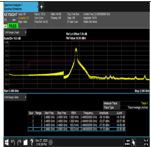
Band41-10MHz-16QAM-39700-1RB#0-PASS
