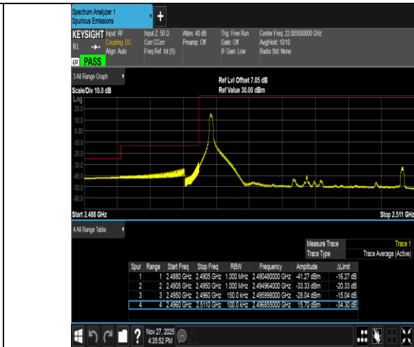
Band41-15MHz-16QAM-39725-1RB#0-PASS
