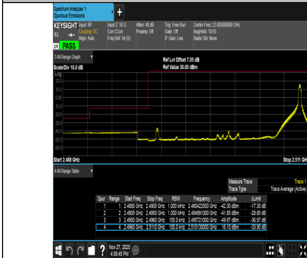
Band41-15MHz-16QAM-39725-1RB#74-PASS
