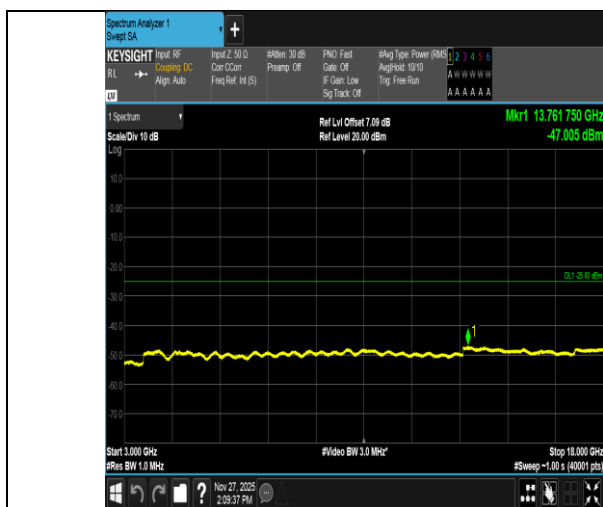
Band41-5MHz-QPSK-39675-1RB#0-3000~18000-PASS
