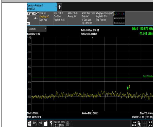
Band41-5MHz-QPSK-39675-1RB#24-0.009~0.15-PASS
