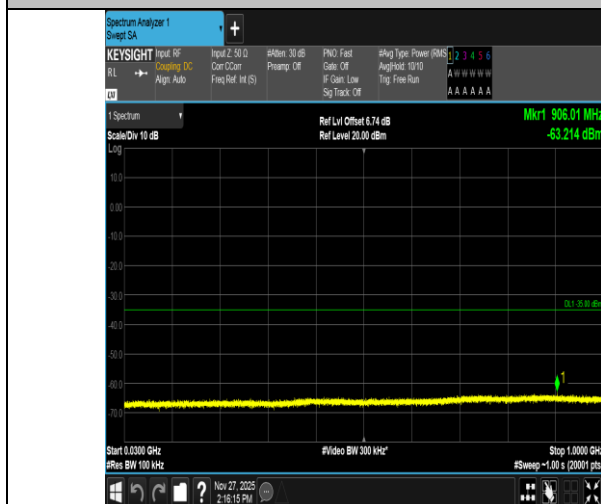
Band41-5MHz-16QAM-39675-1RB#24-30~1000-PASS
