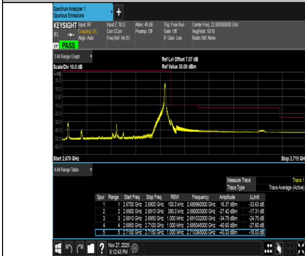
Band41-20MHz-16QAM-41490-1RB#99-PASS
