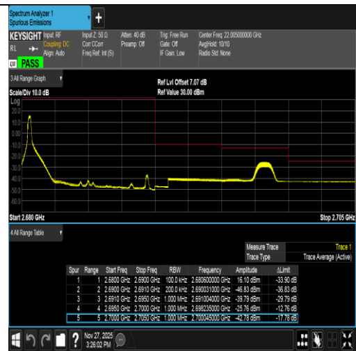
Band41-10MHz-16QAM-41540-1RB#0-PASS
