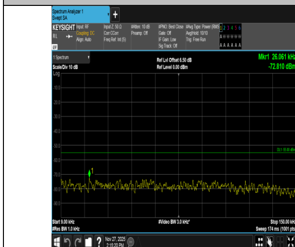
Band41-5MHz-16QAM-39675-1RB#24-0.009~0.15-PASS
