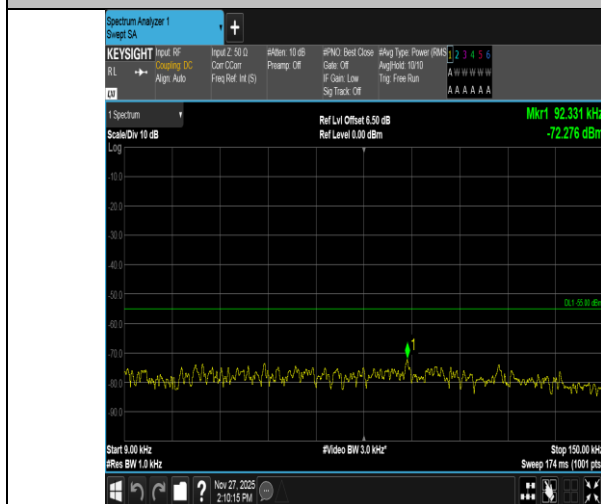
Band41-5MHz-16QAM-39675-1RB#0-0.009~0.15-PASS
