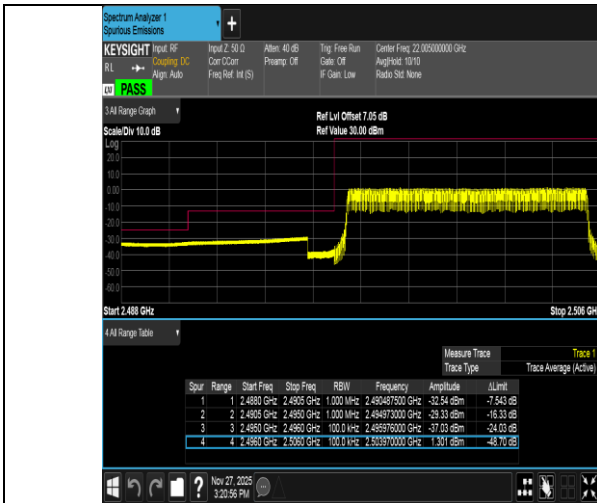
Band41-10MHz-QPSK-39700-50RB#0-PASS
