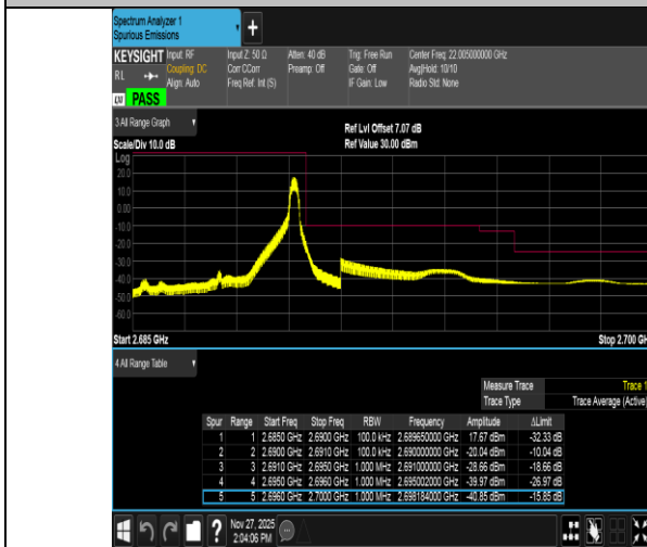
Band41-5MHz-16QAM-41565-1RB#24-PASS
