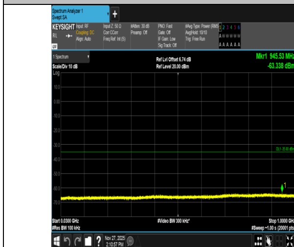
Band41-5MHz-16QAM-39675-1RB#0-30~1000-PASS
