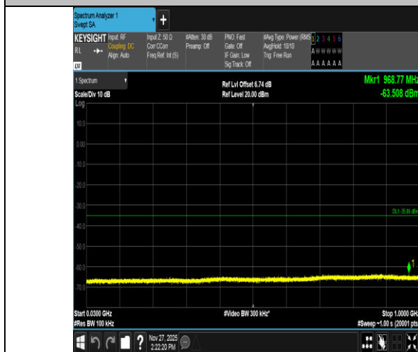
Band41-5MHz-16QAM-39675-25RB#0-30~1000-PASS
