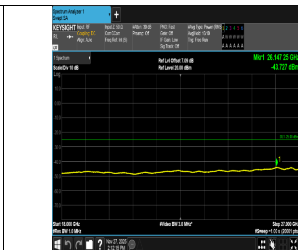
Band41-5MHz-16QAM-39675-1RB#0-18000~27000-PASS
