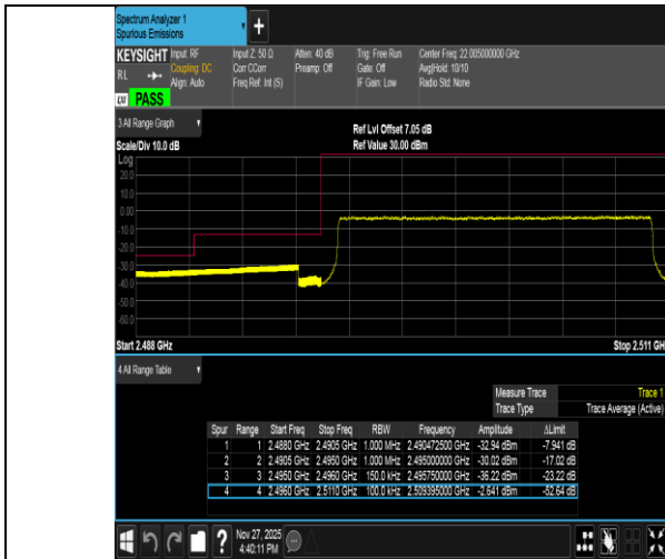
Band41-15MHz-QPSK-39725-75RB#0-PASS
