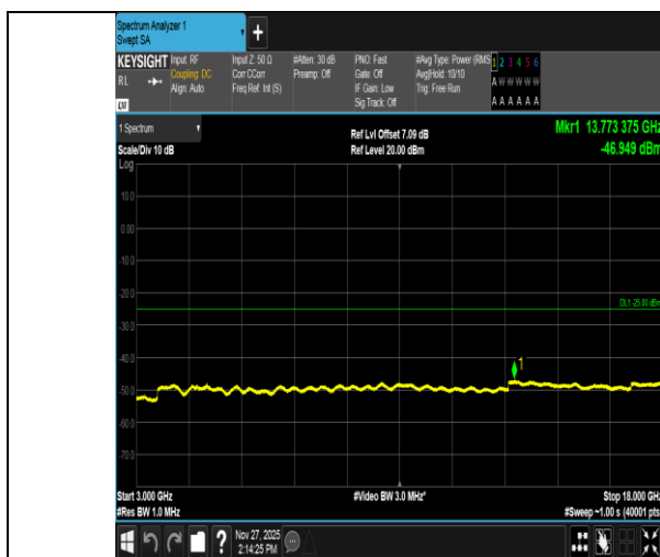
Band41-5MHz-QPSK-39675-1RB#24-3000~18000-PASS
