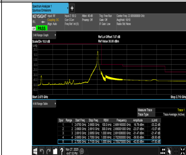
Band41-15MHz-QPSK-41515-1RB#74-PASS
