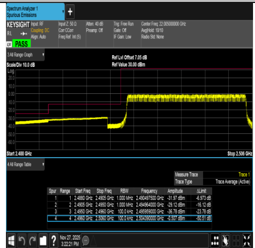
Band41-10MHz-16QAM-39700-50RB#0-PASS
