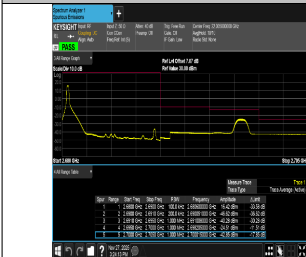
Band41-10MHz-QPSK-41540-1RB#0-PASS
