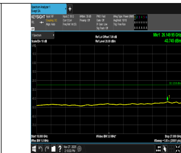
Band41-5MHz-QPSK-39675-1RB#0-18000~27000-PASS
