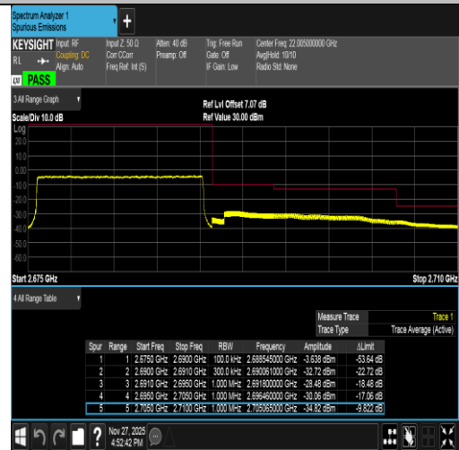
Band41-15MHz-16QAM-41515-75RB#0-PASS
