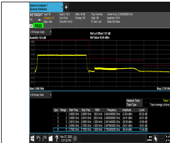
Band41-10MHz-QPSK-41540-50RB#0-PASS
