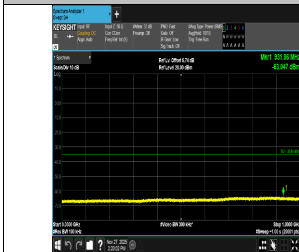
Band41-5MHz-QPSK-39675-25RB#0-30~1000-PASS
