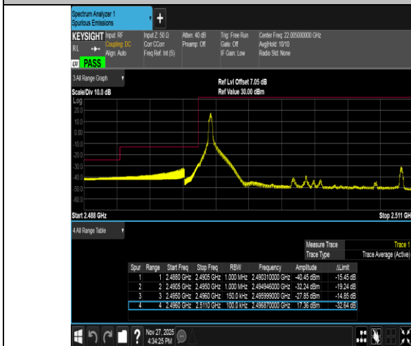
Band41-15MHz-QPSK-39725-1RB#0-PASS
