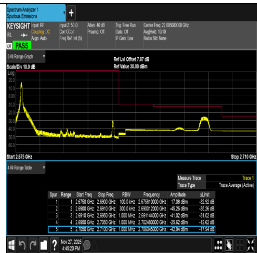
Band41-15MHz-16QAM-41515-1RB#0-PASS
