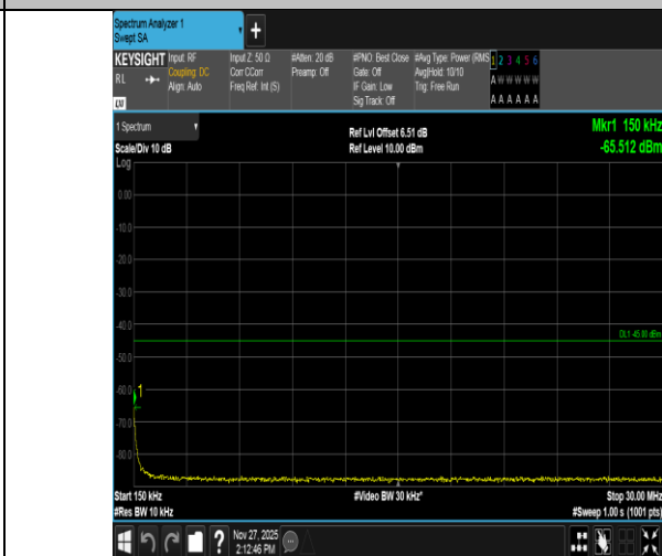
Band41-5MHz-QPSK-39675-1RB#24-0.15~30-PASS
