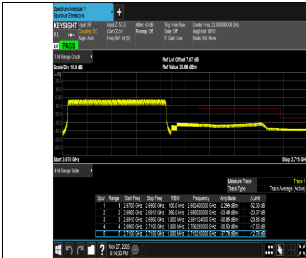
Band41-20MHz-QPSK-41490-100RB#0-PASS
