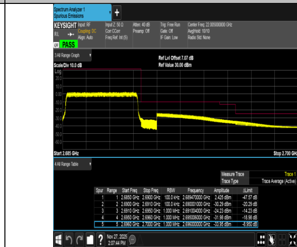
Band41-5MHz-16QAM-41565-25RB#0-PASS
