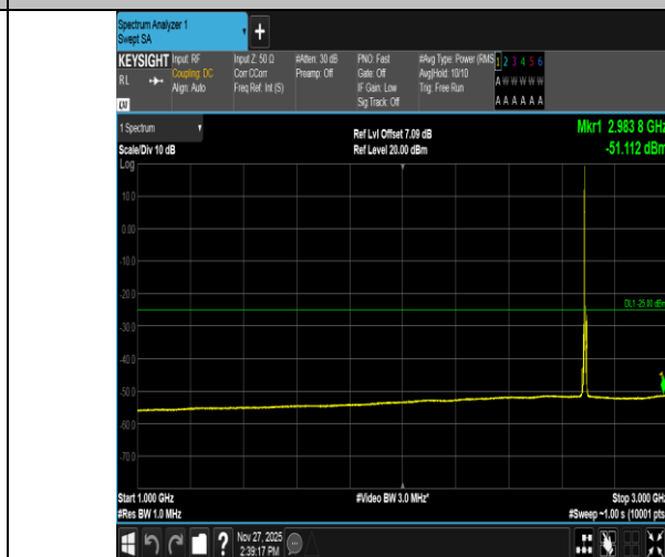
Band41-5MHz-QPSK-41565-1RB#0-1000~3000-PASS
