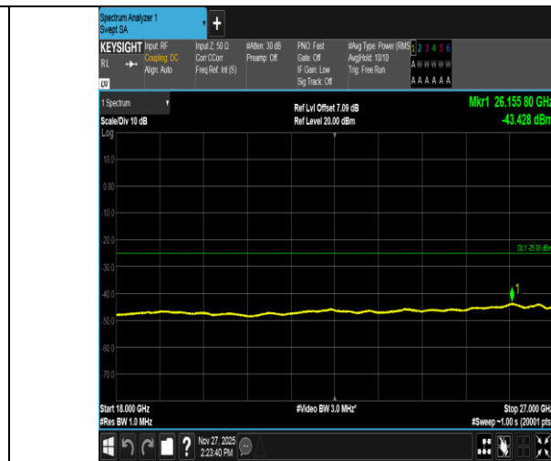
Band41-5MHz-16QAM-39675-25RB#0-18000~27000-PASS
