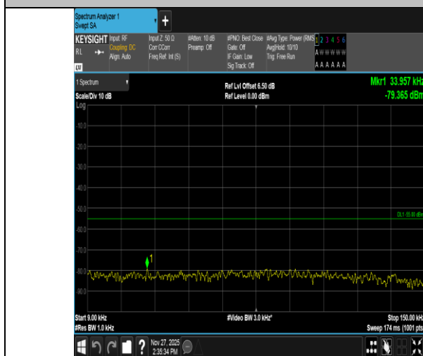
Band41-5MHz-16QAM-40620-25RB#0-0.009~0.15-PASS
