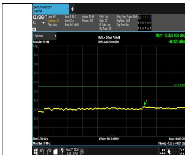
Band41-5MHz-16QAM-41565-1RB#0-3000~18000-PASS
