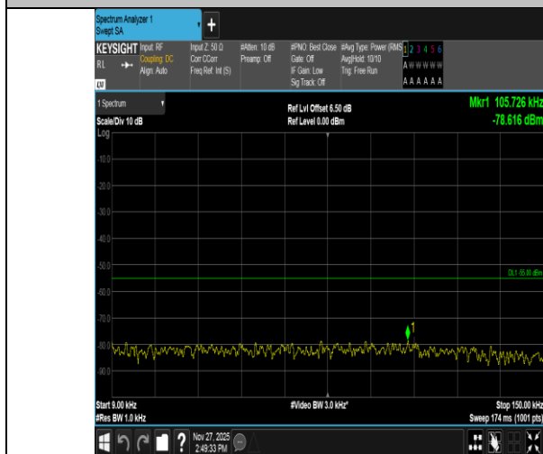
Band41-5MHz-QPSK-41565-25RB#0-0.009~0.15-PASS
