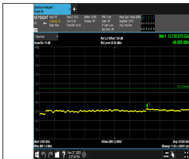
Band41-5MHz-16QAM-40620-25RB#0-3000~18000-PASS
