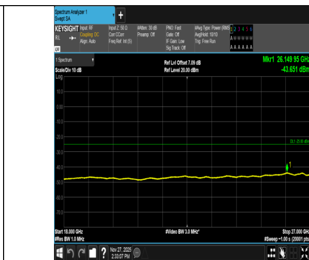
Band41-5MHz-16QAM-40620-1RB#24-18000~27000-PASS
