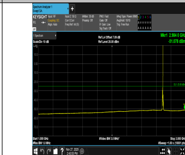
Band41-5MHz-QPSK-41565-1RB#24-1000~3000-PASS
