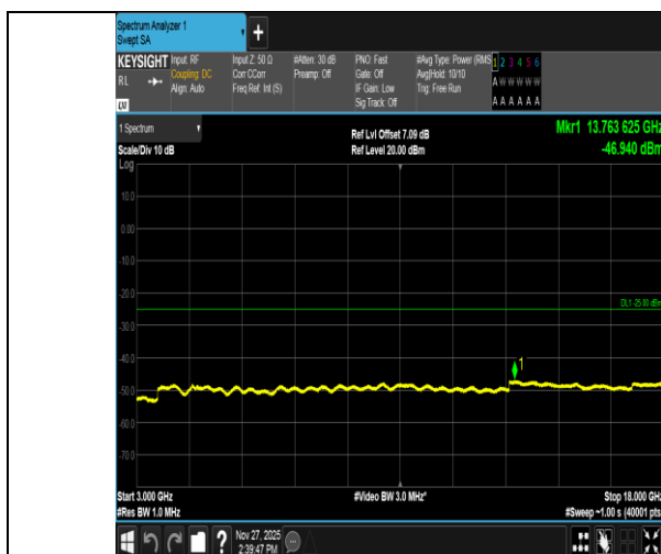
Band41-5MHz-QPSK-41565-1RB#0-3000~18000-PASS
