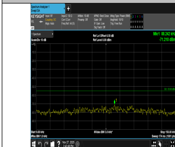
Band41-5MHz-QPSK-41565-1RB#24-0.009~0.15-PASS
