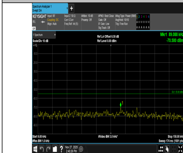
Band41-5MHz-16QAM-41565-1RB#0-0.009~0.15-PASS
