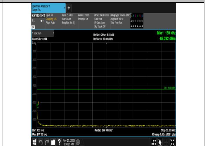
Band41-10MHz-QPSK-39700-1RB#49-0.15~30-PASS
