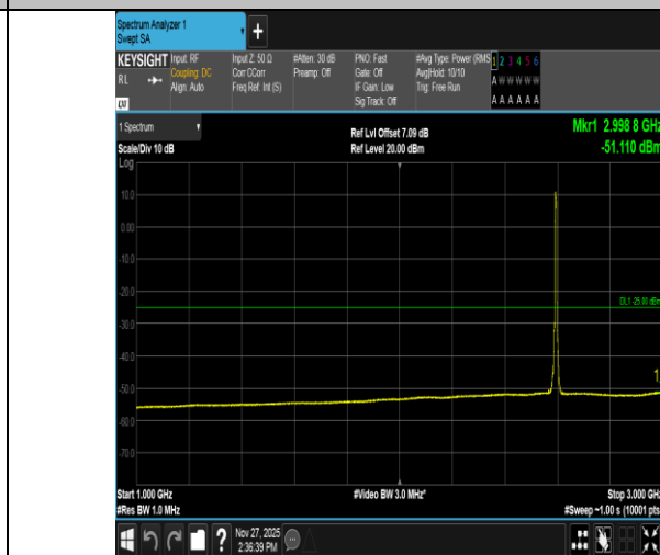
Band41-5MHz-16QAM-40620-25RB#0-1000~3000-PASS
