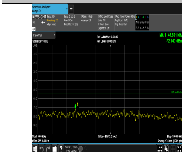
Band41-5MHz-16QAM-40620-1RB#0-0.009~0.15-PASS
