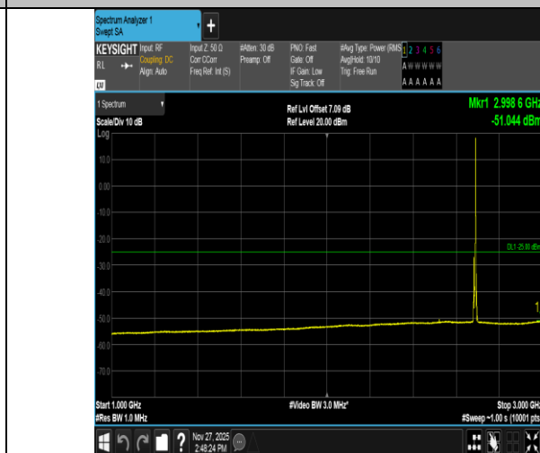
Band41-5MHz-16QAM-41565-1RB#24-1000~3000-PASS
