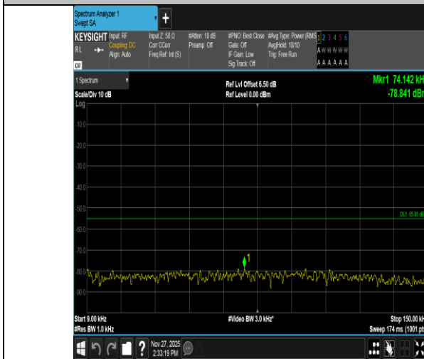
Band41-5MHz-QPSK-40620-25RB#0-0.009~0.15-PASS
