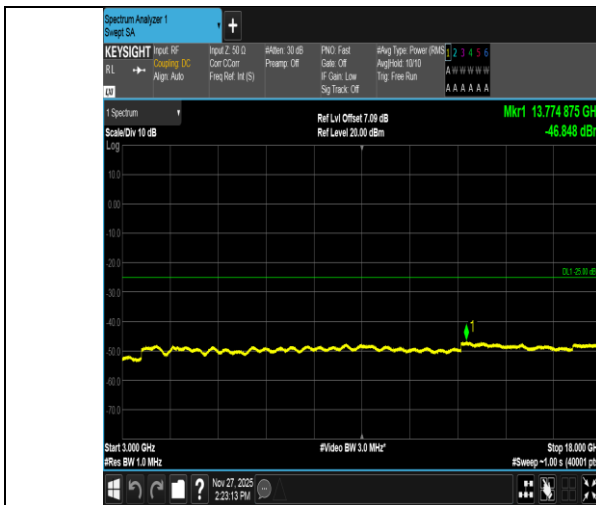
Band41-5MHz-16QAM-39675-25RB#0-3000~18000-PASS
