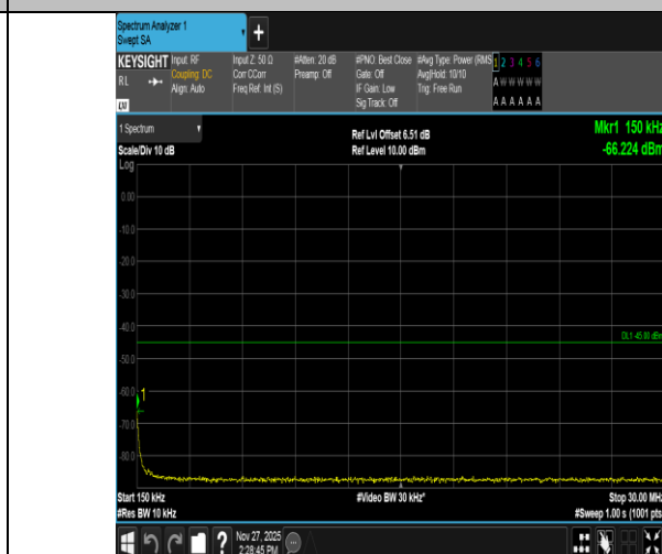
Band41-5MHz-QPSK-40620-1RB#24-0.15~30-PASS
