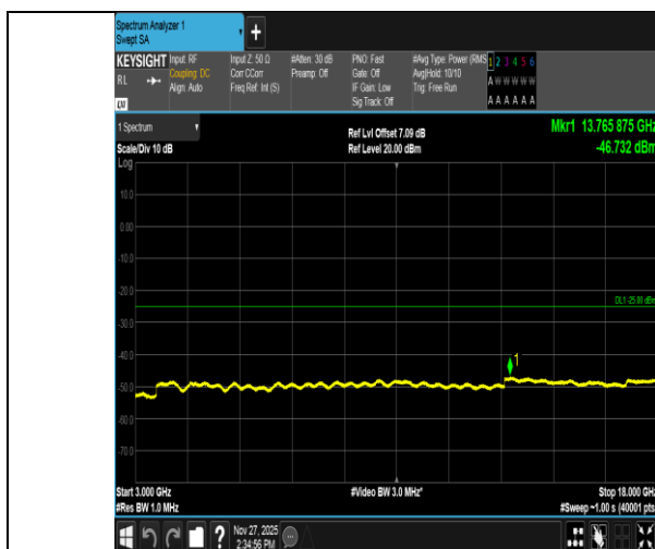
Band41-5MHz-QPSK-40620-25RB#0-3000~18000-PASS
