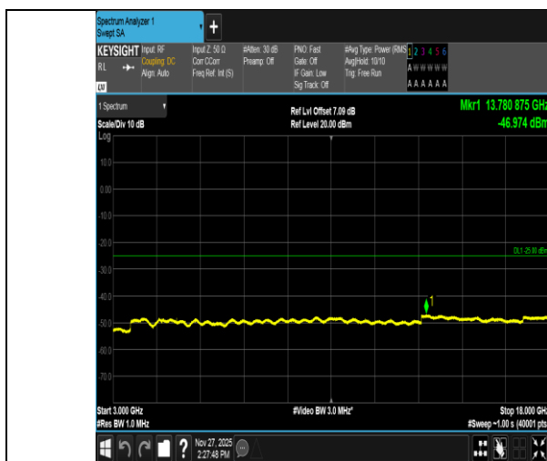
Band41-5MHz-16QAM-40620-1RB#0-3000~18000-PASS
