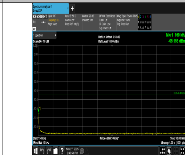
Band41-5MHz-16QAM-41565-1RB#0-0.15~30-PASS
