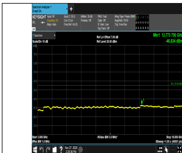
Band41-5MHz-QPSK-40620-1RB#0-3000~18000-PASS
