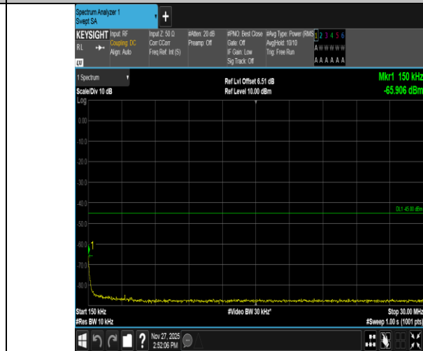
Band41-5MHz-16QAM-41565-25RB#0-0.15~30-PASS
