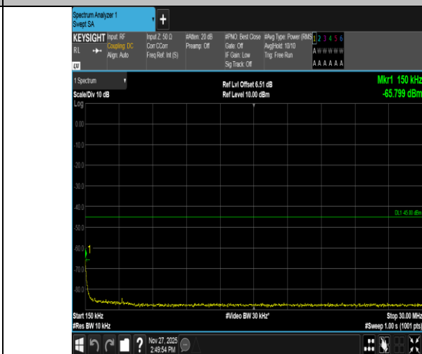
Band41-5MHz-QPSK-41565-25RB#0-0.15~30-PASS
