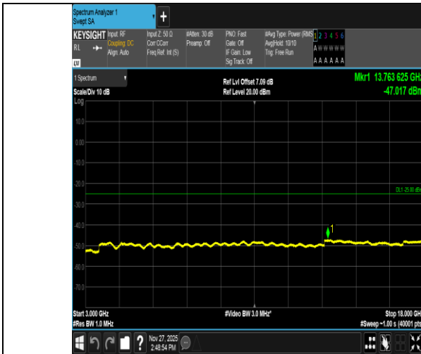
Band41-5MHz-16QAM-41565-1RB#24-3000~18000-PASS
