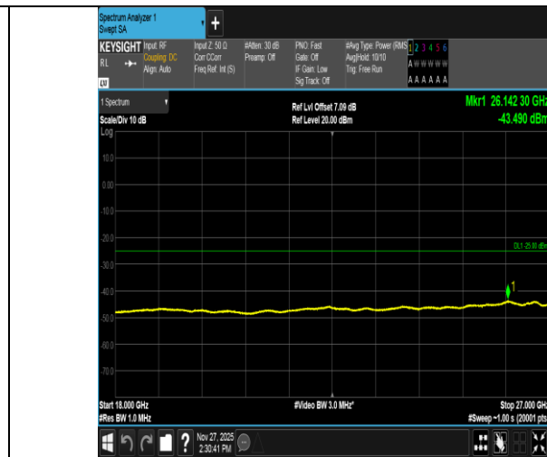
Band41-5MHz-QPSK-40620-1RB#24-18000~27000-PASS
