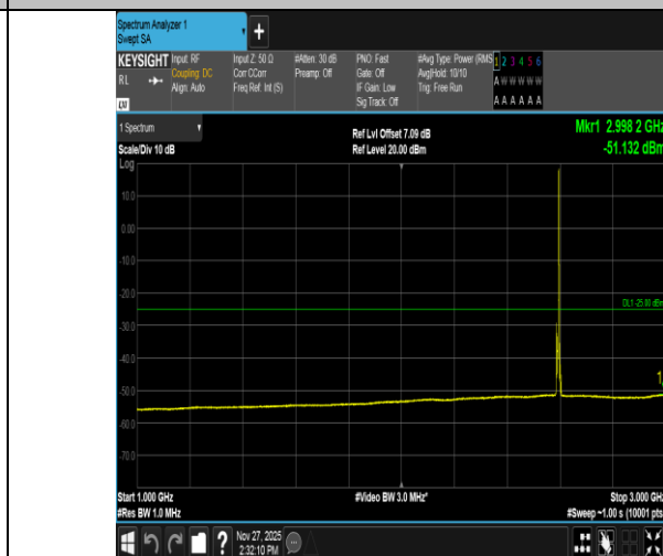
Band41-5MHz-16QAM-40620-1RB#24-1000~3000-PASS
