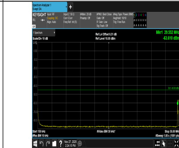
Band41-5MHz-QPSK-40620-1RB#0-0.15~30-PASS
