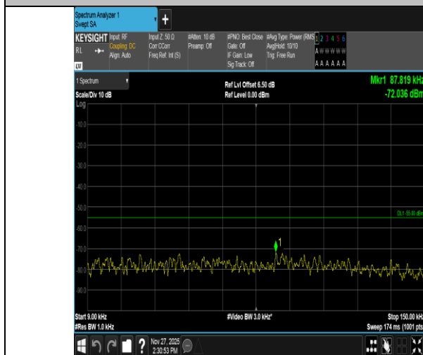
Band41-5MHz-16QAM-40620-1RB#24-0.009~0.15-PASS
