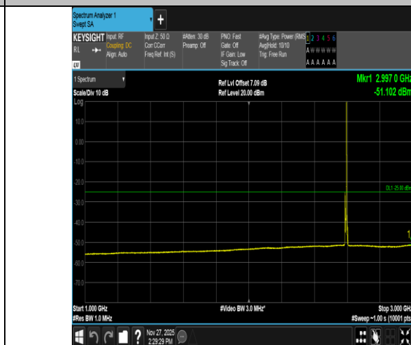
Band41-5MHz-QPSK-40620-1RB#24-1000~3000-PASS
