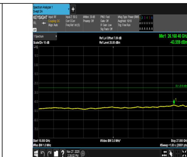
Band41-5MHz-QPSK-40620-1RB#0-18000~27000-PASS
