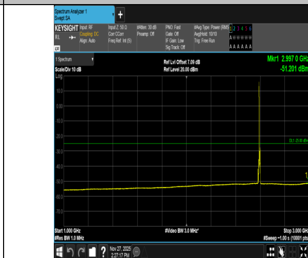
Band41-5MHz-16QAM-40620-1RB#0-1000~3000-PASS
