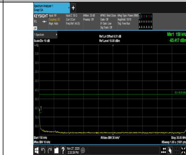
Band41-5MHz-QPSK-40620-25RB#0-0.15~30-PASS
