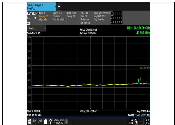
Band41-10MHz-QPSK-39700-1RB#0-18000~27000-PASS
