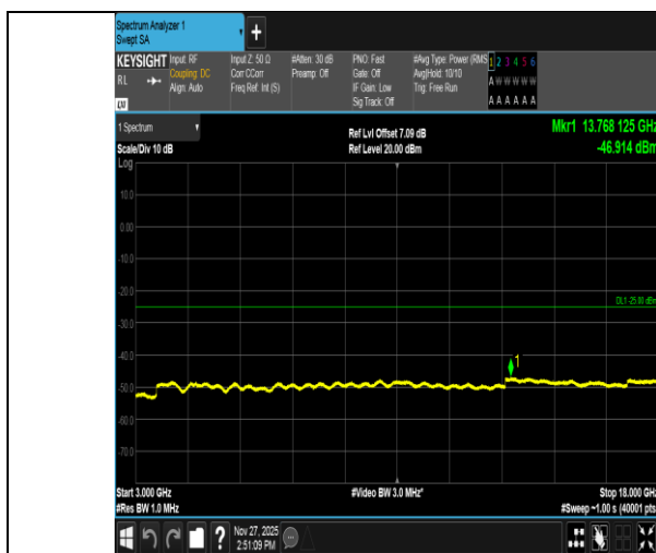
Band41-5MHz-QPSK-41565-25RB#0-3000~18000-PASS
