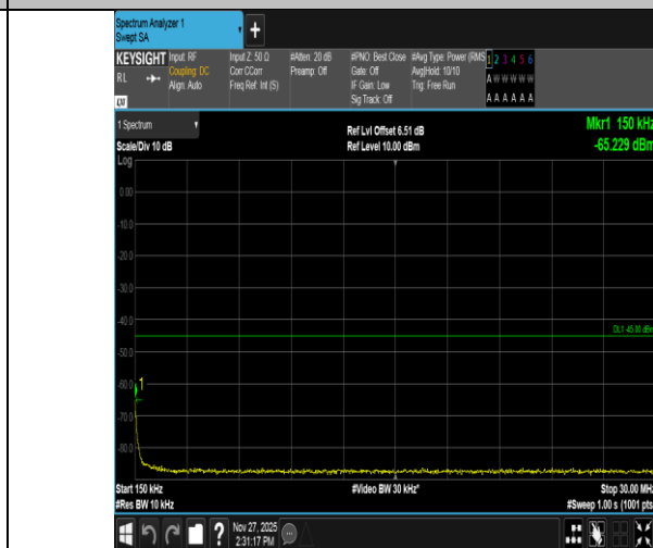
Band41-5MHz-16QAM-40620-1RB#24-0.15~30-PASS
