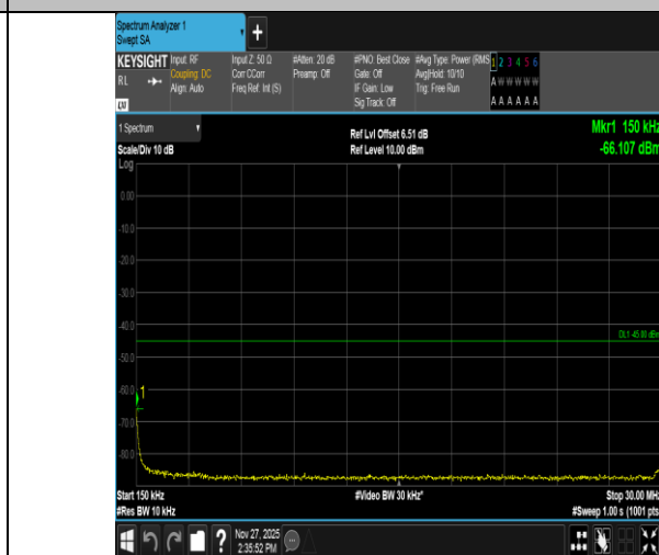
Band41-5MHz-16QAM-40620-25RB#0-0.15~30-PASS
