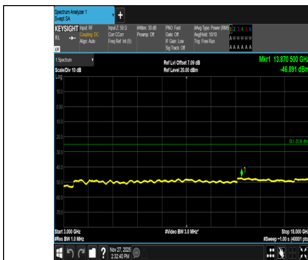
Band41-5MHz-16QAM-40620-1RB#24-3000~18000-PASS
