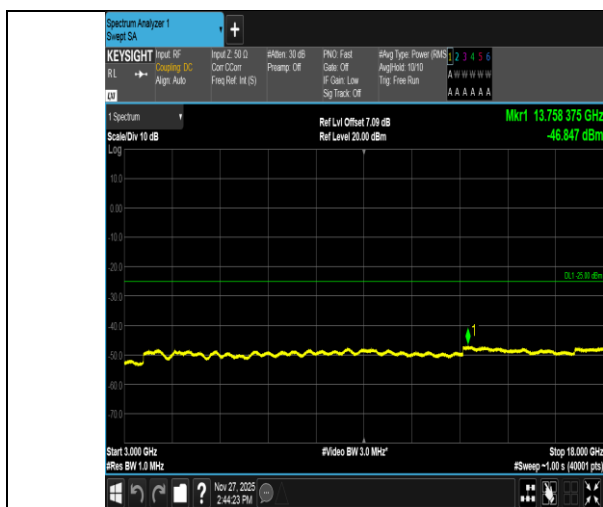
Band41-5MHz-QPSK-41565-1RB#24-3000~18000-PASS
