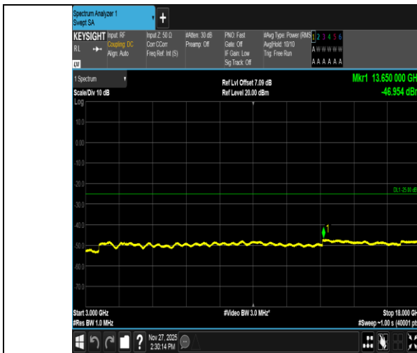
Band41-5MHz-QPSK-40620-1RB#24-3000~18000-PASS
