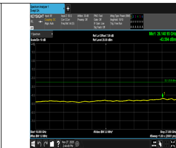
Band41-5MHz-QPSK-41565-1RB#24-18000~27000-PASS
