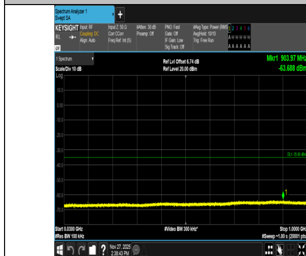
Band41-5MHz-QPSK-41565-1RB#0-30~1000-PASS
