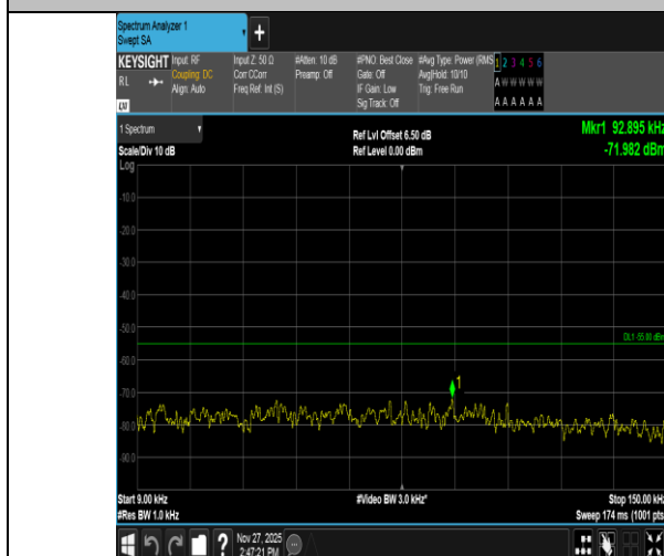
Band41-5MHz-16QAM-41565-1RB#24-0.009~0.15-PASS
