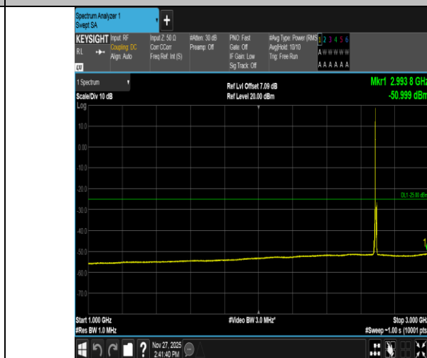
Band41-5MHz-16QAM-41565-1RB#0-1000~3000-PASS
