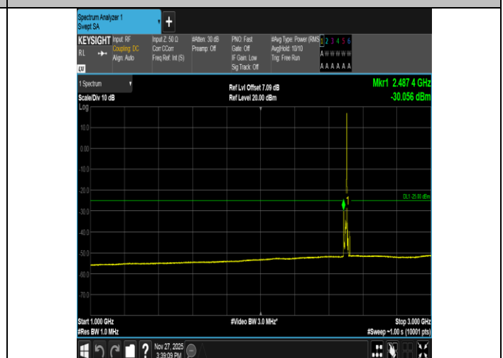
Band41-10MHz-QPSK-39700-1RB#49-1000~3000-PASS
