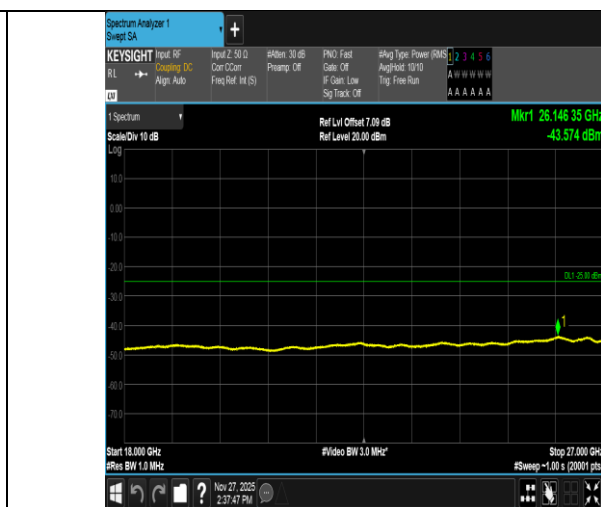
Band41-5MHz-16QAM-40620-25RB#0-18000~27000-PASS
