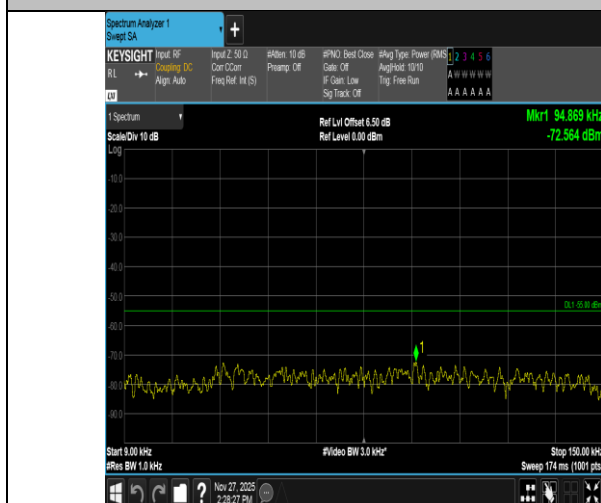
Band41-5MHz-QPSK-40620-1RB#24-0.009~0.15-PASS
