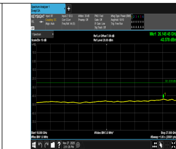
Band41-5MHz-QPSK-41565-25RB#0-18000~27000-PASS
