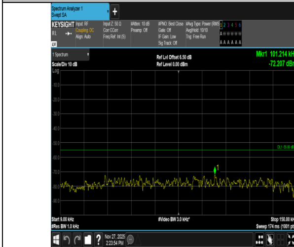
Band41-5MHz-QPSK-40620-1RB#0-0.009~0.15-PASS
