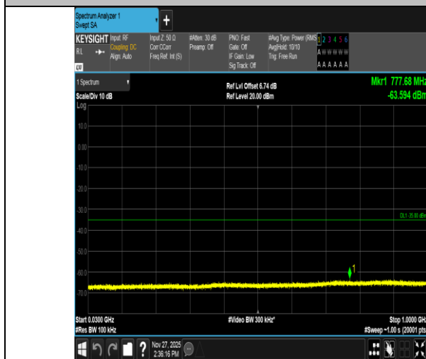
Band41-5MHz-16QAM-40620-25RB#0-30~1000-PASS
