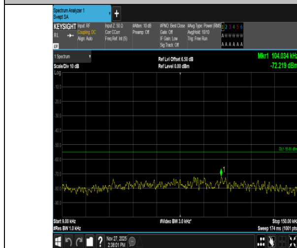
Band41-5MHz-QPSK-41565-1RB#0-0.009~0.15-PASS
