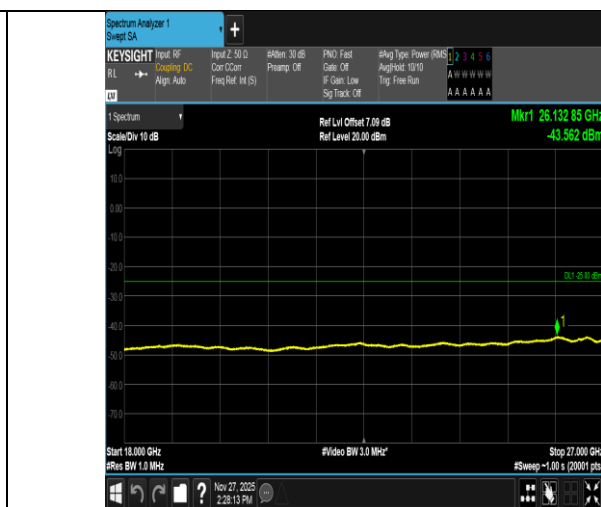
Band41-5MHz-16QAM-40620-1RB#0-18000~27000-PASS
