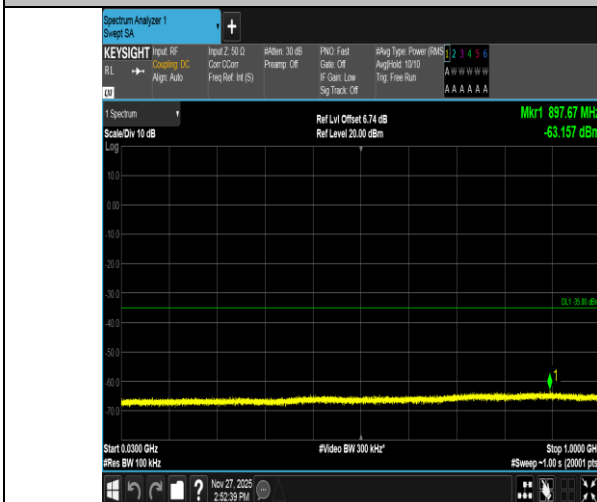
Band41-5MHz-16QAM-41565-25RB#0-30~1000-PASS
