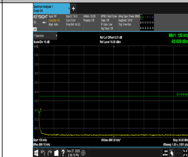
Band41-5MHz-QPSK-41565-1RB#0-0.15~30-PASS
