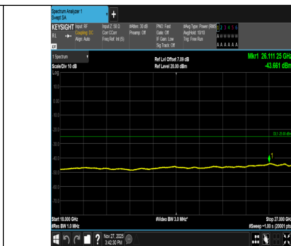
Band41-10MHz-16QAM-39700-1RB#49-18000~27000-PASS
