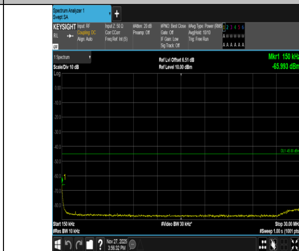
Band41-10MHz-QPSK-40620-50RB#0-0.15~30-PASS
