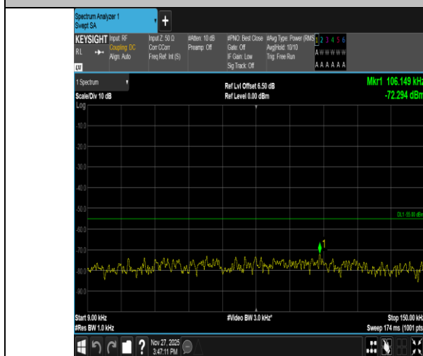
Band41-10MHz-QPSK-40620-1RB#0-0.009~0.15-PASS
