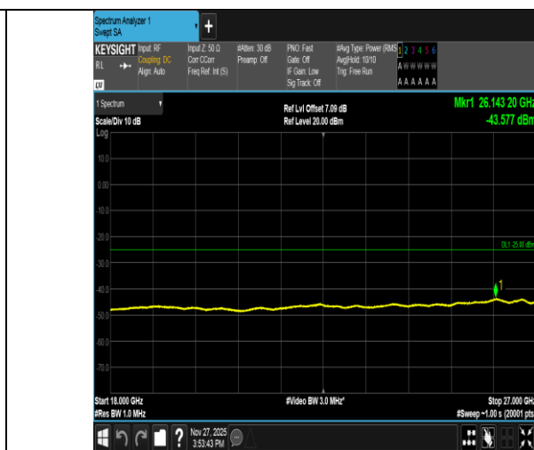
Band41-10MHz-QPSK-40620-1RB#49-18000~27000-PASS
