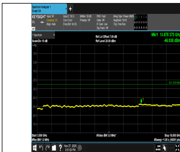
Band41-10MHz-16QAM-40620-1RB#0-3000~18000-PASS
