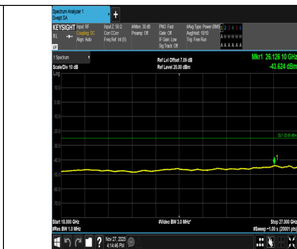
Band41-10MHz-16QAM-41540-50RB#0-18000~27000-PASS
