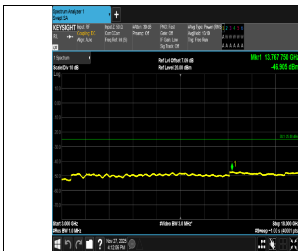
Band41-10MHz-QPSK-41540-50RB#0-3000~18000-PASS
