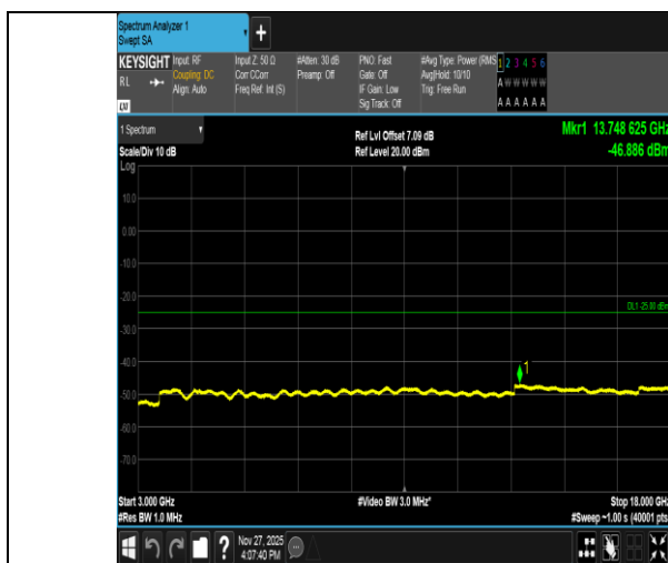
Band41-10MHz-QPSK-41540-1RB#49-3000~18000-PASS
