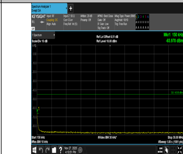
Band41-10MHz-QPSK-41540-50RB#0-0.15~30-PASS
