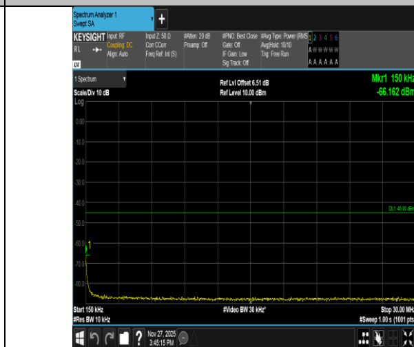
Band41-10MHz-16QAM-39700-50RB#0-0.15~30-PASS
