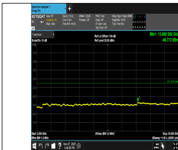
Band41-10MHz-QPSK-40620-1RB#0-3000~18000-PASS
