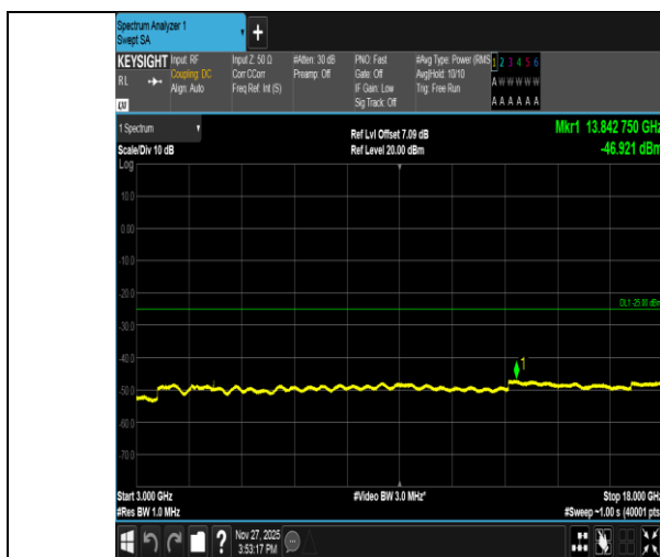
Band41-10MHz-QPSK-40620-1RB#49-3000~18000-PASS
