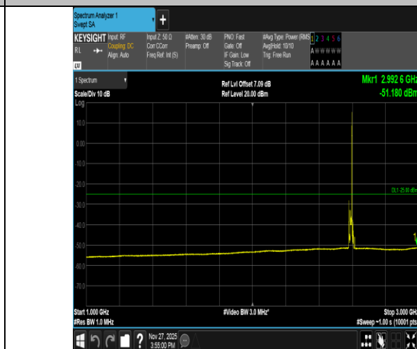
Band41-10MHz-16QAM-40620-1RB#49-1000~3000-PASS
