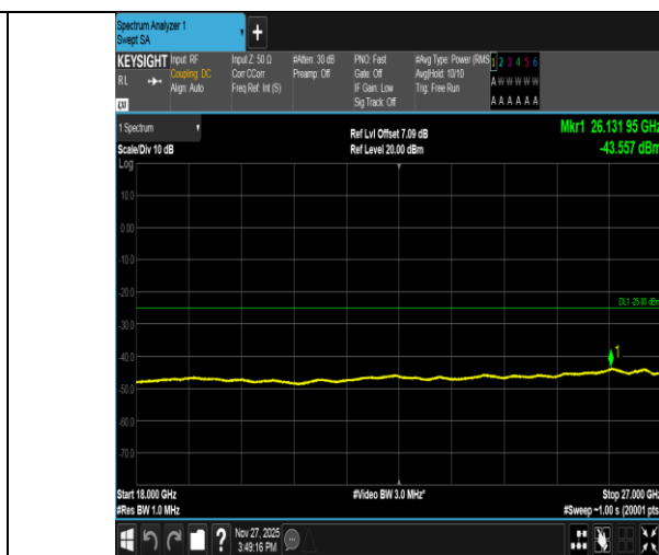
Band41-10MHz-QPSK-40620-1RB#0-18000~27000-PASS
