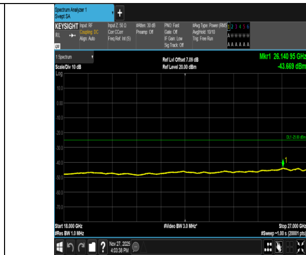
Band41-10MHz-QPSK-41540-1RB#0-18000~27000-PASS
