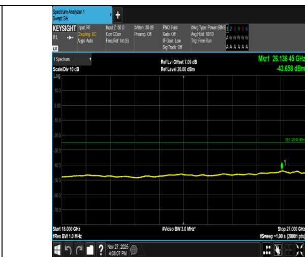
Band41-10MHz-QPSK-41540-1RB#49-18000~27000-PASS
