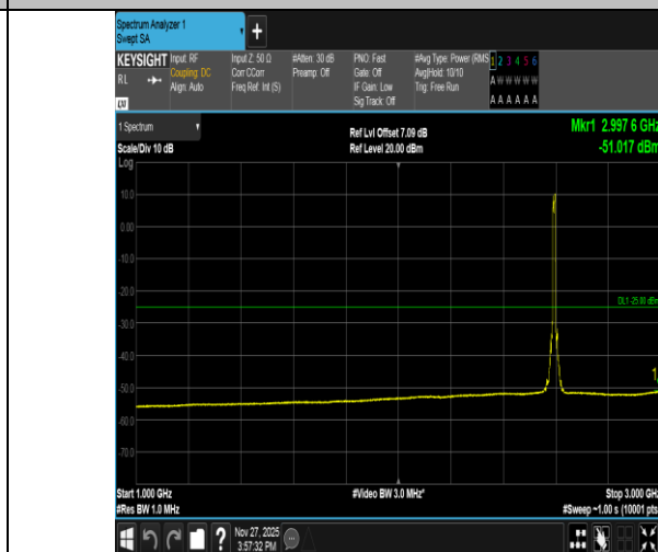
Band41-10MHz-QPSK-40620-50RB#0-1000~3000-PASS
