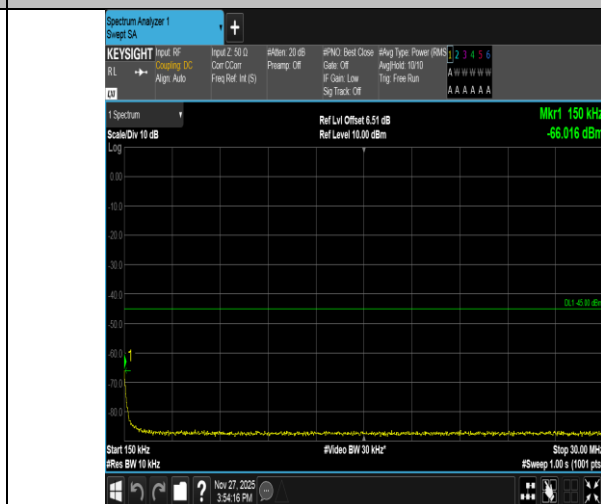
Band41-10MHz-16QAM-40620-1RB#49-0.15~30-PASS
