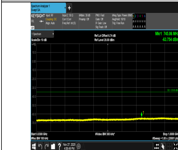
Band41-10MHz-QPSK-41540-1RB#49-30~1000-PASS
