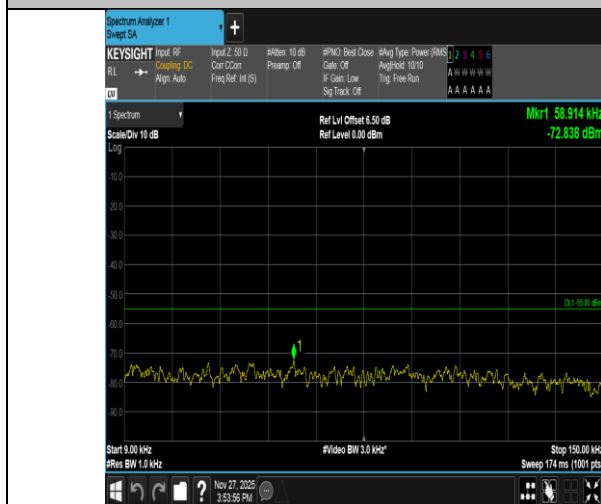
Band41-10MHz-16QAM-40620-1RB#49-0.009~0.15-PASS
