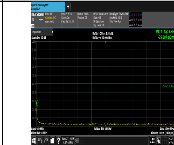
Band41-15MHz-QPSK-39725-1RB#74-0.15~30-PASS
