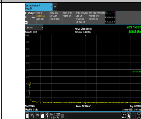
Band41-10MHz-16QAM-41540-50RB#0-0.15~30-PASS
