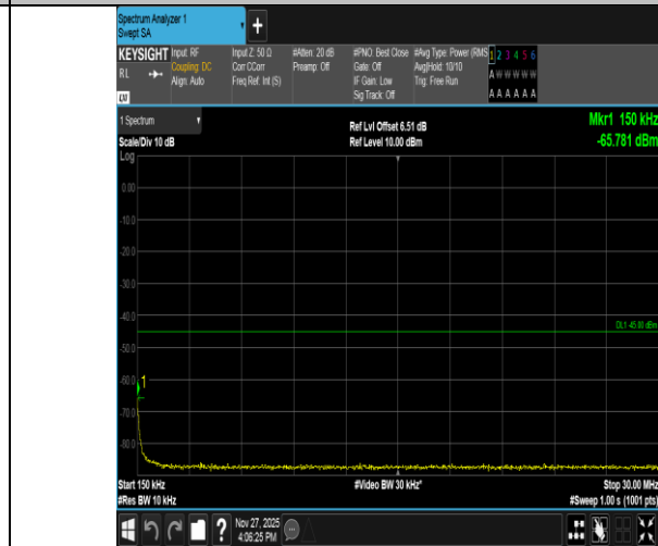
Band41-10MHz-QPSK-41540-1RB#49-0.15~30-PASS
