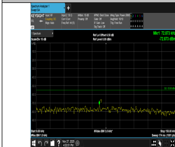
Band41-10MHz-16QAM-41540-1RB#0-0.009~0.15-PASS
