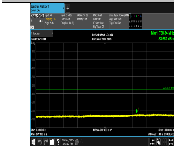
Band41-15MHz-QPSK-39725-1RB#0-30~1000-PASS
