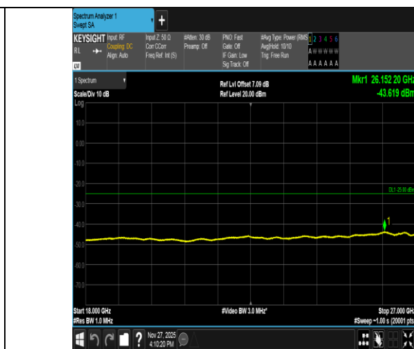
Band41-10MHz-16QAM-41540-1RB#49-18000~27000-PASS
