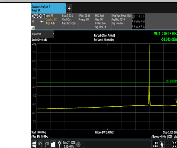
Band41-10MHz-QPSK-40620-1RB#49-1000~3000-PASS
