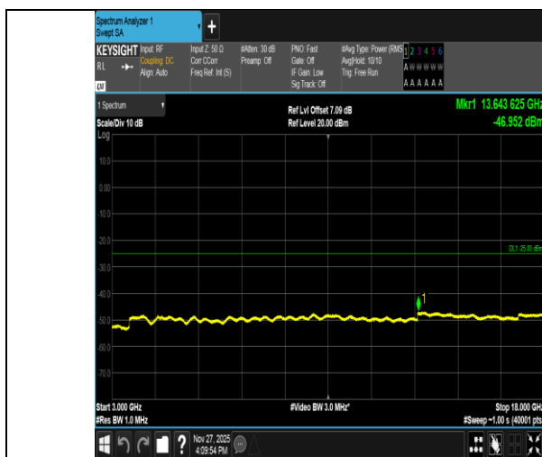
Band41-10MHz-16QAM-41540-1RB#49-3000~18000-PASS
