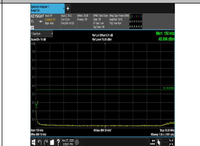
Band41-10MHz-16QAM-40620-50RB#0-0.15~30-PASS
