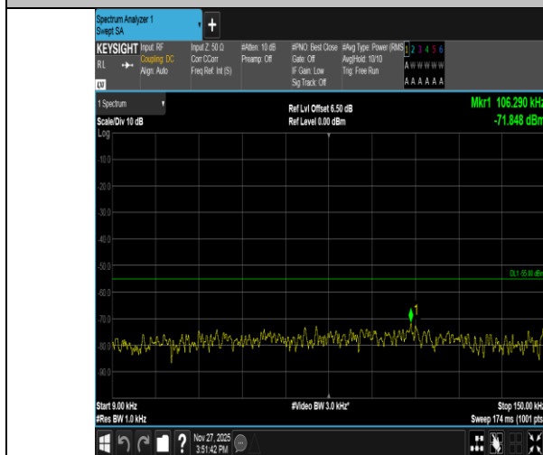
Band41-10MHz-QPSK-40620-1RB#49-0.009~0.15-PASS
