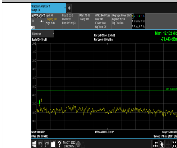
Band41-10MHz-16QAM-40620-1RB#0-0.009~0.15-PASS
