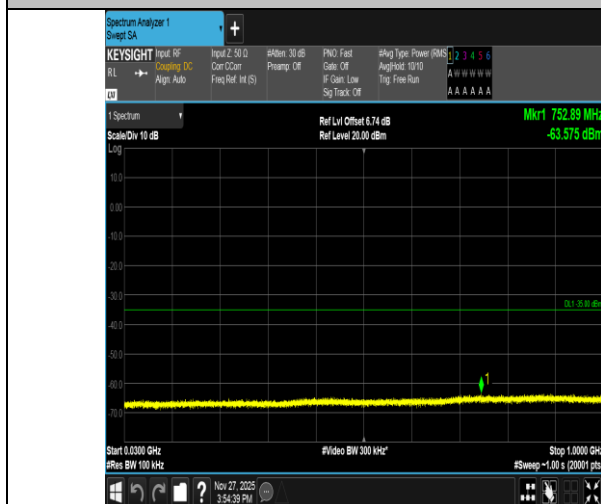
Band41-10MHz-16QAM-40620-1RB#49-30~1000-PASS
