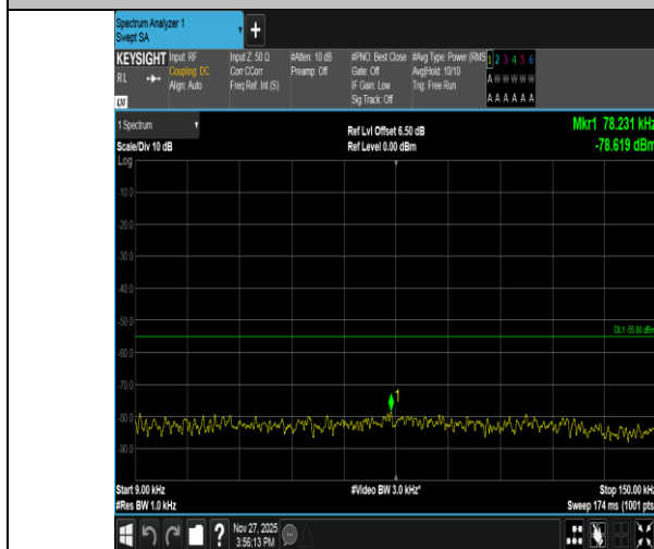
Band41-10MHz-QPSK-40620-50RB#0-0.009~0.15-PASS
