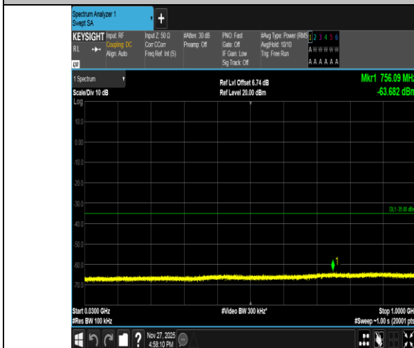
Band41-15MHz-QPSK-39725-1RB#74-30~1000-PASS
