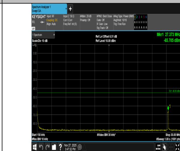
Band41-10MHz-QPSK-40620-1RB#0-0.15~30-PASS
