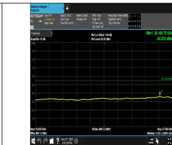
Band41-10MHz-16QAM-40620-1RB#0-18000~27000-PASS
