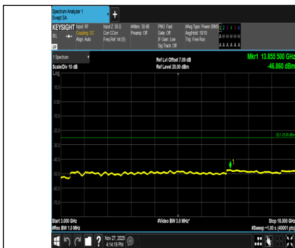
Band41-10MHz-16QAM-41540-50RB#0-3000~18000-PASS
