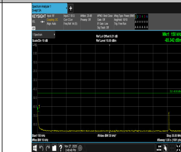
Band41-10MHz-16QAM-40620-1RB#0-0.15~30-PASS
