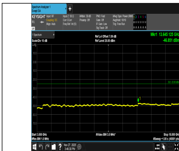
Band41-10MHz-16QAM-39700-50RB#0-3000~18000-PASS
