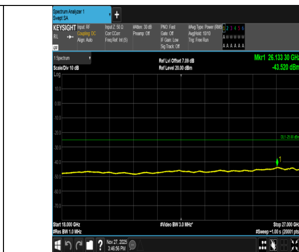
Band41-10MHz-16QAM-39700-50RB#0-18000~27000-PASS
