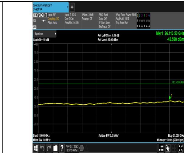
Band41-10MHz-16QAM-39700-1RB#0-18000~27000-PASS
