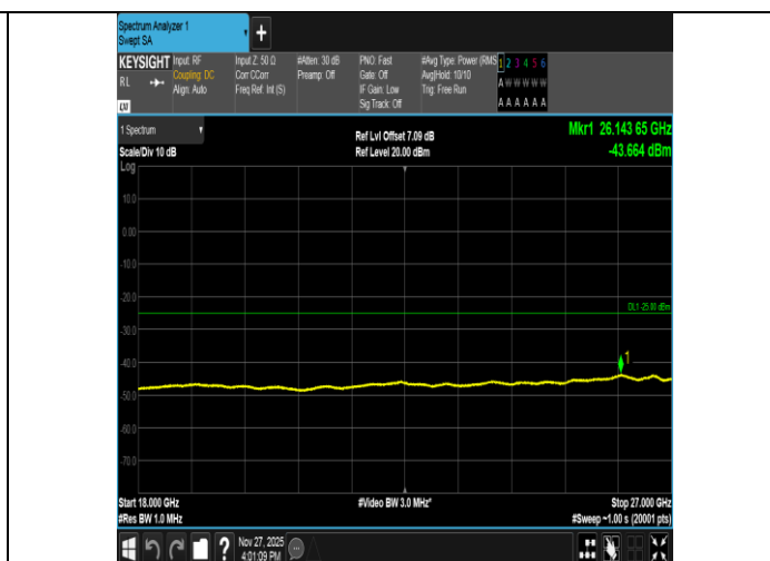
Band41-10MHz-16QAM-40620-50RB#0-18000~27000-PASS
