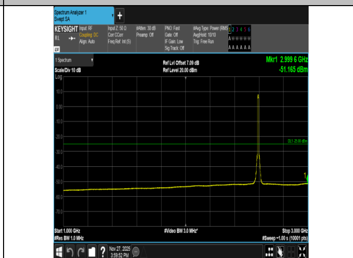
Band41-10MHz-16QAM-40620-50RB#0-1000~3000-PASS
