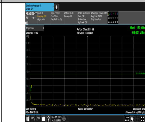
Band41-15MHz-QPSK-39725-1RB#0-0.15~30-PASS
