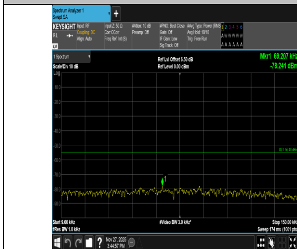
Band41-10MHz-16QAM-39700-50RB#0-0.009~0.15-PASS
