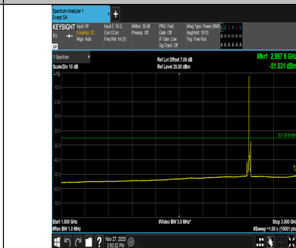
Band41-10MHz-16QAM-40620-1RB#0-1000~3000-PASS
