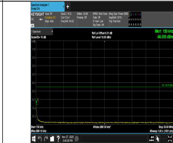
Band41-10MHz-16QAM-39700-1RB#49-0.15~30-PASS
