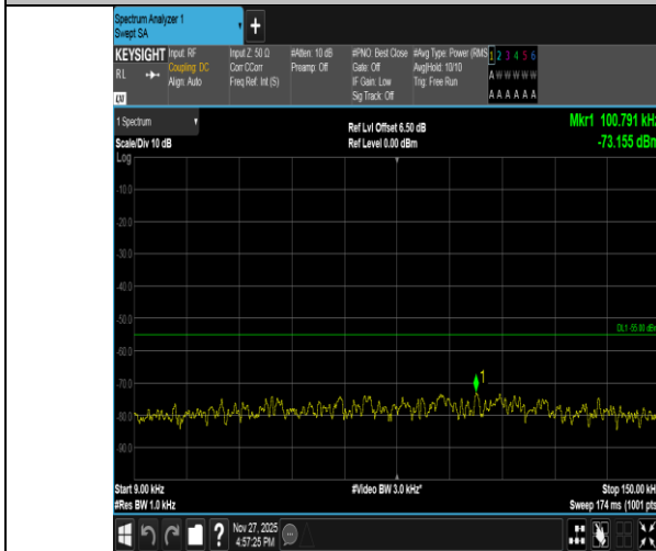
Band41-15MHz-QPSK-39725-1RB#74-0.009~0.15-PASS
