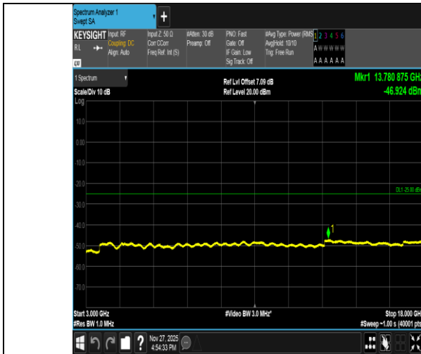
Band41-15MHz-QPSK-39725-1RB#0-3000~18000-PASS
