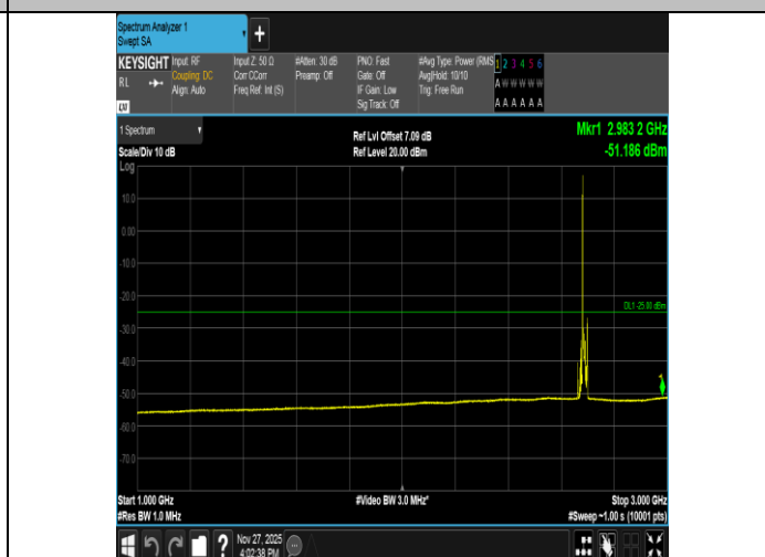
Band41-10MHz-QPSK-41540-1RB#0-1000~3000-PASS
