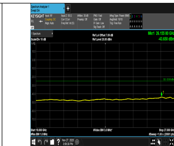
Band41-10MHz-QPSK-40620-50RB#0-18000~27000-PASS
