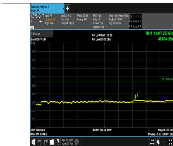
Band41-15MHz-16QAM-40620-1RB#74-3000~18000-PASS
