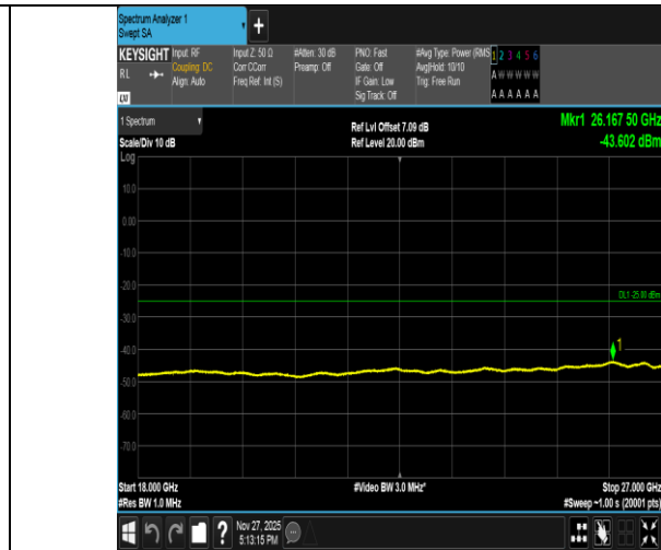
Band41-15MHz-QPSK-40620-1RB#74-18000~27000-PASS
