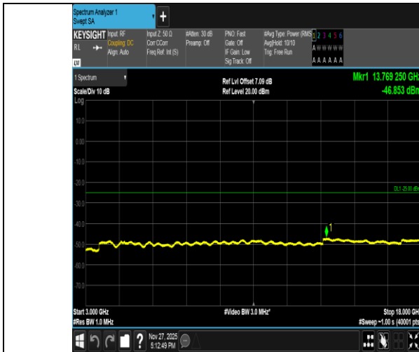
Band41-15MHz-QPSK-40620-1RB#74-3000~18000-PASS
