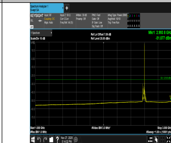
Band41-15MHz-16QAM-40620-1RB#74-1000~3000-PASS
