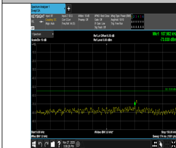
Band41-15MHz-QPSK-40620-1RB#0-0.009~0.15-PASS
