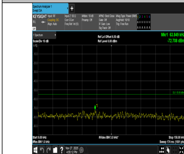
Band41-15MHz-16QAM-39725-1RB#0-0.009~0.15-PASS
