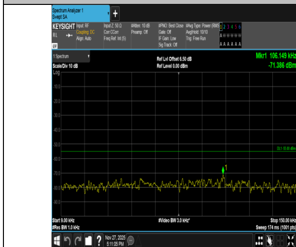
Band41-15MHz-QPSK-40620-1RB#74-0.009~0.15-PASS
