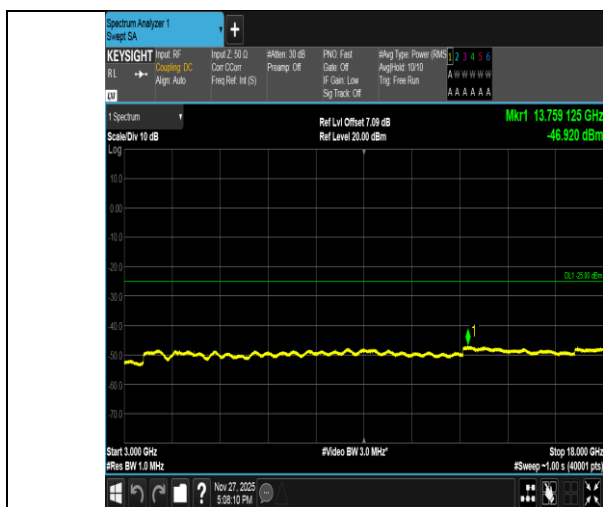
Band41-15MHz-QPSK-40620-1RB#0-3000~18000-PASS
