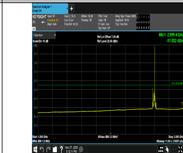
Band41-15MHz-QPSK-40620-1RB#74-1000~3000-PASS
