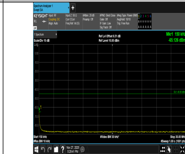
Band41-15MHz-16QAM-41515-1RB#74-0.15~30-PASS
