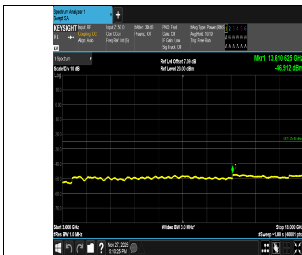
Band41-15MHz-16QAM-40620-1RB#0-3000~18000-PASS
