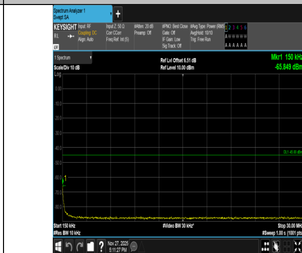
Band41-15MHz-QPSK-40620-1RB#74-0.15~30-PASS
