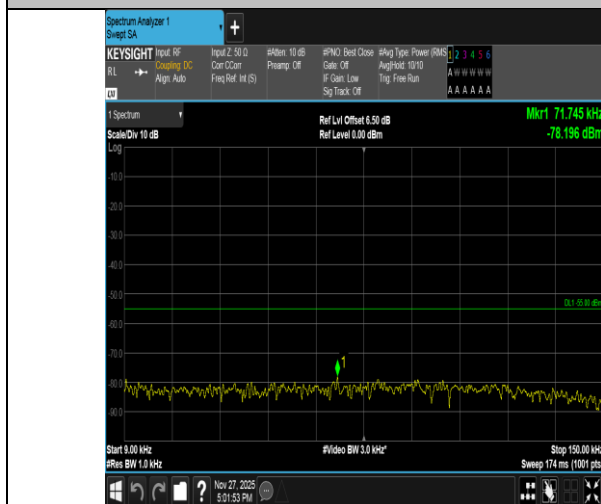
Band41-15MHz-QPSK-39725-75RB#0-0.009~0.15-PASS
