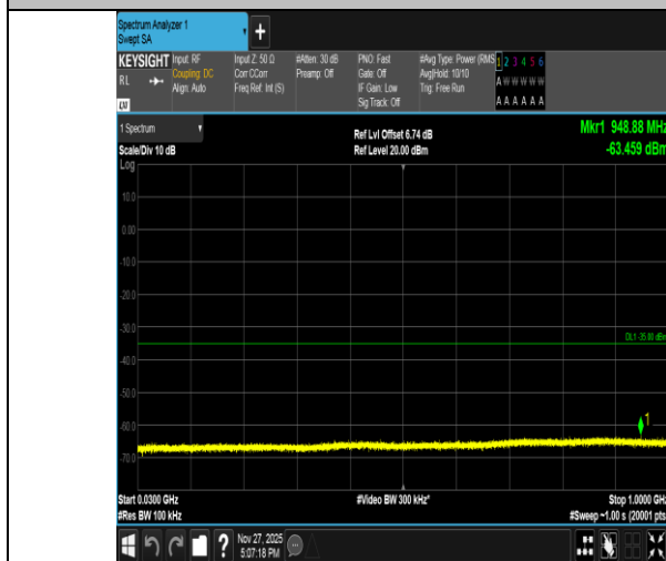
Band41-15MHz-QPSK-40620-1RB#0-30~1000-PASS
