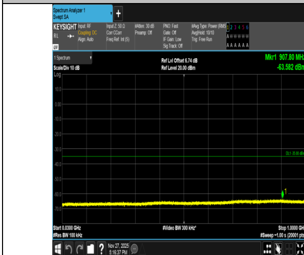
Band41-15MHz-QPSK-40620-75RB#0-30~1000-PASS
