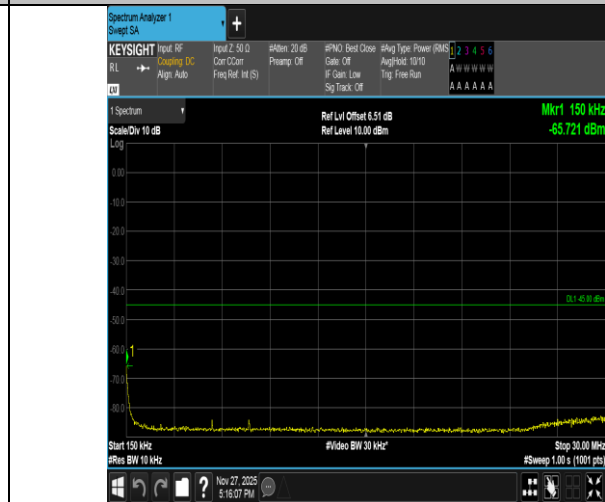
Band41-15MHz-QPSK-40620-75RB#0-0.15~30-PASS
