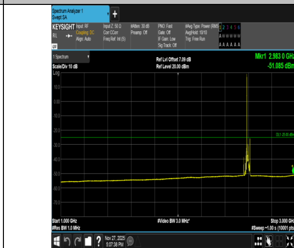
Band41-15MHz-QPSK-40620-1RB#0-1000~3000-PASS
