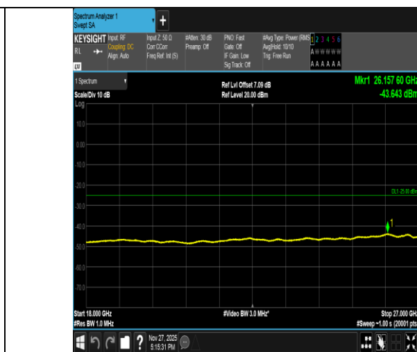
Band41-15MHz-16QAM-40620-1RB#74-18000~27000-PASS
