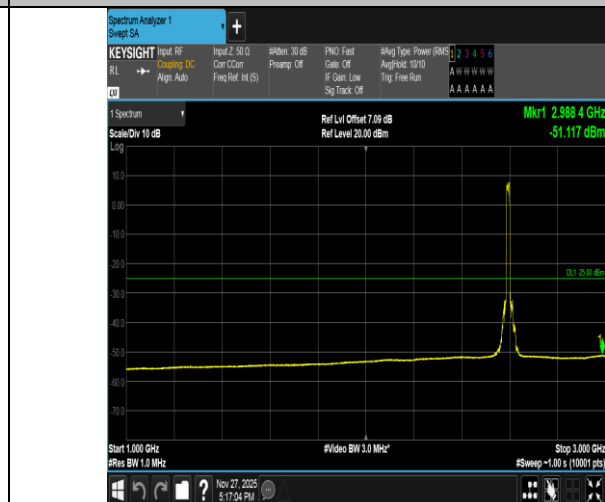
Band41-15MHz-QPSK-40620-75RB#0-1000~3000-PASS
