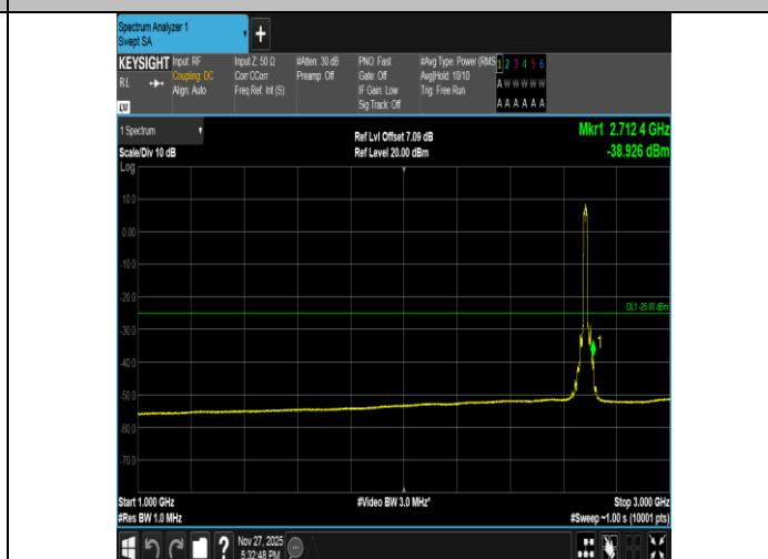
Band41-15MHz-QPSK-41515-75RB#0-1000~3000-PASS
