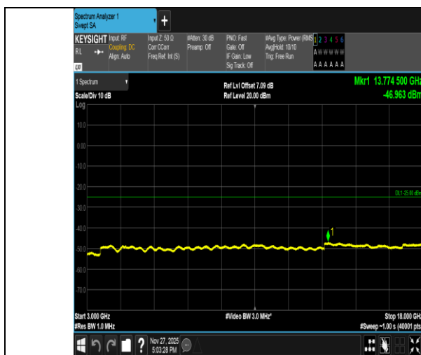
Band41-15MHz-QPSK-39725-75RB#0-3000~18000-PASS
