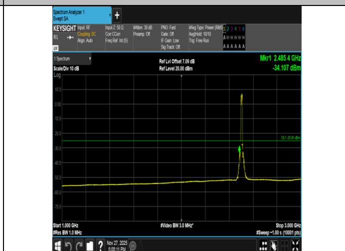
Band41-15MHz-16QAM-39725-75RB#0-1000~3000-PASS
