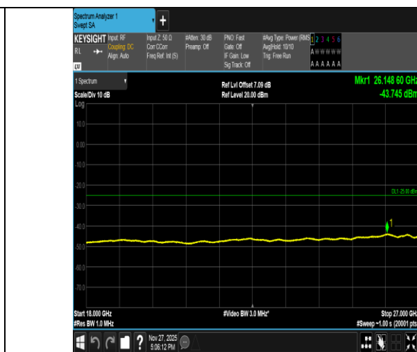
Band41-15MHz-16QAM-39725-75RB#0-18000~27000-PASS
