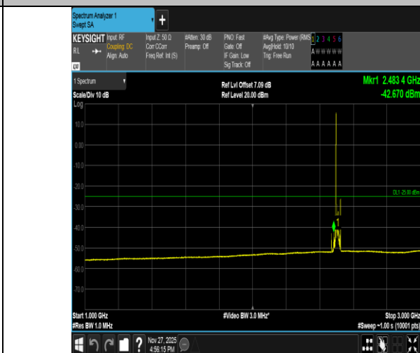
Band41-15MHz-16QAM-39725-1RB#0-1000~3000-PASS
