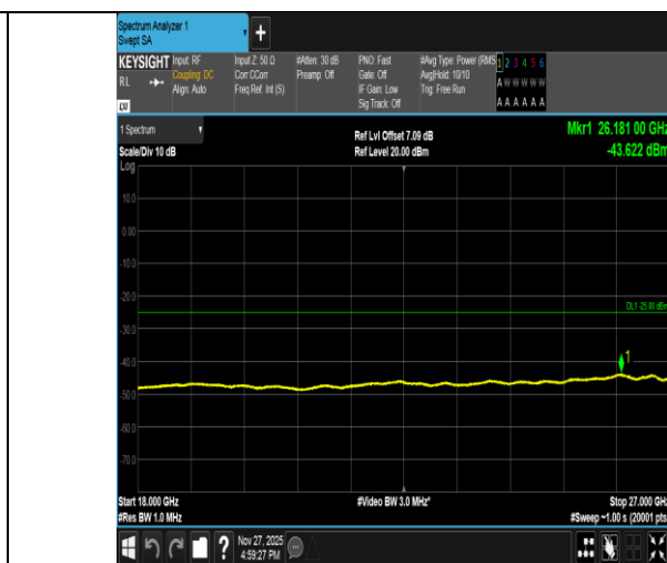
Band41-15MHz-QPSK-39725-1RB#74-18000~27000-PASS
