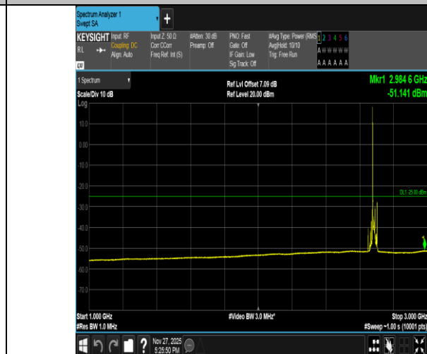
Band41-15MHz-16QAM-41515-1RB#0-1000~3000-PASS
