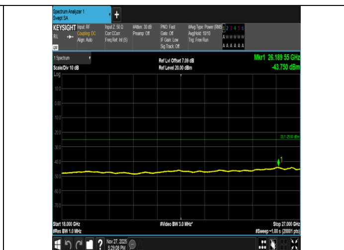
Band41-15MHz-QPSK-41515-1RB#74-18000~27000-PASS
