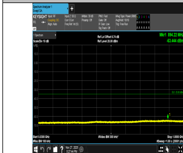
Band41-15MHz-QPSK-41515-1RB#74-30~1000-PASS
