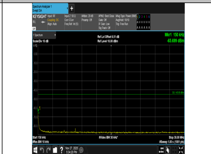
Band41-15MHz-16QAM-41515-75RB#0-0.15~30-PASS
