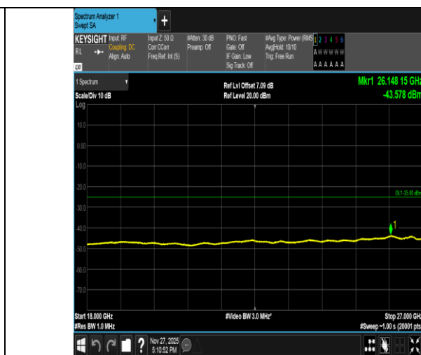
Band41-15MHz-16QAM-40620-1RB#0-18000~27000-PASS
