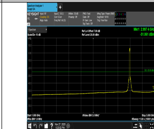
Band41-15MHz-16QAM-40620-75RB#0-1000~3000-PASS
