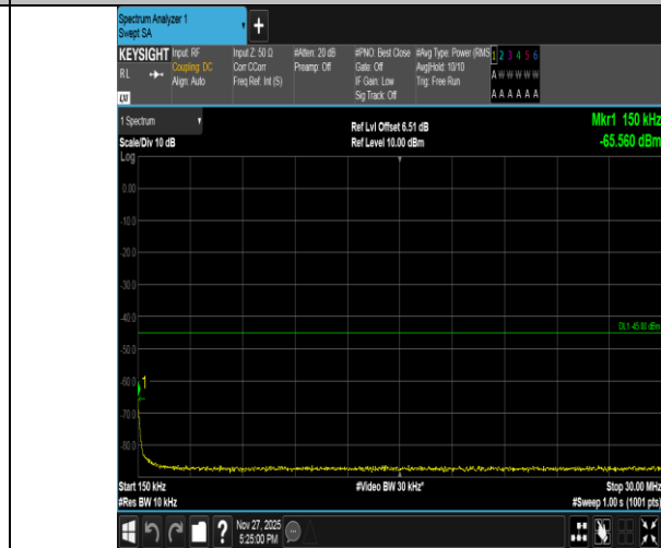
Band41-15MHz-16QAM-41515-1RB#0-0.15~30-PASS
