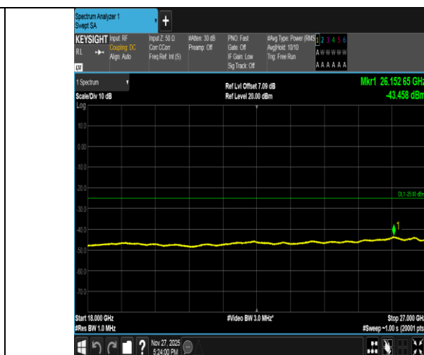
Band41-15MHz-QPSK-41515-1RB#0-18000~27000-PASS
