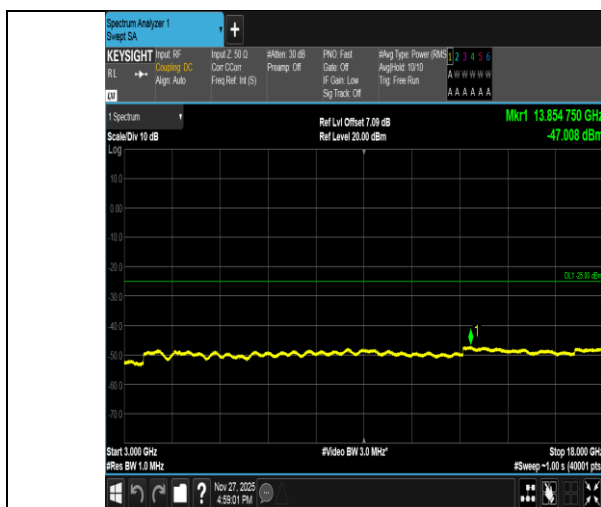
Band41-15MHz-QPSK-39725-1RB#74-3000~18000-PASS
