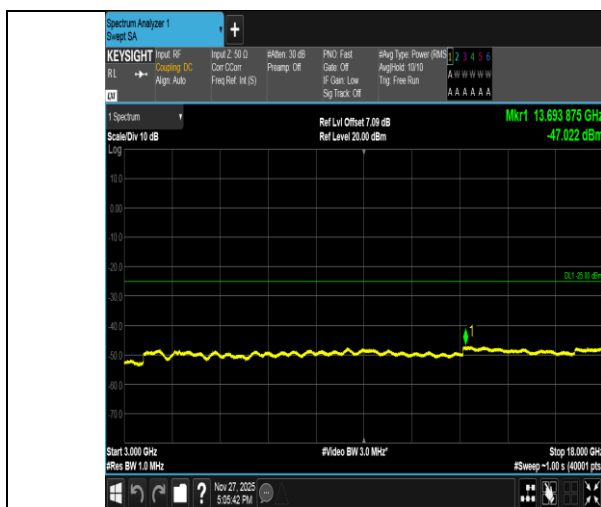
Band41-15MHz-16QAM-39725-75RB#0-3000~18000-PASS
