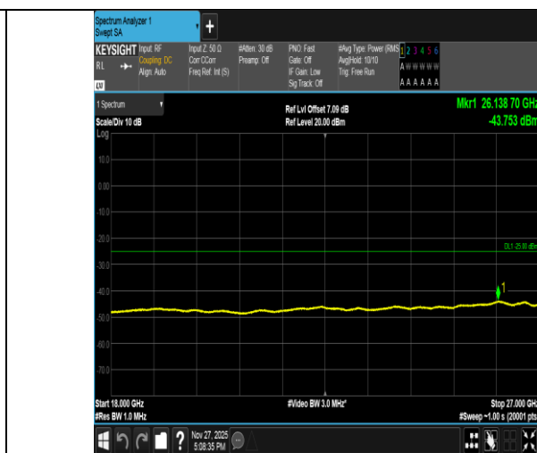
Band41-15MHz-QPSK-40620-1RB#0-18000~27000-PASS
