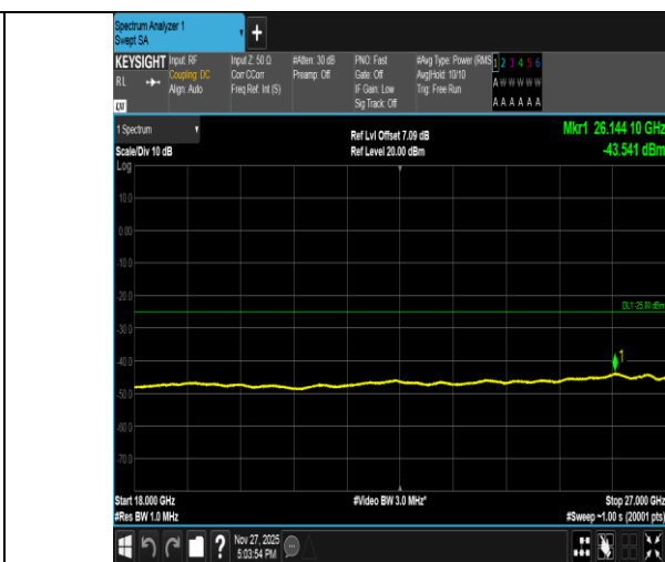
Band41-15MHz-QPSK-39725-75RB#0-18000~27000-PASS
