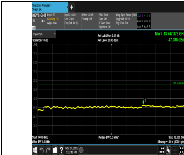
Band41-15MHz-QPSK-41515-75RB#0-3000~18000-PASS
