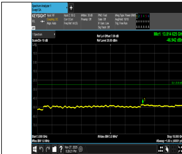
Band41-15MHz-16QAM-41515-1RB#0-3000~18000-PASS
