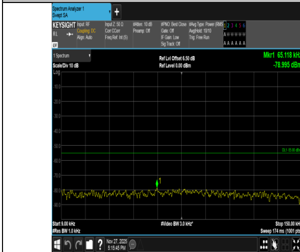
Band41-15MHz-QPSK-40620-75RB#0-0.009~0.15-PASS
