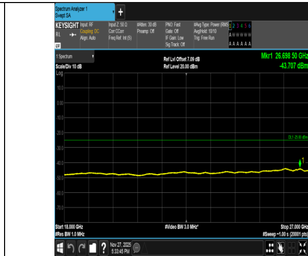
Band41-15MHz-QPSK-41515-75RB#0-18000~27000-PASS
