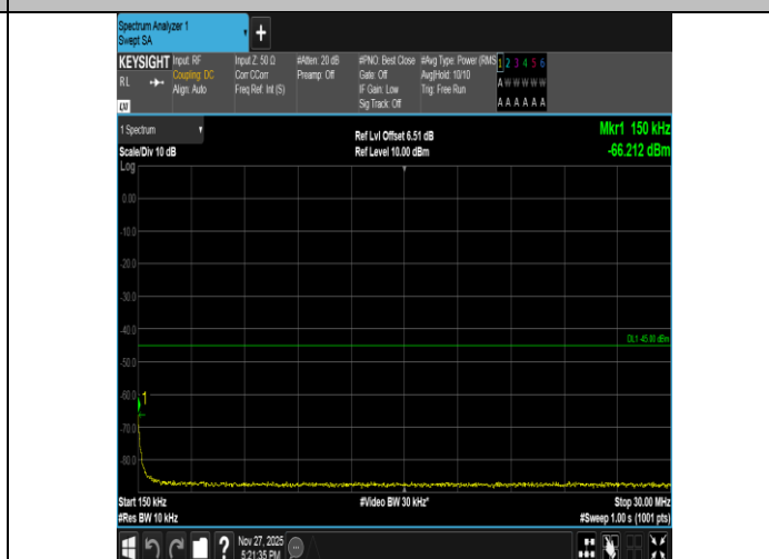
Band41-15MHz-QPSK-41515-1RB#0-0.15~30-PASS
