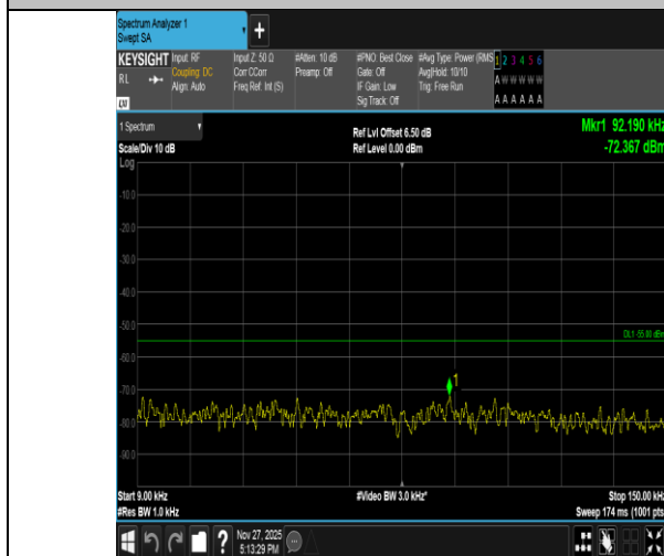
Band41-15MHz-16QAM-40620-1RB#74-0.009~0.15-PASS
