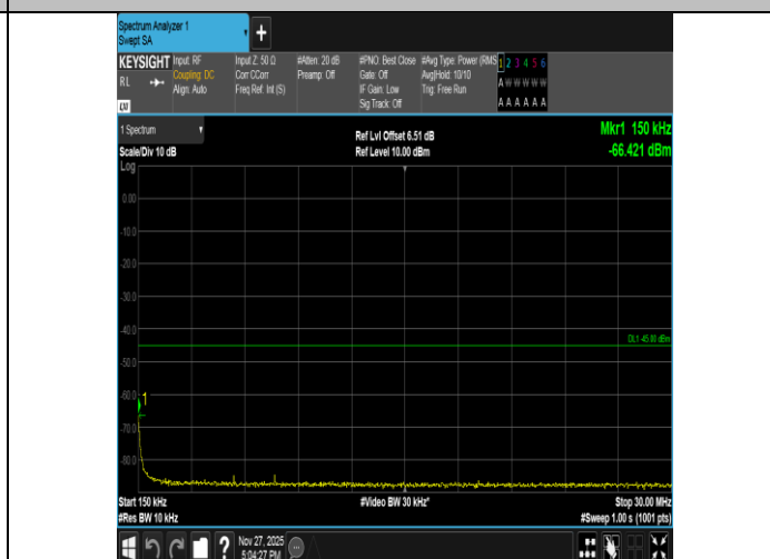
Band41-15MHz-16QAM-39725-75RB#0-0.15~30-PASS
