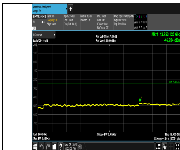
Band41-15MHz-QPSK-41515-1RB#0-3000~18000-PASS
