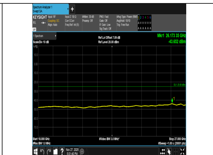
Band41-15MHz-16QAM-39725-1RB#74-18000~27000-PASS
