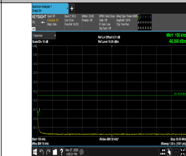
Band41-15MHz-16QAM-39725-1RB#0-0.15~30-PASS
