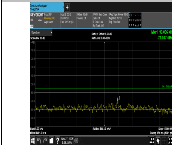
Band41-15MHz-16QAM-41515-1RB#74-0.009~0.15-PASS
