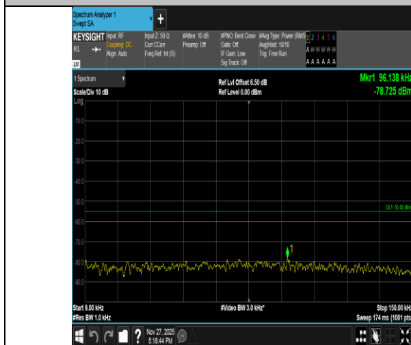
Band41-15MHz-16QAM-40620-75RB#0-0.009~0.15-PASS
