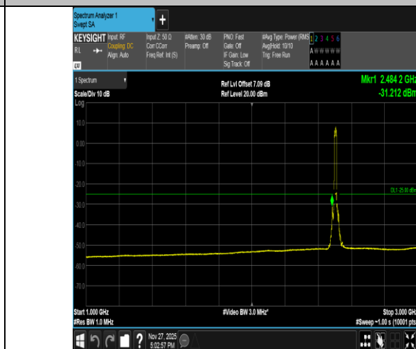
Band41-15MHz-QPSK-39725-75RB#0-1000~3000-PASS
