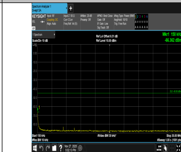
Band41-15MHz-QPSK-39725-75RB#0-0.15~30-PASS
