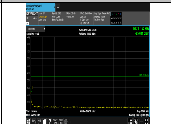
Band41-15MHz-QPSK-41515-75RB#0-0.15~30-PASS
