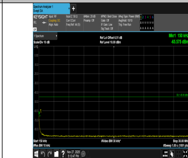
Band41-15MHz-16QAM-40620-1RB#74-0.15~30-PASS
