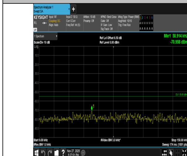
Band41-15MHz-QPSK-41515-1RB#74-0.009~0.15-PASS
