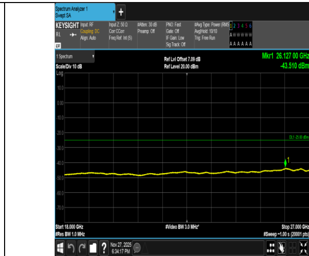
Band41-20MHz-16QAM-40620-1RB#0-18000~27000-PASS
