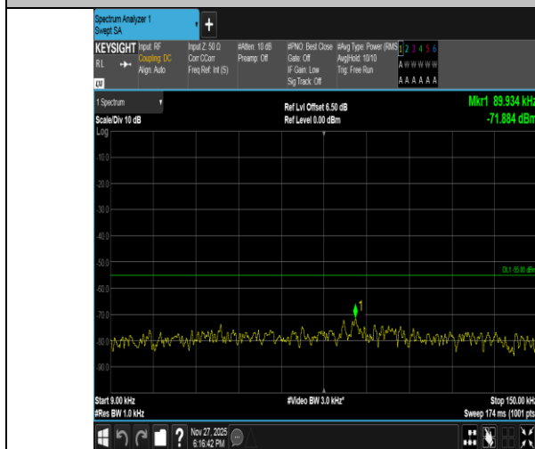
Band41-20MHz-QPSK-39750-1RB#0-0.009~0.15-PASS
