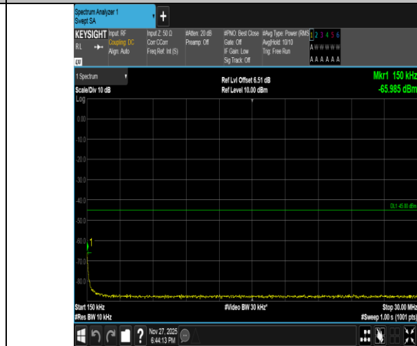
Band41-20MHz-QPSK-41490-1RB#0-0.15~30-PASS
