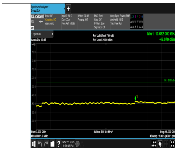
Band41-20MHz-QPSK-40620-1RB#0-3000~18000-PASS
