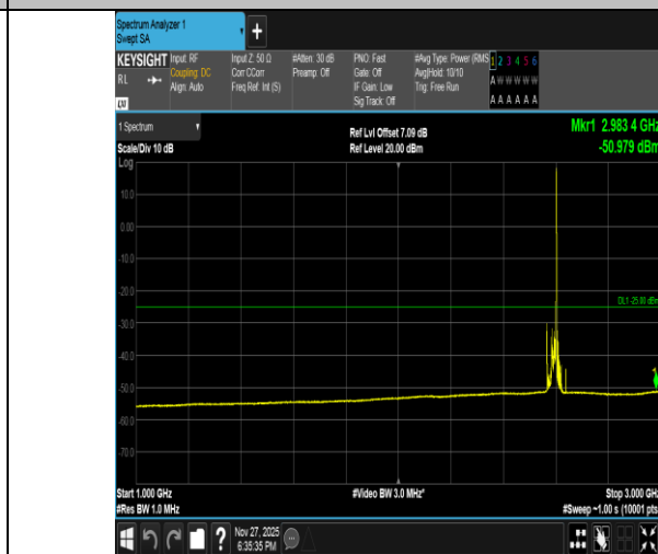
Band41-20MHz-QPSK-40620-1RB#99-1000~3000-PASS
