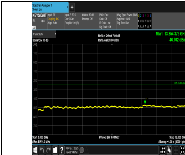
Band41-20MHz-16QAM-40620-100RB#0-3000~18000-PASS
