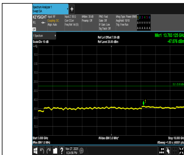
Band41-20MHz-16QAM-39750-1RB#99-3000~18000-PASS
