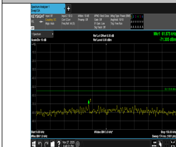
Band41-20MHz-QPSK-41490-1RB#99-0.009~0.15-PASS
