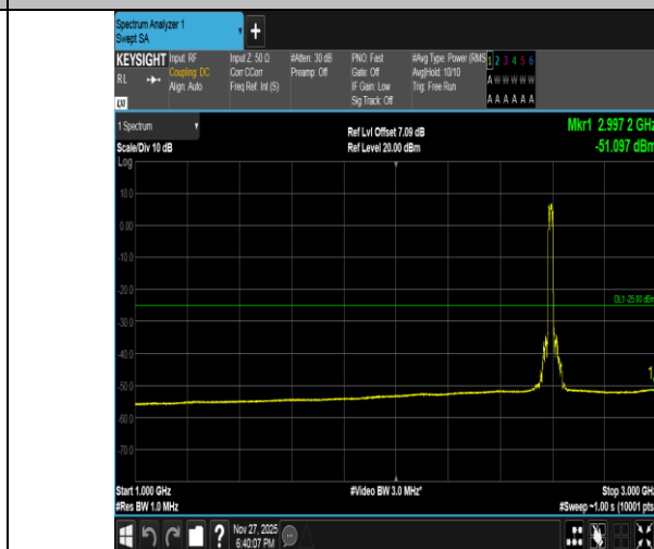
Band41-20MHz-QPSK-40620-100RB#0-1000~3000-PASS
