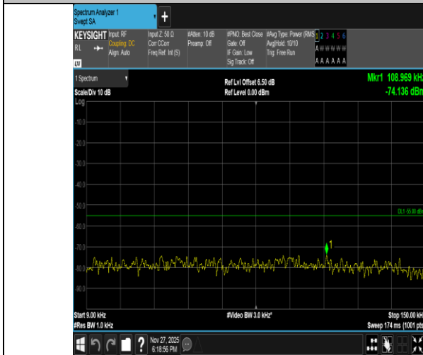
Band41-20MHz-16QAM-39750-1RB#0-0.009~0.15-PASS
