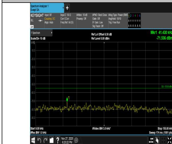
Band41-20MHz-16QAM-39750-1RB#99-0.009~0.15-PASS
