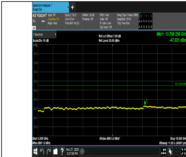
Band41-20MHz-QPSK-39750-100RB#0-3000~18000-PASS
