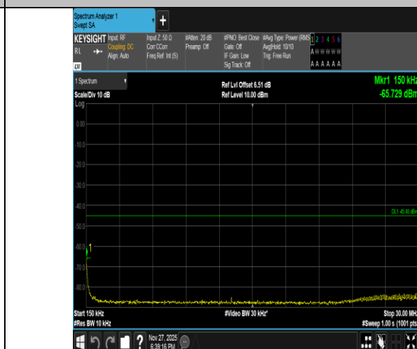
Band41-20MHz-QPSK-40620-100RB#0-0.15~30-PASS
