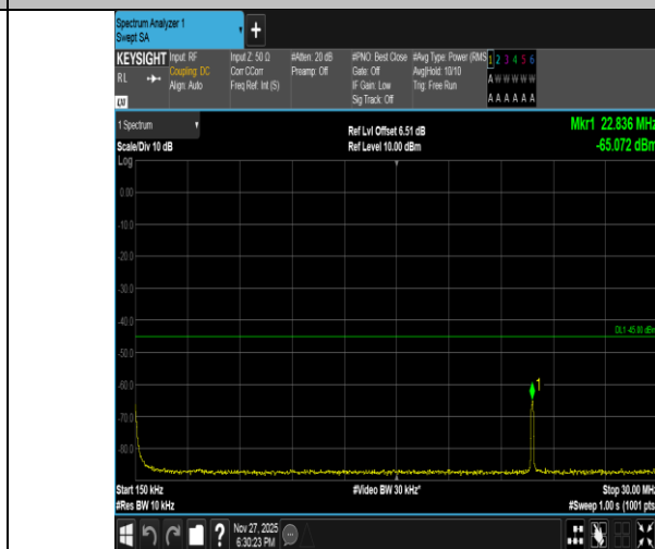
Band41-20MHz-QPSK-40620-1RB#0-0.15~30-PASS
