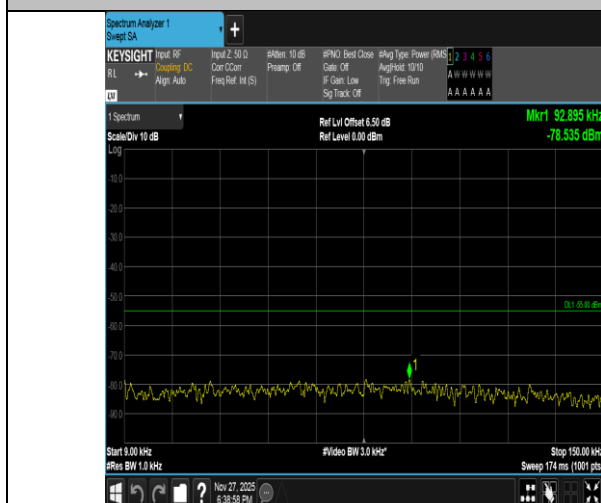
Band41-20MHz-QPSK-40620-100RB#0-0.009~0.15-PASS
