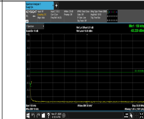
Band41-20MHz-16QAM-39750-1RB#0-0.15~30-PASS
