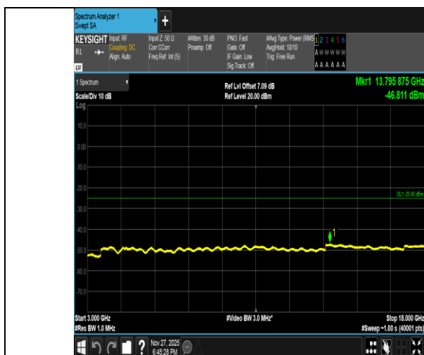
Band41-20MHz-QPSK-41490-1RB#0-3000~18000-PASS
