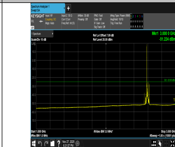
Band41-20MHz-QPSK-40620-1RB#0-1000~3000-PASS
