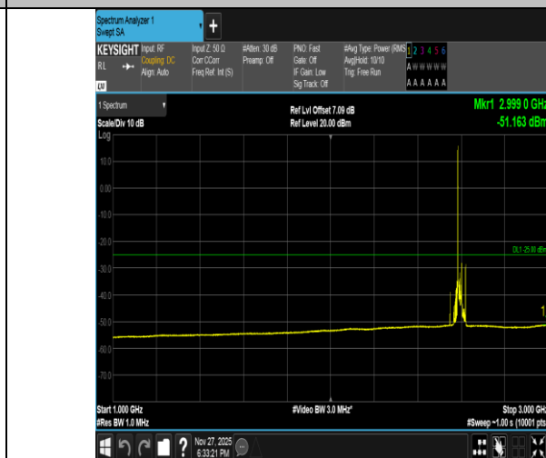
Band41-20MHz-16QAM-40620-1RB#0-1000~3000-PASS
