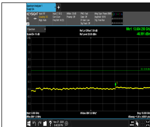
Band41-20MHz-QPSK-40620-100RB#0-3000~18000-PASS
