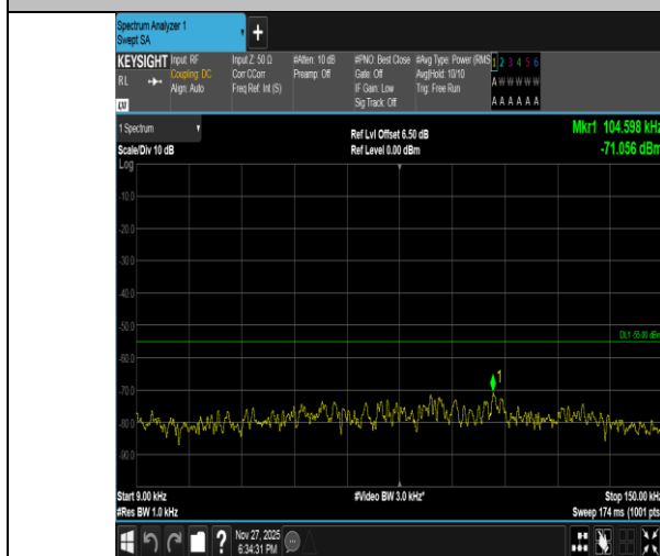
Band41-20MHz-QPSK-40620-1RB#99-0.009~0.15-PASS
