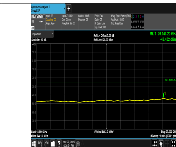
Band41-20MHz-QPSK-40620-1RB#99-18000~27000-PASS
