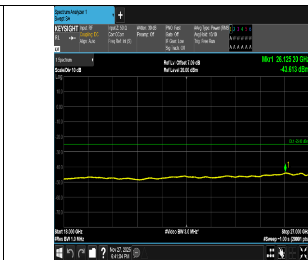
Band41-20MHz-QPSK-40620-100RB#0-18000~27000-PASS
