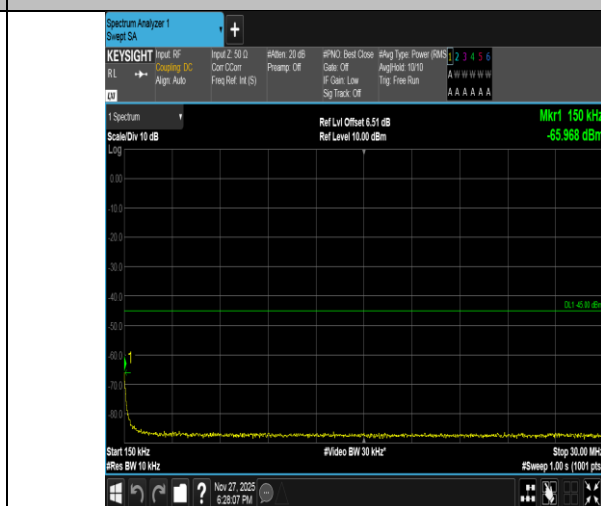
Band41-20MHz-16QAM-39750-100RB#0-0.15~30-PASS
