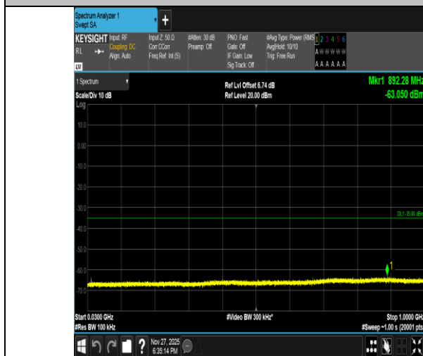
Band41-20MHz-QPSK-40620-1RB#99-30~1000-PASS
