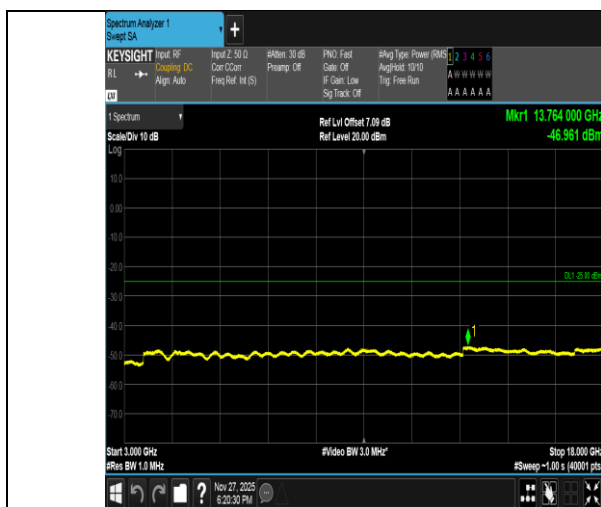
Band41-20MHz-16QAM-39750-1RB#0-3000~18000-PASS
