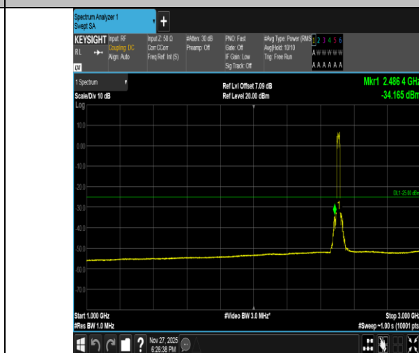
Band41-20MHz-QPSK-39750-100RB#0-1000~3000-PASS
