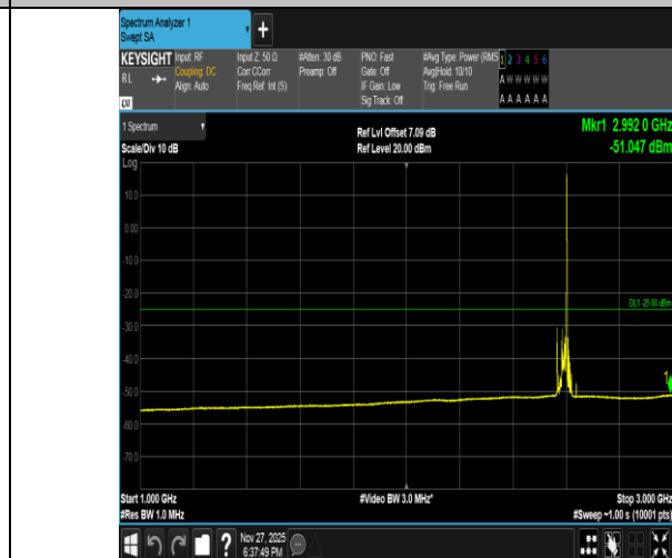
Band41-20MHz-16QAM-40620-1RB#99-1000~3000-PASS
