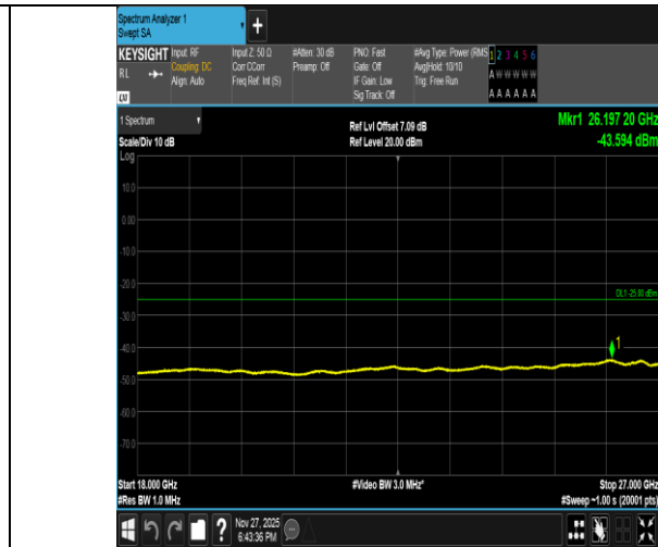
Band41-20MHz-16QAM-40620-100RB#0-18000~27000-PASS
