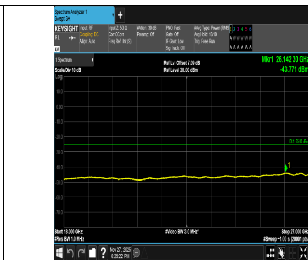
Band41-20MHz-16QAM-39750-1RB#99-18000~27000-PASS
