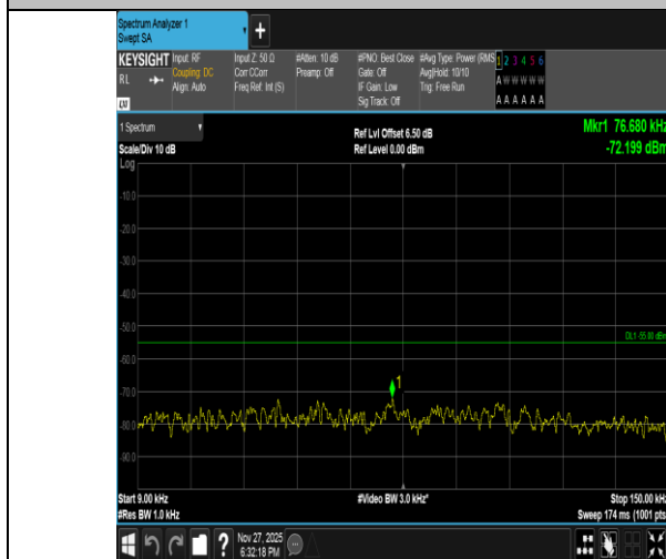
Band41-20MHz-16QAM-40620-1RB#0-0.009~0.15-PASS
