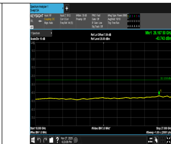
Band41-20MHz-QPSK-39750-1RB#99-18000~27000-PASS
