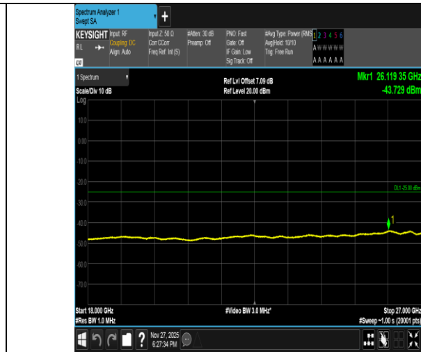
Band41-20MHz-QPSK-39750-100RB#0-18000~27000-PASS
