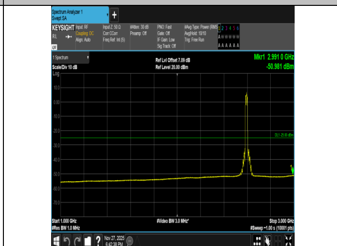
Band41-20MHz-16QAM-40620-100RB#0-1000~3000-PASS
