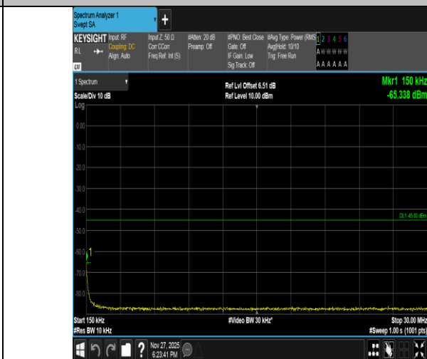
Band41-20MHz-16QAM-39750-1RB#99-0.15~30-PASS
