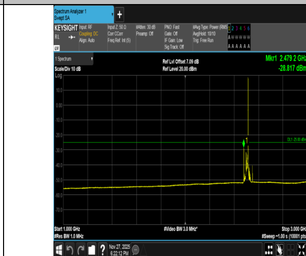
Band41-20MHz-QPSK-39750-1RB#99-1000~3000-PASS
