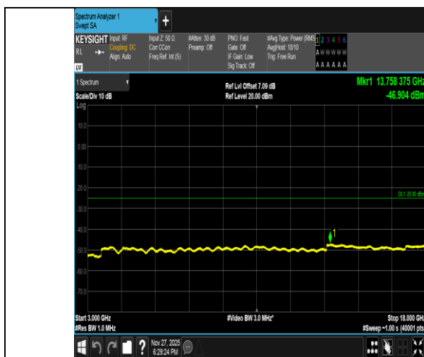
Band41-20MHz-16QAM-39750-100RB#0-3000~18000-PASS
