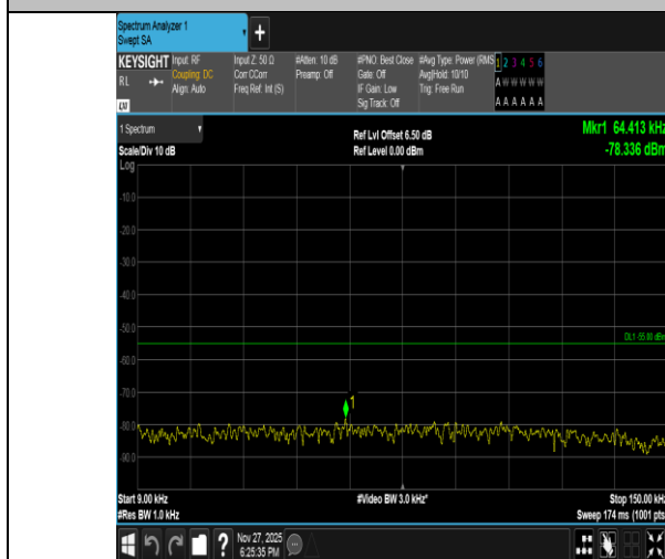
Band41-20MHz-QPSK-39750-100RB#0-0.009~0.15-PASS
