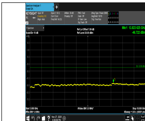
Band41-20MHz-QPSK-40620-1RB#99-3000~18000-PASS
