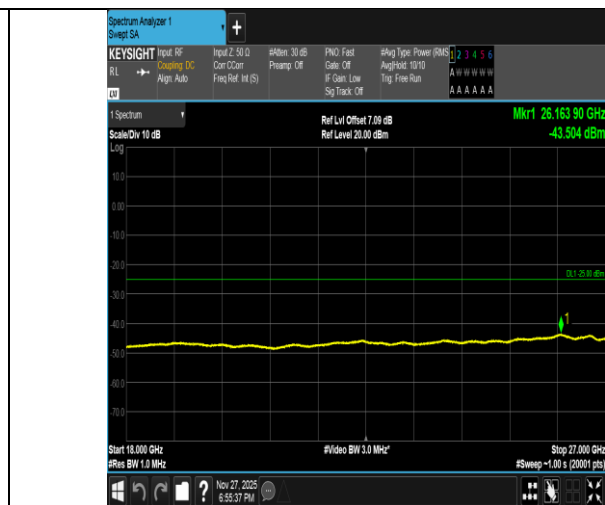
Band41-20MHz-QPSK-41490-100RB#0-18000~27000-PASS
