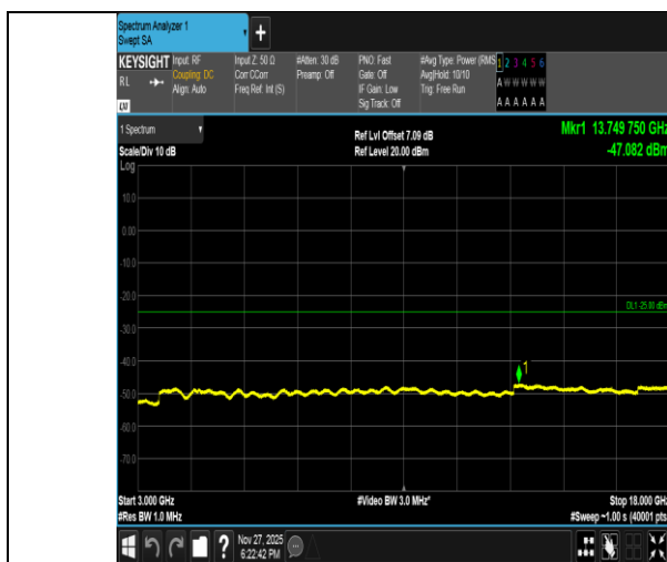
Band41-20MHz-QPSK-39750-1RB#99-3000~18000-PASS
