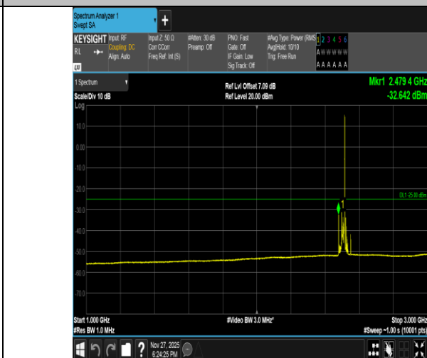
Band41-20MHz-16QAM-39750-1RB#99-1000~3000-PASS
