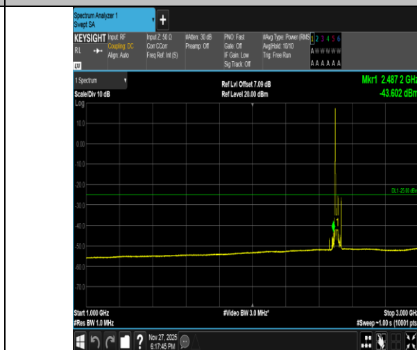
Band41-20MHz-QPSK-39750-1RB#0-1000~3000-PASS
