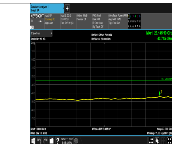
Band41-20MHz-QPSK-39750-1RB#0-18000~27000-PASS
