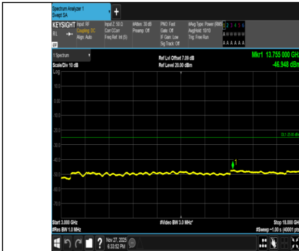
Band41-20MHz-16QAM-40620-1RB#0-3000~18000-PASS
