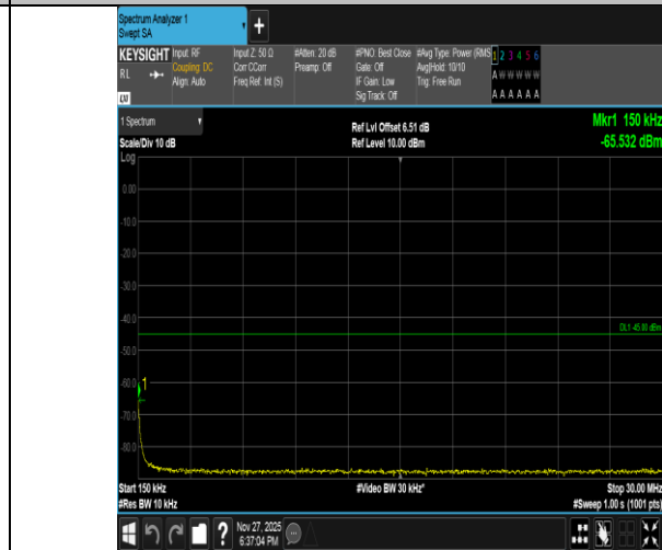
Band41-20MHz-16QAM-40620-1RB#99-0.15~30-PASS
