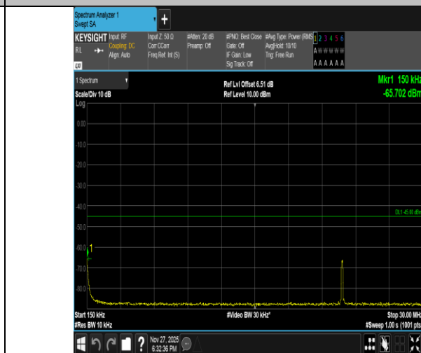
Band41-20MHz-16QAM-40620-1RB#0-0.15~30-PASS
