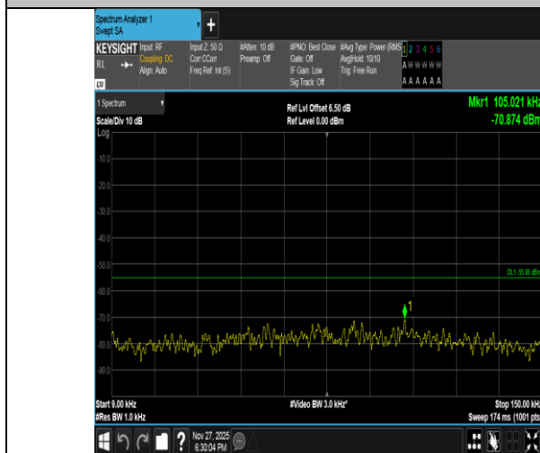
Band41-20MHz-QPSK-40620-1RB#0-0.009~0.15-PASS
