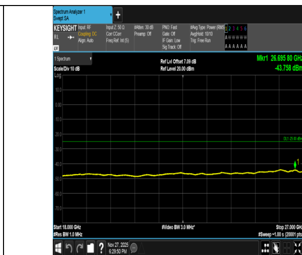
Band41-20MHz-16QAM-39750-100RB#0-18000~27000-PASS
