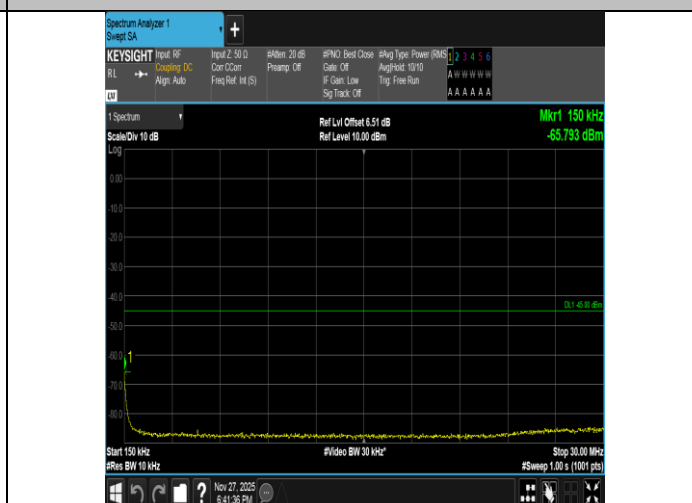
Band41-20MHz-16QAM-40620-100RB#0-0.15~30-PASS
