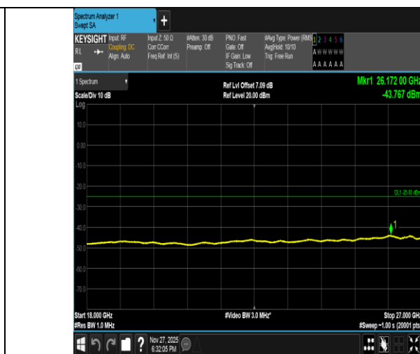
Band41-20MHz-QPSK-40620-1RB#0-18000~27000-PASS
