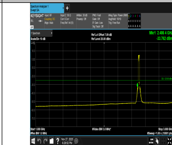
Band41-20MHz-16QAM-39750-100RB#0-1000~3000-PASS
