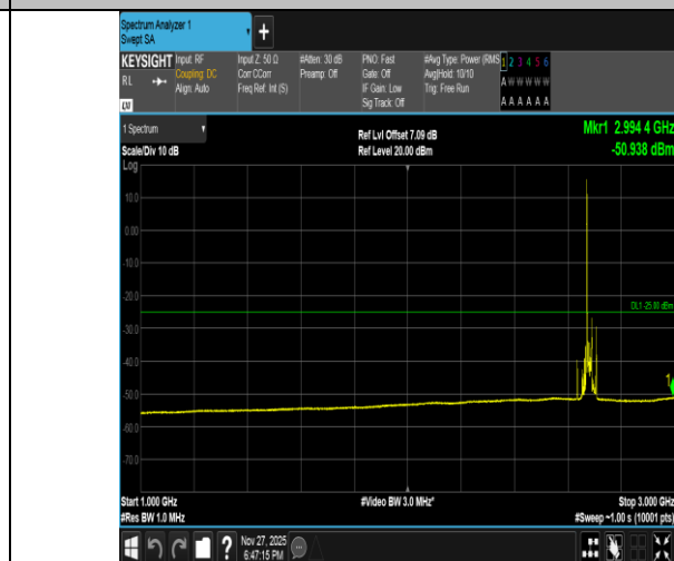
Band41-20MHz-16QAM-41490-1RB#0-1000~3000-PASS
