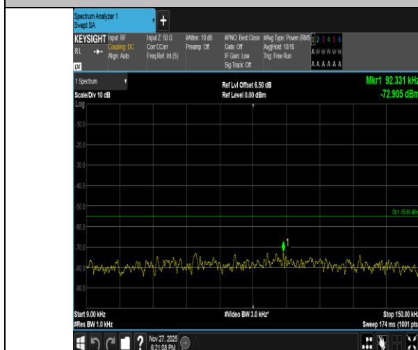
Band41-20MHz-QPSK-39750-1RB#99-0.009~0.15-PASS
