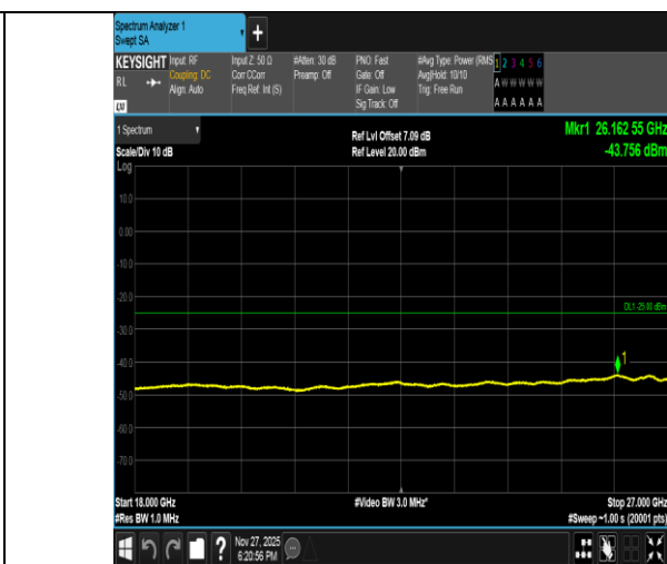
Band41-20MHz-16QAM-39750-1RB#0-18000~27000-PASS
