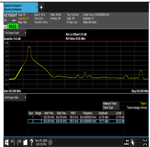
Band5-10MHz-16QAM-20450-1RB#0-PASS
