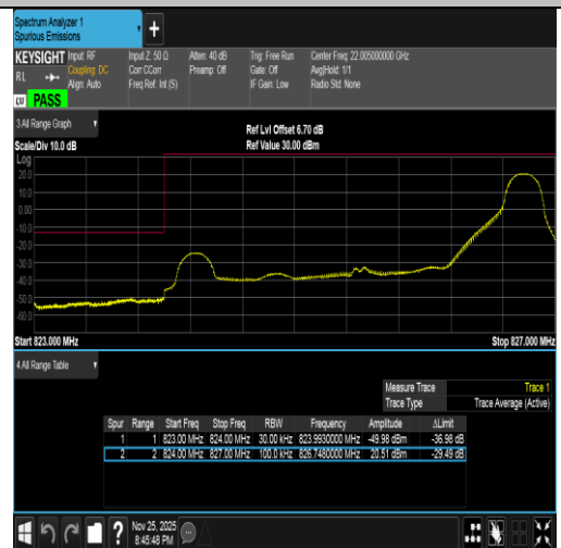
Band5-3MHz-QPSK-20415-1RB#14-PASS
