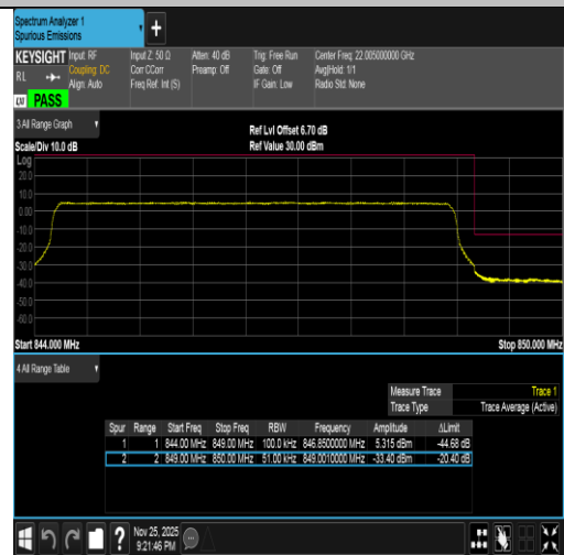
Band5-5MHz-16QAM-20625-25RB#0-PASS
