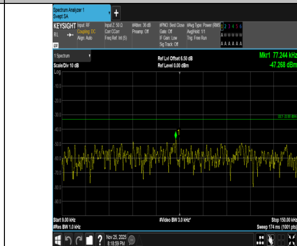
Band5-1.4MHz-16QAM-20407-6RB#0-0.009~0.15-PASS
