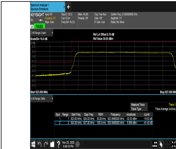
Band5-3MHz-QPSK-20415-15RB#0-PASS
