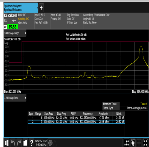
Band5-10MHz-QPSK-20450-1RB#49-PASS
