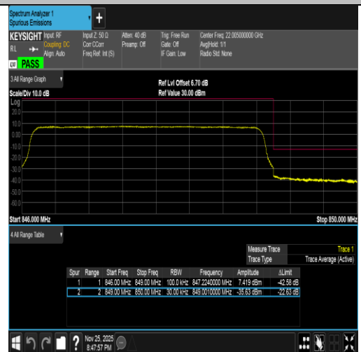
Band5-3MHz-16QAM-20635-15RB#0-PASS
