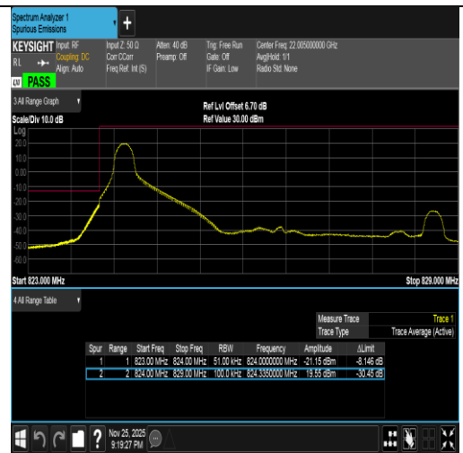
Band5-5MHz-16QAM-20425-1RB#0-PASS
