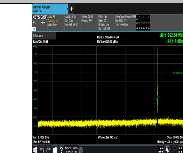
Band5-1.4MHz-16QAM-20407-1RB#0-30~1000-PASS
