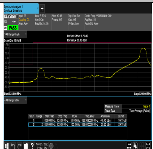
Band5-5MHz-QPSK-20425-1RB#24-PASS
