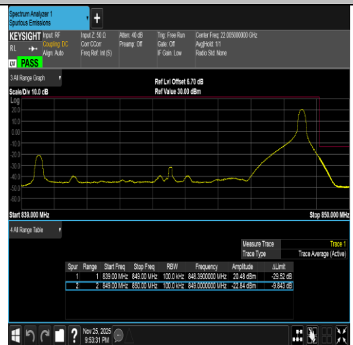
Band5-10MHz-QPSK-20600-1RB#49-PASS
