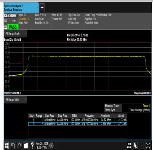
Band5-10MHz-16QAM-20450-50RB#0-PASS
