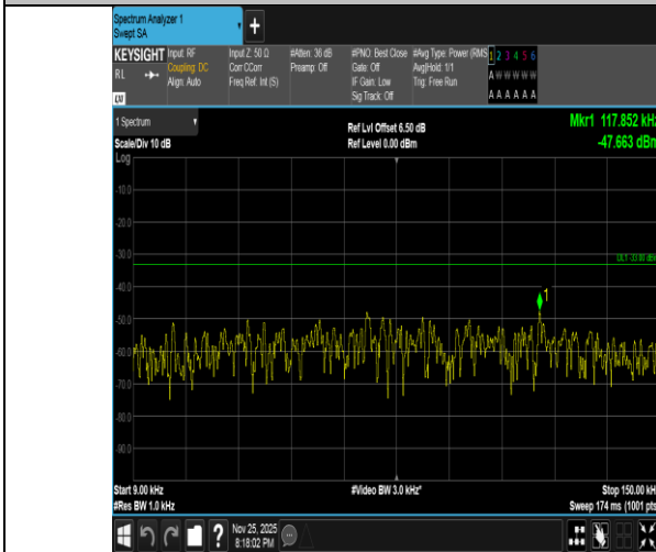
Band5-1.4MHz-QPSK-20407-6RB#0-0.009~0.15-PASS
