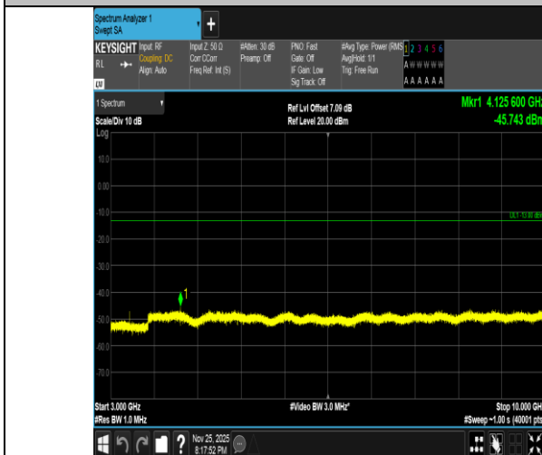
Band5-1.4MHz-16QAM-20407-1RB#5-3000~10000-PASS
