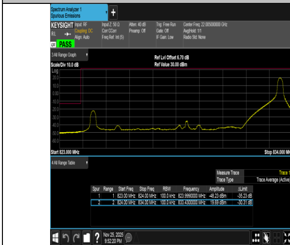
Band5-10MHz-16QAM-20450-1RB#49-PASS
