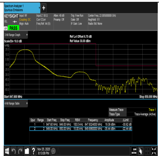
Band5-1.4MHz-16QAM-20643-1RB#0-PASS
