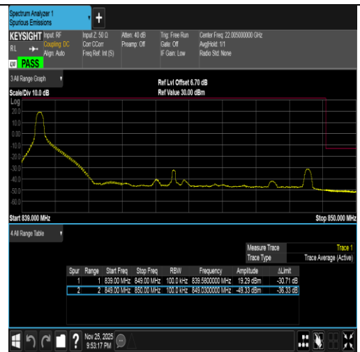
Band5-10MHz-16QAM-20600-1RB#0-PASS
