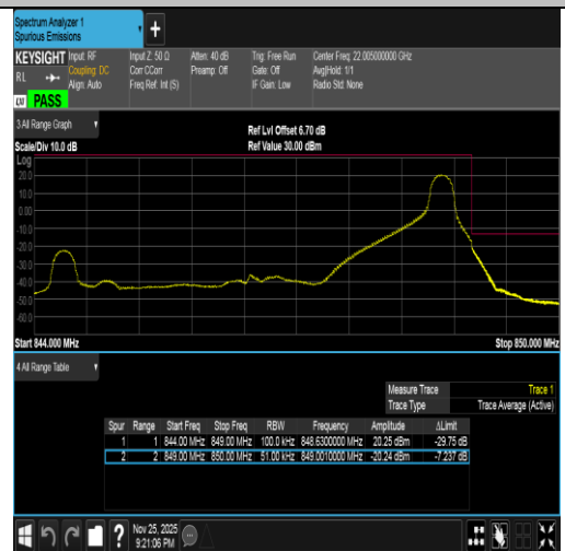
Band5-5MHz-QPSK-20625-1RB#24-PASS
