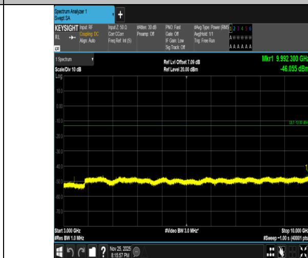
Band5-1.4MHz-16QAM-20407-1RB#0-3000~10000-PASS
