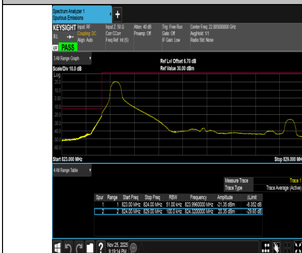
Band5-5MHz-QPSK-20425-1RB#0-PASS
