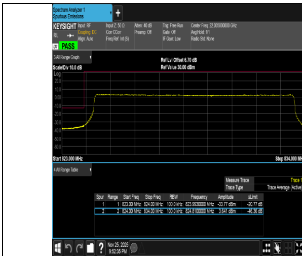
Band5-10MHz-QPSK-20450-50RB#0-PASS
