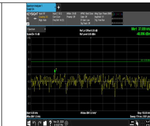
Band5-1.4MHz-16QAM-20407-1RB#0-0.009~0.15-PASS
