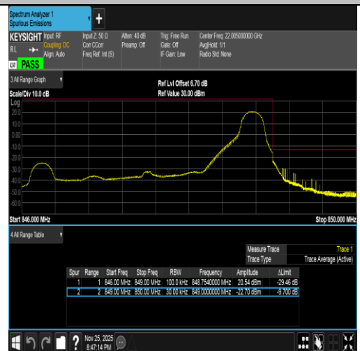
Band5-3MHz-QPSK-20635-1RB#14-PASS
