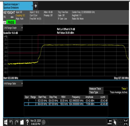
Band5-3MHz-16QAM-20415-15RB#0-PASS
