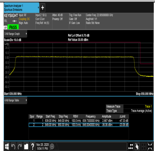
Band5-10MHz-16QAM-20600-50RB#0-PASS
