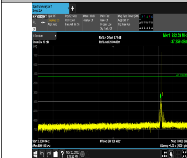
Band5-1.4MHz-QPSK-20407-6RB#0-30~1000-PASS
