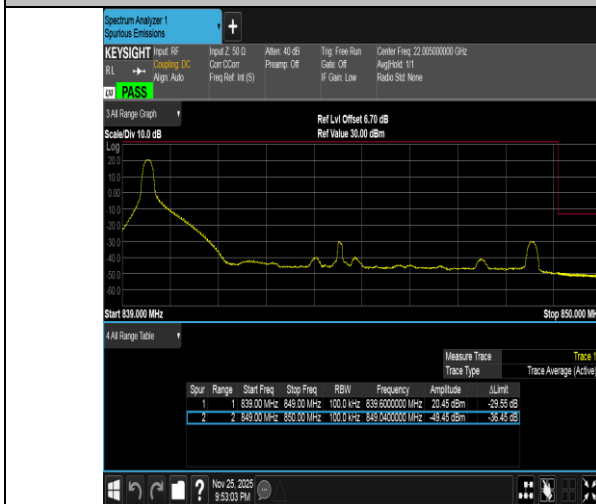
Band5-10MHz-QPSK-20600-1RB#0-PASS
