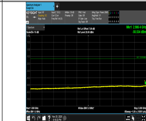
Band5-1.4MHz-QPSK-20407-6RB#0-1000~3000-PASS
