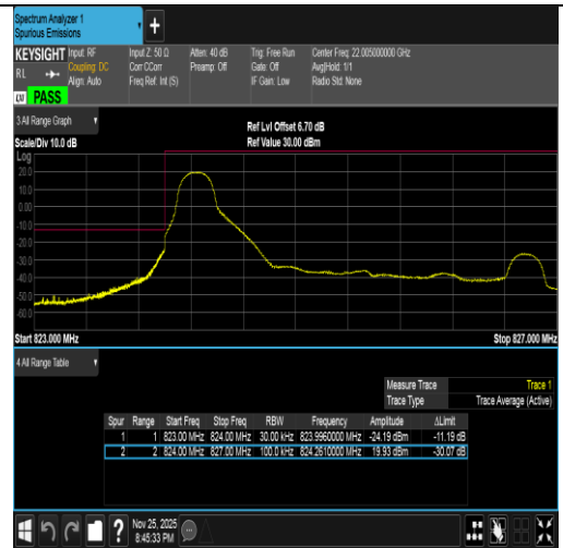
Band5-3MHz-16QAM-20415-1RB#0-PASS
