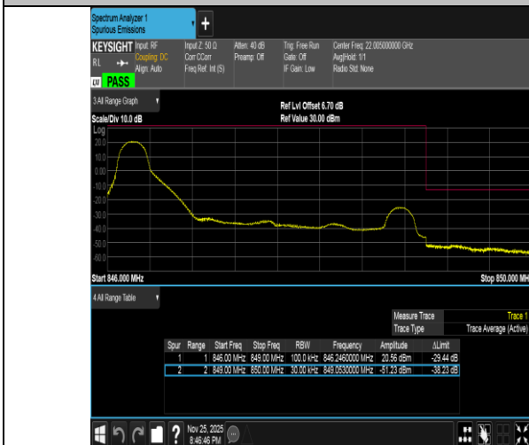
Band5-3MHz-QPSK-20635-1RB#0-PASS
