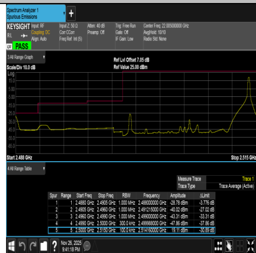
Band7-15MHz-QPSK-20825-1RB#74-PASS
