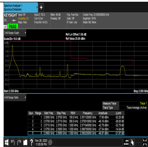
Band7-20MHz-16QAM-21350-1RB#0-PASS
