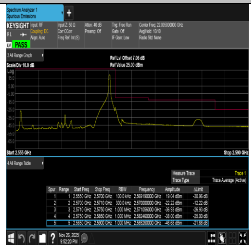
Band7-15MHz-QPSK-21375-1RB#74-PASS
