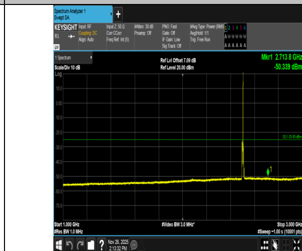
Band7-5MHz-16QAM-20775-1RB#24-1000~3000-PASS
