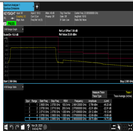
Band7-10MHz-16QAM-21400-50RB#0-PASS
