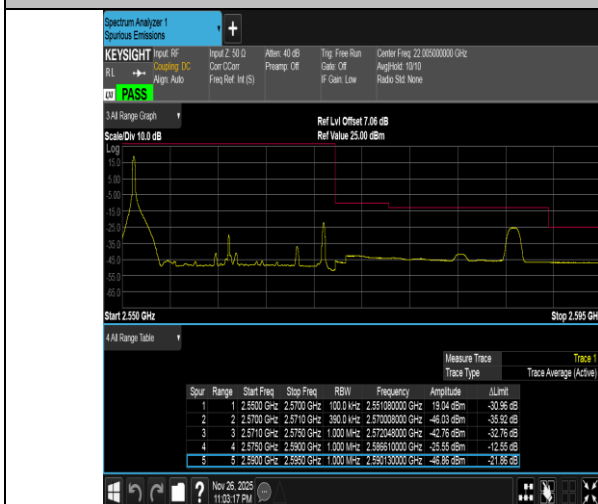
Band7-20MHz-QPSK-21350-1RB#0-PASS
