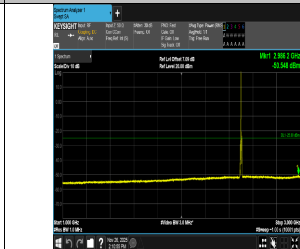
Band7-5MHz-16QAM-20775-1RB#0-1000~3000-PASS
