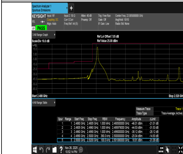
Band7-20MHz-QPSK-20850-1RB#0-PASS
