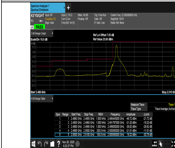
Band7-10MHz-QPSK-20800-1RB#0-PASS
