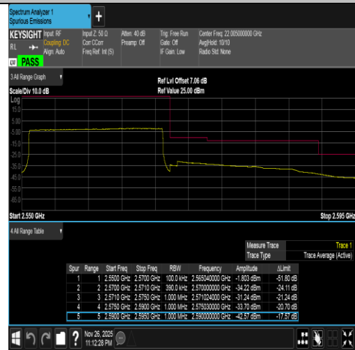
Band7-20MHz-16QAM-21350-100RB#0-PASS
