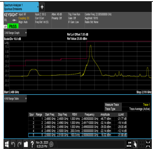
Band7-10MHz-16QAM-20800-1RB#0-PASS
