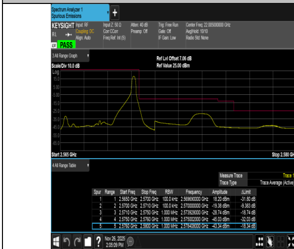
Band7-5MHz-16QAM-21425-1RB#24-PASS
