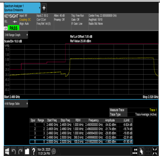
Band7-20MHz-16QAM-20850-100RB#0-PASS
