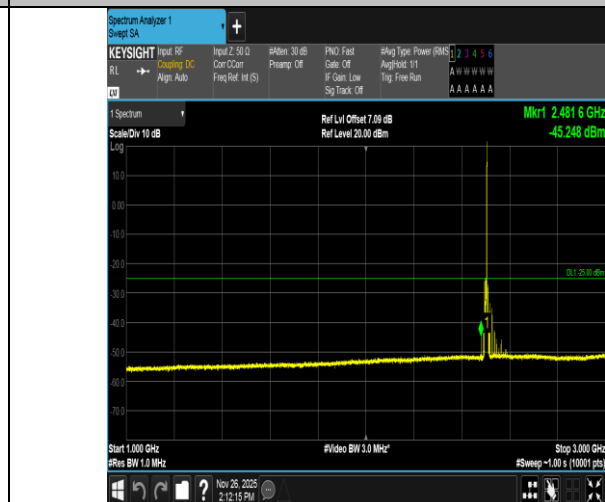
Band7-5MHz-QPSK-20775-1RB#24-1000~3000-PASS
