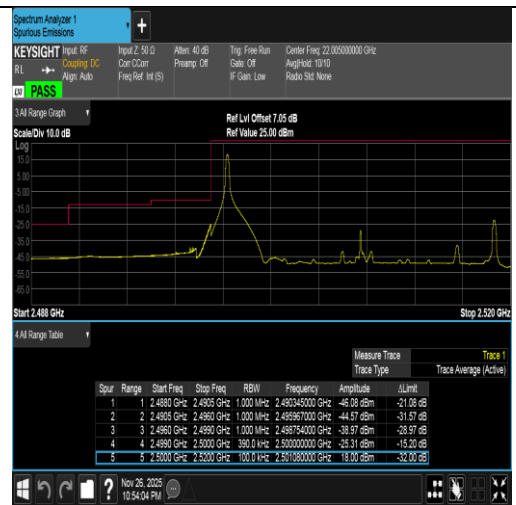
Band7-20MHz-16QAM-20850-1RB#0-PASS
