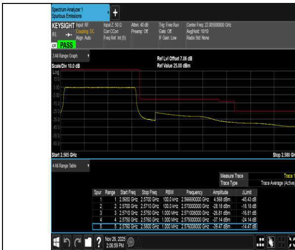
Band7-5MHz-QPSK-21425-25RB#0-PASS
