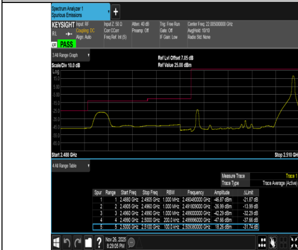
Band7-10MHz-16QAM-20800-1RB#49-PASS
