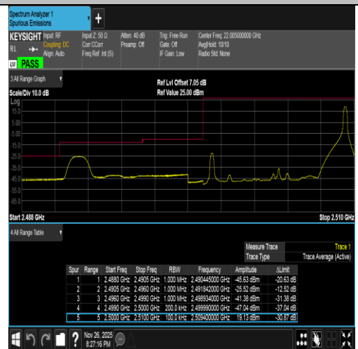
Band7-10MHz-QPSK-20800-1RB#49-PASS
