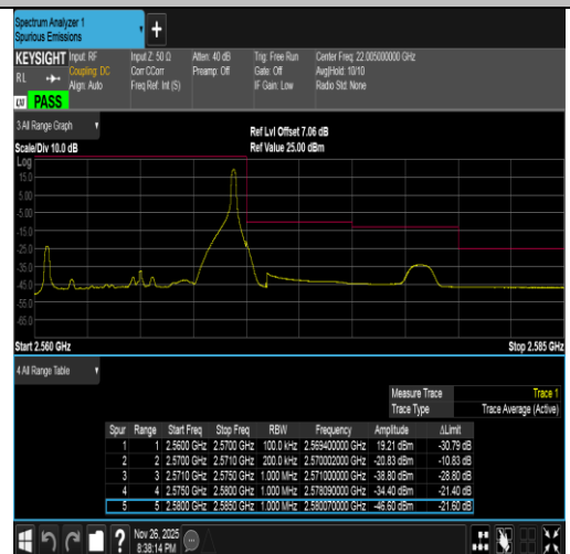
Band7-10MHz-QPSK-21400-1RB#49-PASS
