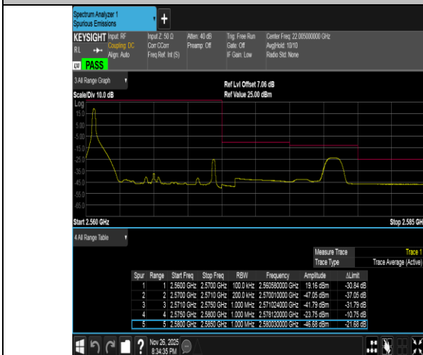
Band7-10MHz-QPSK-21400-1RB#0-PASS
