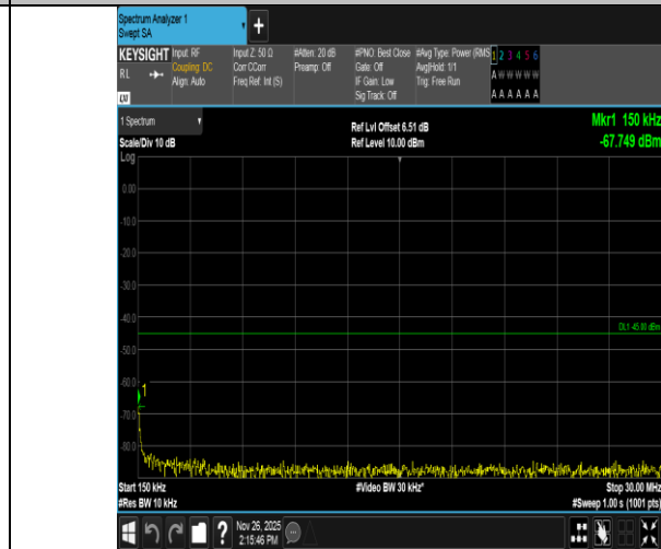
Band7-5MHz-16QAM-20775-25RB#0-0.15~30-PASS
