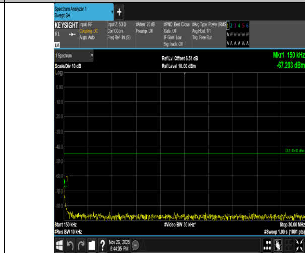
Band7-10MHz-QPSK-20800-1RB#0-0.15~30-PASS
