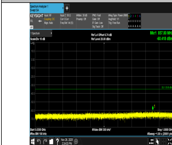
Band7-5MHz-16QAM-21100-25RB#0-30~1000-PASS
