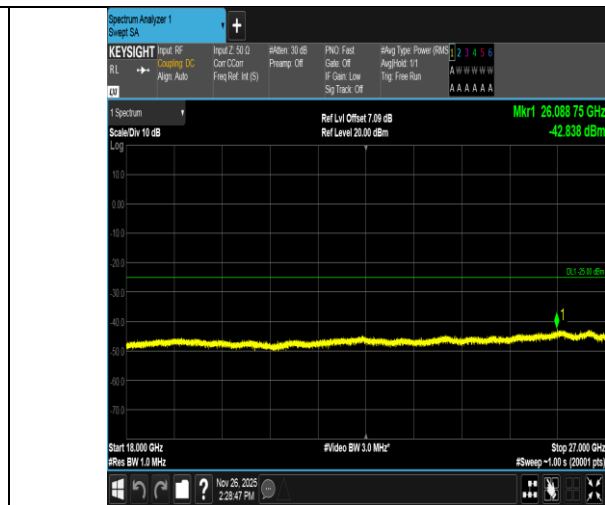
Band7-5MHz-QPSK-21425-1RB#24-18000~27000-PASS
