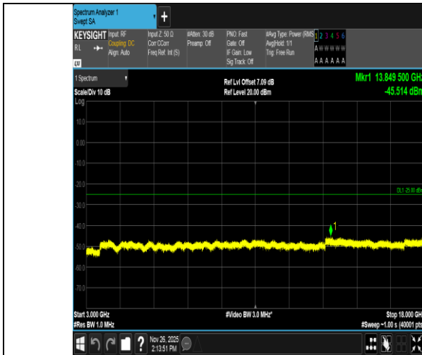
Band7-5MHz-16QAM-20775-1RB#24-3000~18000-PASS
