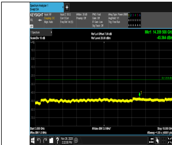
Band7-5MHz-16QAM-21100-1RB#24-3000~18000-PASS
