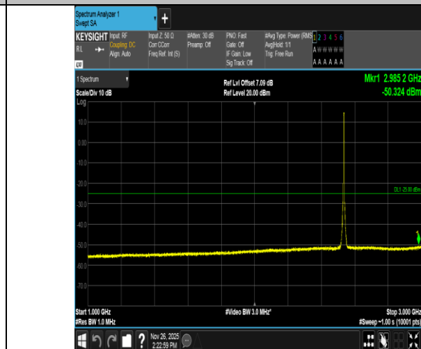
Band7-5MHz-QPSK-21100-25RB#0-1000~3000-PASS
