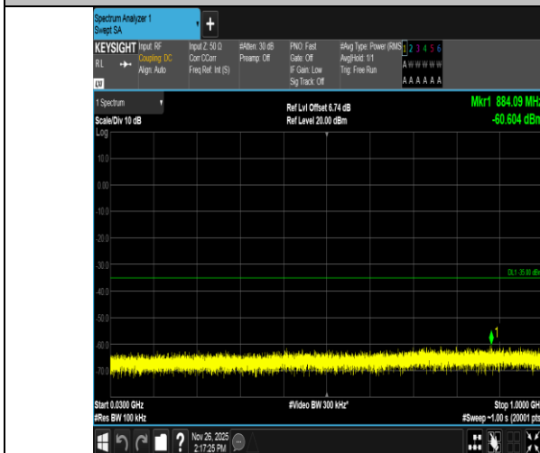
Band7-5MHz-QPSK-21100-1RB#0-30~1000-PASS
