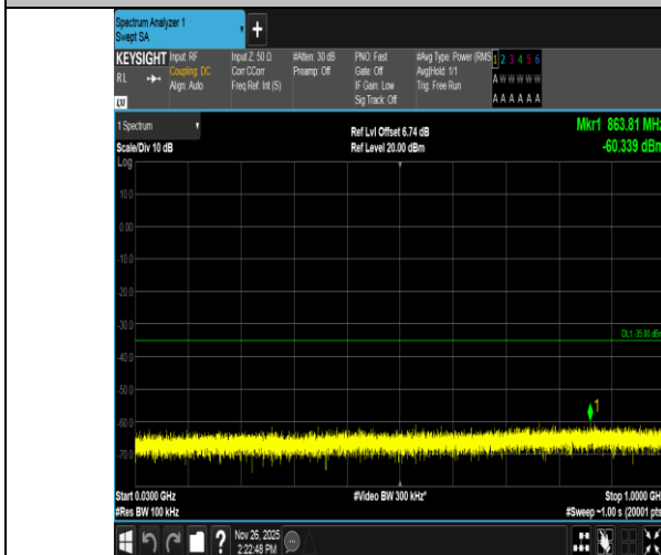
Band7-5MHz-QPSK-21100-25RB#0-30~1000-PASS
