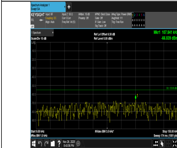
Band7-10MHz-QPSK-20800-1RB#0-0.009~0.15-PASS
