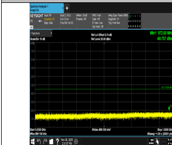
Band7-5MHz-16QAM-21425-25RB#0-30~1000-PASS
