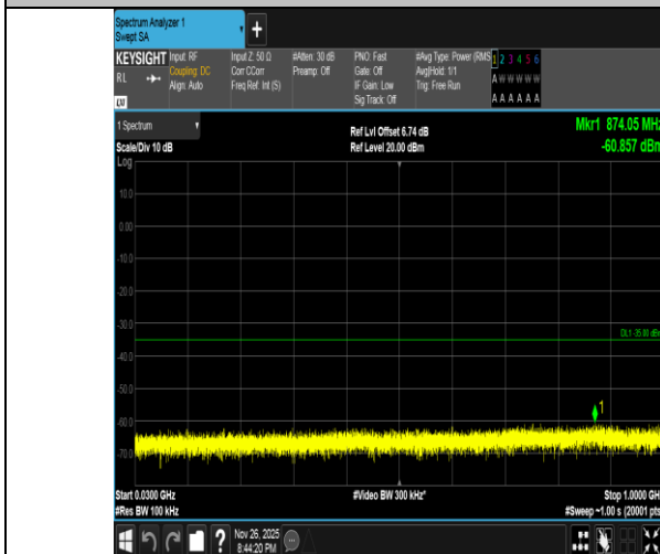
Band7-10MHz-QPSK-20800-1RB#0-30~1000-PASS
