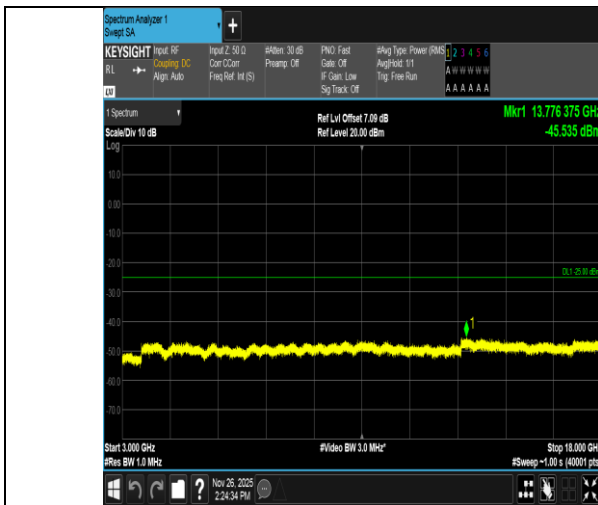
Band7-5MHz-16QAM-21100-25RB#0-3000~18000-PASS
