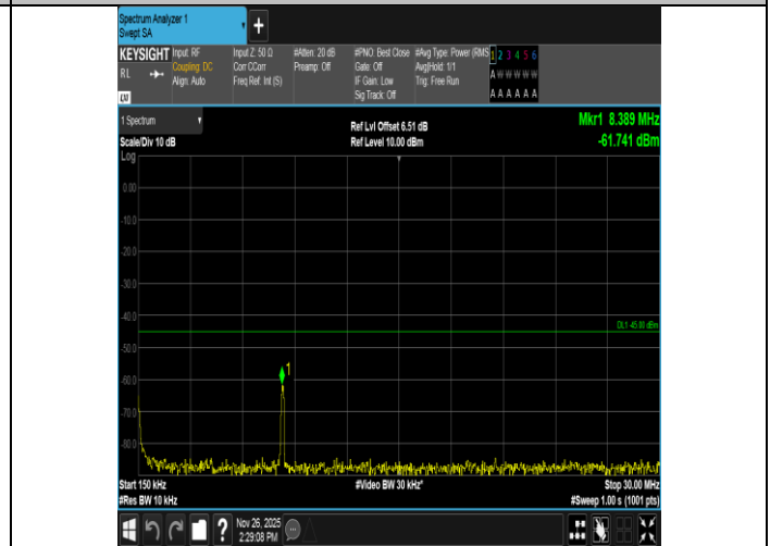
Band7-5MHz-16QAM-21425-1RB#24-0.15~30-PASS
