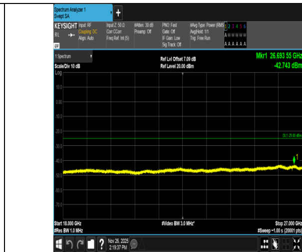
Band7-5MHz-16QAM-21100-1RB#0-18000~27000-PASS
