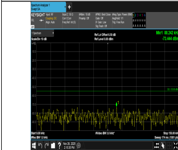
Band7-5MHz-16QAM-20775-25RB#0-0.009~0.15-PASS
