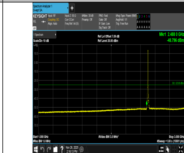
Band7-5MHz-16QAM-20775-25RB#0-1000~3000-PASS
