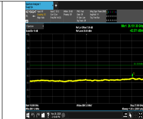
Band7-5MHz-16QAM-20775-25RB#0-18000~27000-PASS
