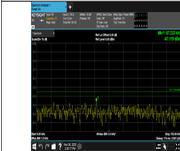
Band7-5MHz-16QAM-21425-1RB#0-0.009~0.15-PASS
