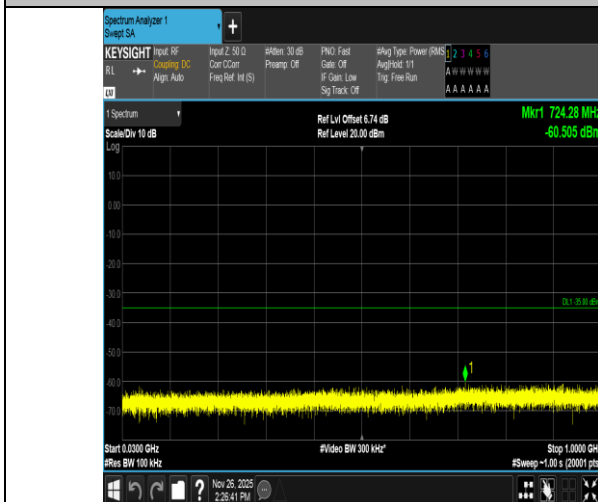
Band7-5MHz-16QAM-21425-1RB#0-30~1000-PASS
