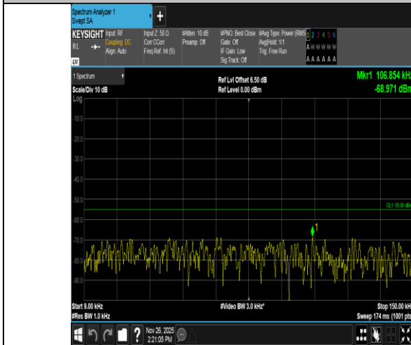
Band7-5MHz-16QAM-21100-1RB#24-0.009~0.15-PASS
