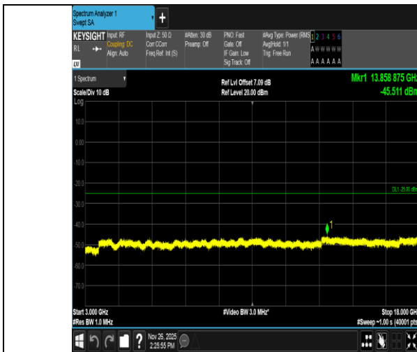
Band7-5MHz-QPSK-21425-1RB#0-3000~18000-PASS
