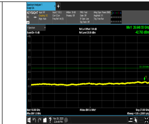
Band7-5MHz-16QAM-21100-25RB#0-18000~27000-PASS
