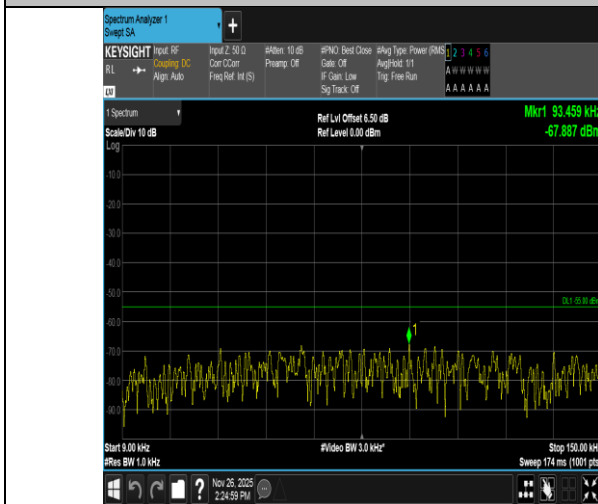
Band7-5MHz-QPSK-21425-1RB#0-0.009~0.15-PASS
