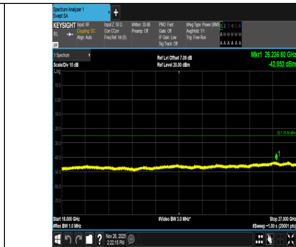
Band7-5MHz-16QAM-21100-1RB#24-18000~27000-PASS
