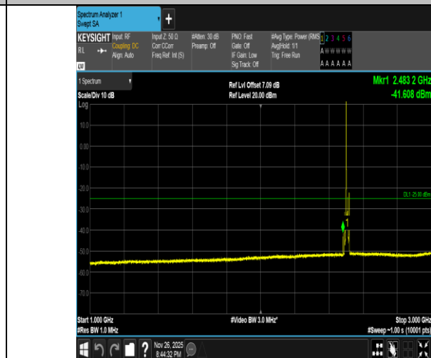
Band7-10MHz-QPSK-20800-1RB#0-1000~3000-PASS
