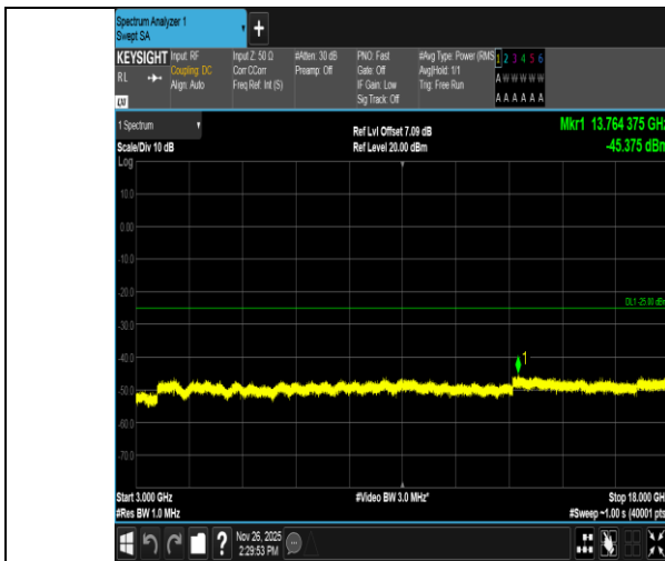
Band7-5MHz-16QAM-21425-1RB#24-3000~18000-PASS
