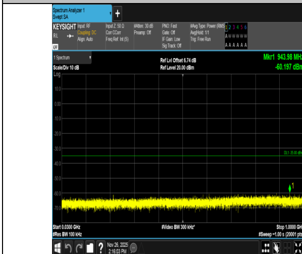
Band7-5MHz-16QAM-20775-25RB#0-30~1000-PASS
