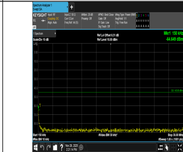
Band7-5MHz-16QAM-21100-1RB#24-0.15~30-PASS
