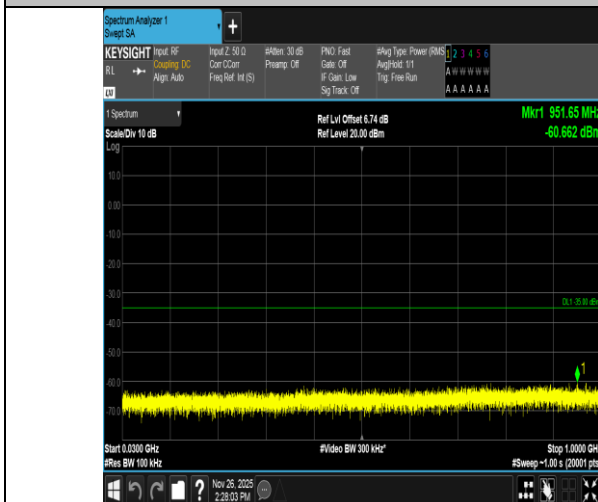
Band7-5MHz-QPSK-21425-1RB#24-30~1000-PASS
