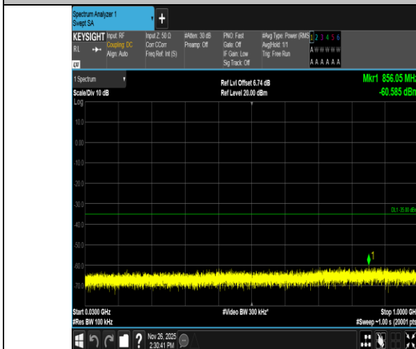
Band7-5MHz-QPSK-21425-25RB#0-30~1000-PASS
