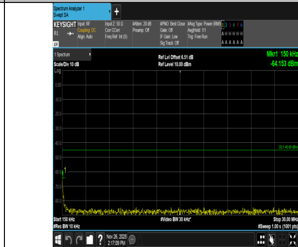
Band7-5MHz-QPSK-21100-1RB#0-0.15~30-PASS
