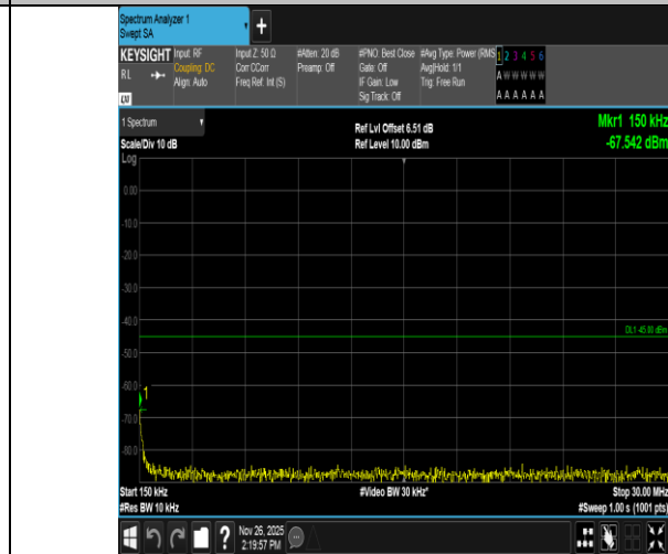
Band7-5MHz-QPSK-21100-1RB#24-0.15~30-PASS
