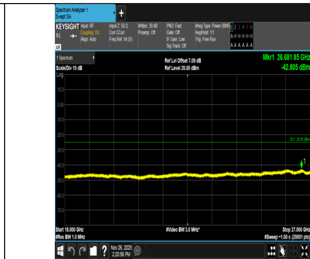
Band7-5MHz-QPSK-21100-1RB#24-18000~27000-PASS
