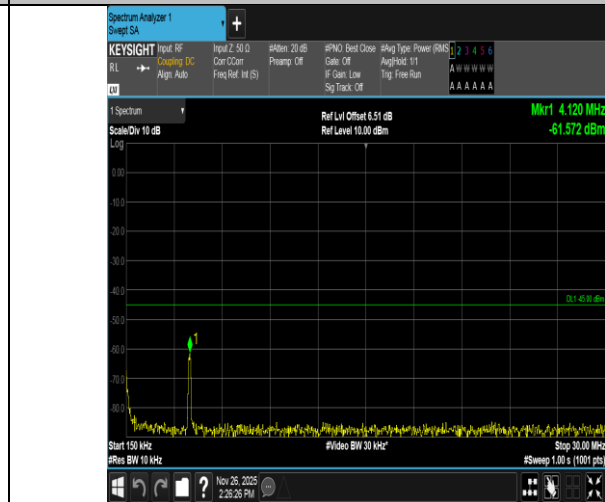
Band7-5MHz-16QAM-21425-1RB#0-0.15~30-PASS
