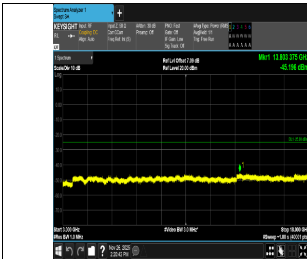
Band7-5MHz-QPSK-21100-1RB#24-3000~18000-PASS
