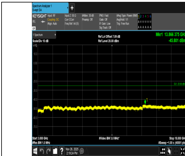
Band7-5MHz-16QAM-21100-1RB#0-3000~18000-PASS
