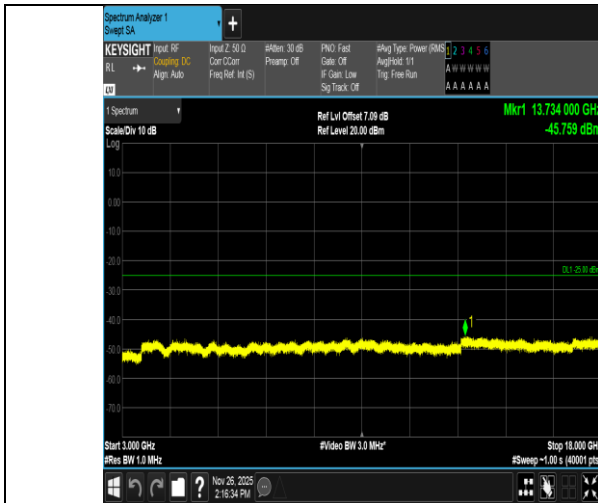
Band7-5MHz-16QAM-20775-25RB#0-3000~18000-PASS
