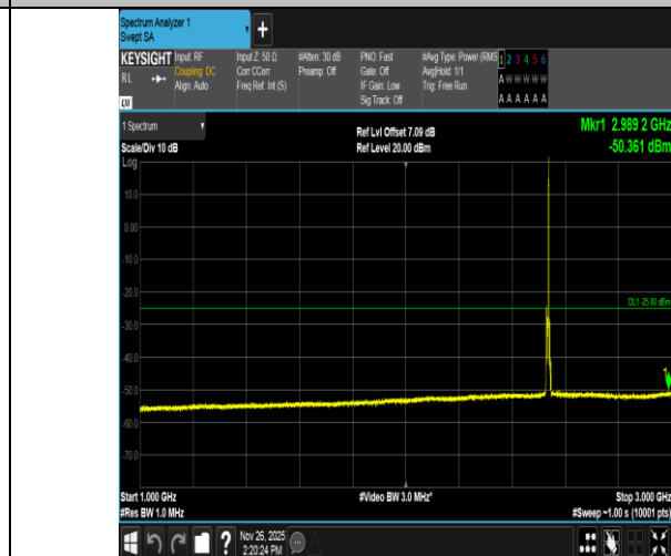
Band7-5MHz-QPSK-21100-1RB#24-1000~3000-PASS
