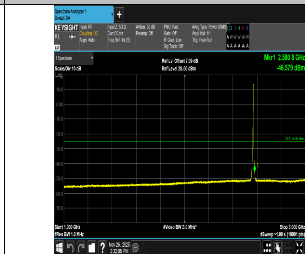
Band7-5MHz-16QAM-21425-25RB#0-1000~3000-PASS
