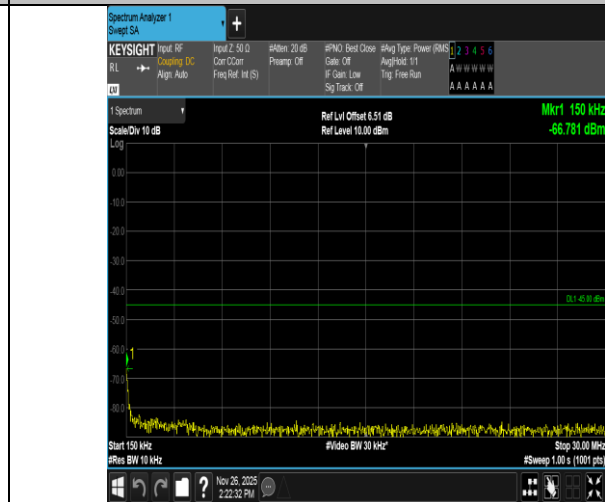
Band7-5MHz-QPSK-21100-25RB#0-0.15~30-PASS
