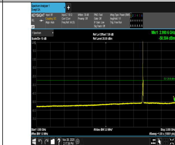
Band7-5MHz-QPSK-21100-1RB#0-1000~3000-PASS
