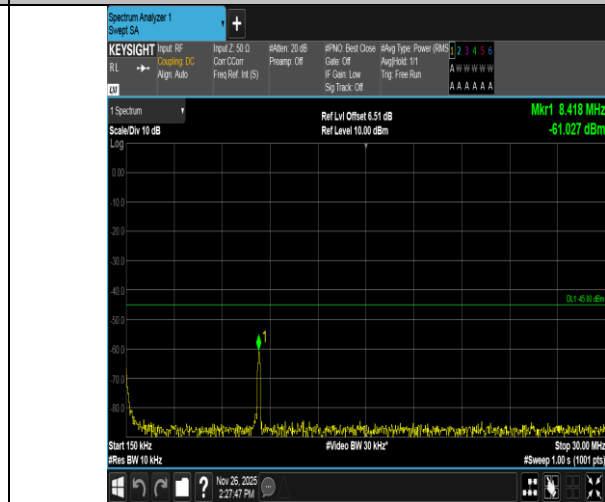
Band7-5MHz-QPSK-21425-1RB#24-0.15~30-PASS
