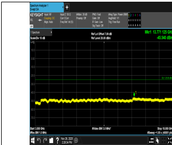
Band7-5MHz-QPSK-21425-1RB#24-3000~18000-PASS
