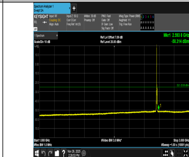
Band7-5MHz-16QAM-21425-1RB#0-1000~3000-PASS
