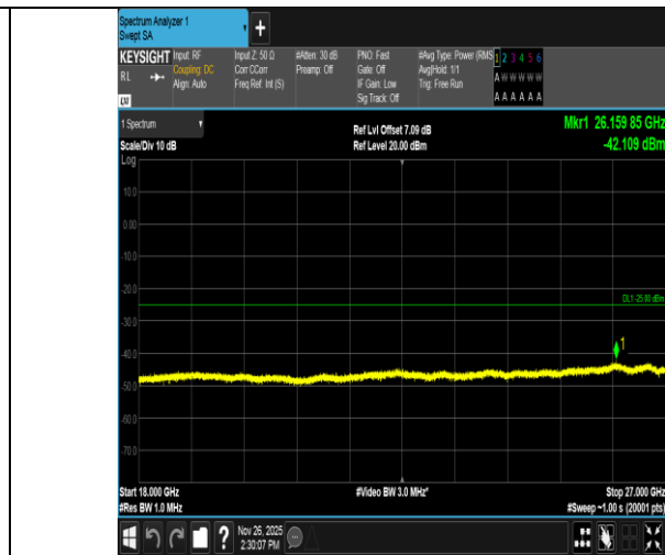
Band7-5MHz-16QAM-21425-1RB#24-18000~27000-PASS
