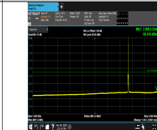
Band7-5MHz-16QAM-21100-1RB#24-1000~3000-PASS
