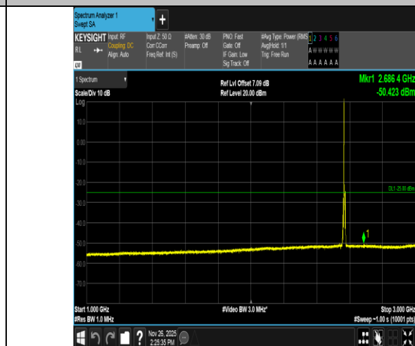
Band7-5MHz-QPSK-21425-1RB#0-1000~3000-PASS
