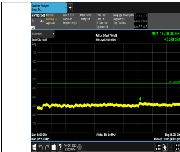
Band7-5MHz-16QAM-21425-25RB#0-3000~18000-PASS
