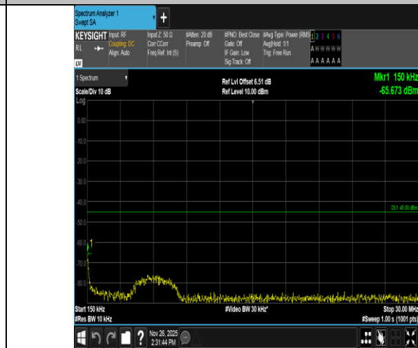
Band7-5MHz-16QAM-21425-25RB#0-0.15~30-PASS
