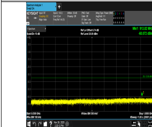
Band7-5MHz-QPSK-21100-1RB#24-30~1000-PASS
