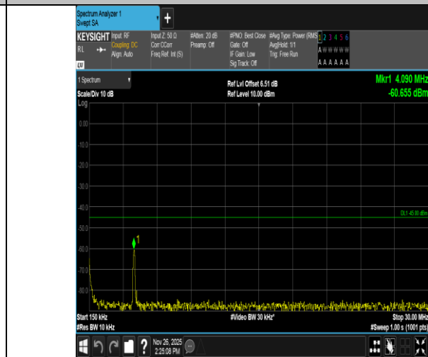
Band7-5MHz-QPSK-21425-1RB#0-0.15~30-PASS
