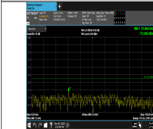
Band7-5MHz-16QAM-21100-25RB#0-0.009~0.15-PASS
