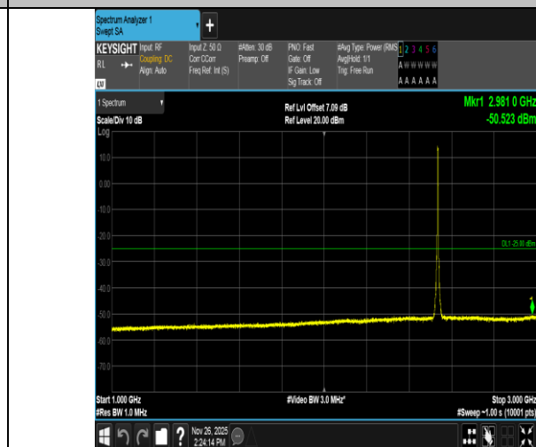
Band7-5MHz-16QAM-21100-25RB#0-1000~3000-PASS
