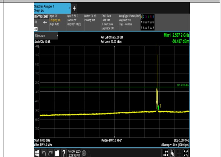
Band7-5MHz-16QAM-21425-1RB#24-1000~3000-PASS
