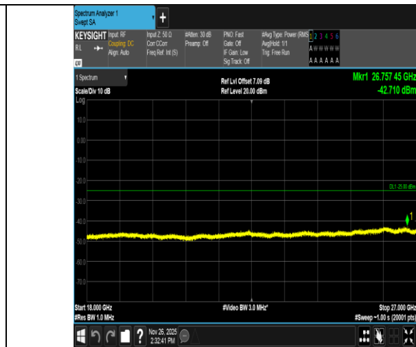
Band7-5MHz-16QAM-21425-25RB#0-18000~27000-PASS
