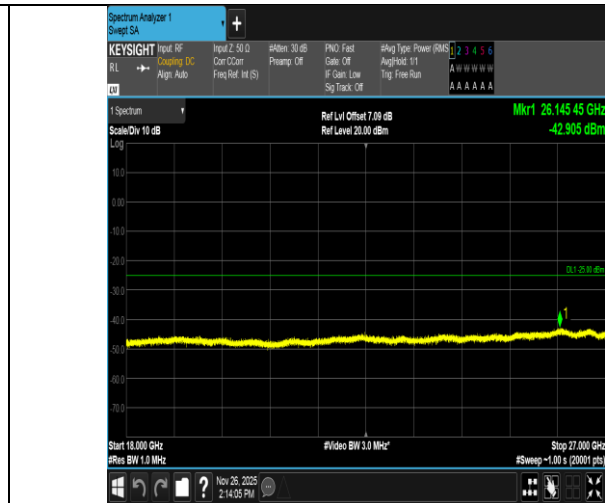
Band7-5MHz-16QAM-20775-1RB#24-18000~27000-PASS
