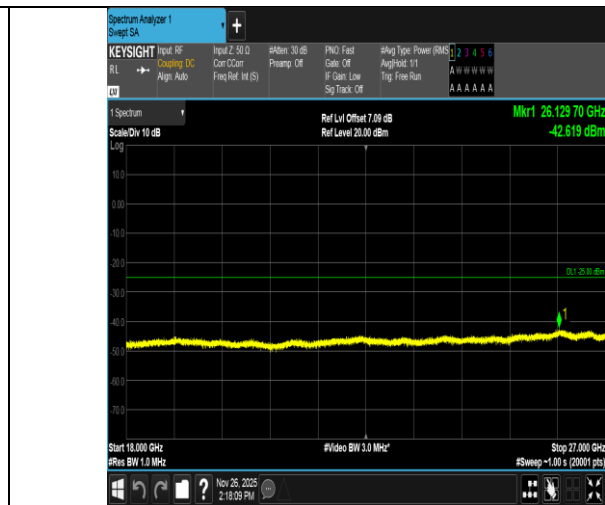
Band7-5MHz-QPSK-21100-1RB#0-18000~27000-PASS
