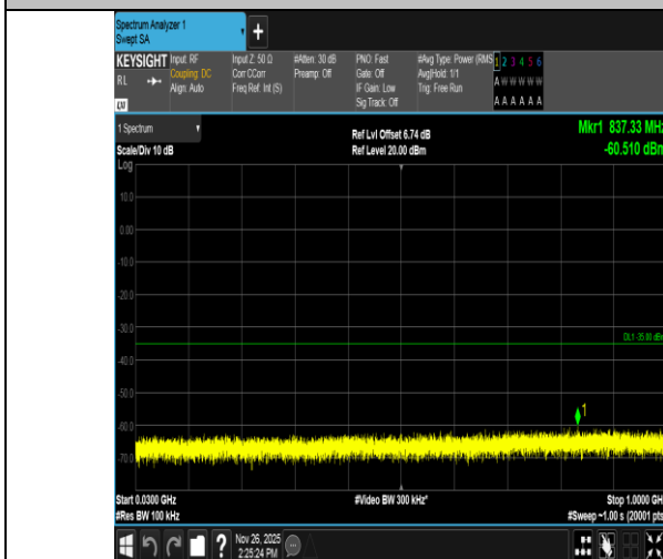
Band7-5MHz-QPSK-21425-1RB#0-30~1000-PASS
