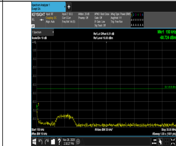
Band7-5MHz-QPSK-21425-25RB#0-0.15~30-PASS
