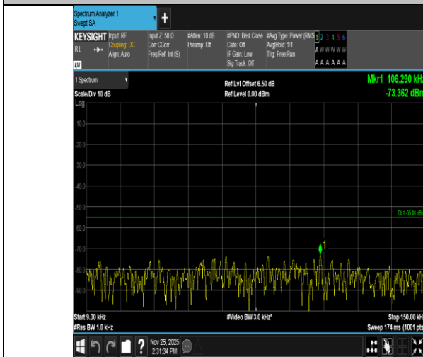
Band7-5MHz-16QAM-21425-25RB#0-0.009~0.15-PASS
