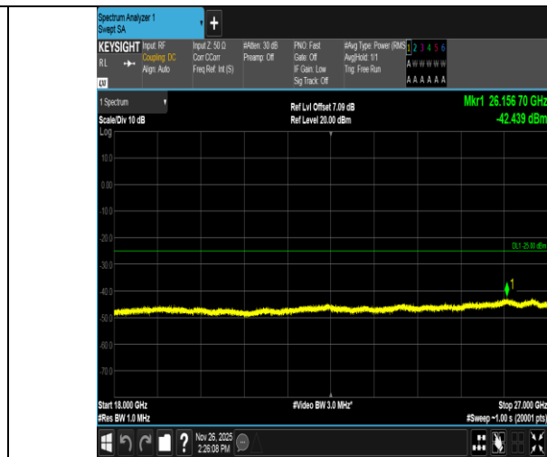
Band7-5MHz-QPSK-21425-1RB#0-18000~27000-PASS
