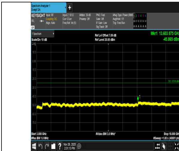
Band7-5MHz-QPSK-21425-25RB#0-3000~18000-PASS
