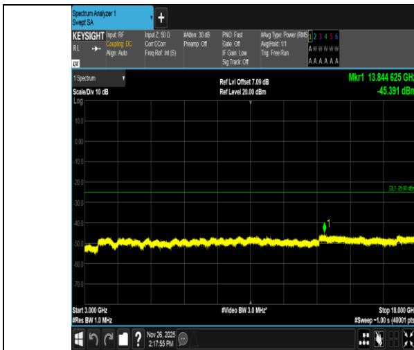
Band7-5MHz-QPSK-21100-1RB#0-3000~18000-PASS
