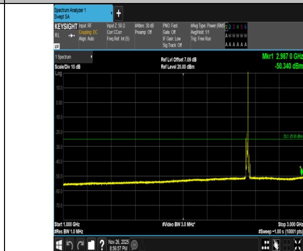
Band7-10MHz-16QAM-21100-1RB#49-1000~3000-PASS
