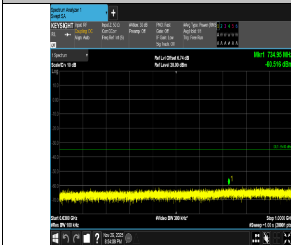
Band7-10MHz-16QAM-21100-1RB#0-30~1000-PASS
