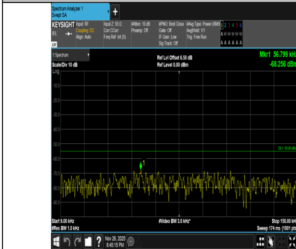
Band7-10MHz-16QAM-20800-1RB#0-0.009~0.15-PASS
