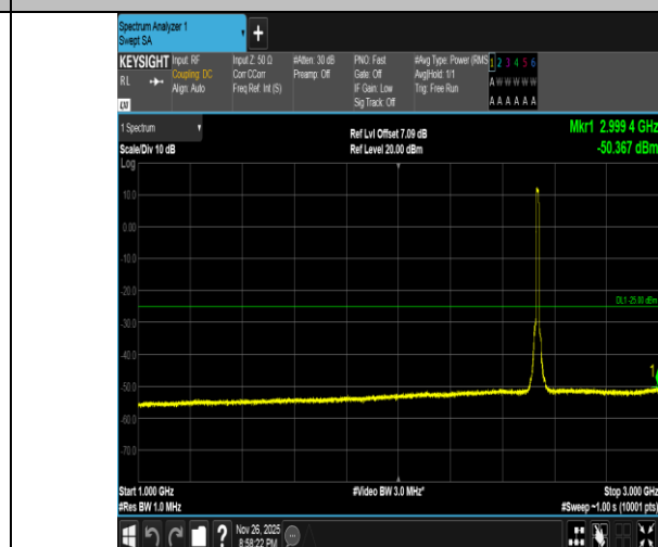
Band7-10MHz-QPSK-21100-50RB#0-1000~3000-PASS
