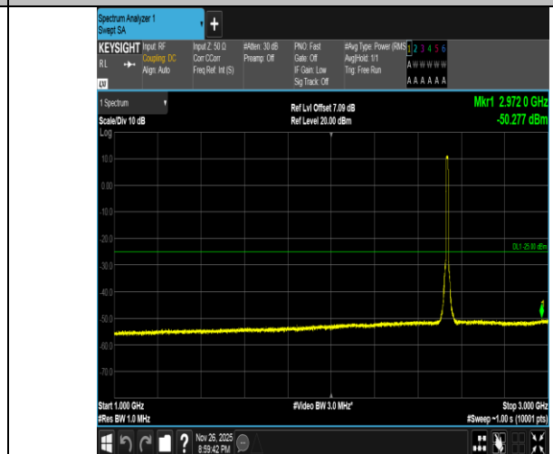
Band7-10MHz-16QAM-21100-50RB#0-1000~3000-PASS
