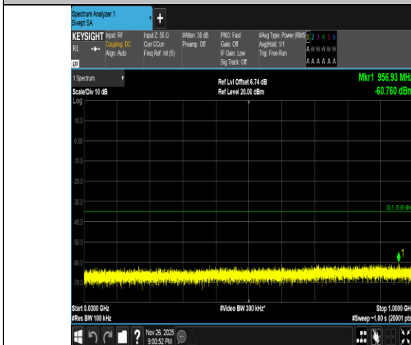
Band7-10MHz-QPSK-21400-1RB#0-30~1000-PASS
