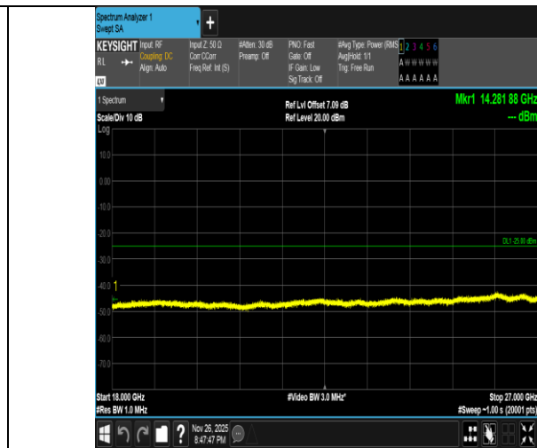
Band7-10MHz-QPSK-20800-1RB#49-18000~27000-PASS
