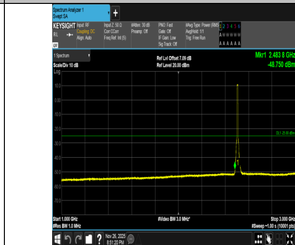
Band7-10MHz-16QAM-20800-50RB#0-1000~3000-PASS
