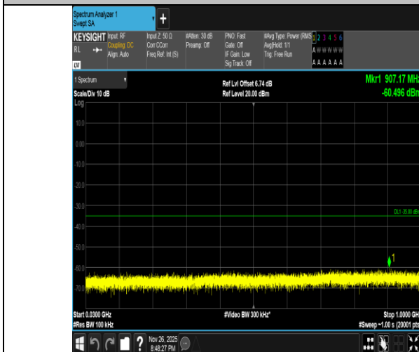
Band7-10MHz-16QAM-20800-1RB#49-30~1000-PASS
