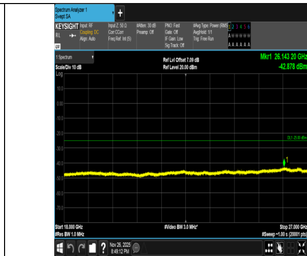
Band7-10MHz-16QAM-20800-1RB#49-18000~27000-PASS
