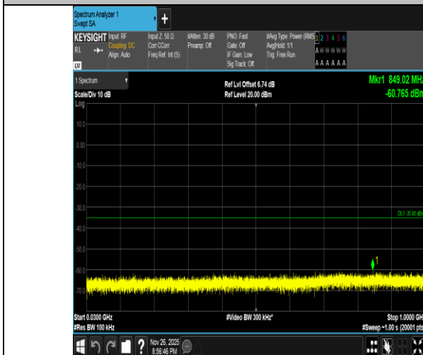
Band7-10MHz-16QAM-21100-1RB#49-30~1000-PASS
