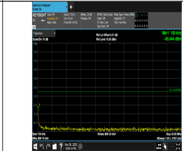
Band7-10MHz-16QAM-21100-50RB#0-0.15~30-PASS
