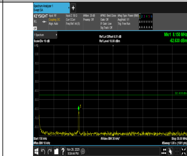
Band7-10MHz-16QAM-21400-1RB#49-0.15~30-PASS
