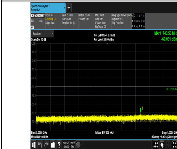
Band7-10MHz-16QAM-21400-1RB#49-30~1000-PASS
