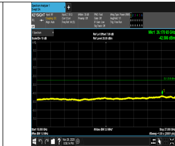
Band7-10MHz-QPSK-21100-1RB#49-18000~27000-PASS
