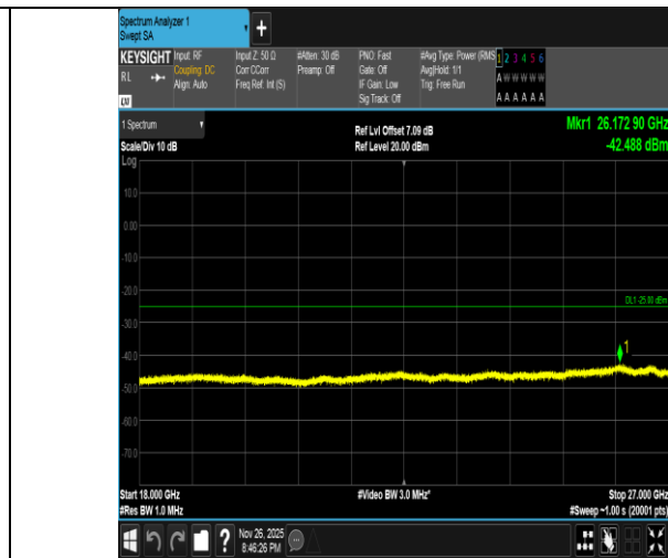
Band7-10MHz-16QAM-20800-1RB#0-18000~27000-PASS
