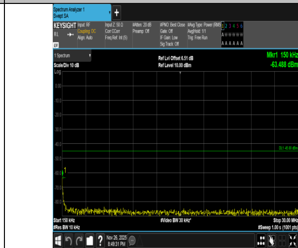
Band7-10MHz-QPSK-20800-50RB#0-0.15~30-PASS
