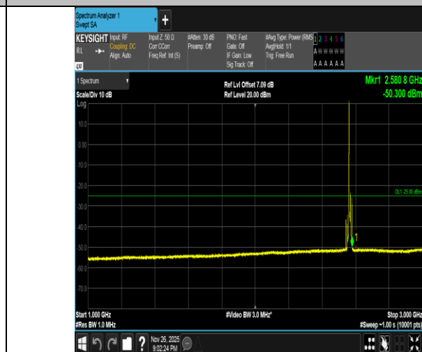
Band7-10MHz-16QAM-21400-1RB#0-1000~3000-PASS
