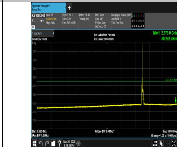
Band7-10MHz-16QAM-20800-1RB#49-1000~3000-PASS
