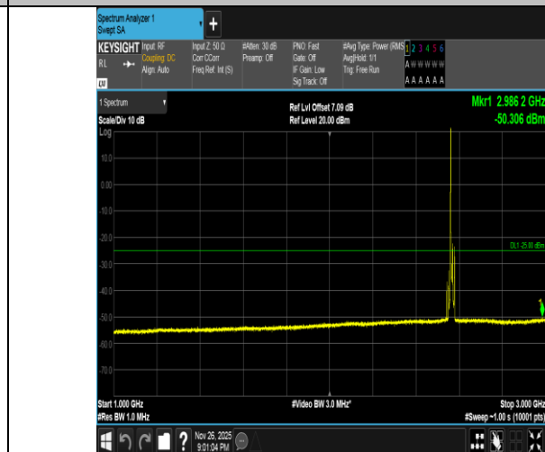
Band7-10MHz-QPSK-21400-1RB#0-1000~3000-PASS
