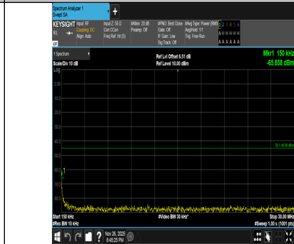
Band7-10MHz-16QAM-20800-1RB#0-0.15~30-PASS
