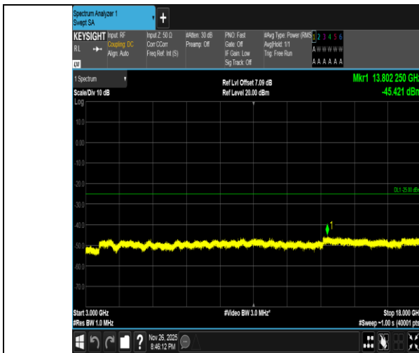
Band7-10MHz-16QAM-20800-1RB#0-3000~18000-PASS
