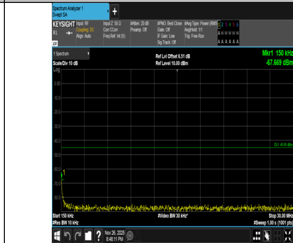
Band7-10MHz-16QAM-20800-1RB#49-0.15~30-PASS
