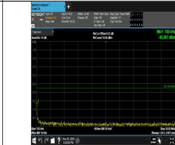
Band7-10MHz-16QAM-20800-50RB#0-0.15~30-PASS
