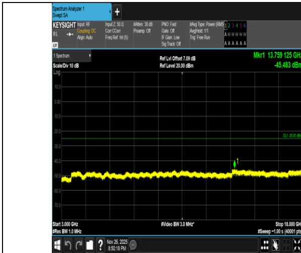
Band7-10MHz-QPSK-20800-50RB#0-3000~18000-PASS
