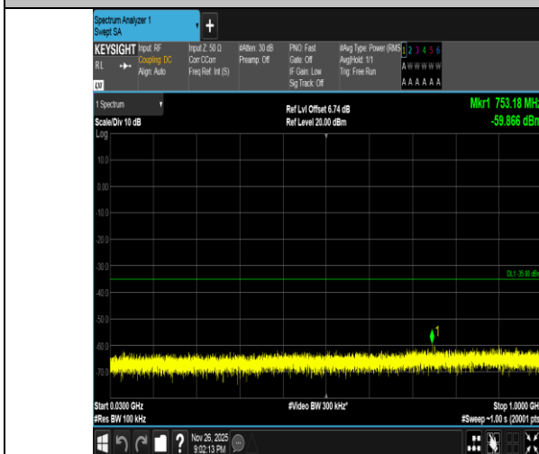
Band7-10MHz-16QAM-21400-1RB#0-30~1000-PASS
