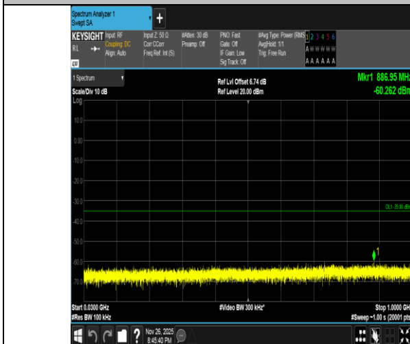
Band7-10MHz-16QAM-20800-1RB#0-30~1000-PASS
