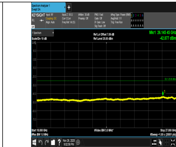
Band7-10MHz-16QAM-21400-1RB#0-18000~27000-PASS
