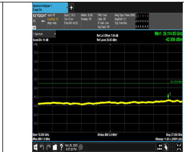
Band7-10MHz-16QAM-21100-1RB#49-18000~27000-PASS
