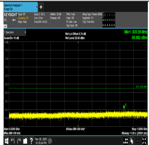
Band7-15MHz-QPSK-21375-1RB#74-30~1000-PASS
