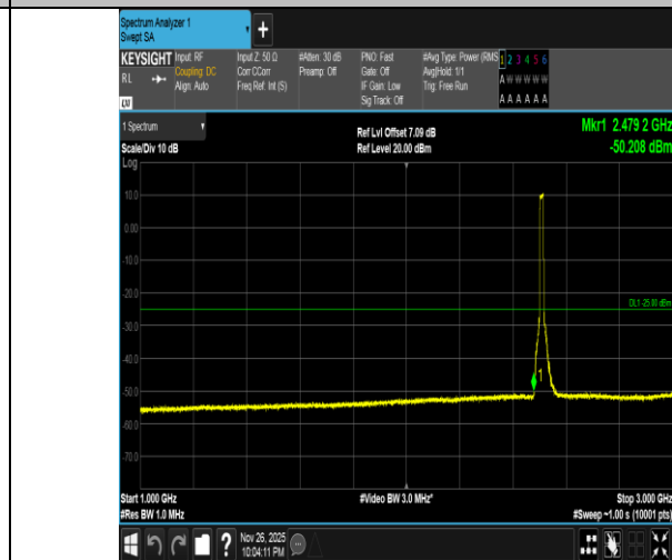
Band7-15MHz-QPSK-20825-75RB#0-1000~3000-PASS
