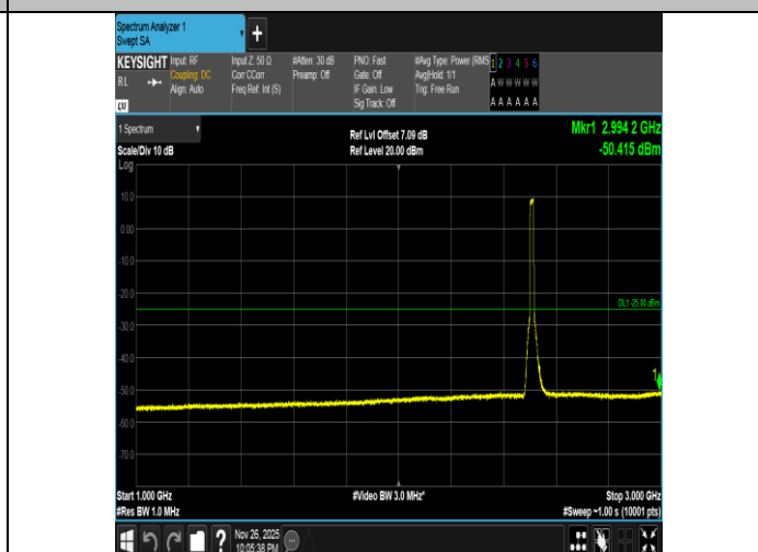
Band7-15MHz-16QAM-20825-75RB#0-1000~3000-PASS
