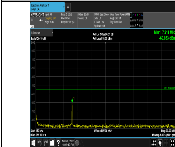
Band7-15MHz-QPSK-21375-1RB#74-0.15~30-PASS
