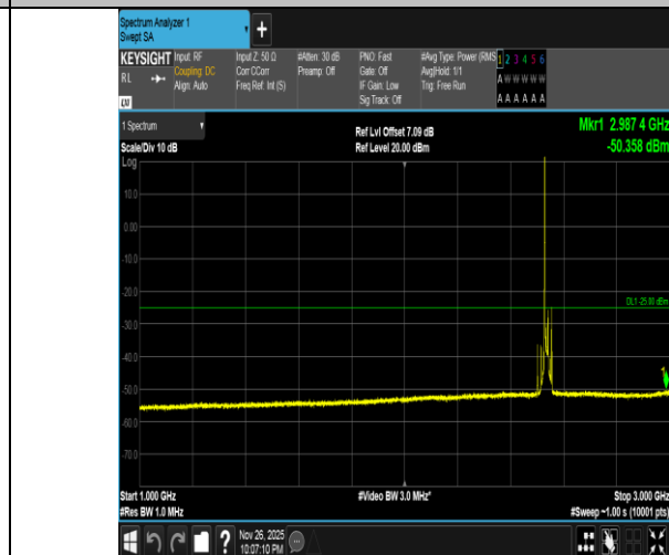
Band7-15MHz-QPSK-21100-1RB#0-1000~3000-PASS
