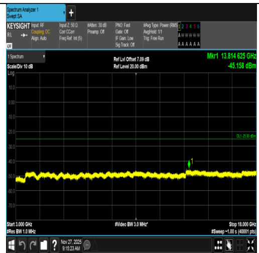
Band7-15MHz-QPSK-21375-1RB#0-3000~18000-PASS
