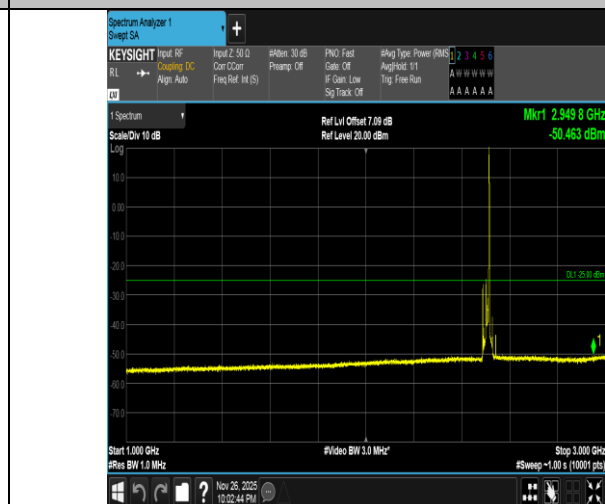
Band7-15MHz-16QAM-20825-1RB#74-1000~3000-PASS
