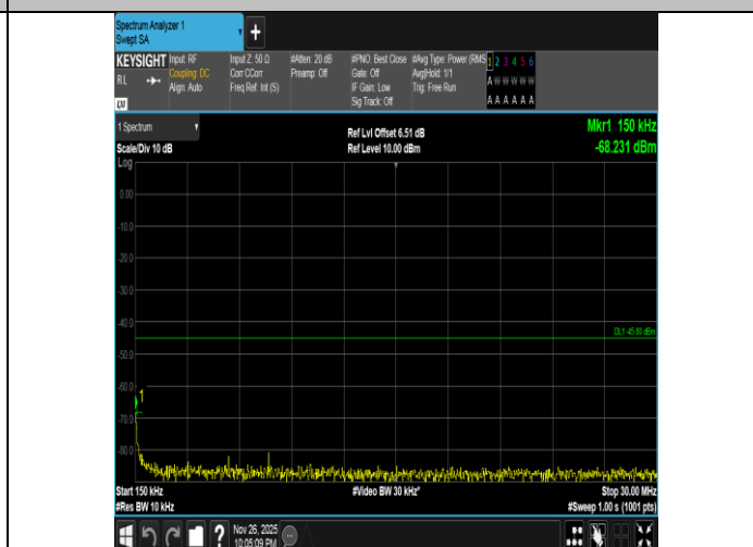
Band7-15MHz-16QAM-20825-75RB#0-0.15~30-PASS
