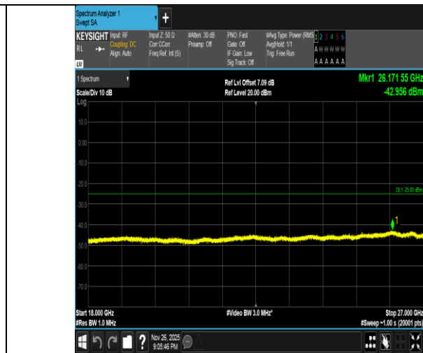
Band7-10MHz-16QAM-21400-1RB#49-18000~27000-PASS
