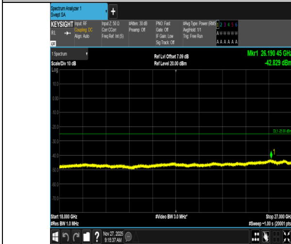
Band7-15MHz-QPSK-21375-1RB#0-18000~27000-PASS
