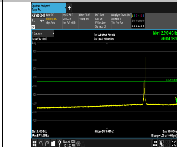
Band7-15MHz-16QAM-21100-1RB#74-1000~3000-PASS
