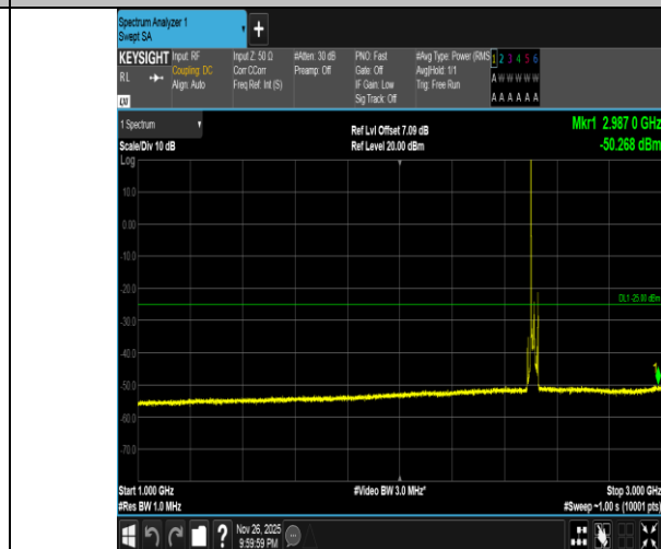
Band7-15MHz-16QAM-20825-1RB#0-1000~3000-PASS
