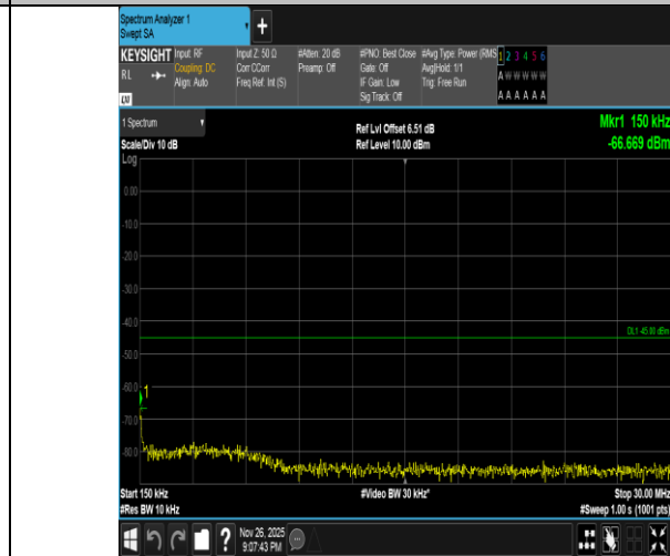
Band7-10MHz-16QAM-21400-50RB#0-0.15~30-PASS
