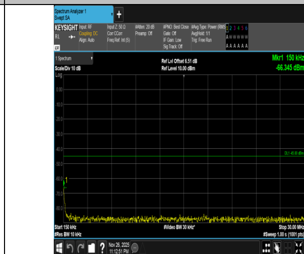
Band7-20MHz-QPSK-20850-1RB#0-0.15~30-PASS
