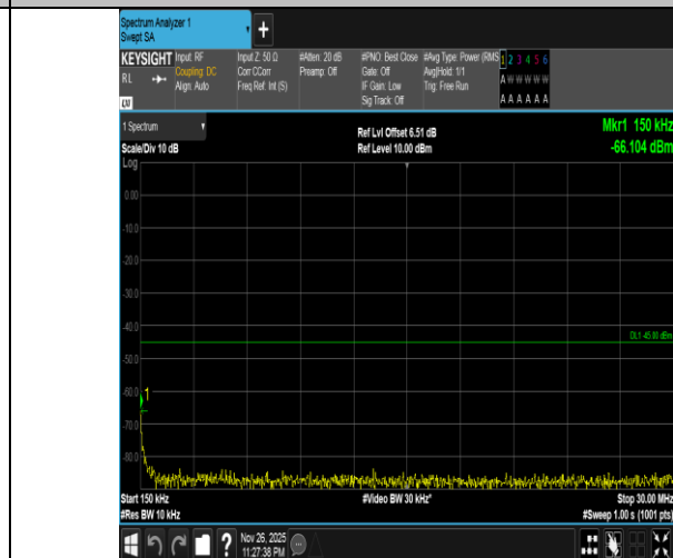
Band7-20MHz-QPSK-21100-100RB#0-0.15~30-PASS
