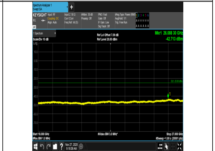
Band7-15MHz-16QAM-21375-1RB#0-18000~27000-PASS
