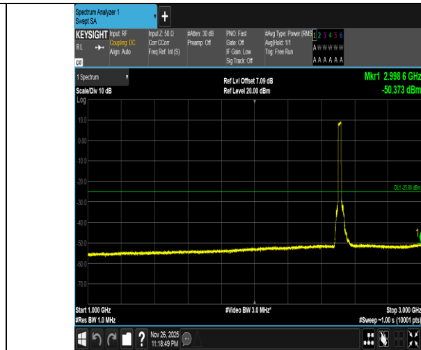
Band7-20MHz-QPSK-20850-100RB#0-1000~3000-PASS
