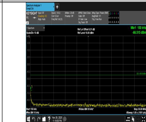
Band7-20MHz-16QAM-20850-100RB#0-0.15~30-PASS
