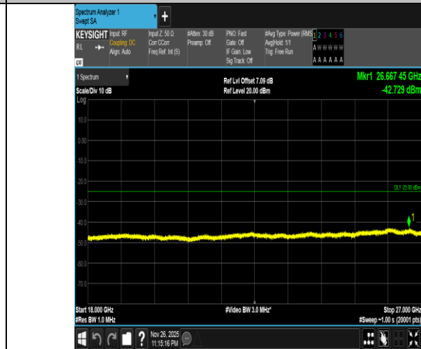
Band7-20MHz-16QAM-20850-1RB#0-18000~27000-PASS
