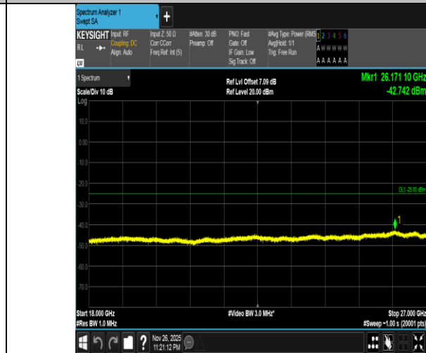
Band7-20MHz-16QAM-20850-100RB#0-18000~27000-PASS
