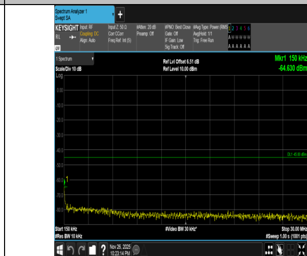
Band7-15MHz-16QAM-21375-75RB#0-0.15~30-PASS
