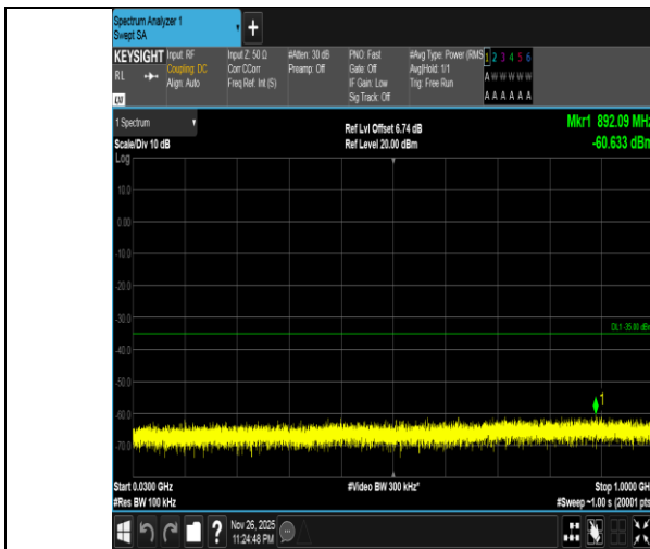
Band7-20MHz-QPSK-21100-1RB#99-30~1000-PASS
