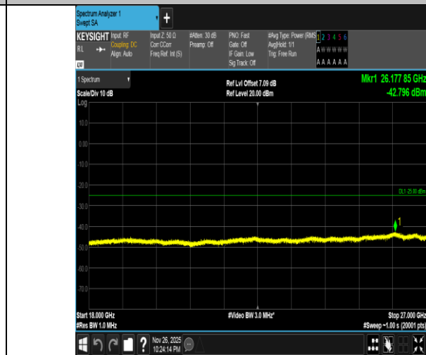
Band7-15MHz-16QAM-21375-75RB#0-18000~27000-PASS
