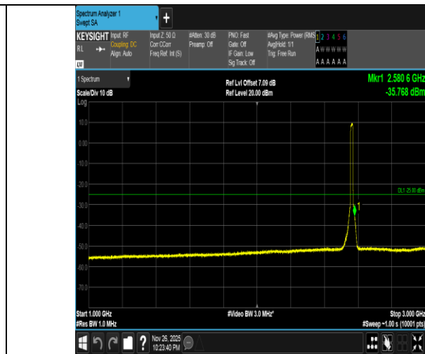
Band7-15MHz-16QAM-21375-75RB#0-1000~3000-PASS
