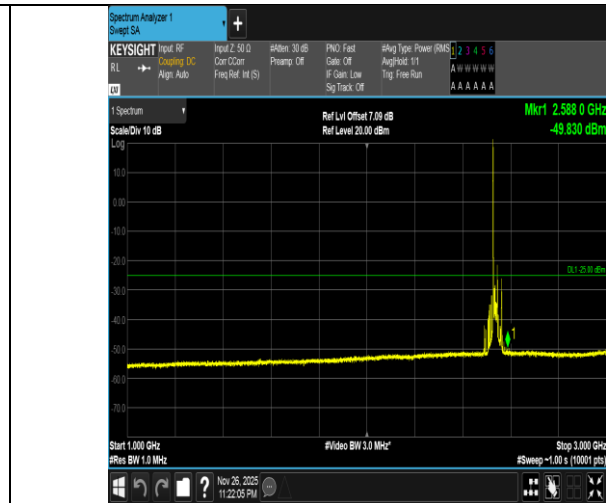
Band7-20MHz-QPSK-21100-1RB#0-1000~3000-PASS
