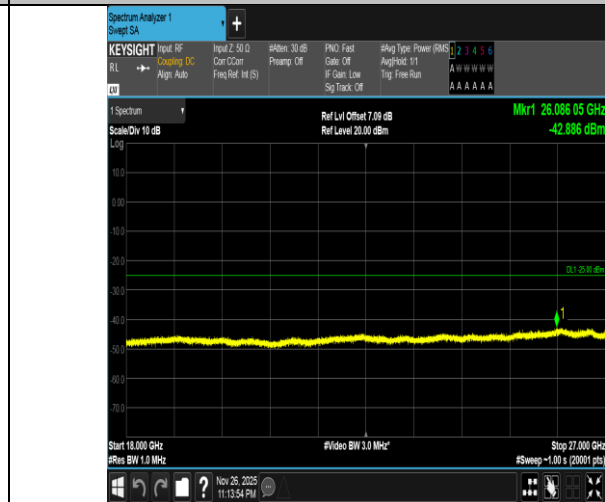
Band7-20MHz-QPSK-20850-1RB#0-18000~27000-PASS
