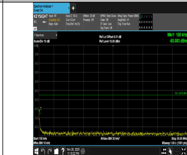
Band7-20MHz-QPSK-20850-100RB#0-0.15~30-PASS
