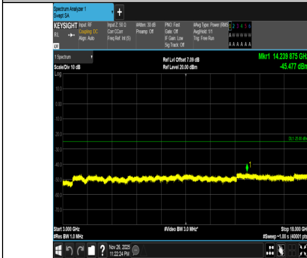
Band7-20MHz-QPSK-21100-1RB#0-3000~18000-PASS
