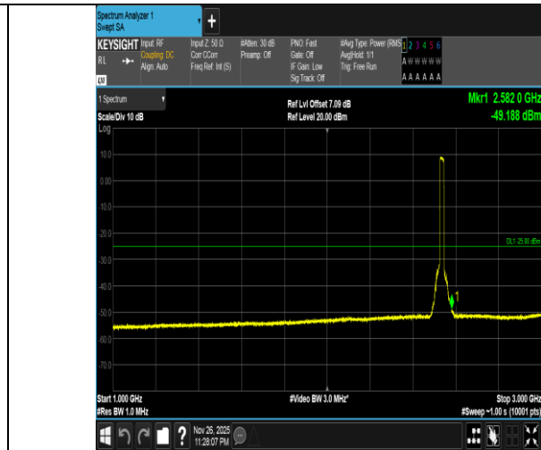
Band7-20MHz-QPSK-21100-100RB#0-1000~3000-PASS
