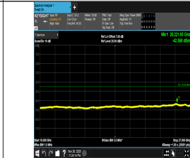
Band7-20MHz-16QAM-21100-1RB#0-18000~27000-PASS
