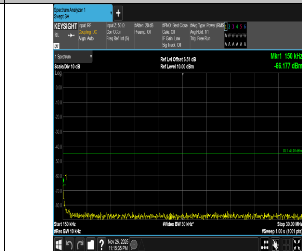
Band7-20MHz-QPSK-20850-1RB#99-0.15~30-PASS
