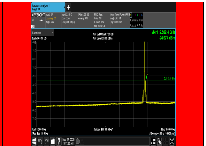
Band7-15MHz-16QAM-21375-1RB#0-1000~3000-FAIL
