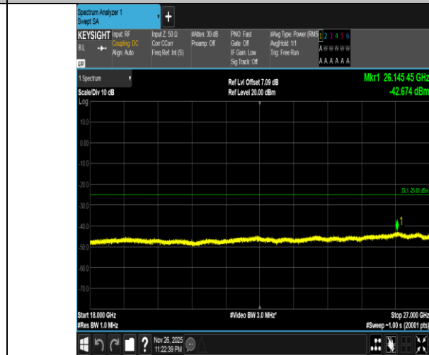
Band7-20MHz-QPSK-21100-1RB#0-18000~27000-PASS
