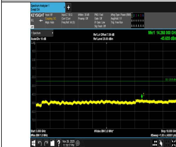
Band7-20MHz-QPSK-20850-100RB#0-3000~18000-PASS
