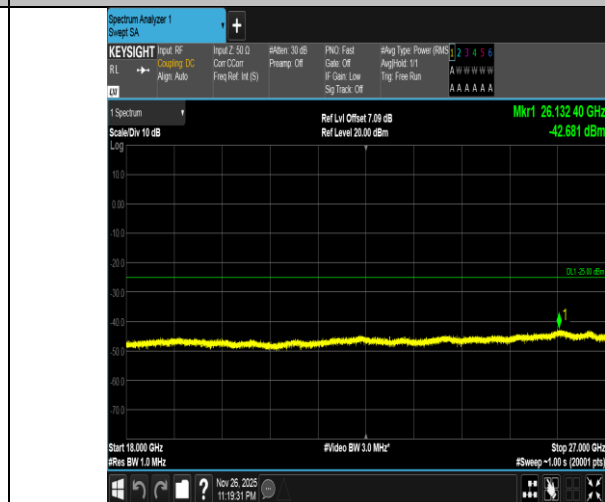
Band7-20MHz-QPSK-20850-100RB#0-18000~27000-PASS
