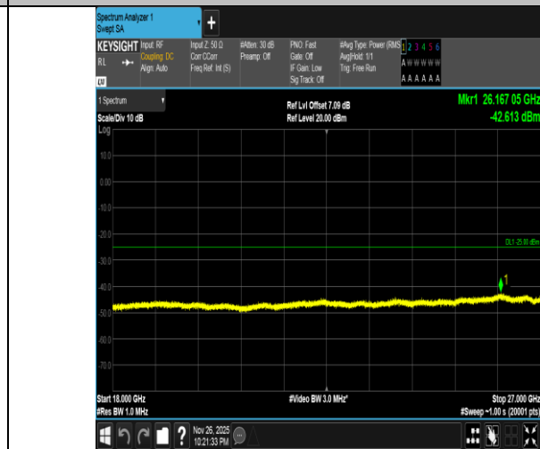
Band7-15MHz-16QAM-21375-1RB#74-18000~27000-PASS
