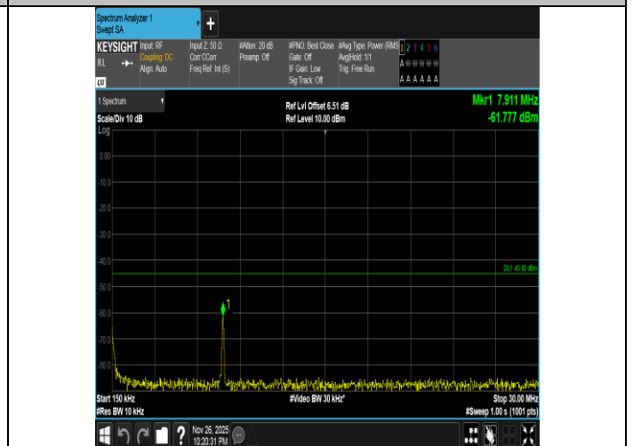
Band7-15MHz-16QAM-21375-1RB#74-0.15~30-PASS
