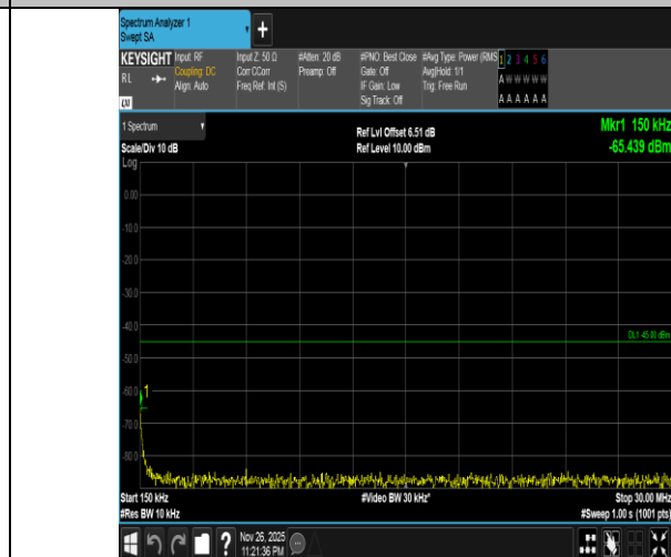
Band7-20MHz-QPSK-21100-1RB#0-0.15~30-PASS
