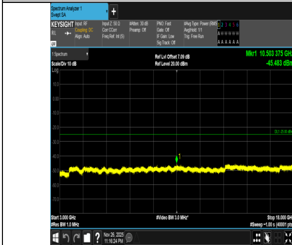
Band7-20MHz-QPSK-20850-1RB#99-3000~18000-PASS
