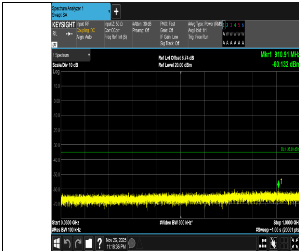
Band7-20MHz-QPSK-20850-100RB#0-30~1000-PASS
