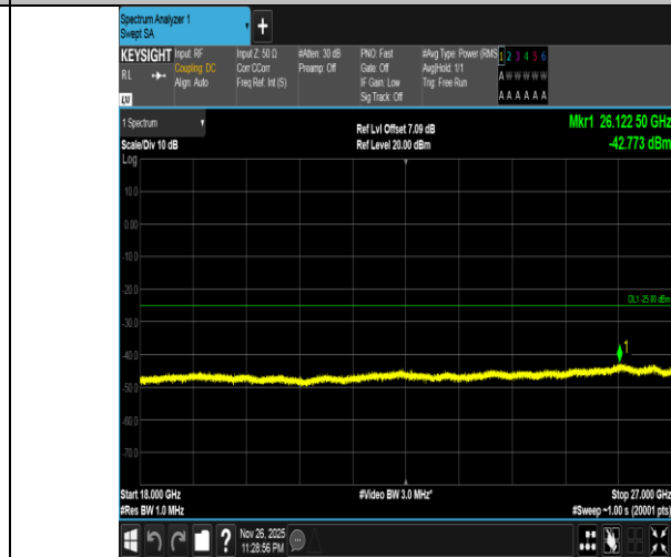
Band7-20MHz-QPSK-21100-100RB#0-18000~27000-PASS
