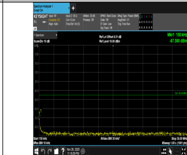
Band7-20MHz-16QAM-20850-1RB#99-0.15~30-PASS
