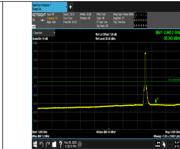
Band7-20MHz-16QAM-20850-100RB#0-1000~3000-PASS
