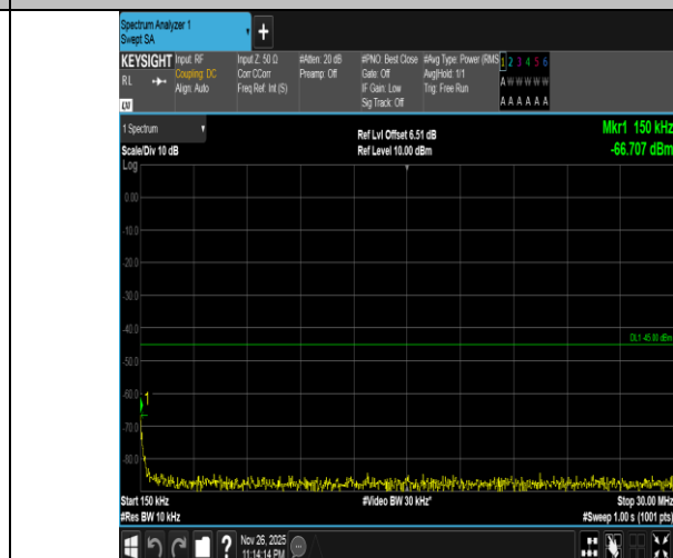
Band7-20MHz-16QAM-20850-1RB#0-0.15~30-PASS
