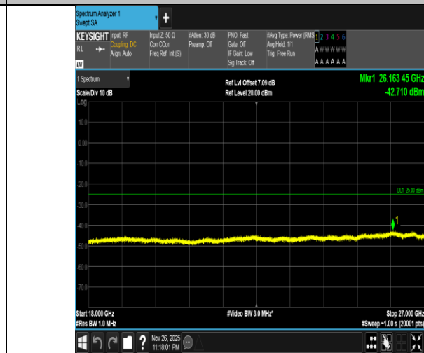
Band7-20MHz-16QAM-20850-1RB#99-18000~27000-PASS
