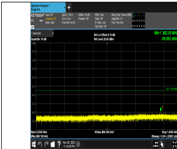
Band7-20MHz-16QAM-20850-1RB#0-30~1000-PASS
