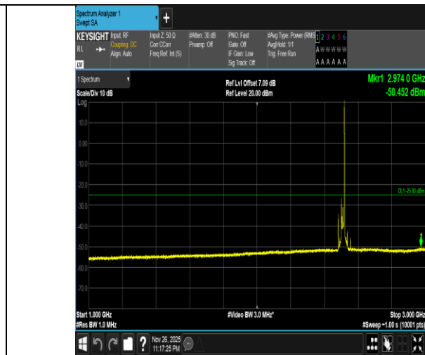
Band7-20MHz-16QAM-20850-1RB#99-1000~3000-PASS
