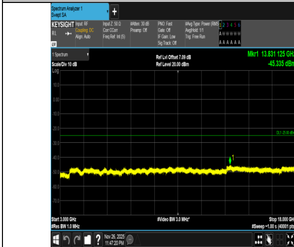
Band7-20MHz-QPSK-21350-100RB#0-3000~18000-PASS
