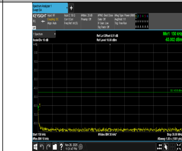
Band7-20MHz-QPSK-21350-1RB#0-0.15~30-PASS
