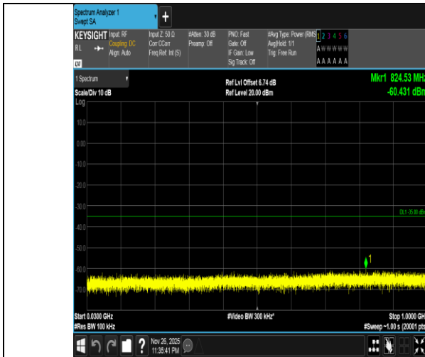
Band7-20MHz-16QAM-21350-1RB#0-30~1000-PASS
