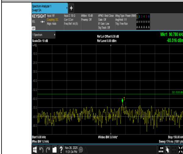
Band7-20MHz-QPSK-21350-1RB#0-0.009~0.15-PASS
