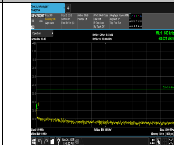
Band7-20MHz-16QAM-21350-100RB#0-0.15~30-PASS
