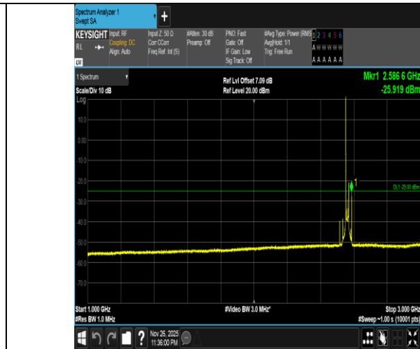
Band7-20MHz-16QAM-21350-1RB#0-1000~3000-PASS
