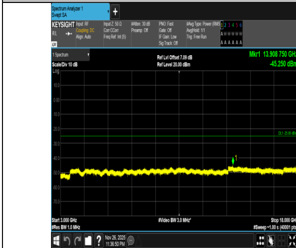
Band7-20MHz-16QAM-21350-1RB#0-3000~18000-PASS
