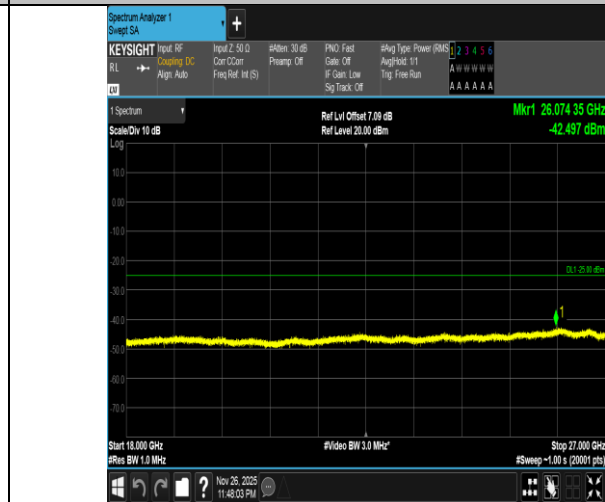
Band7-20MHz-QPSK-21350-100RB#0-18000~27000-PASS
