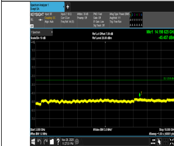
Band7-20MHz-16QAM-21100-1RB#99-3000~18000-PASS
