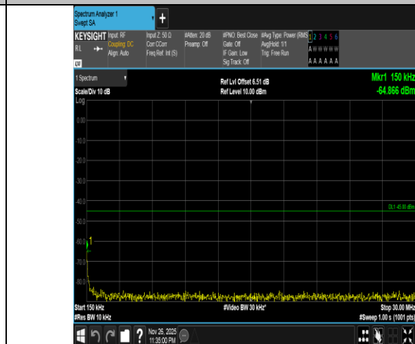
Band7-20MHz-16QAM-21350-1RB#0-0.15~30-PASS
