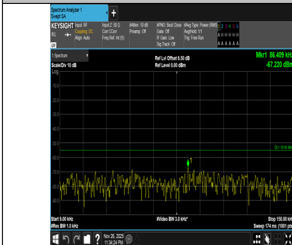
Band7-20MHz-16QAM-21350-1RB#0-0.009~0.15-PASS
