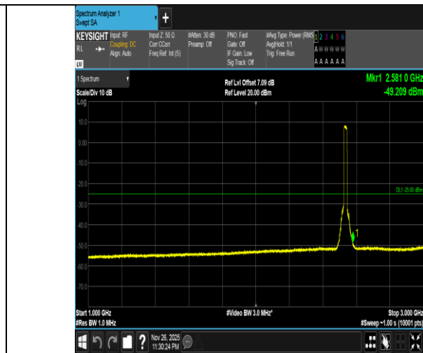
Band7-20MHz-16QAM-21100-100RB#0-1000~3000-PASS
