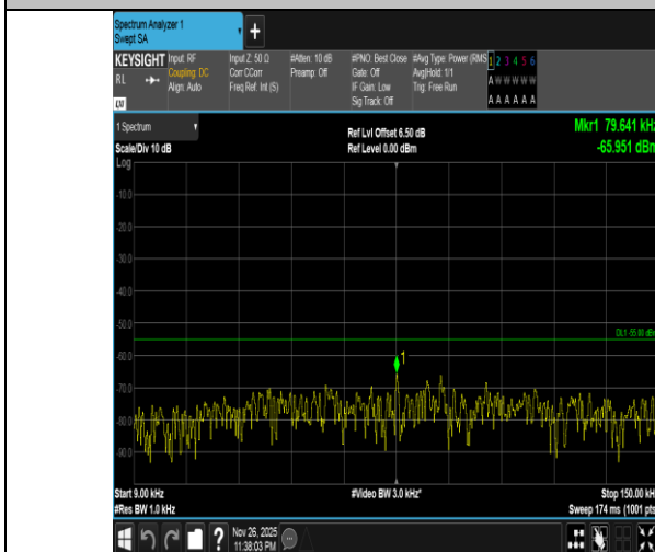
Band7-20MHz-QPSK-21350-1RB#99-0.009~0.15-PASS
