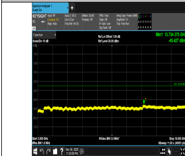
Band7-20MHz-QPSK-21350-1RB#0-3000~18000-PASS
