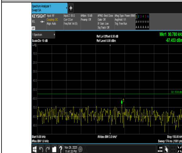
Band7-20MHz-16QAM-21350-1RB#99-0.009~0.15-PASS
