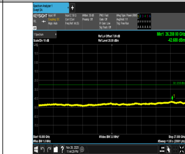
Band7-20MHz-16QAM-21350-1RB#99-18000~27000-PASS
