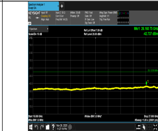
Band7-20MHz-16QAM-21100-1RB#99-18000~27000-PASS
