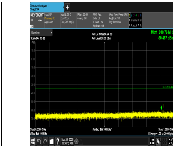
Band7-20MHz-16QAM-21100-100RB#0-30~1000-PASS
