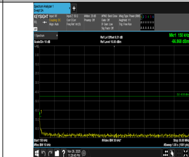
Band7-20MHz-16QAM-21100-100RB#0-0.15~30-PASS
