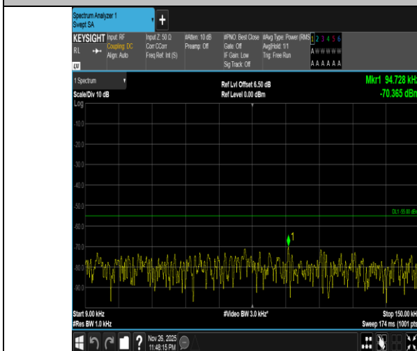
Band7-20MHz-16QAM-21350-100RB#0-0.009~0.15-PASS
