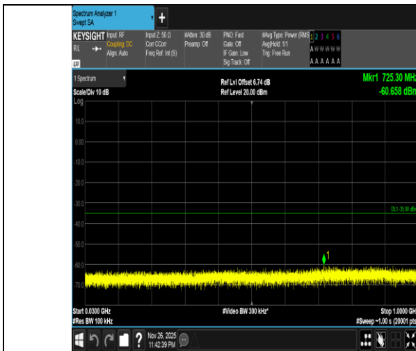
Band7-20MHz-16QAM-21350-1RB#99-30~1000-PASS
