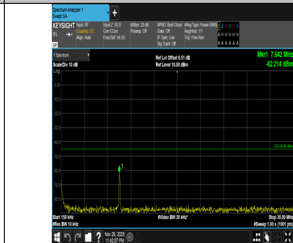
Band7-20MHz-16QAM-21350-1RB#99-0.15~30-PASS
