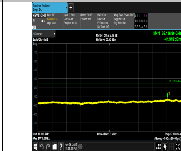
Band7-20MHz-QPSK-21350-1RB#0-18000~27000-PASS
