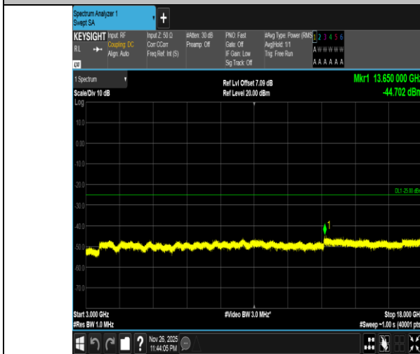
Band7-20MHz-16QAM-21350-1RB#99-3000~18000-PASS
