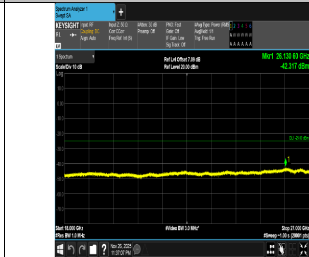
Band7-20MHz-16QAM-21350-1RB#0-18000~27000-PASS
