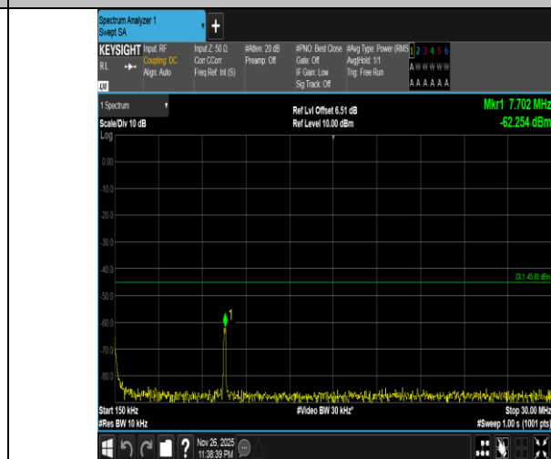
Band7-20MHz-QPSK-21350-1RB#99-0.15~30-PASS
