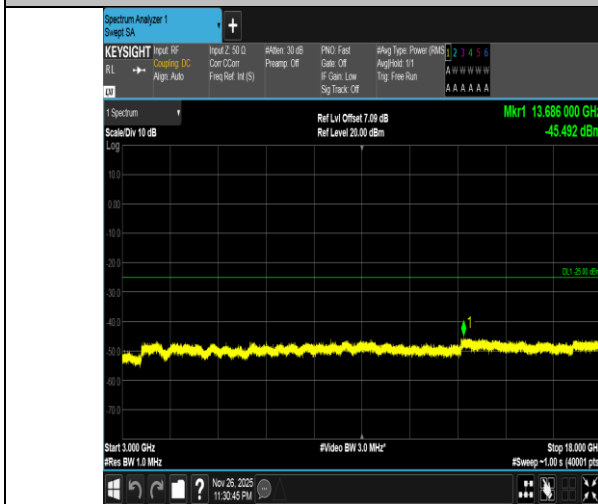
Band7-20MHz-16QAM-21100-100RB#0-3000~18000-PASS
