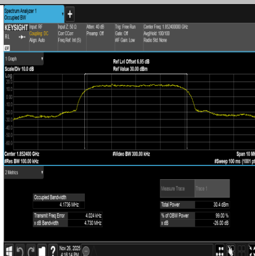
Band2-9262-3-PASS
