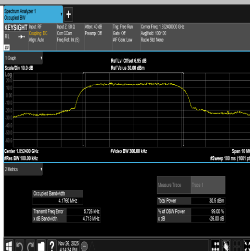
Band2-9262-2-PASS
