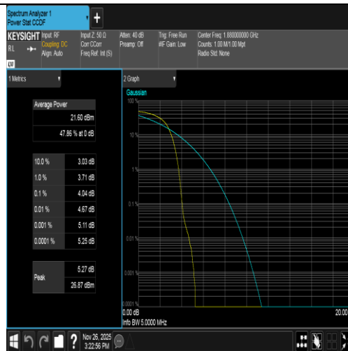
Band2-9400-3-PASS
