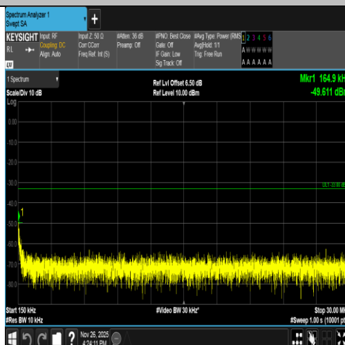
Band2-9538-1-0.15~30MHz-PASS
