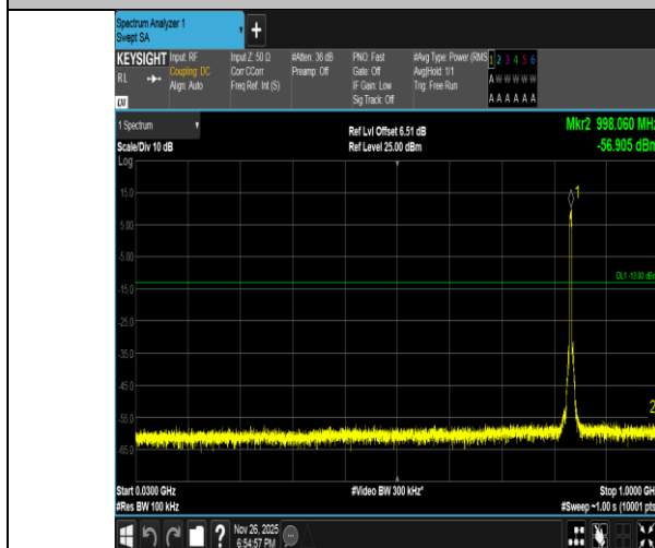
Band5-4182-30~1000MHz-PASS
