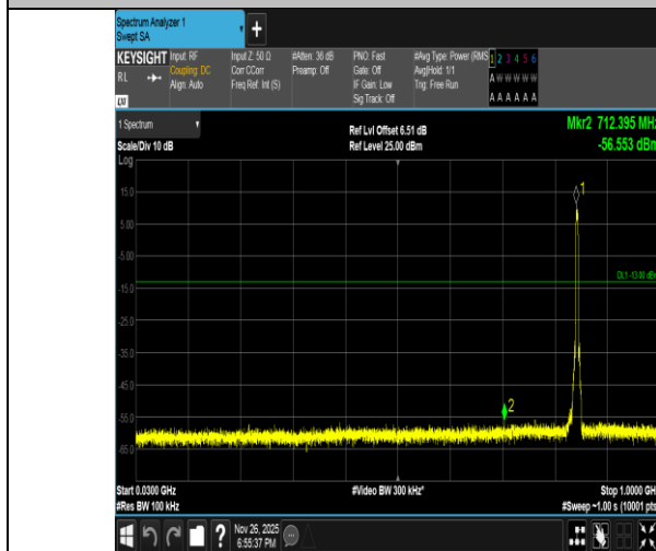
Band5-4233-30~1000MHz-PASS
