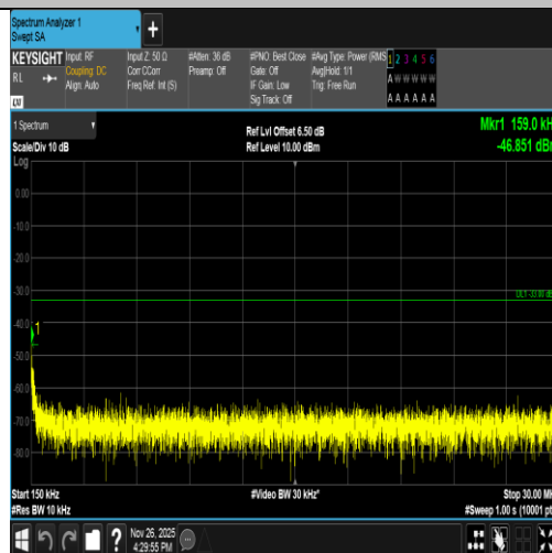
Band2-9262-4-0.15~30MHz-PASS
