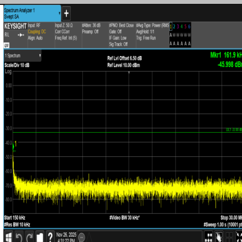
Band2-9538-4-0.15~30MHz-PASS
