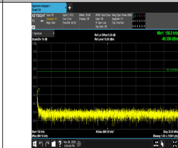
Band5-4182-0.15~30MHz-PASS
