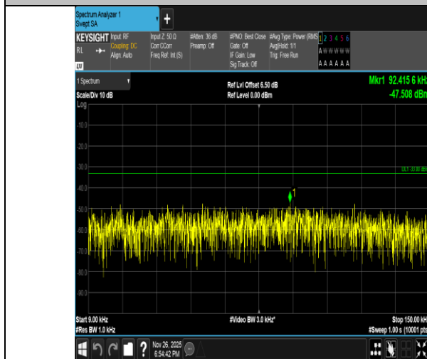
Band5-4182-0.009~0.15MHz-PASS
