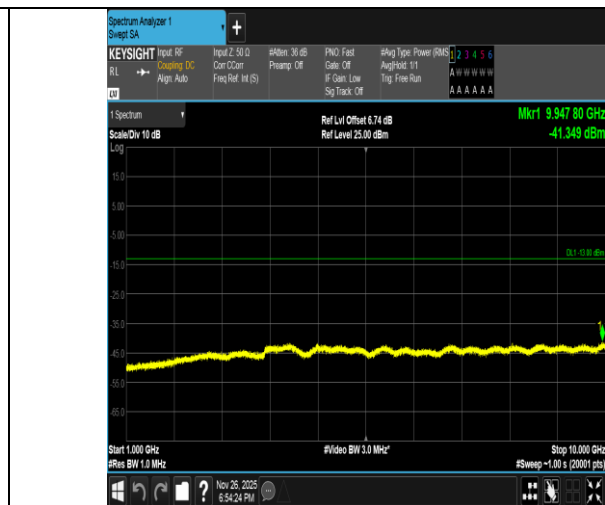
Band5-4132-1000~10000MHz-PASS
