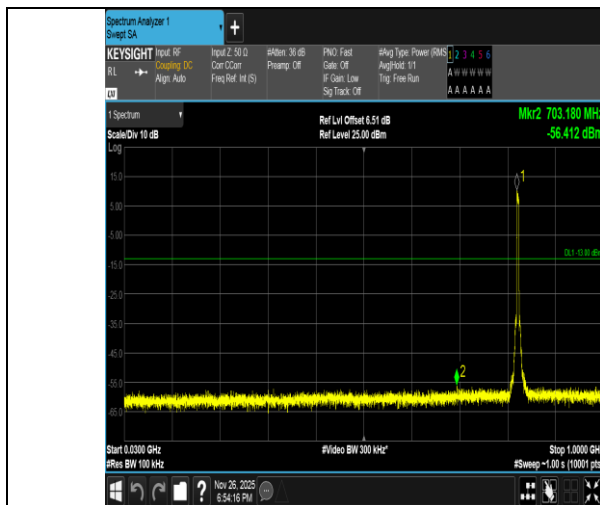
Band5-4132-30~1000MHz-PASS
