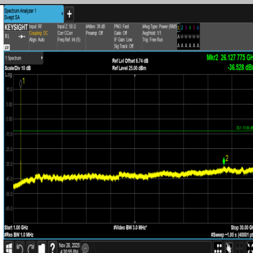
Band2-9400-4-1000~30000MHz-PASS
