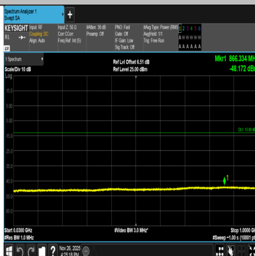
Band2-9262-2-30~1000MHz-PASS
