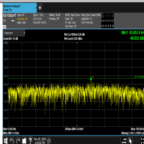
Band2-9262-2-0.009~0.15MHz-PASS
