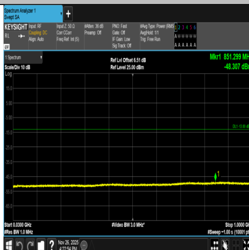
Band2-9262-1-30~1000MHz-PASS
