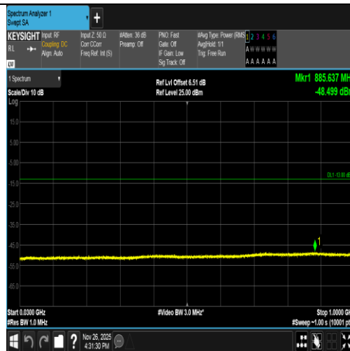
Band2-9538-4-30~1000MHz-PASS
