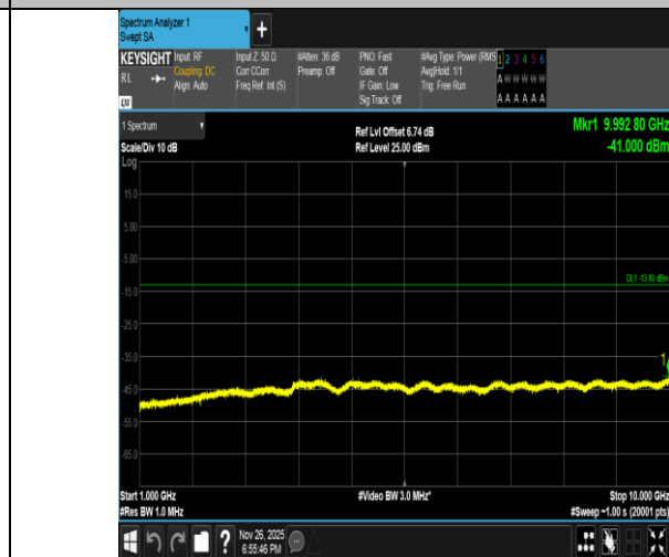
Band5-4233-1000~10000MHz-PASS
