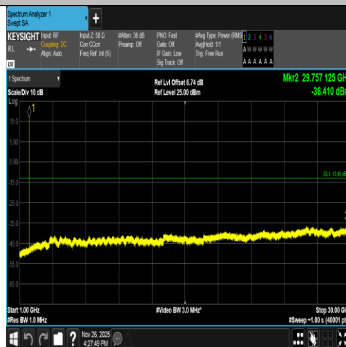
Band2-9262-3-1000~30000MHz-PASS
