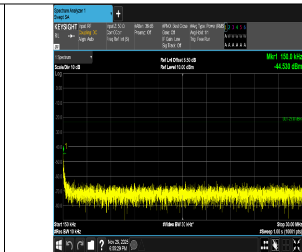
Band5-4233-0.15~30MHz-PASS
