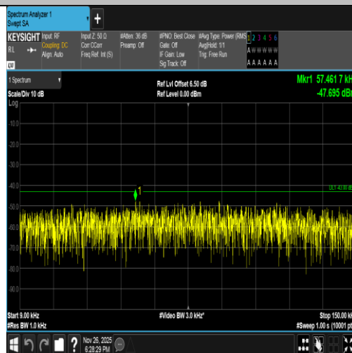
Band2-9400-1-0.009~0.15MHz-PASS
