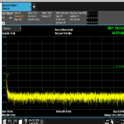
Band2-9400-4-0.15~30MHz-PASS
