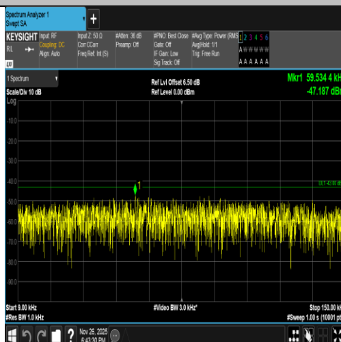
Band2-9262-5-0.009~0.15MHz-PASS
