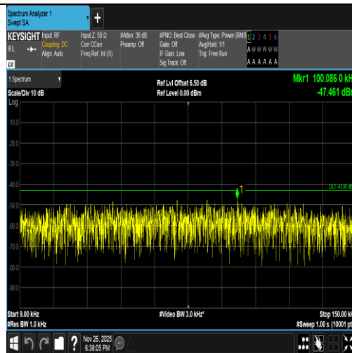
Band2-9538-3-0.009~0.15MHz-PASS
