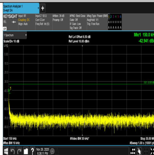
Band2-9538-3-0.15~30MHz-PASS
