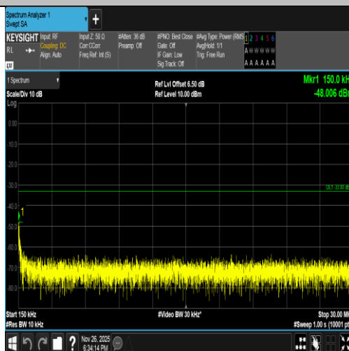
Band2-9538-2-0.15~30MHz-PASS
