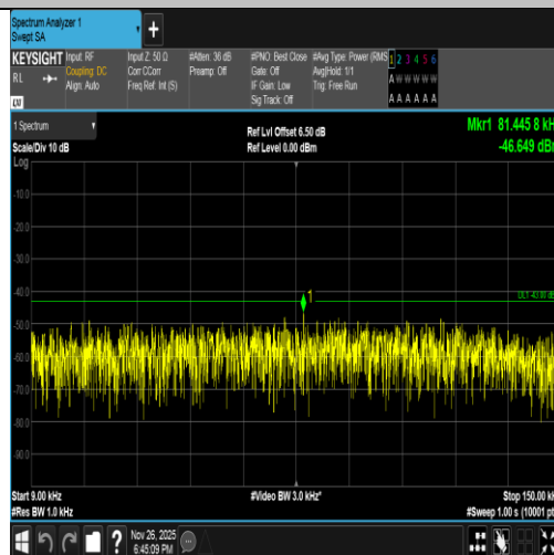
Band2-9538-5-0.009~0.15MHz-PASS
