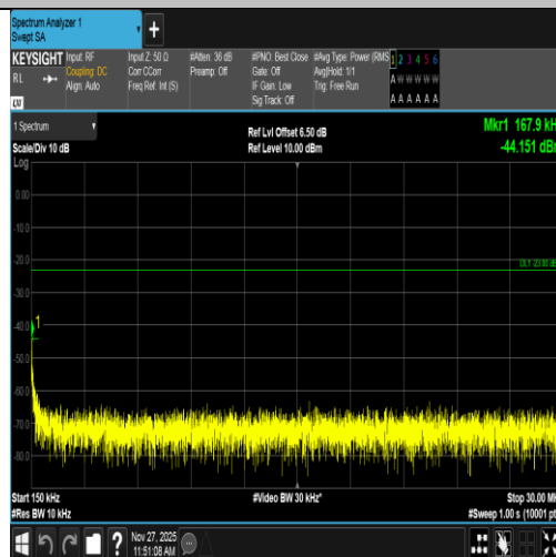
Band5-4182-5-0.15~30MHz-PASS
