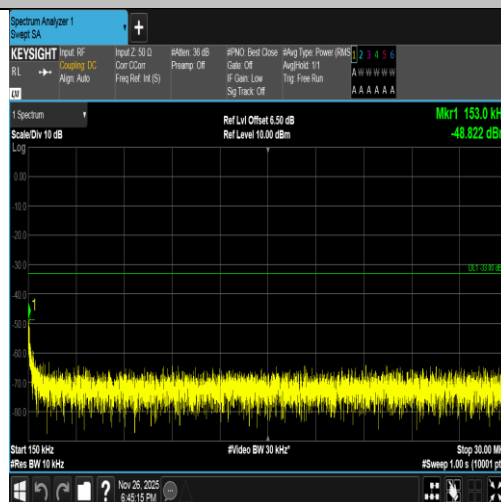
Band2-9538-5-0.15~30MHz-PASS
