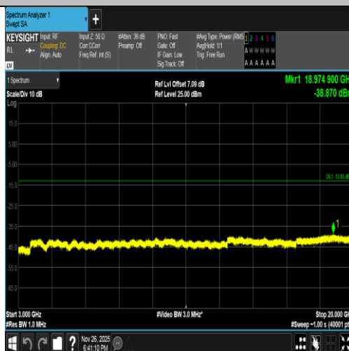
Band2-9400-4-3000~20000MHz-PASS
