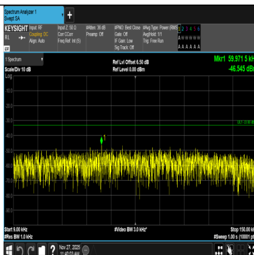
Band5-4182-2-0.009~0.15MHz-PASS
