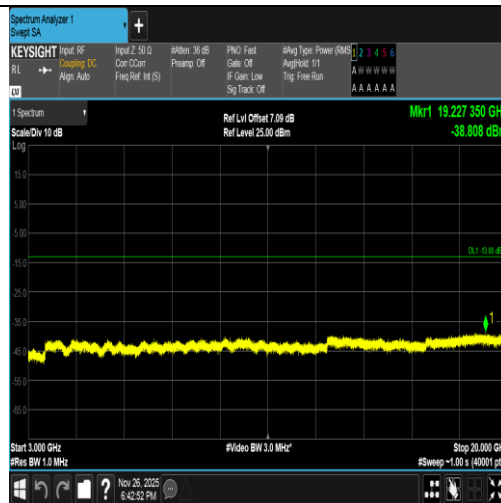
Band2-9538-4-3000~20000MHz-PASS
