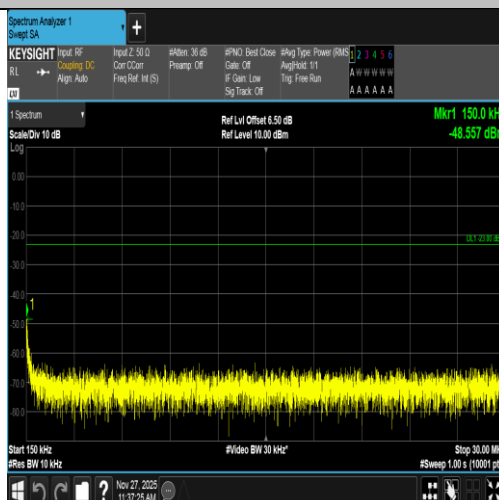
Band5-4233-1-0.15~30MHz-PASS
