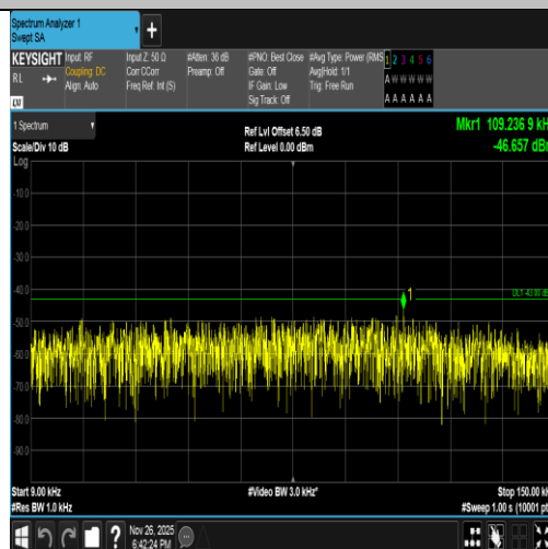
Band2-9538-4-0.009~0.15MHz-PASS
