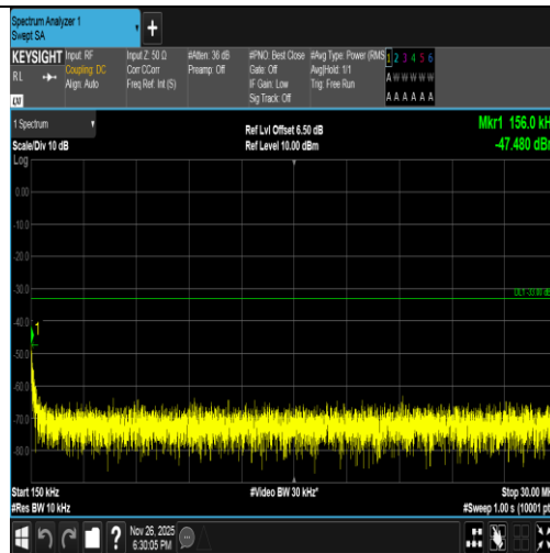
Band2-9538-1-0.15~30MHz-PASS
