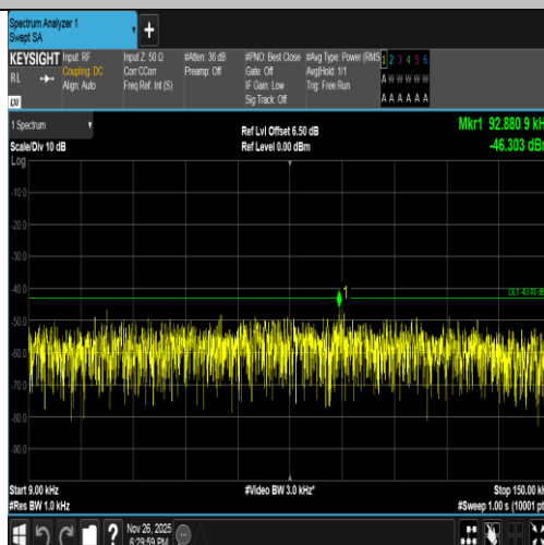
Band2-9538-1-0.009~0.15MHz-PASS
