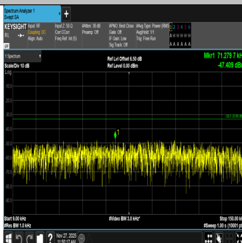
Band5-4132-5-0.009~0.15MHz-PASS
