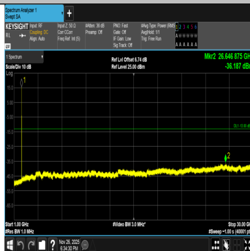
Band2-9538-2-1000~30000MHz-PASS
