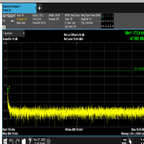
Band5-4132-1-0.15~30MHz-PASS
