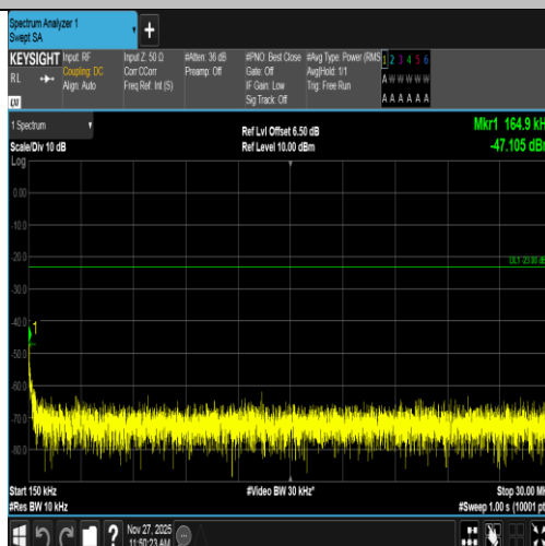
Band5-4132-5-0.15~30MHz-PASS
