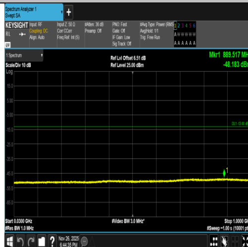
Band2-9400-5-30~1000MHz-PASS
