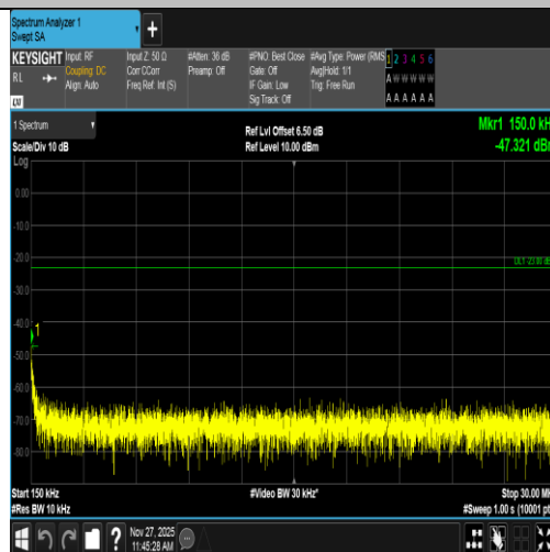
Band5-4233-3-0.15~30MHz-PASS
