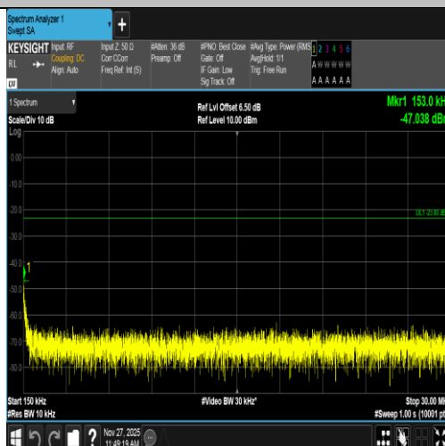
Band5-4233-4-0.15~30MHz-PASS
