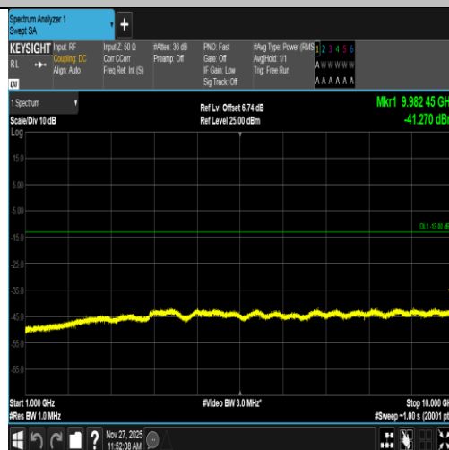
Band5-4233-5-1000~10000MHz-PASS
