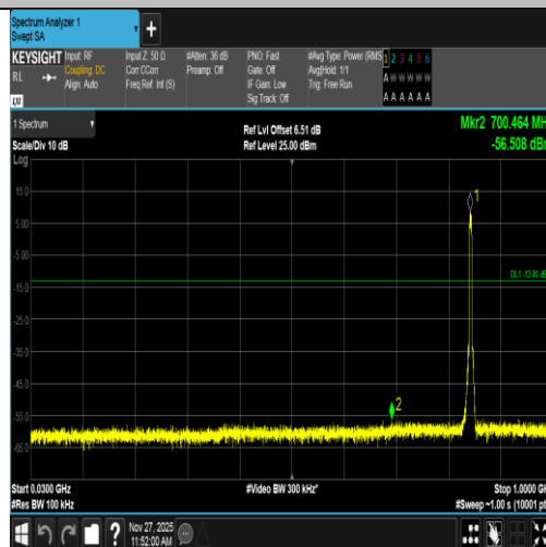
Band5-4233-5-30~1000MHz-PASS
