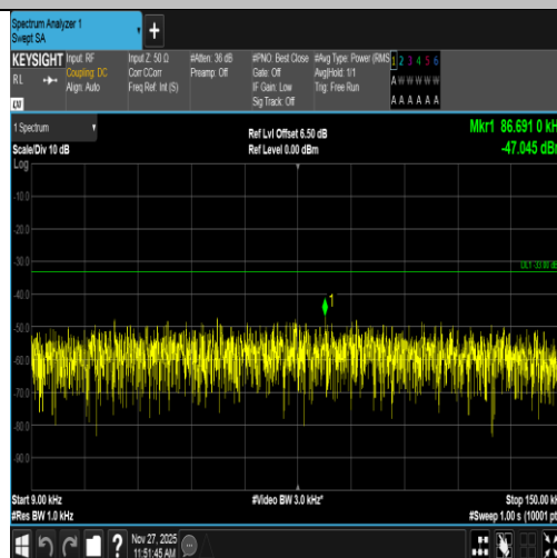
Band5-4233-5-0.009~0.15MHz-PASS
