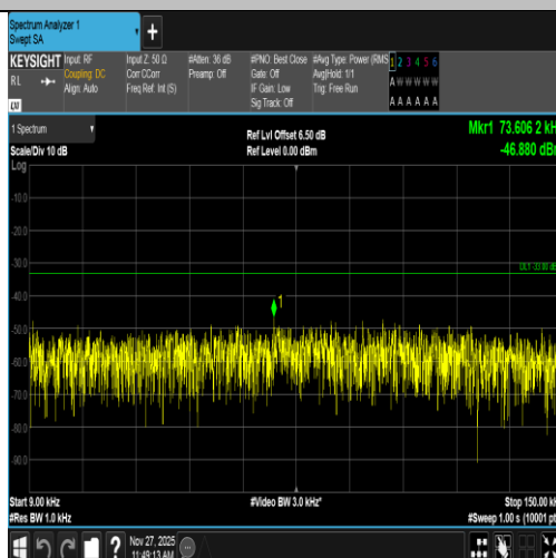
Band5-4233-4-0.009~0.15MHz-PASS
