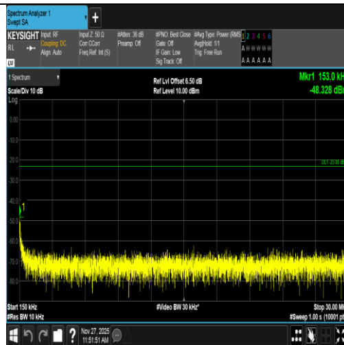
Band5-4233-5-0.15~30MHz-PASS
