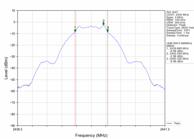
1M_MCH_2440MHz_Ant1_NTNV
