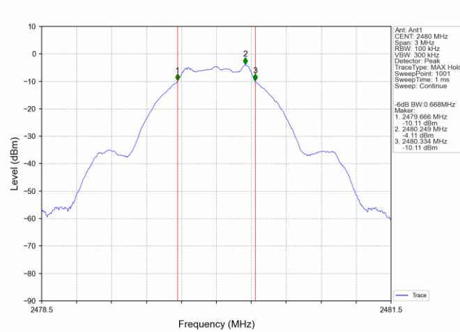
1M_HCH_2480MHz_Ant1_NTNV
