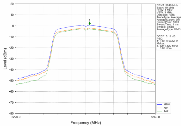
802.11ax(HEW20)_HCH_5240MHz_SU_/_MIMO_NTNV
