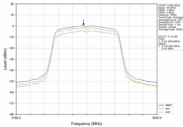
802.11ax(HEW20)_LCH_5180MHz_SU_/_MIMO_NTNV
