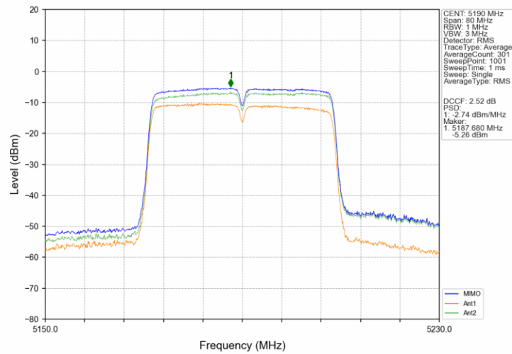
802.11ac(VHT40)_LCH_5190MHz_MIMO_NTNV
