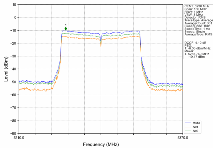
802.11ac(VHT80)_MCH_5290MHz_MIMO_NTNV
