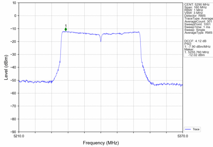
802.11ac(VHT80)_MCH_5290MHz_MIMO_NTNV
