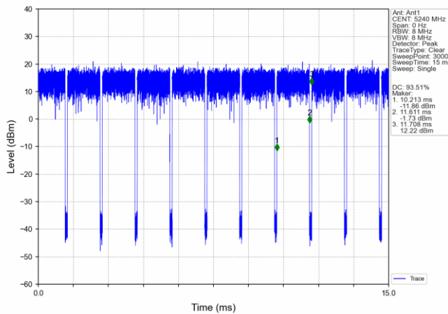
802.11a_HCH_5240MHz_Ant1_NTNV
