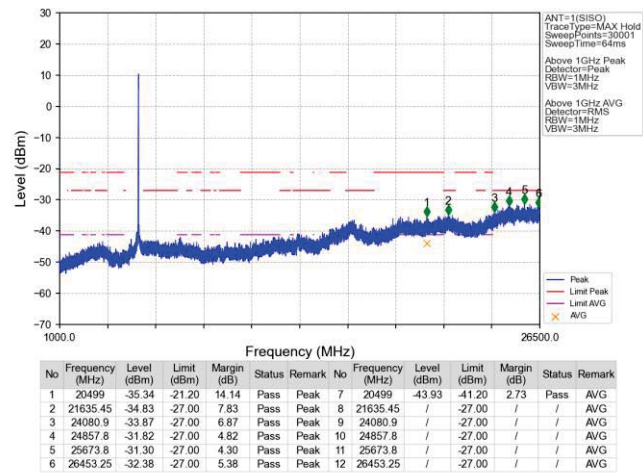
802.11a_LCH_5180MHz_Ant1_NTNV
