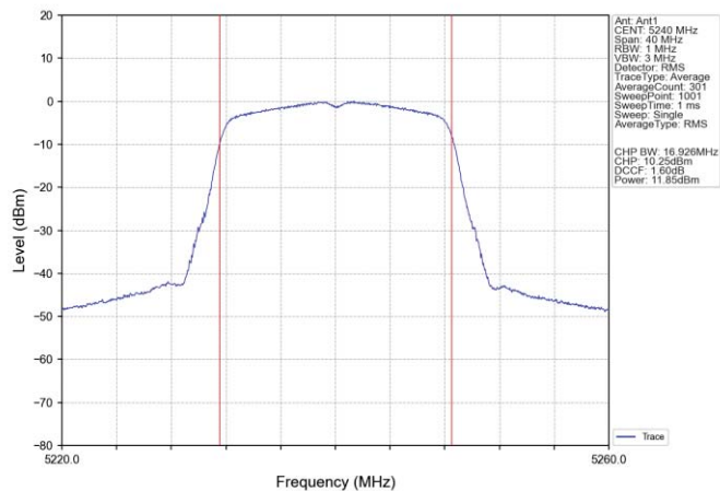
802.11a_HCH_5240MHz_Ant1_NTNV
