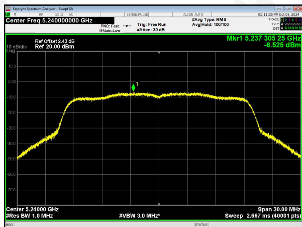
(802.11ax20) PSD plot on channel 48
