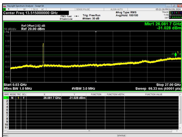
802.11ax80 on channel 42
