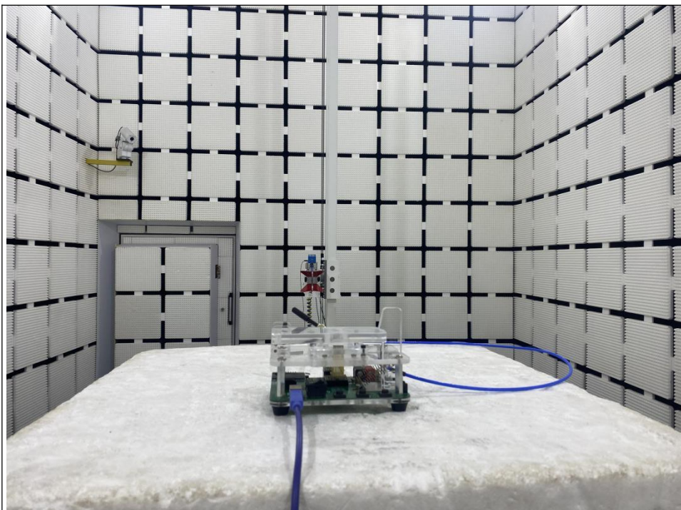
RADIATED EMISSION TEST 1GHz-18GHz-2
