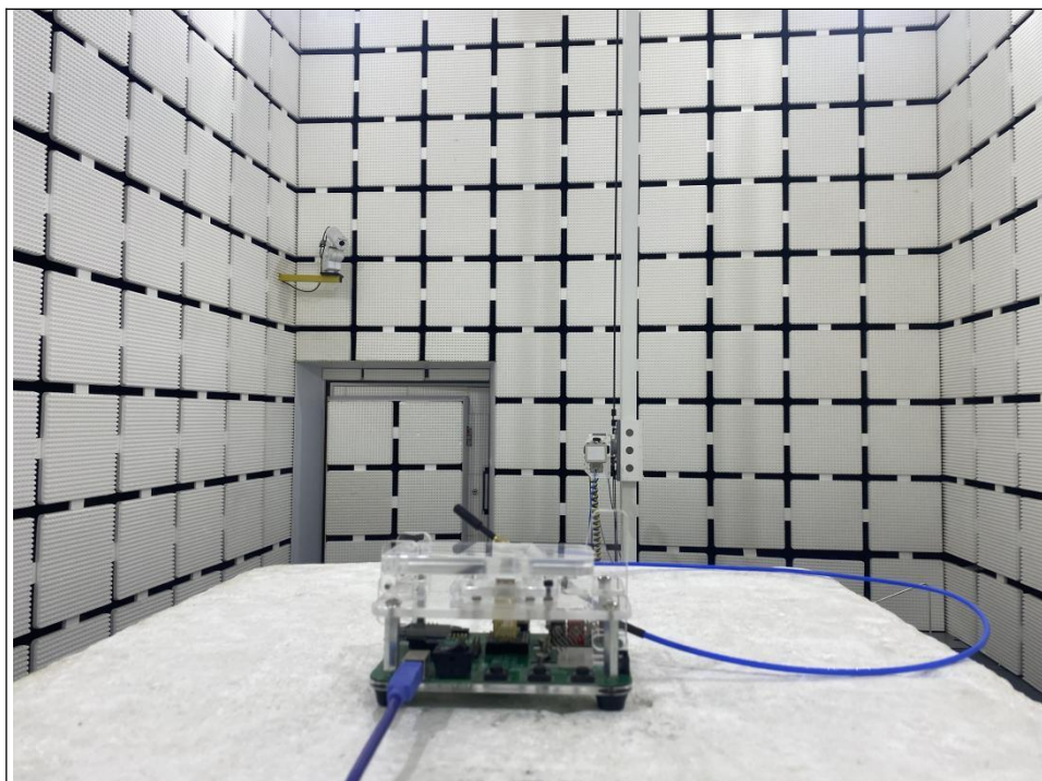
RADIATED EMISSION TEST 18GHz-40GHz-2
