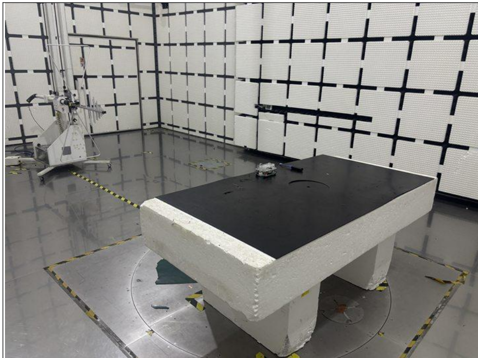
RADIATED EMISSION TEST BELOW 1GHz-1
