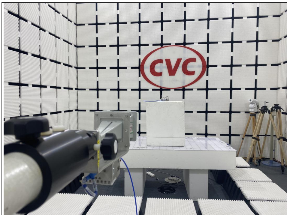
RADIATED EMISSION TEST 18GHz-40GHz-1
