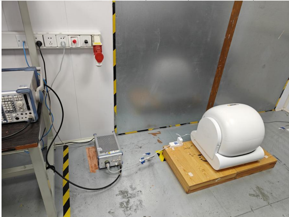
Conducted emissions at AC power line (150 kHz-30 MHz)
