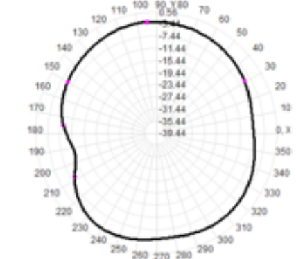
Total(H-XY), Max=-2.64dB, CrD=9.03
