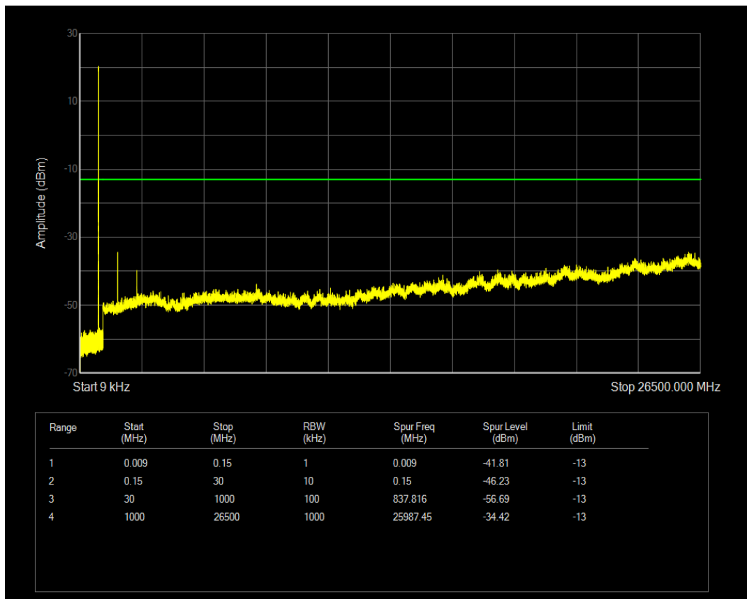
Band26a 16QAM BW=1.4MHz Channel=26697 RB Size=1 Position=#0
