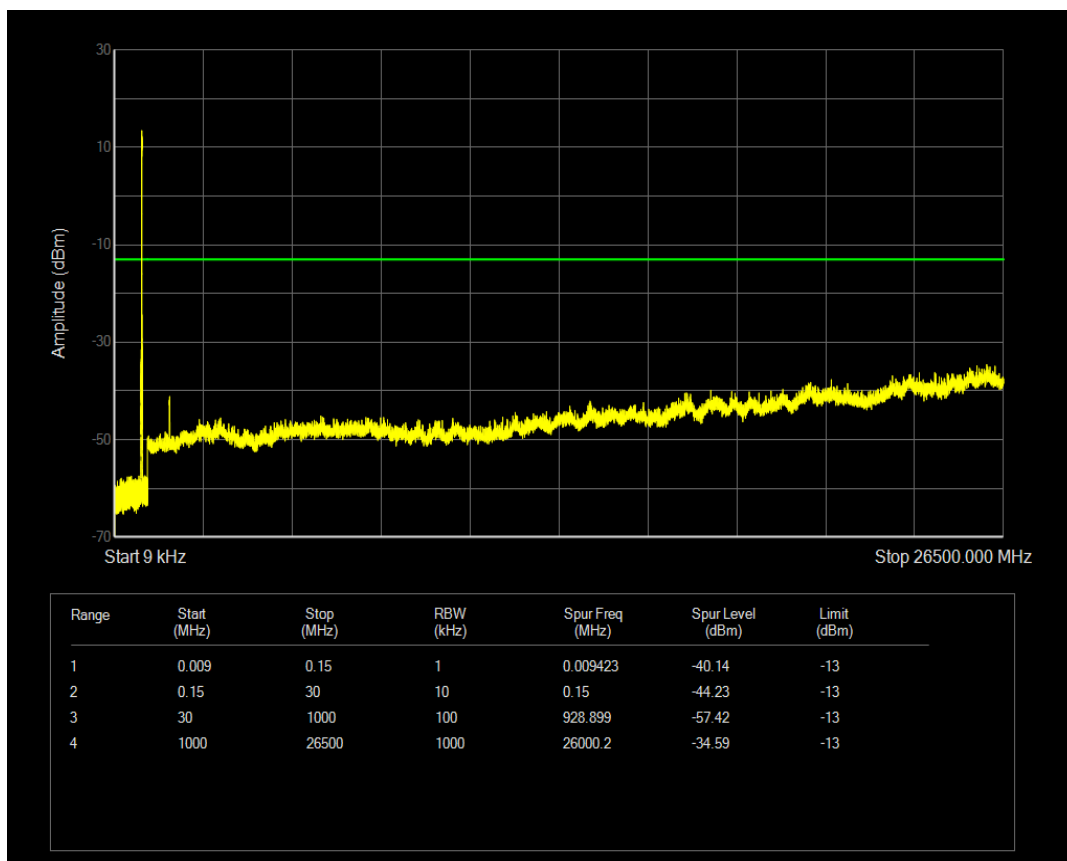
Band26b 16QAM BW=10MHz Channel=26840 RB Size=50 Position=#0
