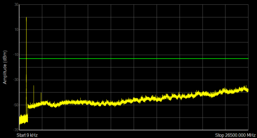
Band26b 16QAM BW=1.4MHz Channel=27033 RB Size=6 Position=#0
