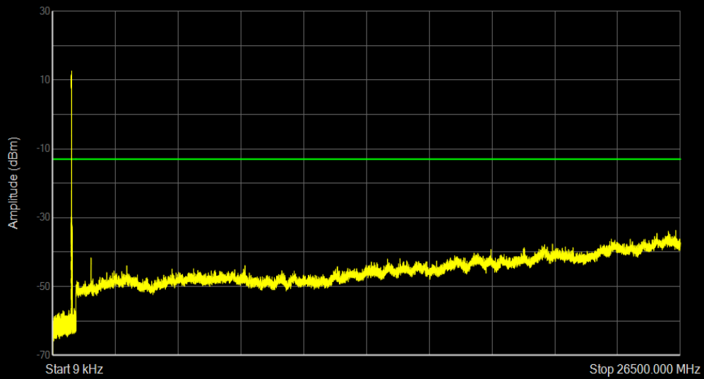
Band26a 16QAM BW=10MHz Channel=26740 RB Size=50 Position=#0
