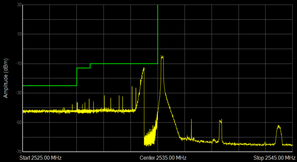
Band41 16QAM BW=5MHz Channel=40065 RB Size=1 Position=#0
