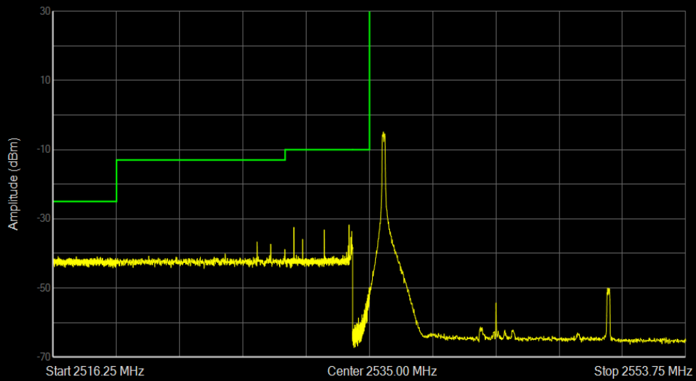
Band41 16QAM BW=15MHz Channel=40115 RB Size=1 Position=#0
