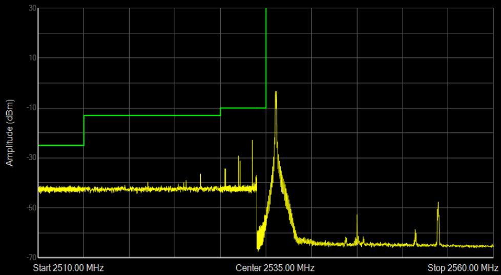
Band41 16QAM BW=20MHz Channel=40140 RB Size=1 Position=#0
