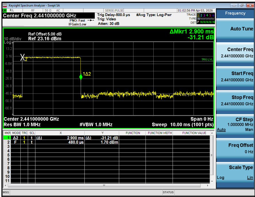
Dwell_Time_(Hopping)_NVNT_ANT1_3-DH5_2441_00_Accumulated
